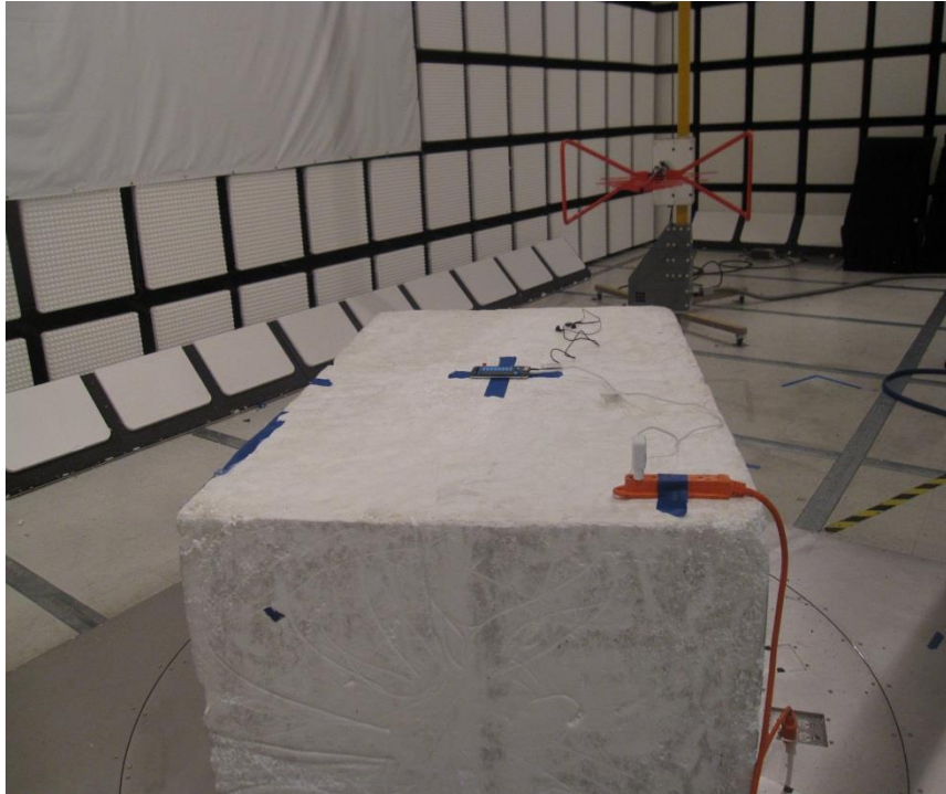
RADIATED BACK PHOTO (BELOW 1 GHz)
