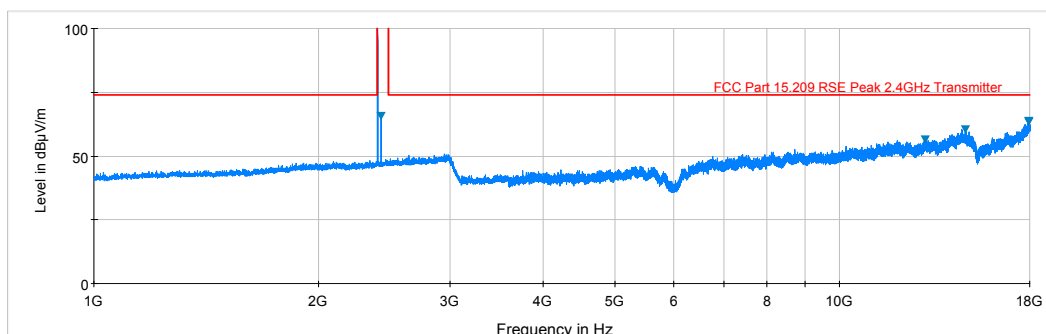
Plot 6-2. Radiated Spurious Plot above 1GHz (BTLE – Ch. 0, Ant. Pol. V)
