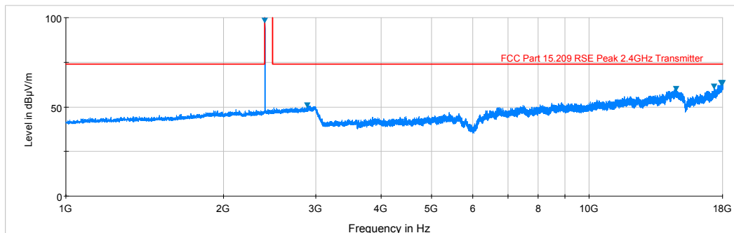
Plot 6-1. Radiated Spurious Plot above 1GHz (BTLE – Ch. 0, Ant. Pol. H)
