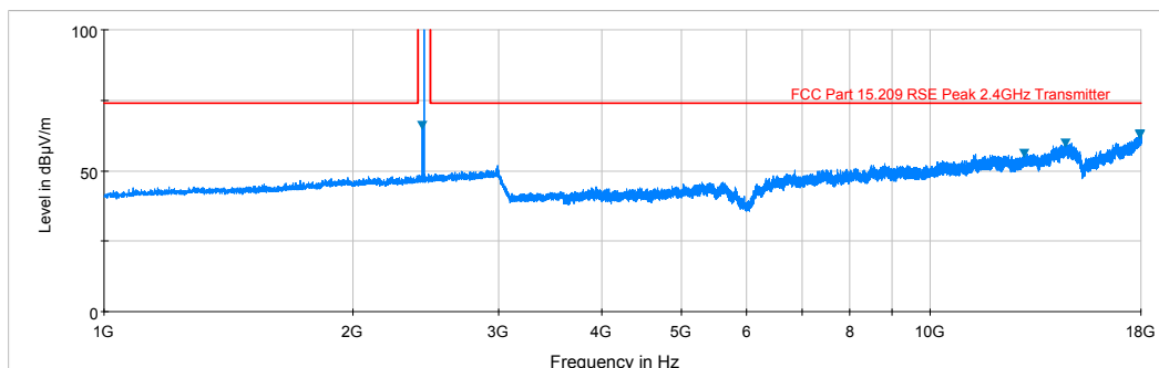
Plot 6-3. Radiated Spurious Plot above 1GHz (BTLE – Ch. 19, Ant. Pol. H)
