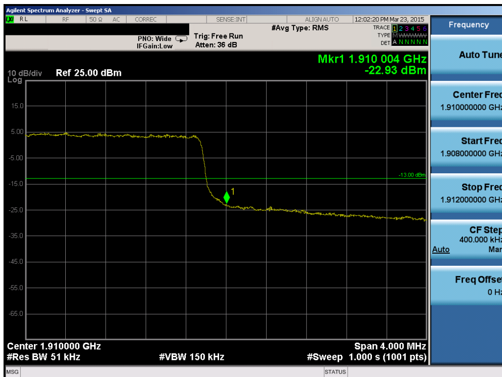
Plot 6-181. Upper Band Edge Plot (Band 2 – 5.0MHz QPSK – RB Size 25)
