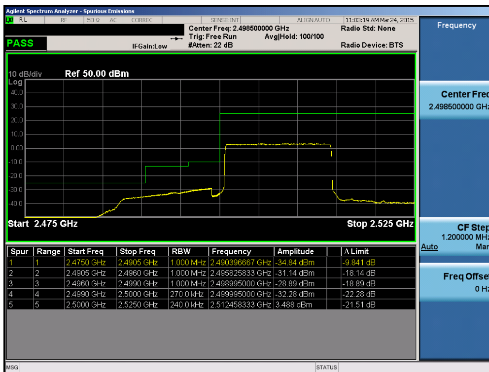
Plot 6-199. Lower ACP Plot (Band 7 – 15.0MHz QPSK – RB Size 75)
