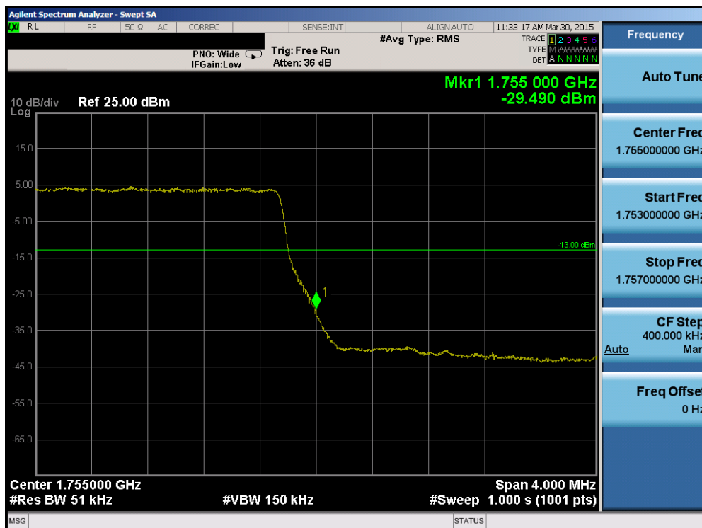
Plot 6-157. Upper Band Edge Plot (Band 4 – 5.0MHz QPSK – RB Size 25)
