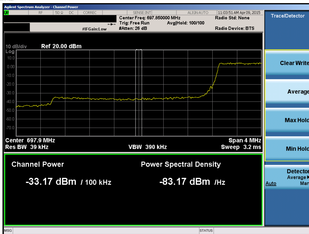
Plot 6-112. Lower Extended Band Edge Plot (Band 12 – 3.0MHz QPSK – RB Size 15)
