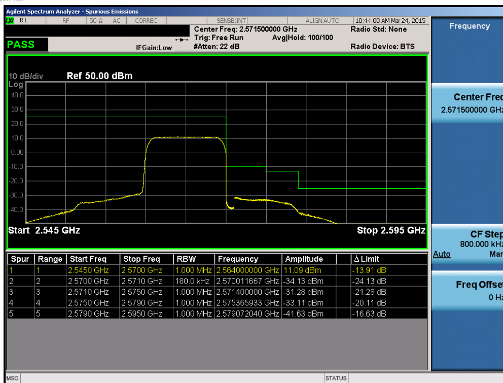
Plot 6-198. Upper ACP Plot (Band 7 – 10.0MHz QPSK – RB Size 50)
