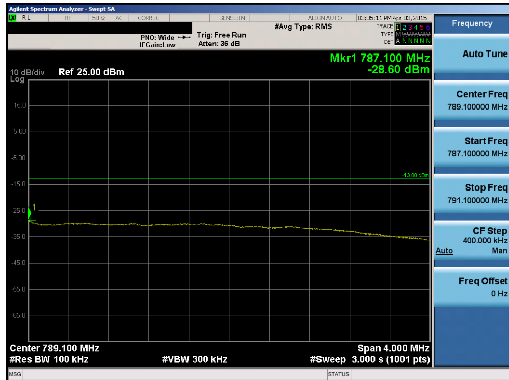
Plot 6-125. Upper Extended Band Edge Plot (Band 13 - 5.0MHz QPSK - RB Size 25)
