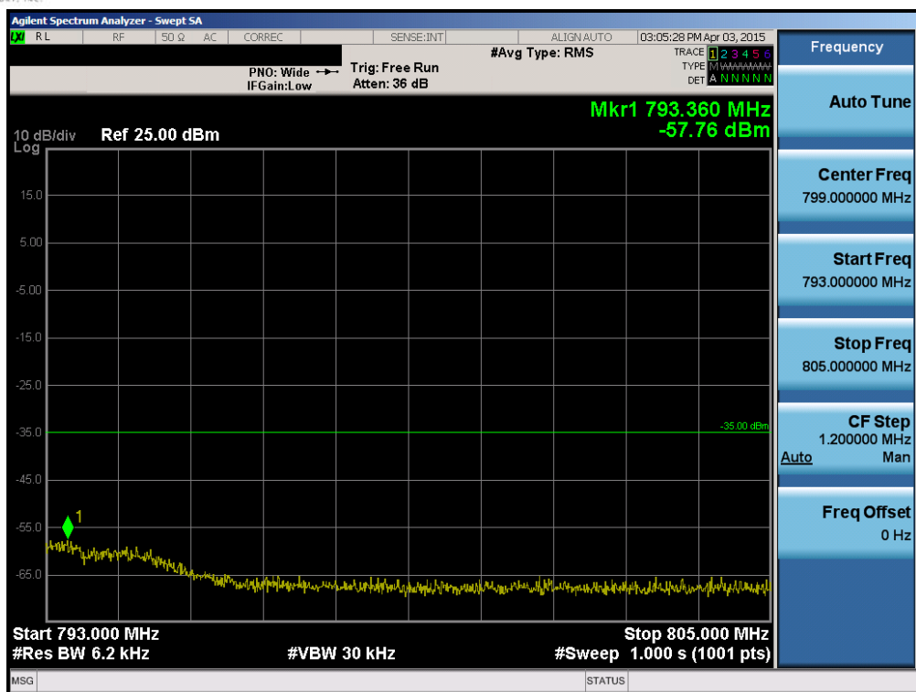
Plot 6-126. Upper Emission Mask Edge Plot (Band 13 – 5.0MHz QPSK – RB Size 25)
