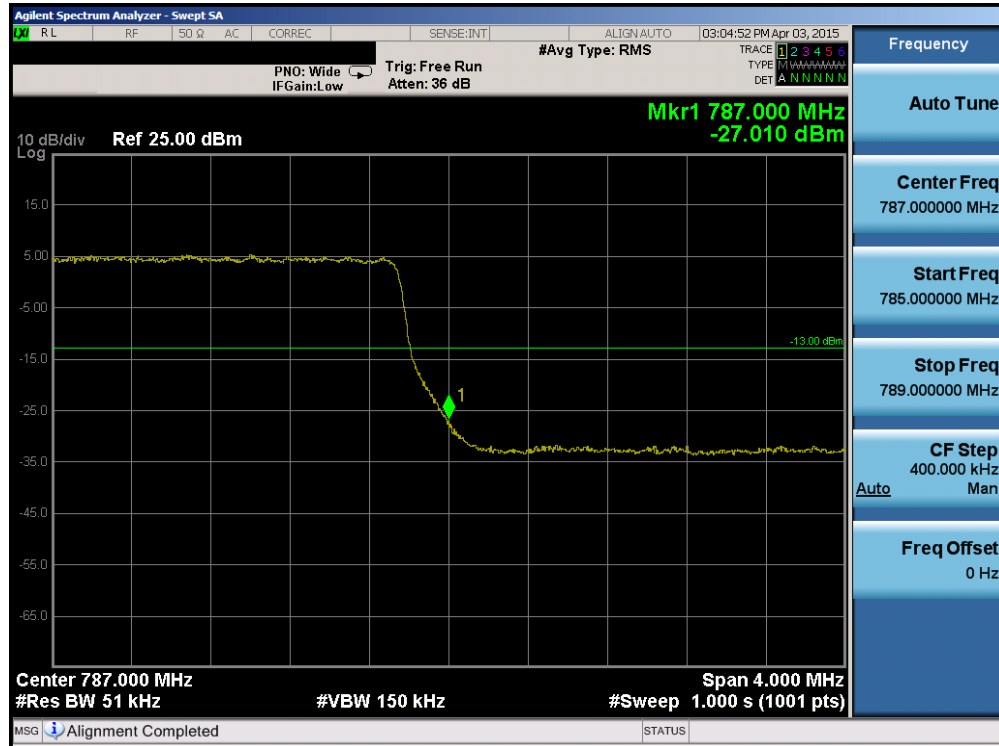
Plot 6-124. Upper Band Edge Plot (Band 13 - 5.0MHz QPSK - RB Size 25)
