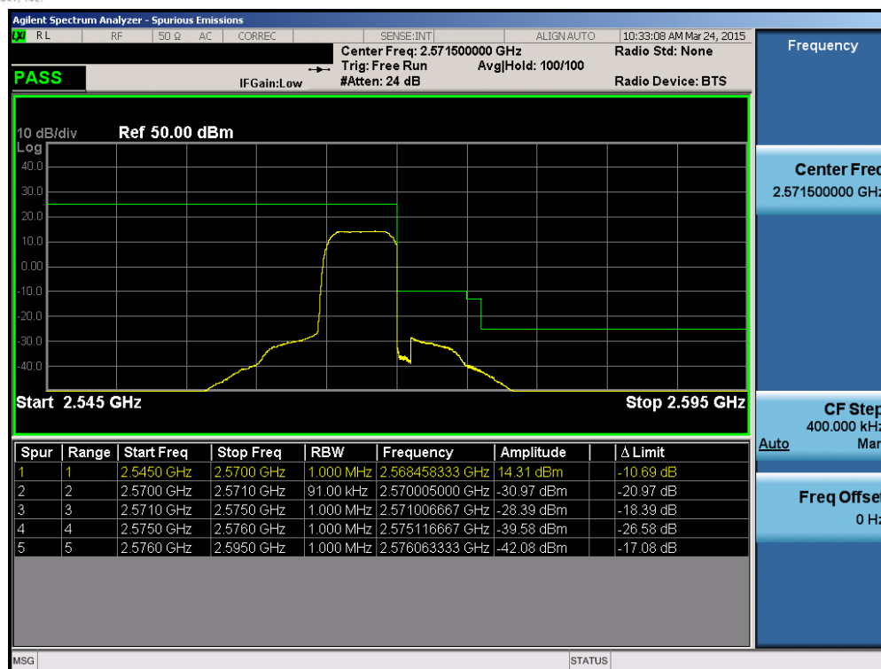
Plot 6-196. Upper ACP Plot (Band 7 – 5.0MHz QPSK – RB Size 25)
