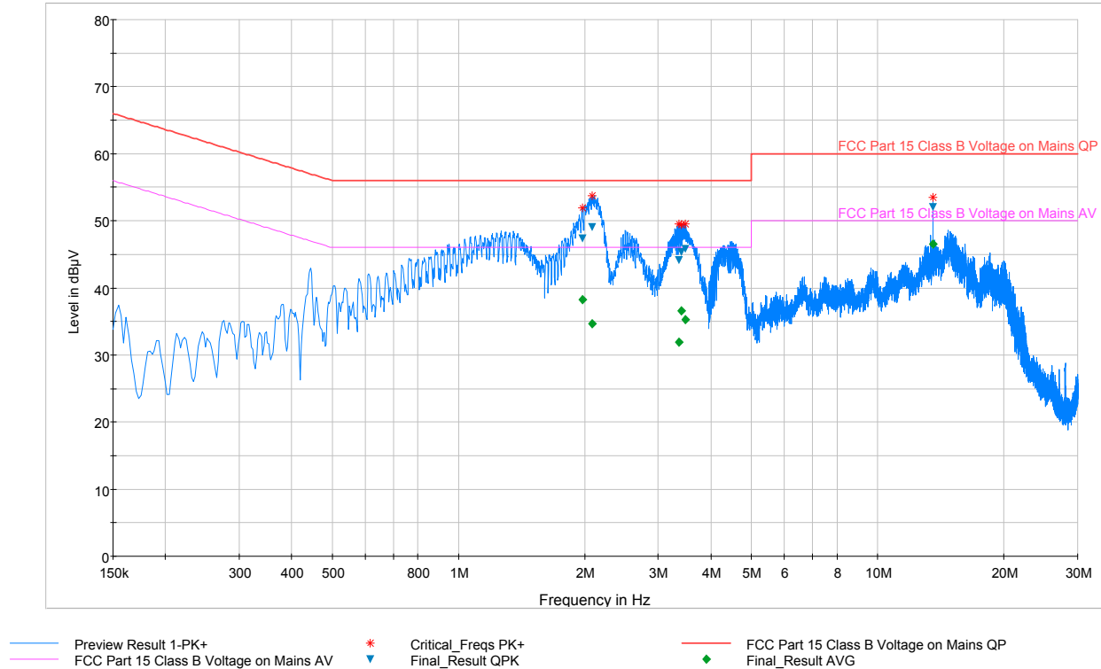
Plot 7-2. Line-Conducted Test Plot (N)
