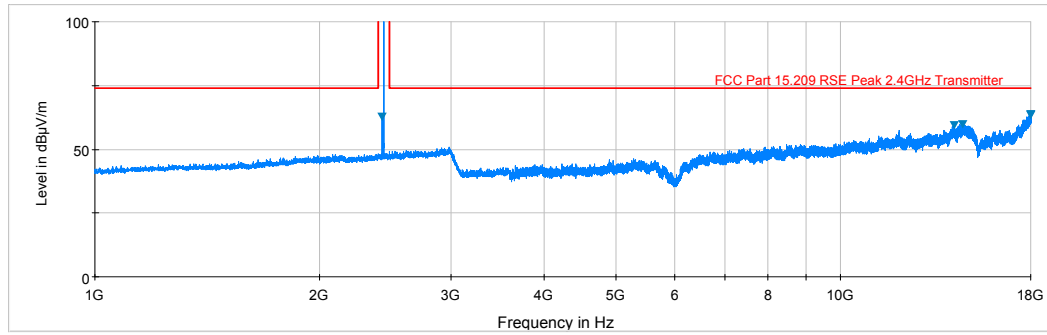
Plot 6-4. Radiated Spurious Plot above 1GHz (BT – Ch. 39, Ant. Pol. V)
