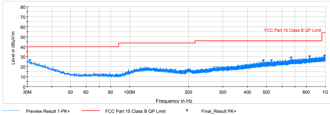
Plot 6-11. Radiated Spurious Plot below 1GHz (Pol. H)
