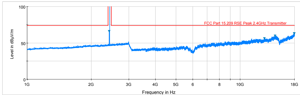
Plot 6-3. Radiated Spurious Plot above 1GHz (BT – Ch. 39, Ant. Pol. H)
