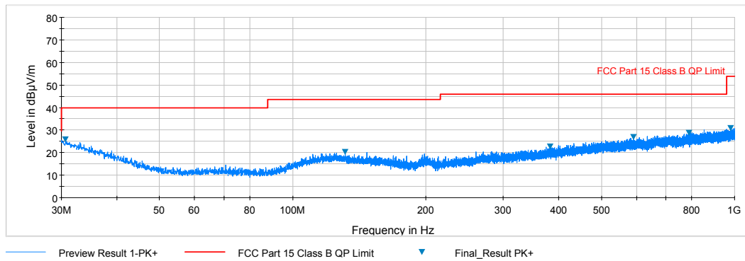
Plot 6-12. Radiated Spurious Plot below 1GHz (Pol. V)
