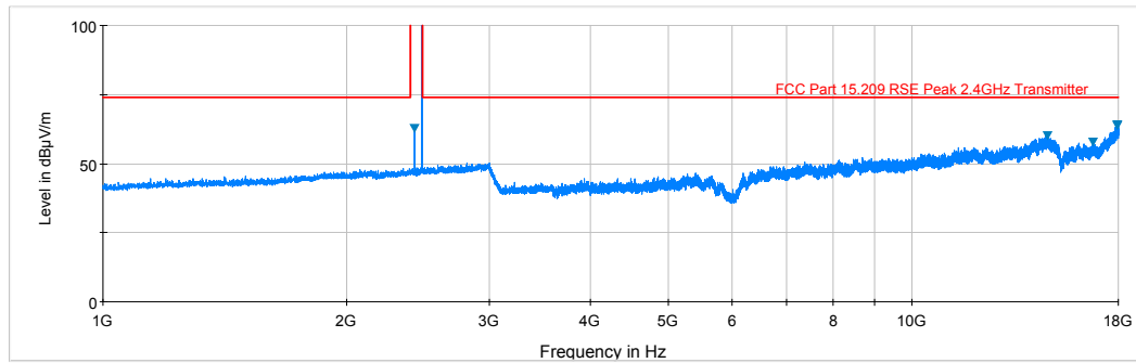
Plot 6-6. Radiated Spurious Plot above 1GHz (BT – Ch. 78, Ant. Pol. V)
