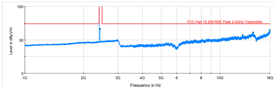
Plot 6-2. Radiated Spurious Plot above 1GHz (BT – Ch. 0, Ant. Pol. V)
