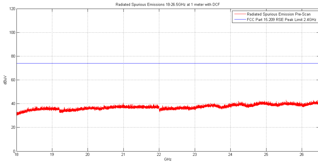
Plot 6-7. Radiated Spurious Plot above 18GHz (Pol. H)
