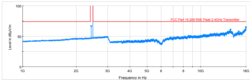
Plot 6-5. Radiated Spurious Plot above 1GHz (BT – Ch. 78, Ant. Pol. H)
