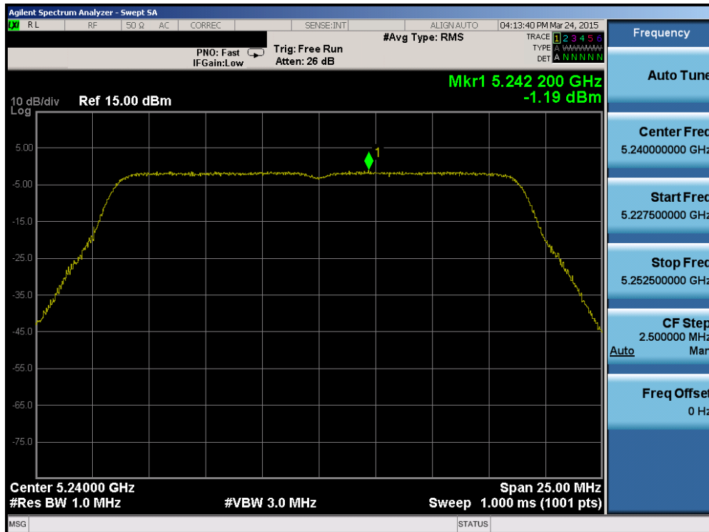
Plot 6-44. Power Spectral Density Plot (20MHz BW 802.11n (UNII Band 1) – Ch. 48)
