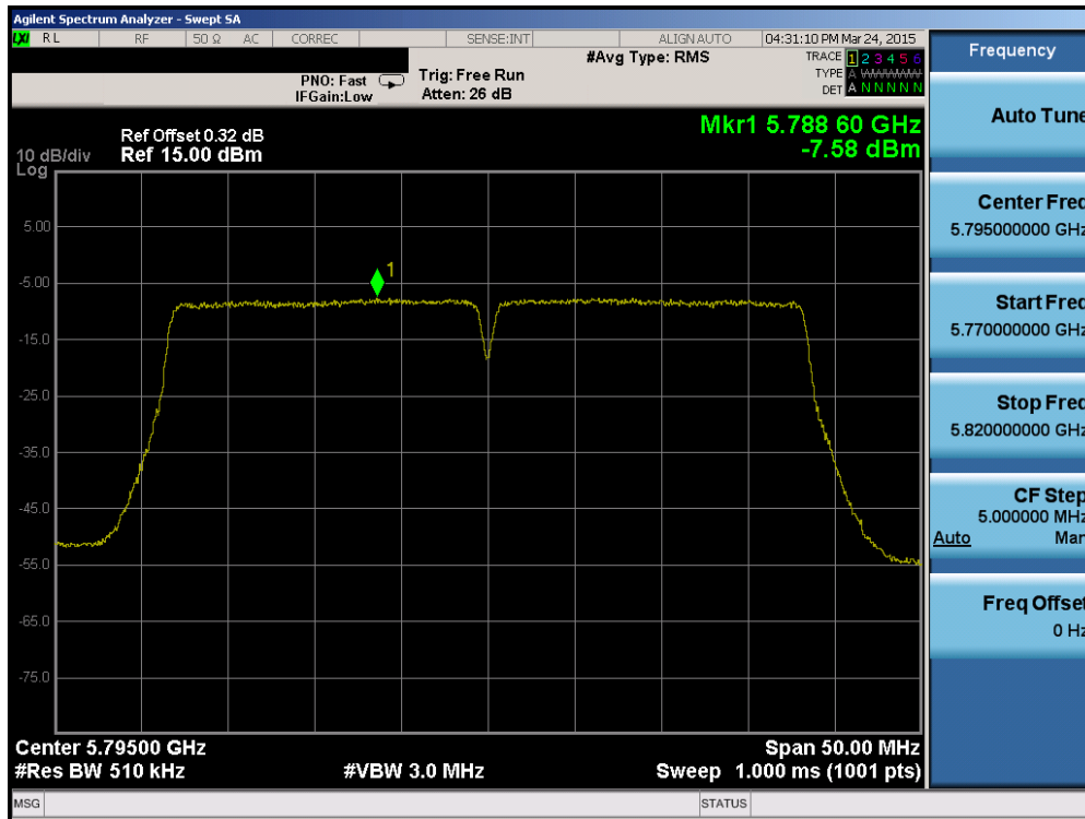
Plot 6-75. Power Spectral Density Plot (40MHz BW 802.11n (UNII Band 3) – Ch. 159)
