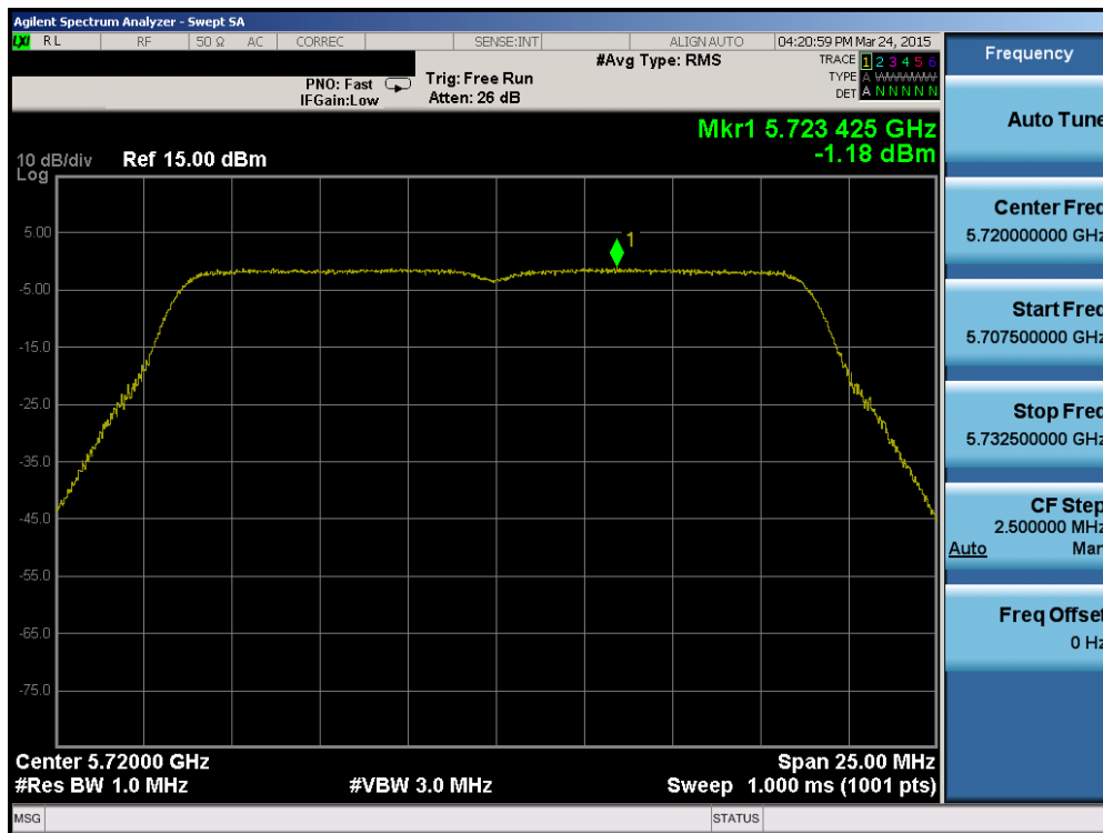
Plot 6-62. Power Spectral Density Plot (20MHz BW 802.11n (UNII Band 2C) – Ch. 144)
