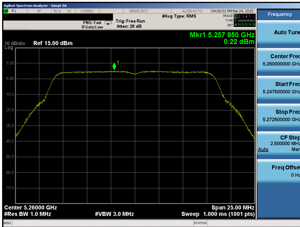
Plot 6-48. Power Spectral Density Plot (802.11a (UNII Band 2A) – Ch. 52)
