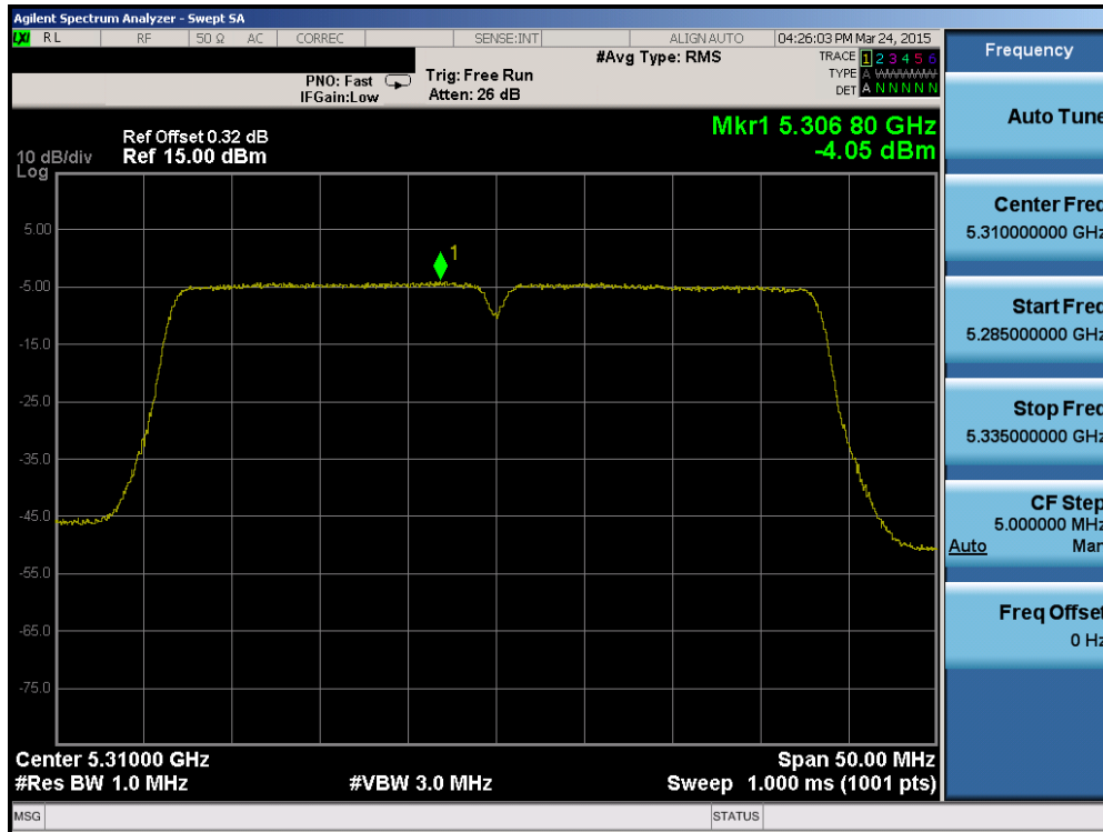
Plot 6-55. Power Spectral Density Plot (40MHz BW 802.11n (UNII Band 2A) – Ch. 62)
