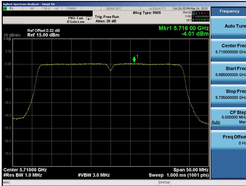
Plot 6-65. Power Spectral Density Plot (40MHz BW 802.11n (UNII Band 2C) – Ch. 142)
