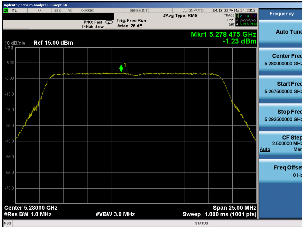
Plot 6-52. Power Spectral Density Plot (20MHz BW 802.11n (UNII Band 2A) – Ch. 56)
