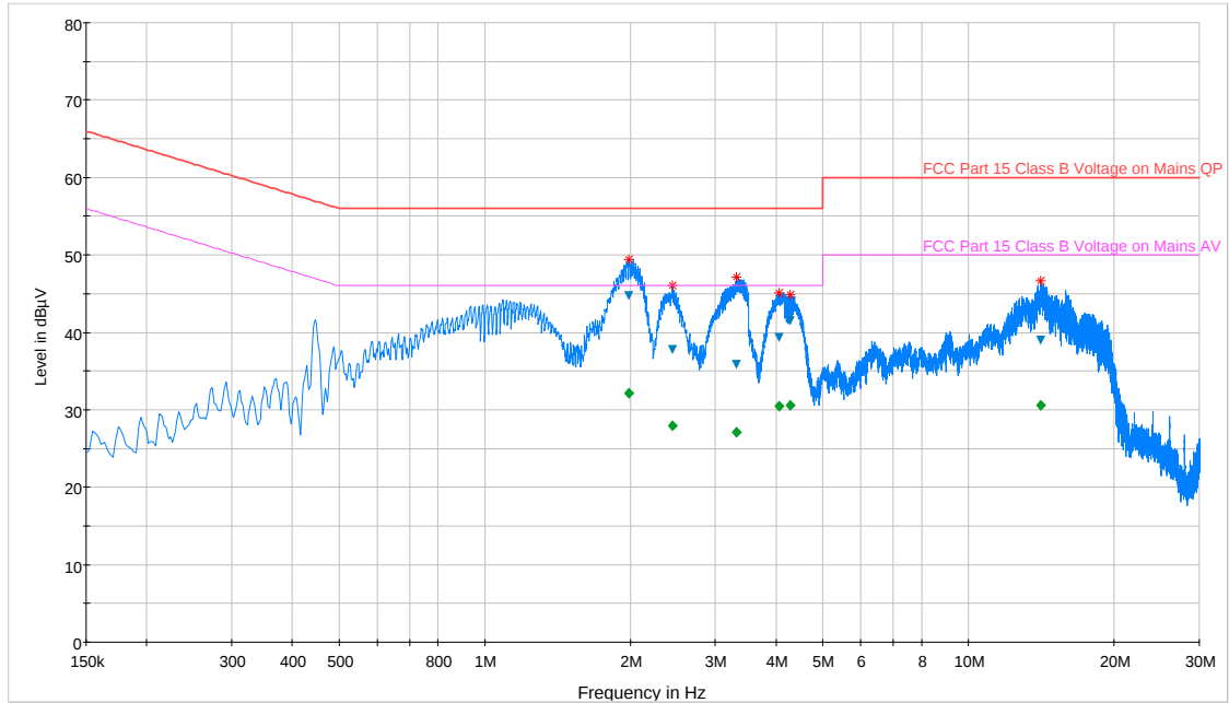
Plot 6-111. Line Conducted Plot with 802.11a UNII Band 1 (N)
