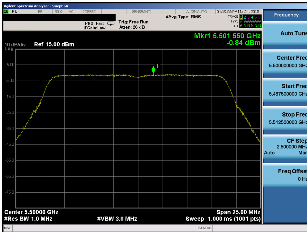
Plot 6-60. Power Spectral Density Plot (20MHz BW 802.11n (UNII Band 2C) – Ch. 100)
