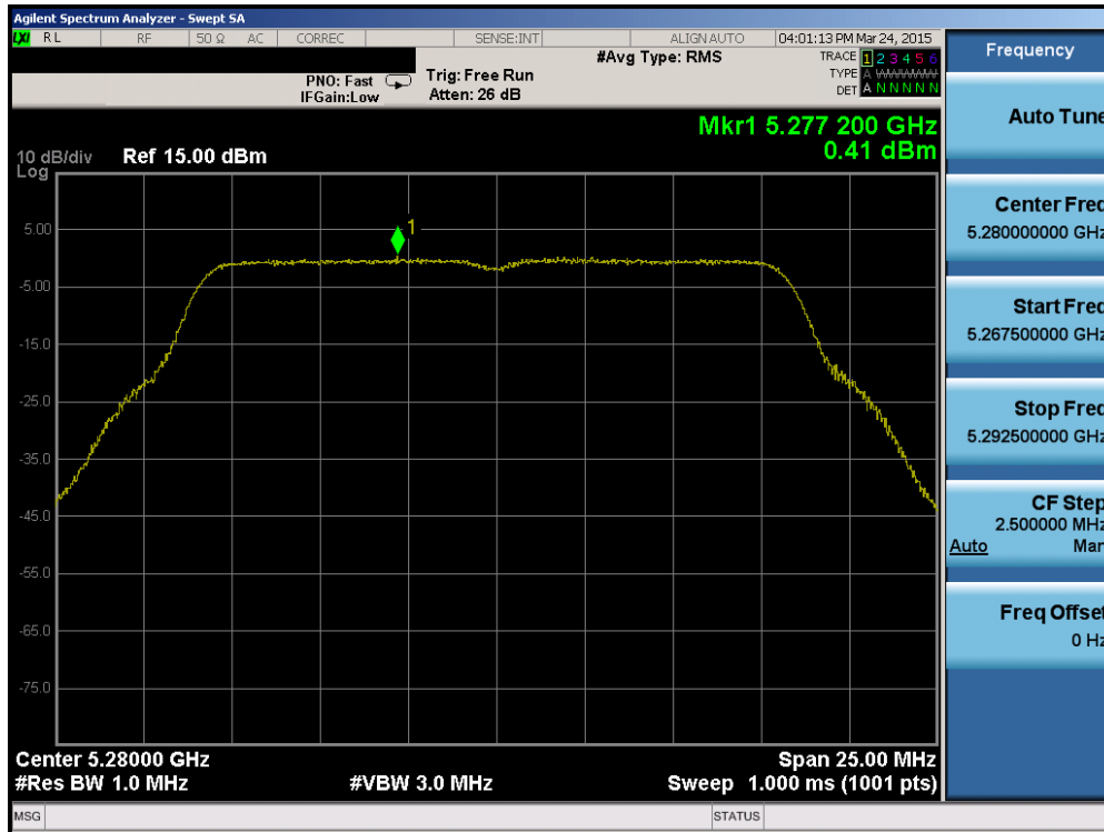
Plot 6-49. Power Spectral Density Plot (802.11a (UNII Band 2A) – Ch. 56)
