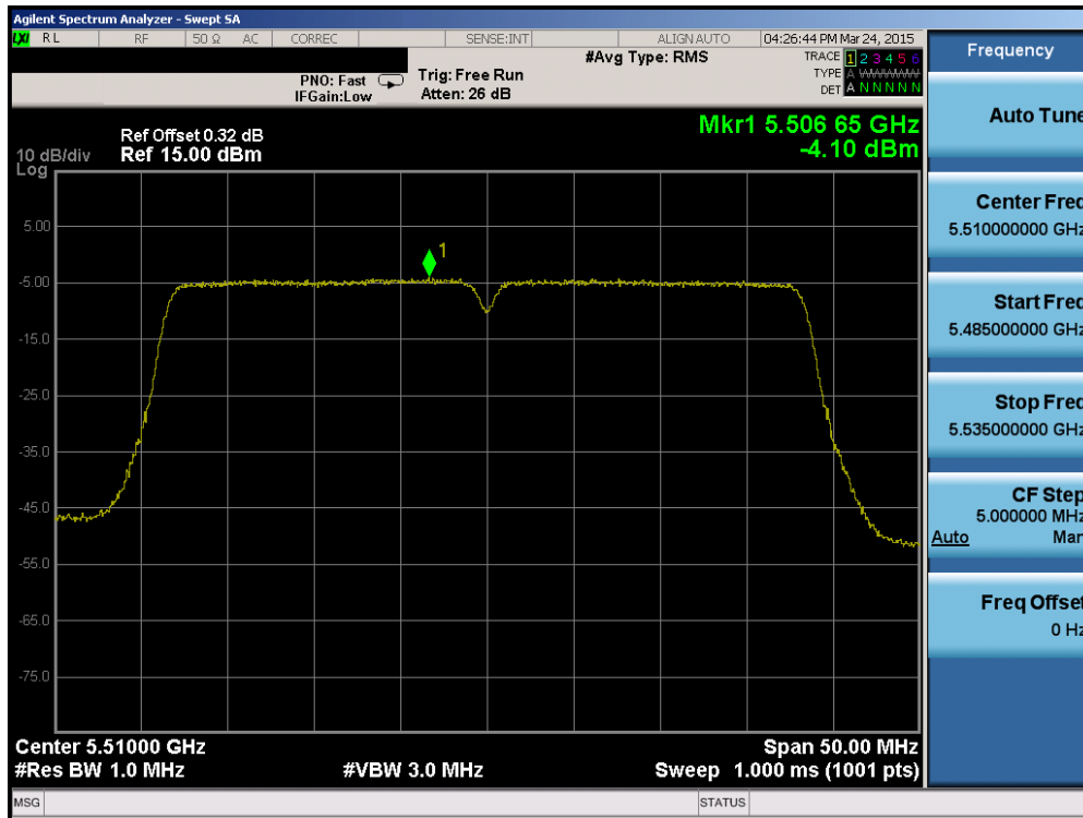
Plot 6-63. Power Spectral Density Plot (40MHz BW 802.11n (UNII Band 2C) – Ch. 102)
