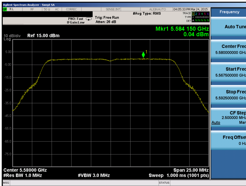
Plot 6-58. Power Spectral Density Plot (802.11a (UNII Band 2C) – Ch. 116)
