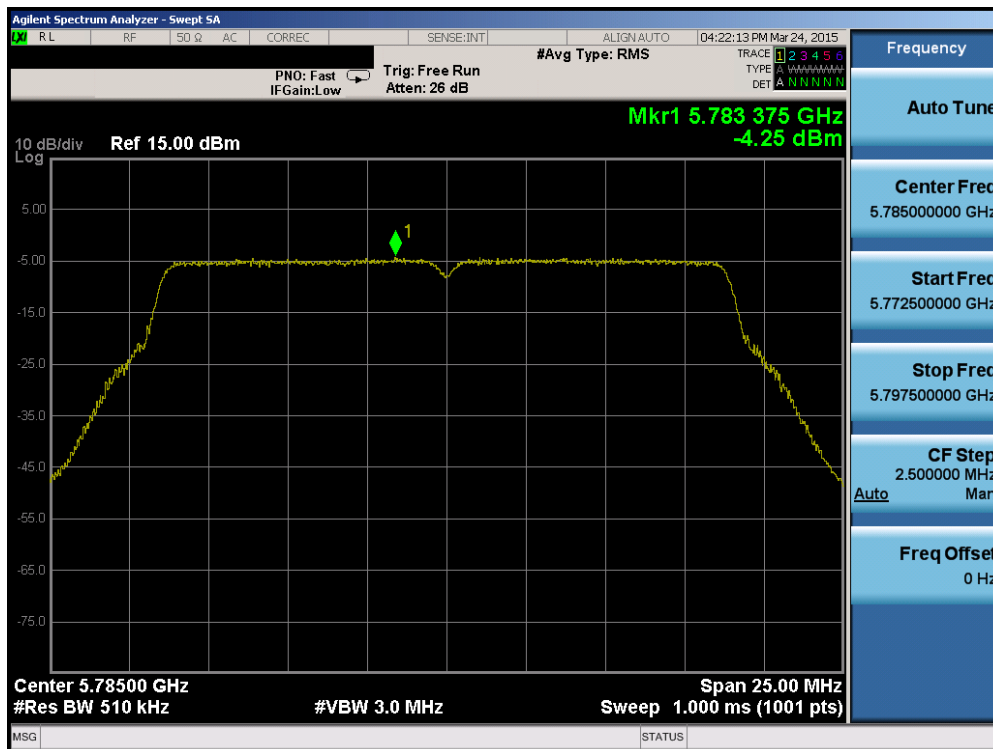
Plot 6-72. Power Spectral Density Plot (20MHz BW 802.11n (UNII Band 3) – Ch. 157)
