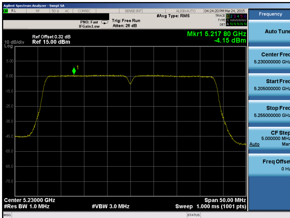
Plot 6-46. Power Spectral Density Plot (40MHz BW 802.11n (UNII Band 1) – Ch. 46)
