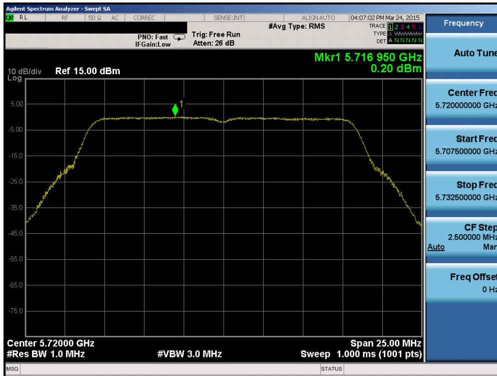
Plot 6-59. Power Spectral Density Plot (802.11a (UNII Band 2C) – Ch. 144)
