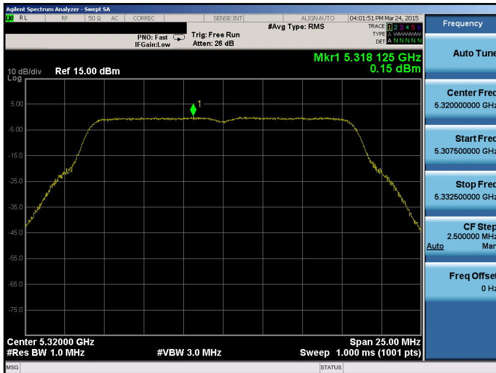
Plot 6-50. Power Spectral Density Plot (802.11a (UNII Band 2A) – Ch. 64)
