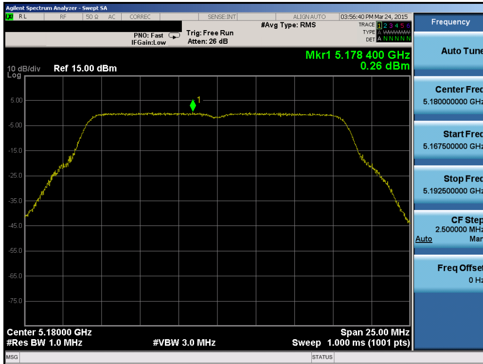
Plot 6-39. Power Spectral Density Plot (802.11a (UNII Band 1) – Ch. 36)
