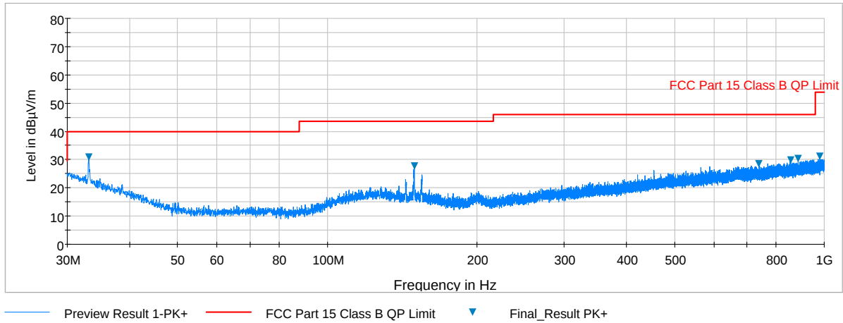
Plot 6-109. Radiated Spurious Plot below 1GHz (802.11a – U3 Ch. 157, Ant. Pol. V)
