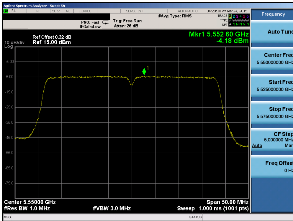
Plot 6-64. Power Spectral Density Plot (40MHz BW 802.11n (UNII Band 2C) – Ch. 110)
