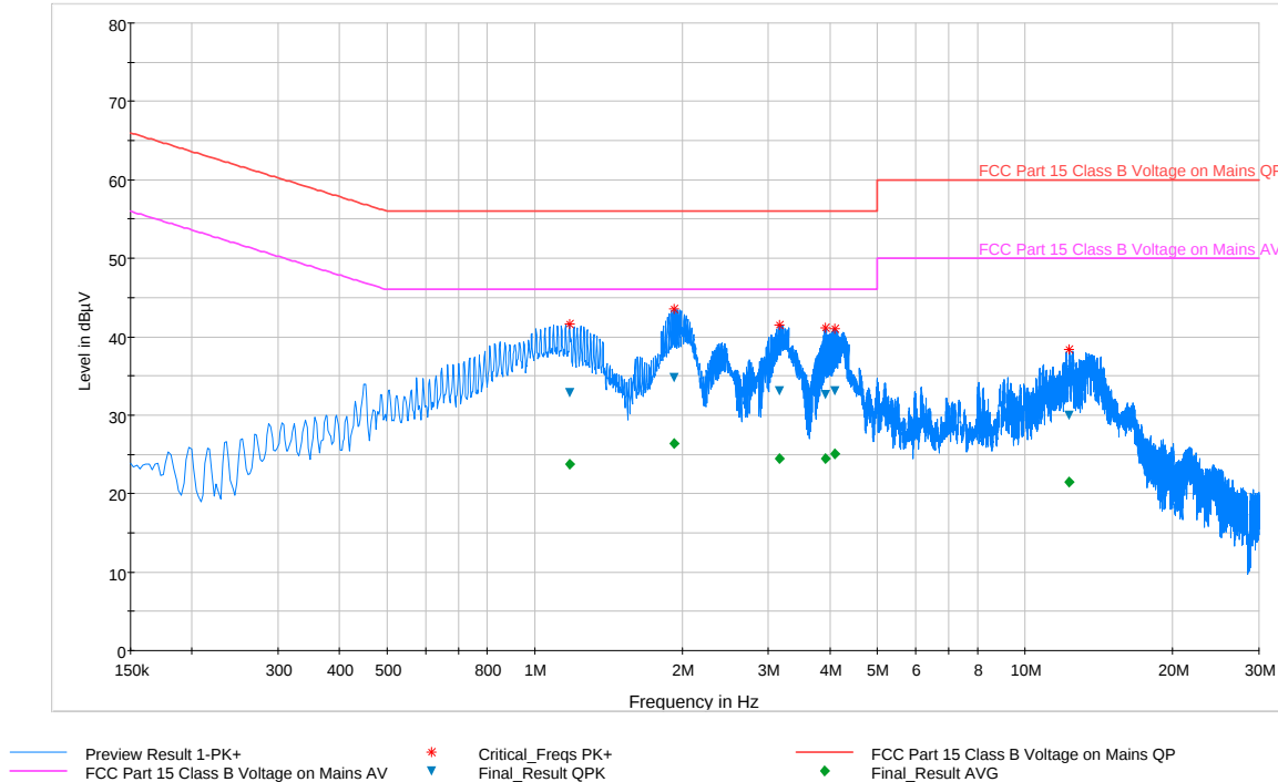
Plot 6-114. Line Conducted Plot with 802.11a UNII Band 2C (L1)
