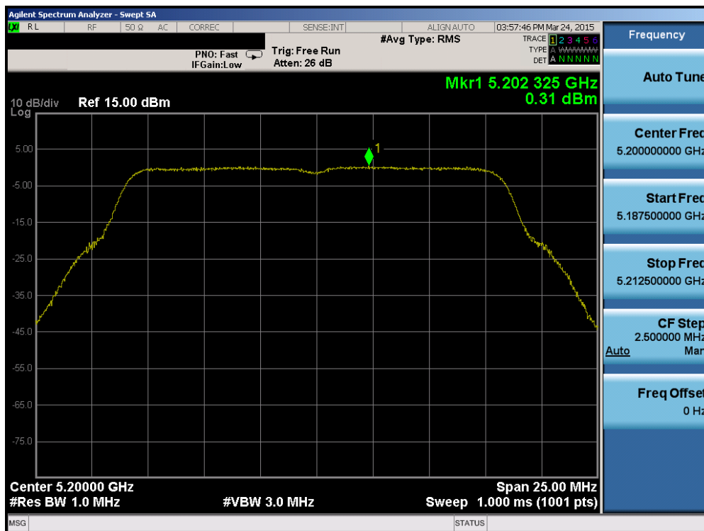
Plot 6-40. Power Spectral Density Plot (802.11a (UNII Band 1) – Ch. 40)
