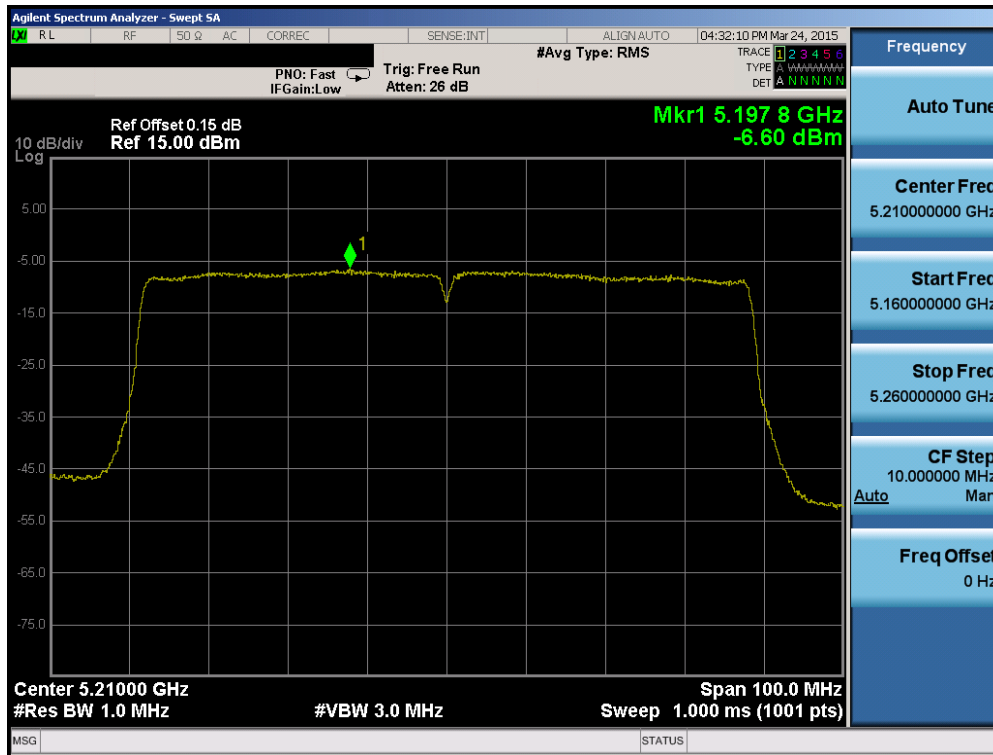
Plot 6-47. Power Spectral Density Plot (80MHz BW 802.11ac (UNII Band 1) – Ch. 42)
