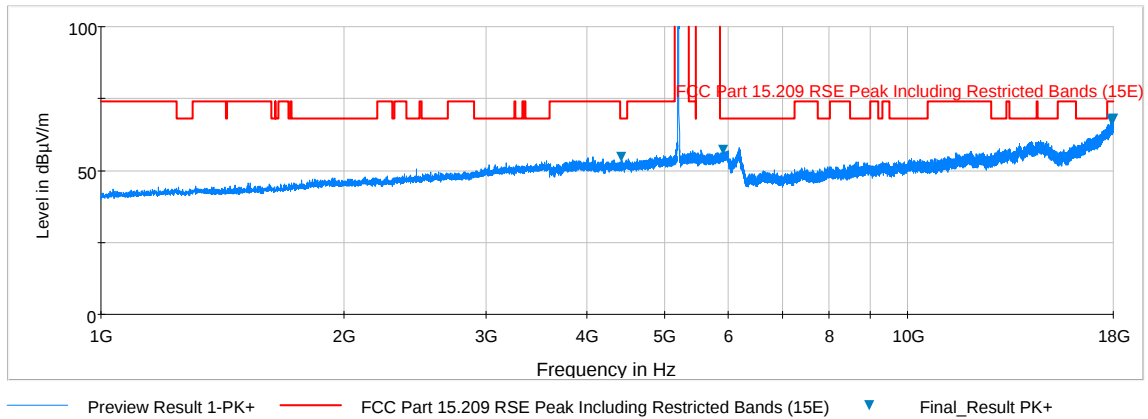
Plot 6-77. Radiated Spurious Plot above 1GHz (802.11a – U1 Ch. 40, Ant. Pol. H)
