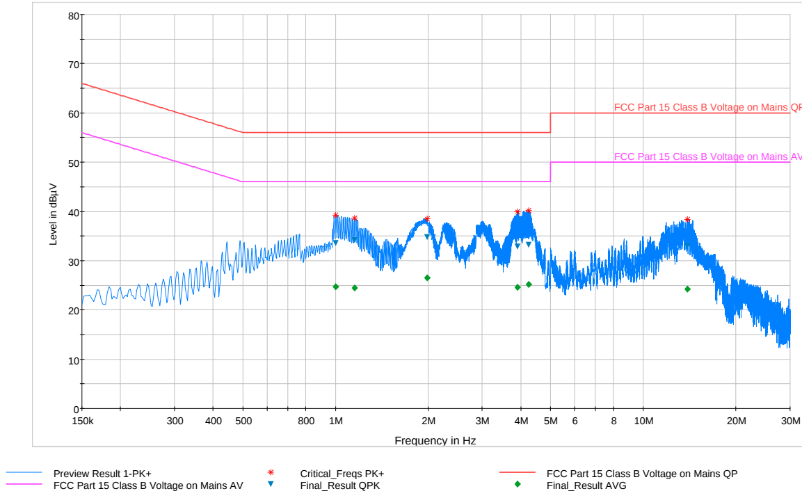
Plot 6-112. Line Conducted Plot with 802.11a UNII Band 2A (L1)
