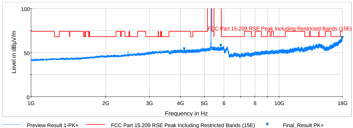
Plot 6-79. Radiated Spurious Plot above 1GHz (802.11a – U2A Ch. 56, Ant. Pol. H)
