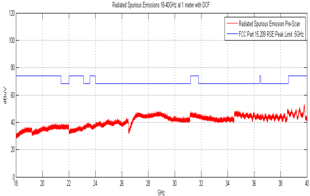
Plot 6-85. Radiated Spurious Plot above 18GHz (802.11a – Ant. Pol. H)
