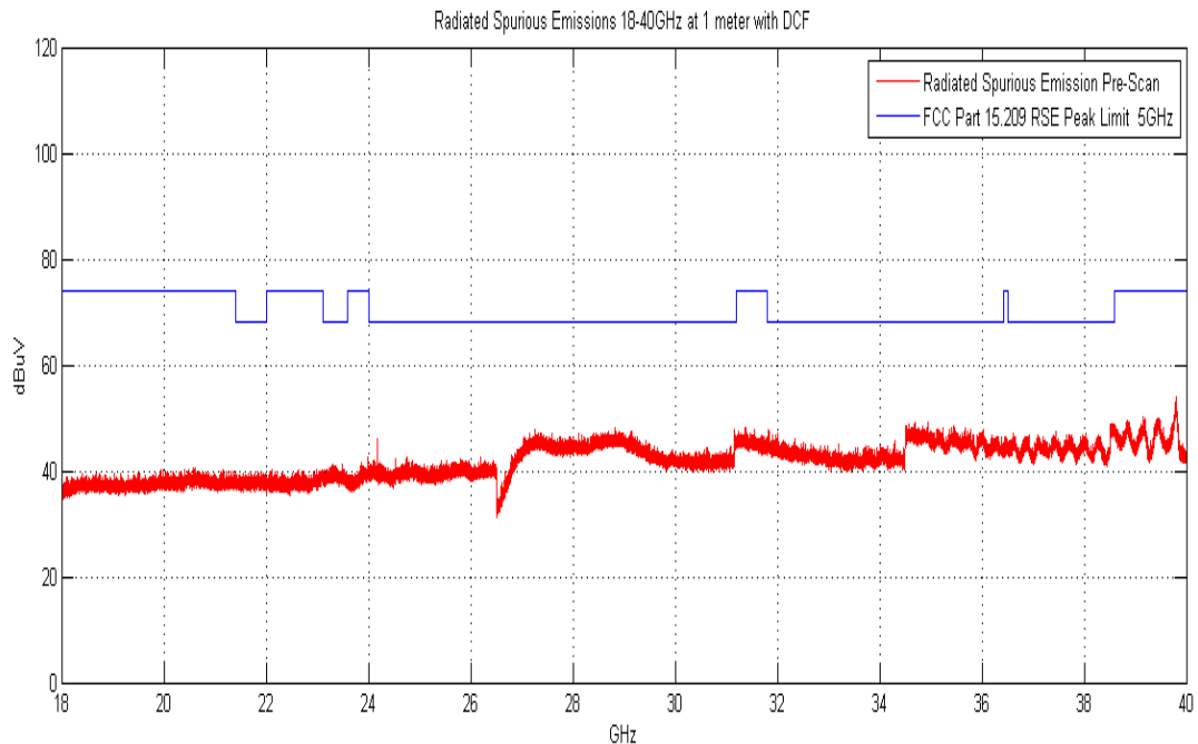
Plot 6-86. Radiated Spurious Plot above 18GHz (802.11a – Ant. Pol. V)
