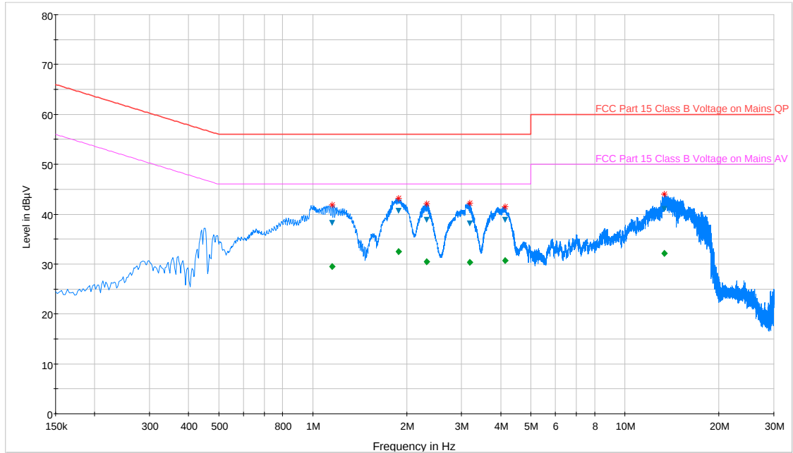
Plot 6-115. Line Conducted Plot with 802.11a UNII Band 2C (N)
