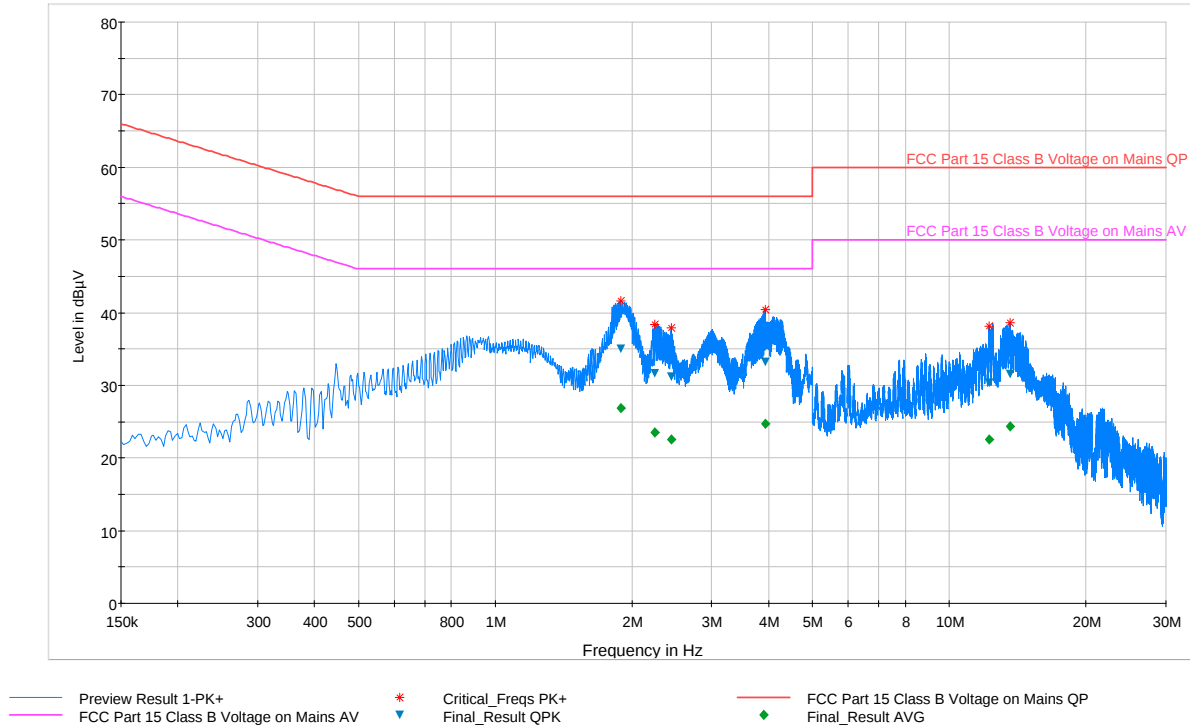
Plot 6-110. Line Conducted Plot with 802.11a UNII Band 1 (L1)
