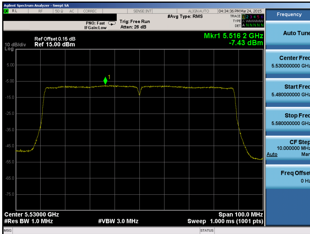
Plot 6-66. Power Spectral Density Plot (80MHz BW 802.11ac (UNII Band 2C) – Ch. 106)
