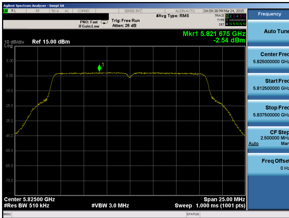
Plot 6-70. Power Spectral Density Plot (802.11a (UNII Band 3) – Ch. 165)
