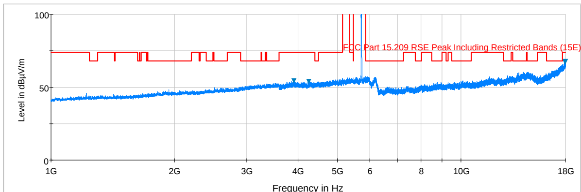
Plot 6-81. Radiated Spurious Plot above 1GHz (802.11a – U2C Ch. 116, Ant. Pol. H)
