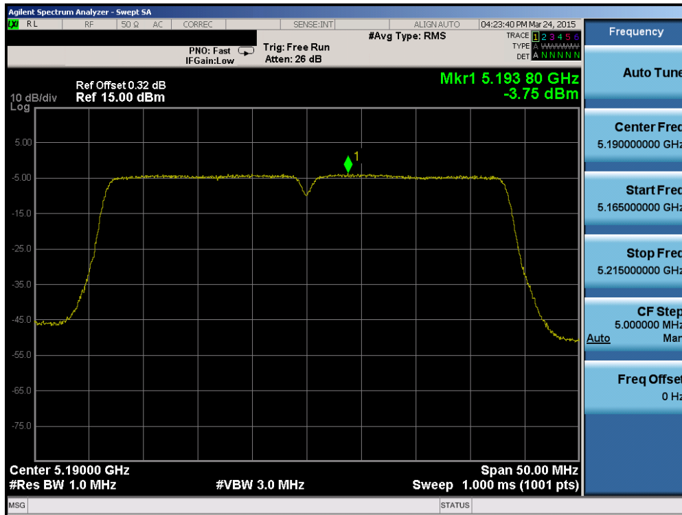
Plot 6-45. Power Spectral Density Plot (40MHz BW 802.11n (UNII Band 1) – Ch. 38)
