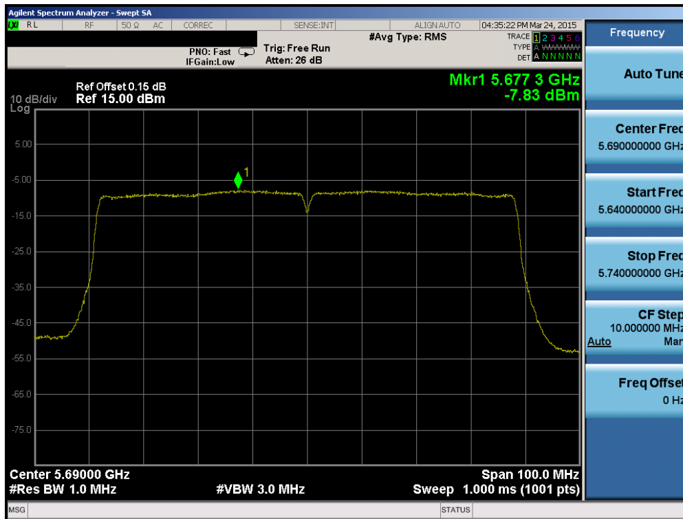
Plot 6-67. Power Spectral Density Plot (80MHz BW 802.11ac (UNII Band 2C) – Ch. 138)
