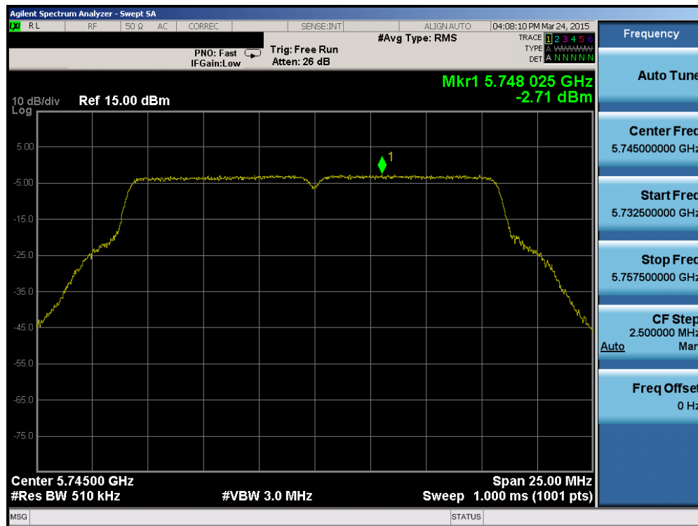
Plot 6-68. Power Spectral Density Plot (802.11a (UNII Band 3) – Ch. 149)
