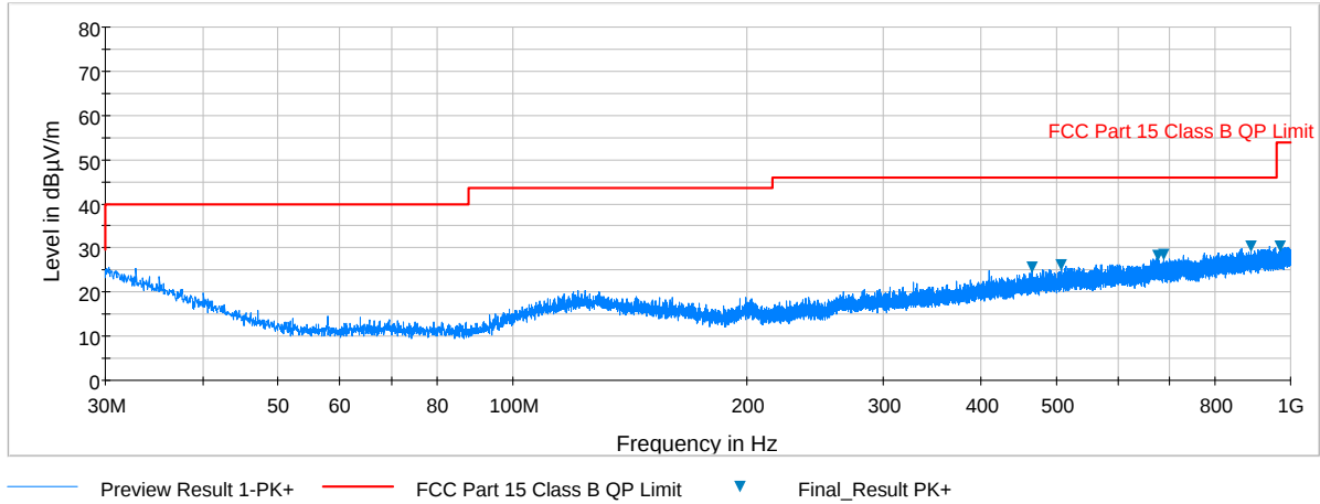
Plot 6-108. Radiated Spurious Plot below 1GHz (802.11a – U3 Ch. 157, Ant. Pol. H)
