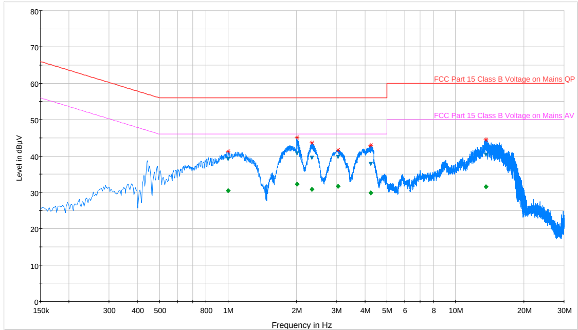
Plot 6-113. Line Conducted Plot with 802.11a UNII Band 2A (N)
