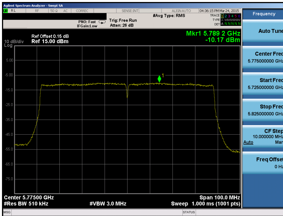
Plot 6-76. Power Spectral Density Plot (80MHz BW 802.11ac (UNII Band 3) – Ch. 155)
