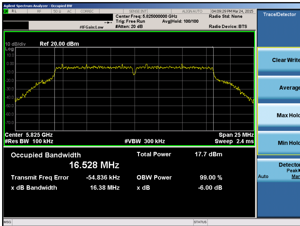
Plot 6-32. 6dB Bandwidth Plot (802.11a (UNII Band 3) – Ch. 165)
