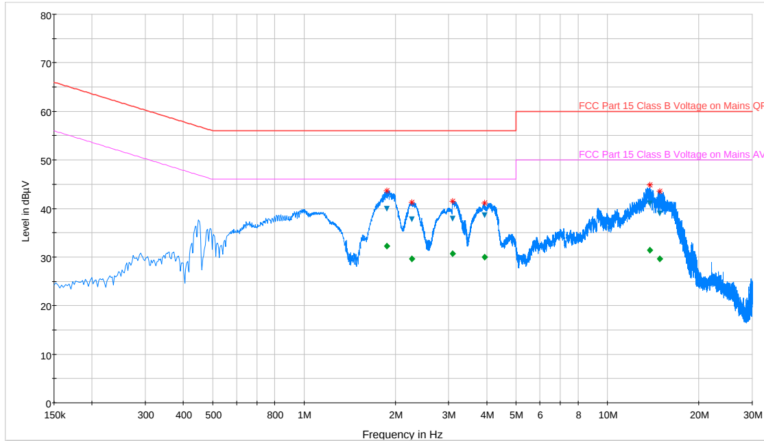
Plot 6-117. Line Conducted Plot with 802.11a UNII Band 3 (N)
