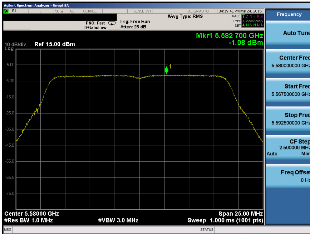
Plot 6-61. Power Spectral Density Plot (20MHz BW 802.11n (UNII Band 2C) – Ch. 116)
