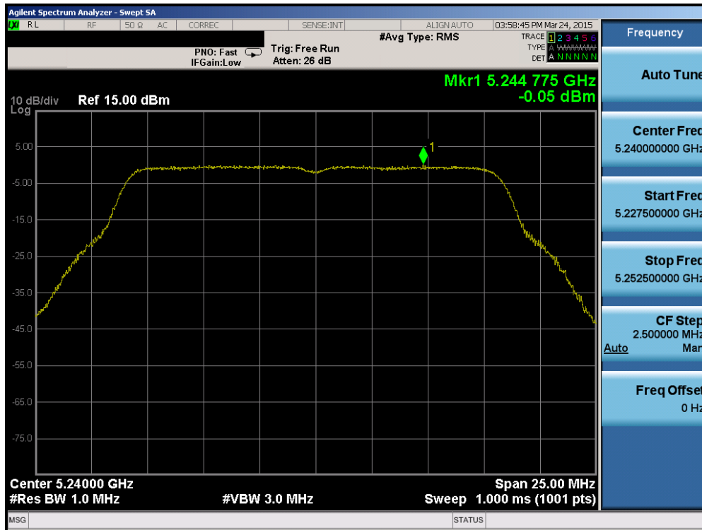
Plot 6-41. Power Spectral Density Plot (802.11a (UNII Band 1) – Ch. 48)
