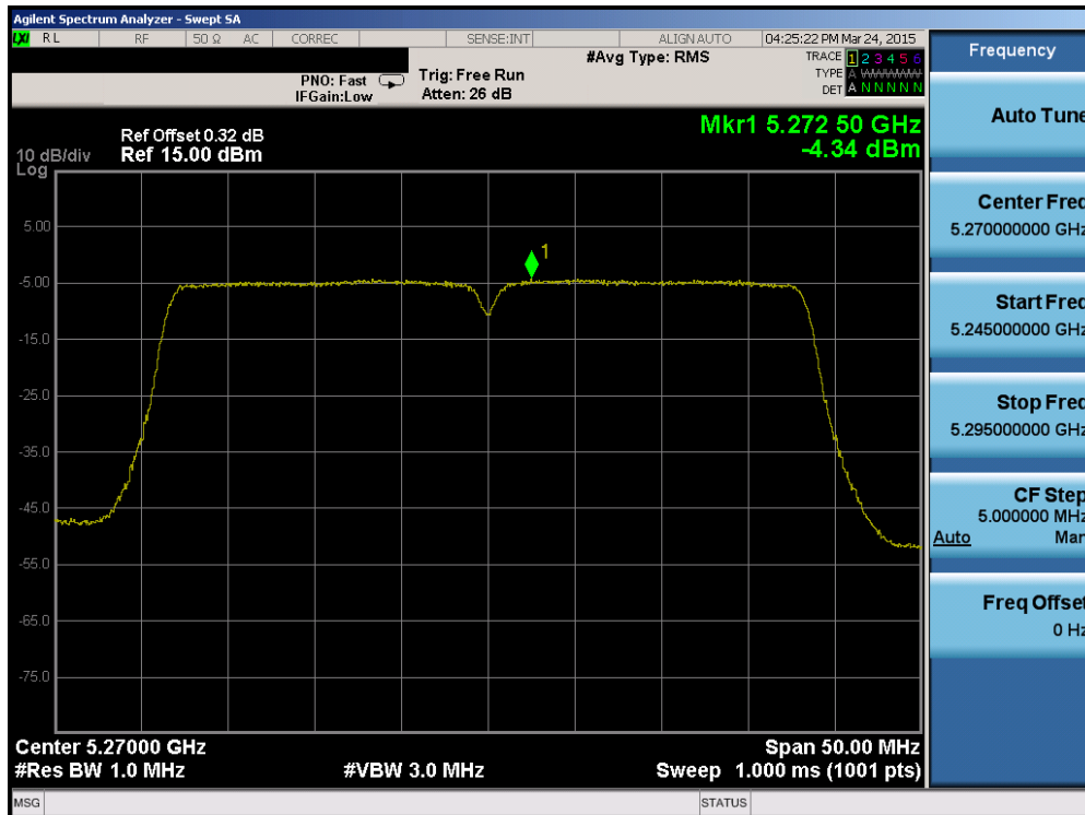
Plot 6-54. Power Spectral Density Plot (40MHz BW 802.11n (UNII Band 2A) – Ch. 54)
