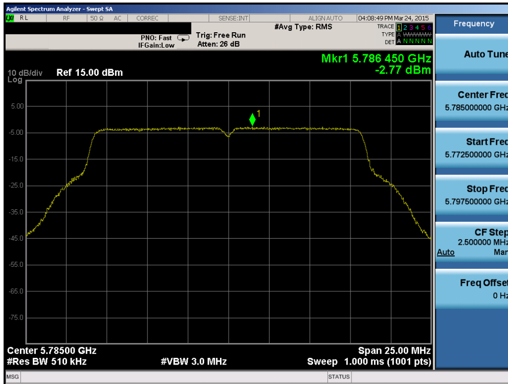
Plot 6-69. Power Spectral Density Plot (802.11a (UNII Band 3) – Ch. 157)
