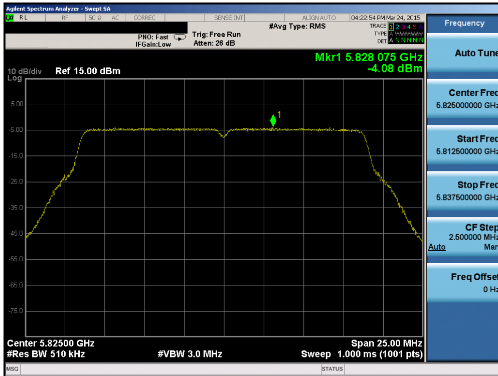
Plot 6-73. Power Spectral Density Plot (20MHz BW 802.11n (UNII Band 3) – Ch. 165)
