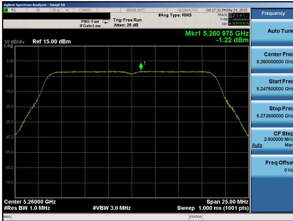
Plot 6-51. Power Spectral Density Plot (20MHz BW 802.11n (UNII Band 2A) – Ch. 52)
