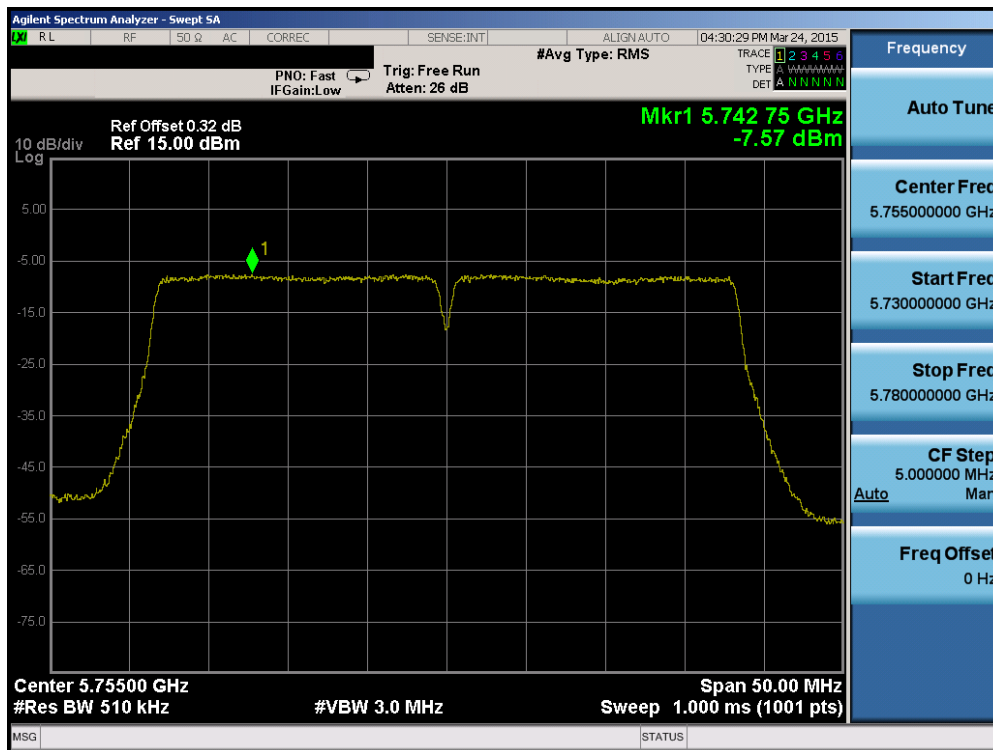
Plot 6-74. Power Spectral Density Plot (40MHz BW 802.11n (UNII Band 3) – Ch. 151)
