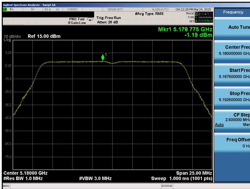
Plot 6-42. Power Spectral Density Plot (20MHz BW 802.11n (UNII Band 1) – Ch. 36)
