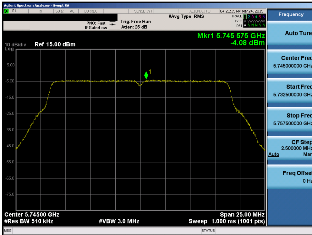
Plot 6-71. Power Spectral Density Plot (20MHz BW 802.11n (UNII Band 3) – Ch. 149)
