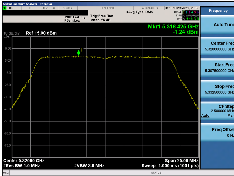
Plot 6-53. Power Spectral Density Plot (20MHz BW 802.11n (UNII Band 2A) – Ch. 64)
