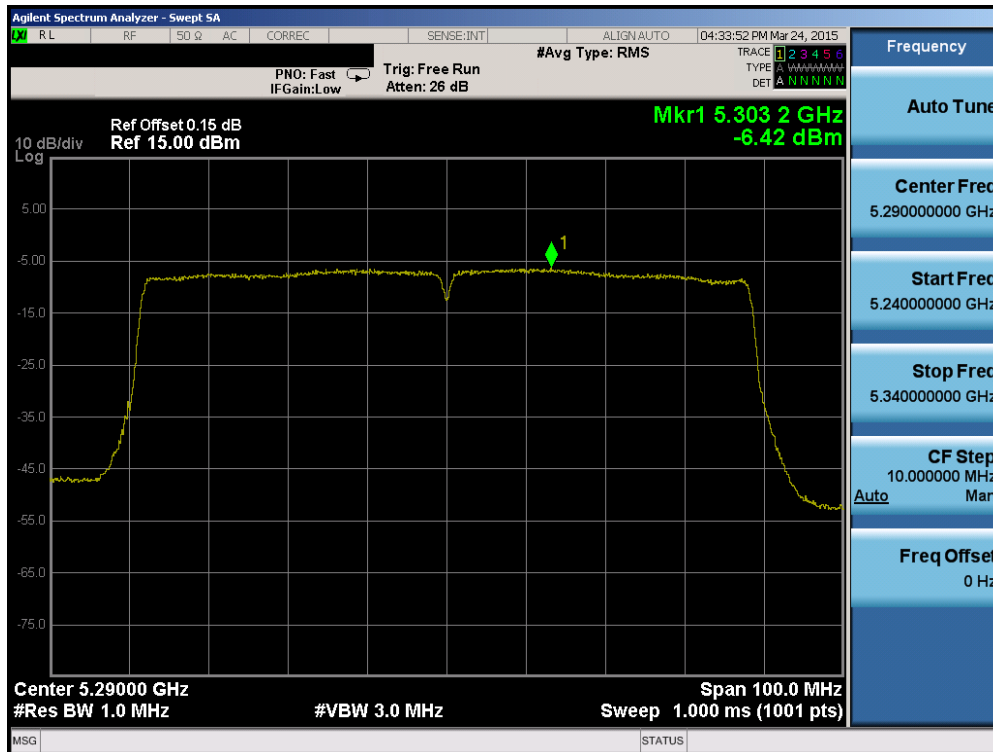
Plot 6-56. Power Spectral Density Plot (80MHz BW 802.11ac (UNII Band 2A) – Ch. 58)
