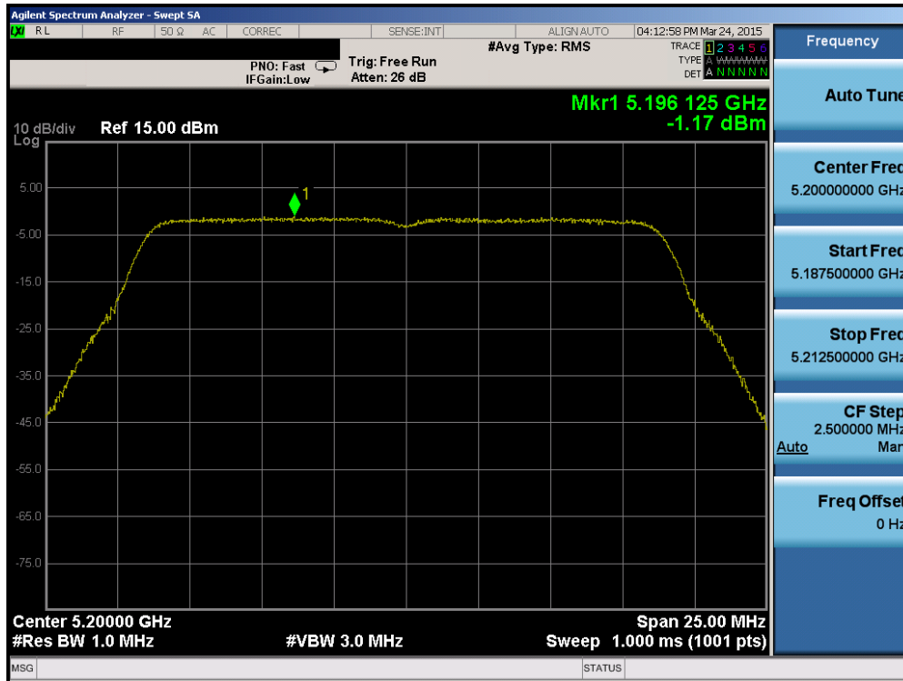
Plot 6-43. Power Spectral Density Plot (20MHz BW 802.11n (UNII Band 1) – Ch. 40)
