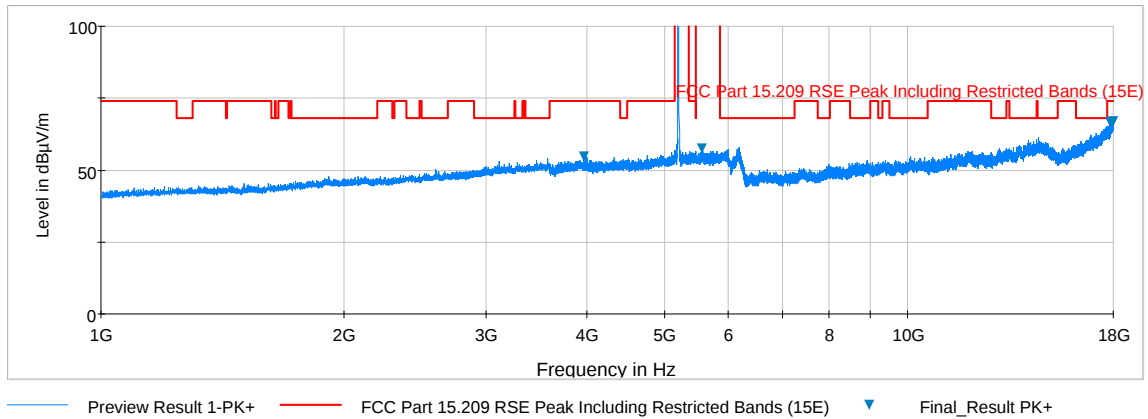
Plot 6-78. Radiated Spurious Plot above 1GHz (802.11a – U1 Ch. 40, Ant. Pol. V)
