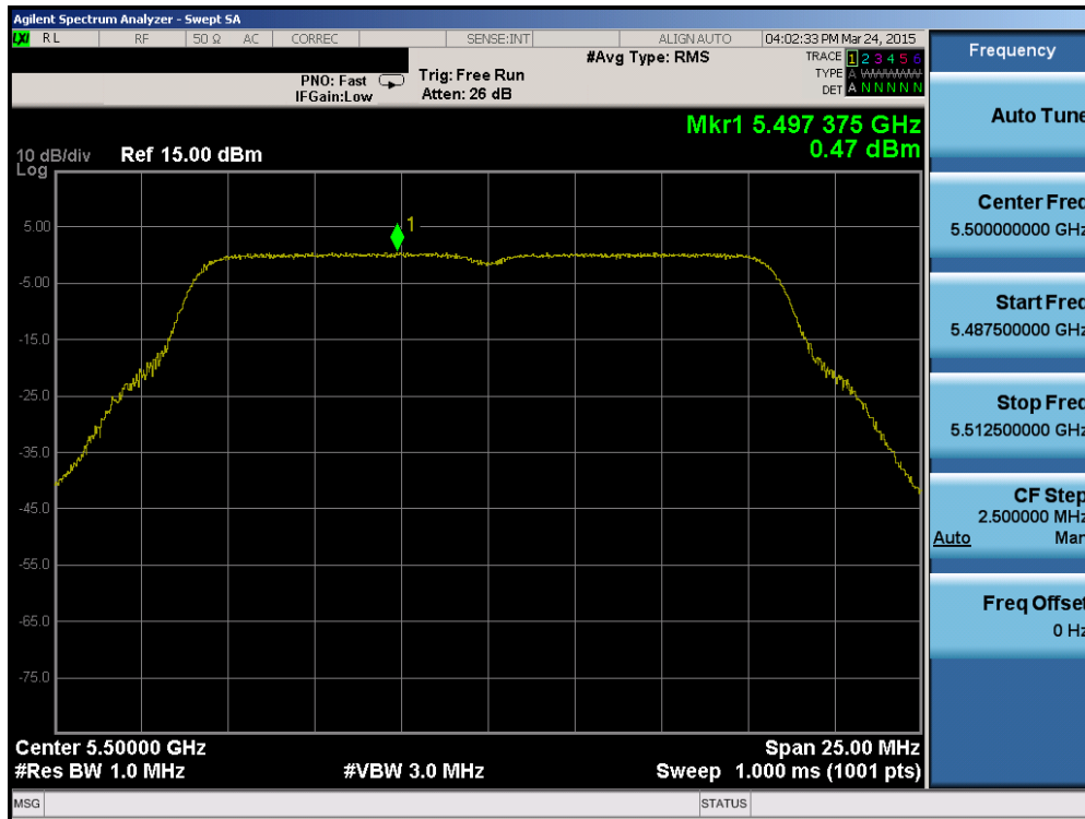
Plot 6-57. Power Spectral Density Plot (802.11a (UNII Band 2C) – Ch. 100)
