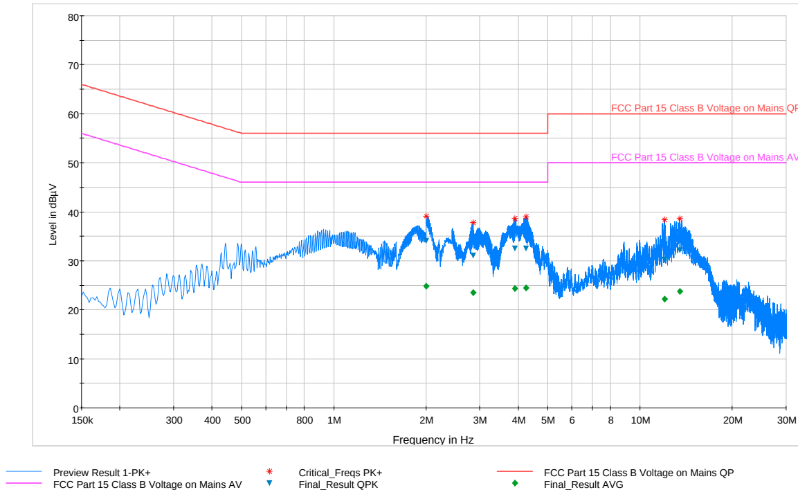
Plot 6-116. Line Conducted Plot with 802.11a UNII Band 3 (L1)
