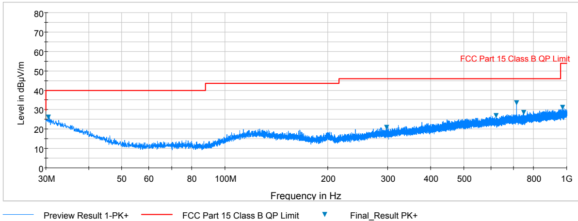
Plot 6-24. Radiated Spurious Plot below 1GHz (802.11a – U3 Ch. 157, Ant. Pol. V)
