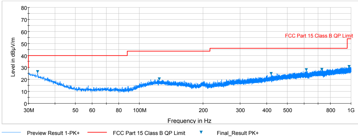
Plot 6-23. Radiated Spurious Plot below 1GHz (802.11a – U3 Ch. 157, Ant. Pol. H)
