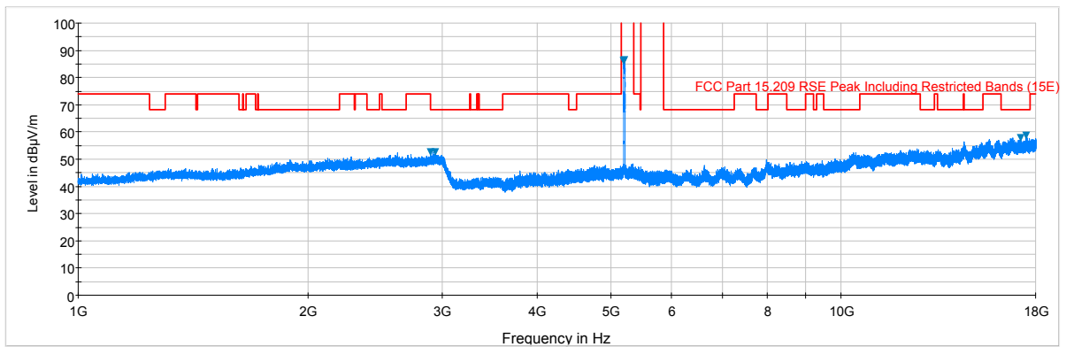
Plot 6-2. Radiated Spurious Plot above 1GHz (802.11a – U1 Ch. 40, Ant. Pol. V)
