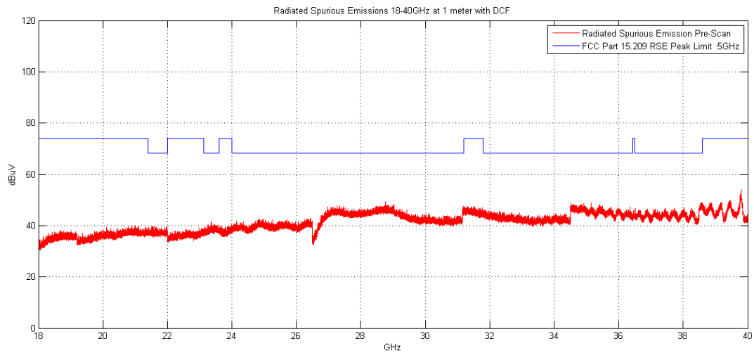
Plot 6-10. Radiated Spurious Plot above 18GHz (802.11a – Ant. Pol. V)
