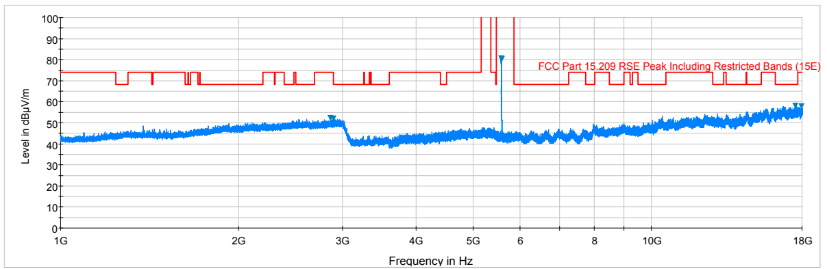
Plot 6-5. Radiated Spurious Plot above 1GHz (802.11a – U2C Ch. 116, Ant. Pol. H)
