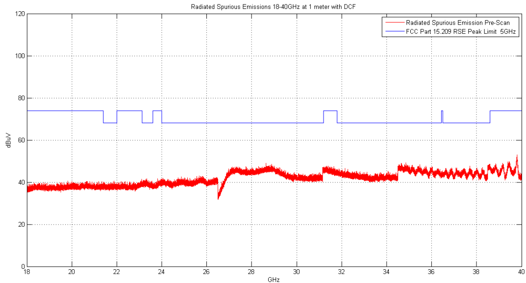
Plot 6-9. Radiated Spurious Plot above 18GHz (802.11a – Ant. Pol. H)
