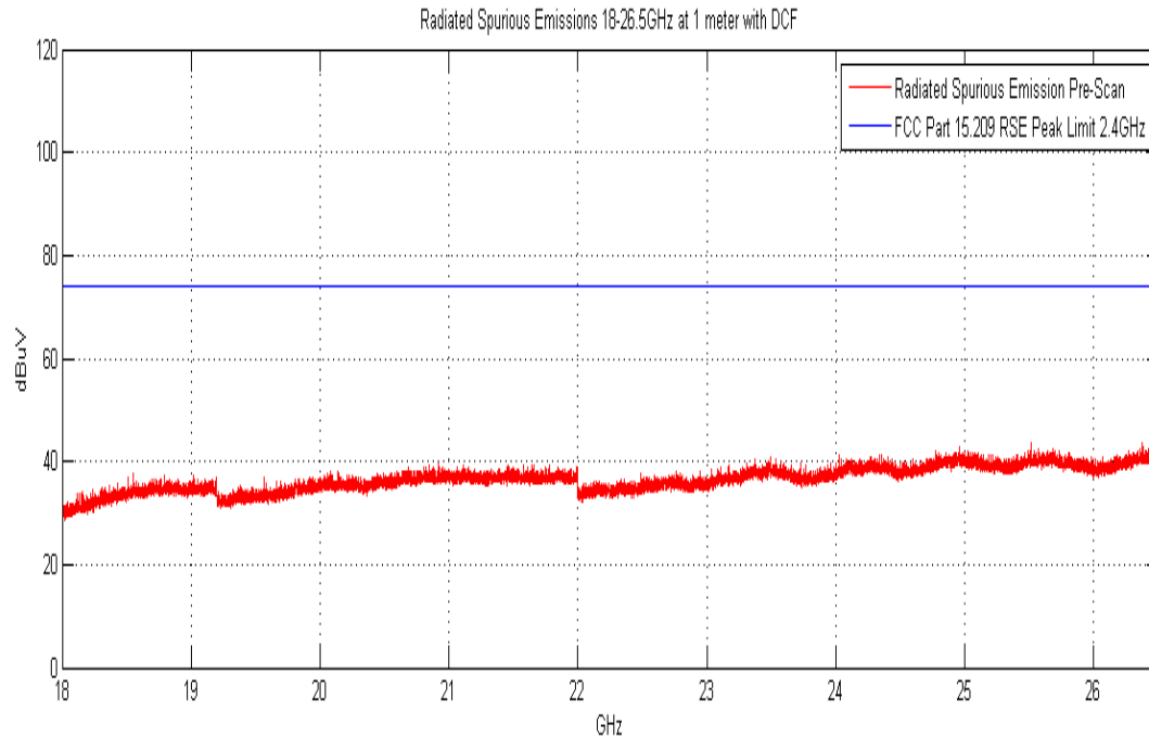
Plot 6-37. Radiated Spurious Plot above 18GHz (Pol. H)
