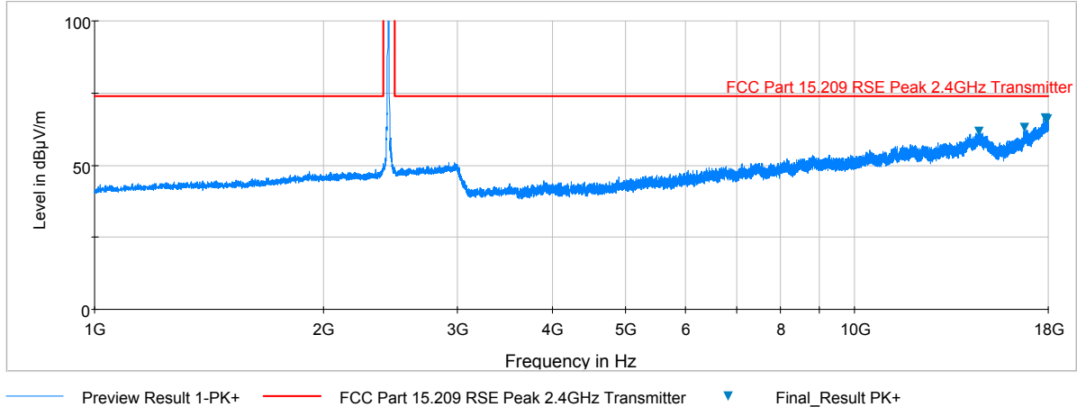
Plot 6-34. Radiated Spurious Plot above 1GHz (802.11b – Ch. 6, Ant. Pol. V)
