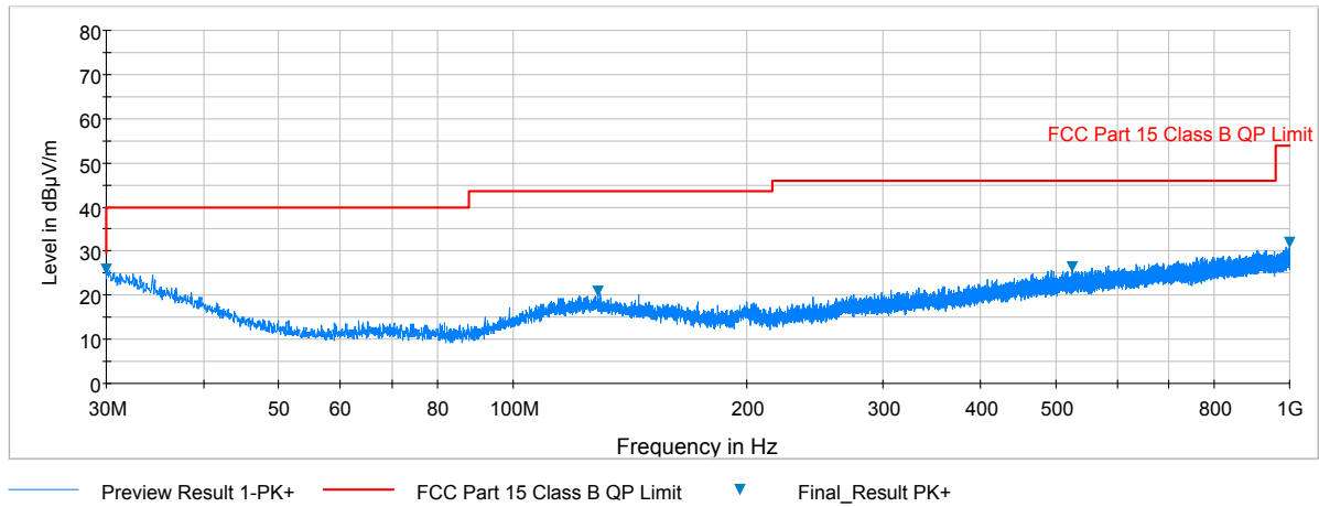
Plot 6-43. Radiated Spurious Plot below 1GHz (Pol. H)
