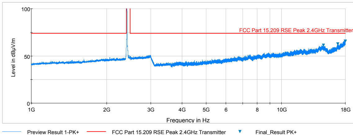
Plot 6-32. Radiated Spurious Plot above 1GHz (802.11b – Ch. 1, Ant. Pol. V)
