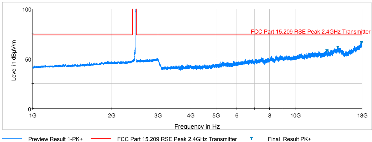
Plot 6-35. Radiated Spurious Plot above 1GHz (802.11b – Ch. 11, Ant. Pol. H)
