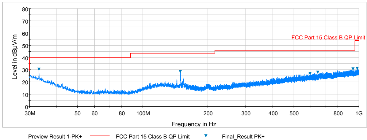
Plot 6-44. Radiated Spurious Plot below 1GHz (Pol. V)
