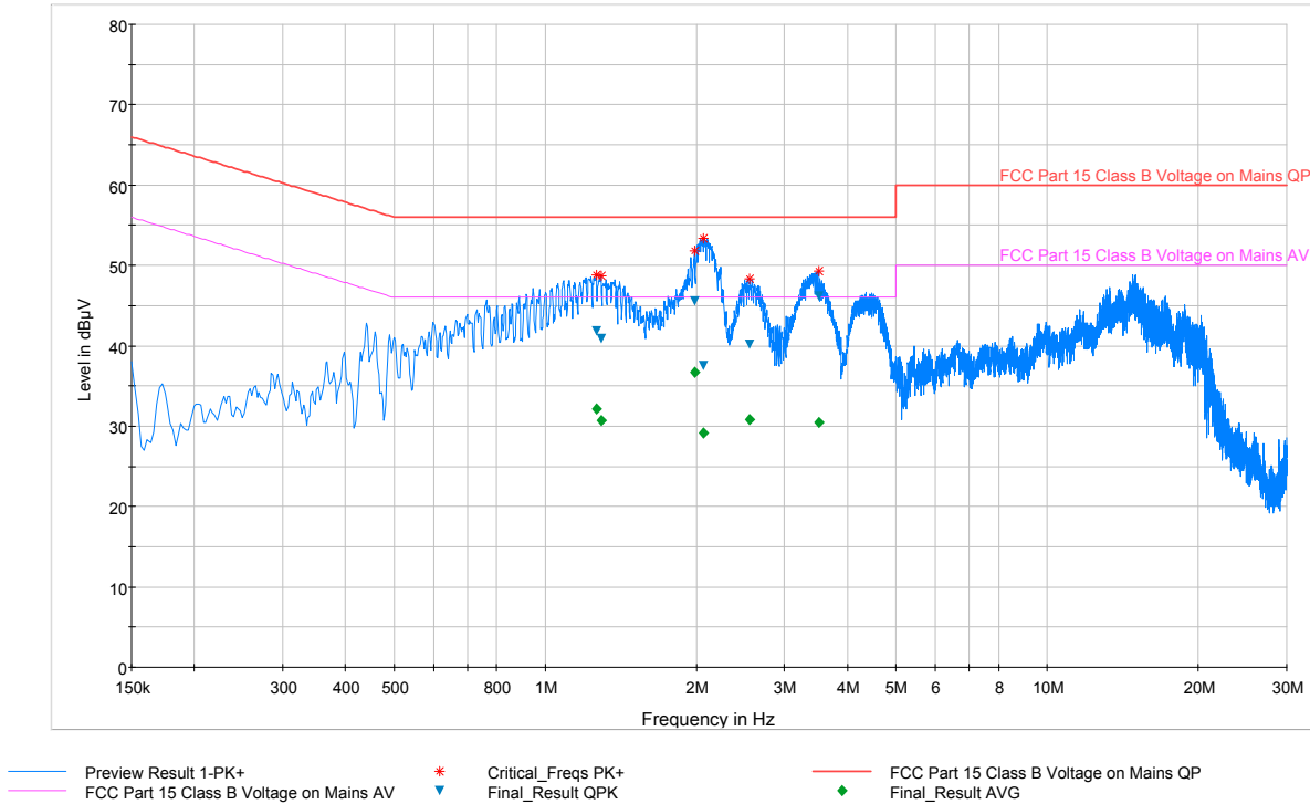
Plot 6-46. Line Conducted Plot with 802.11b (N)
