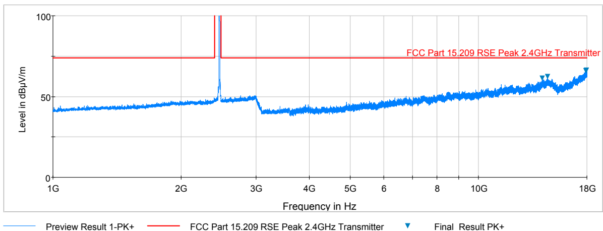
Plot 6-36. Radiated Spurious Plot above 1GHz (802.11b – Ch. 11, Ant. Pol. V)
