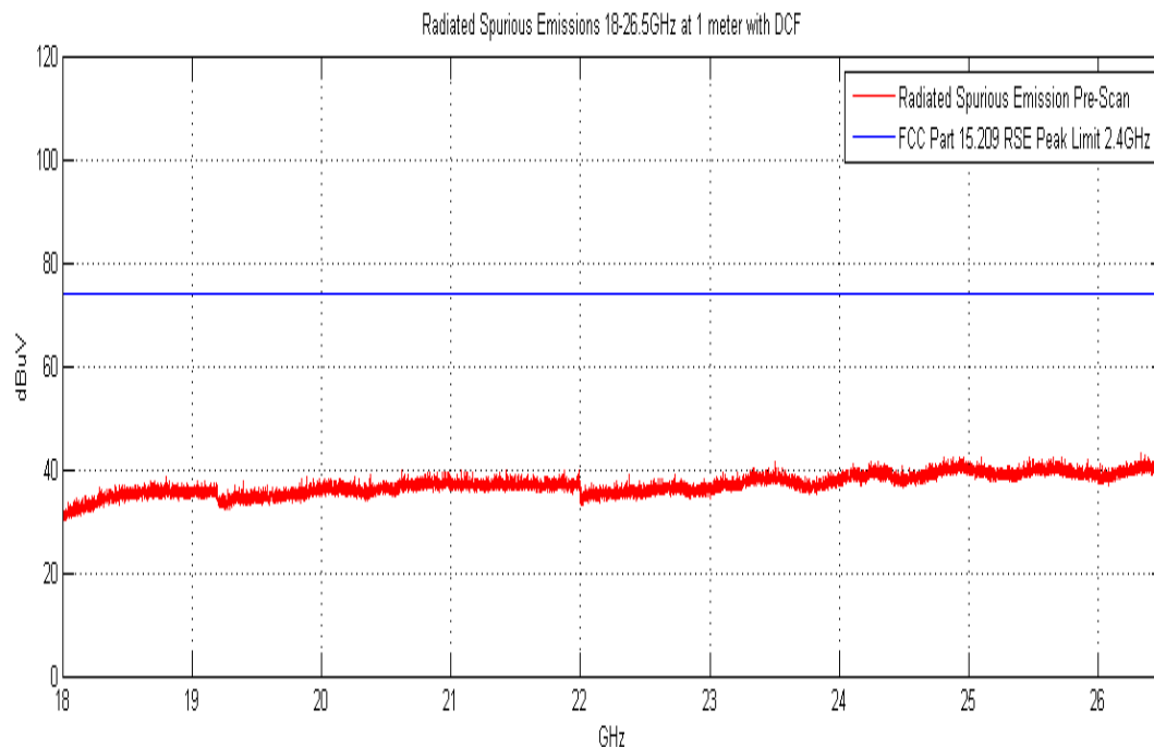
Plot 6-38. Radiated Spurious Plot above 18GHz (Pol. V)
