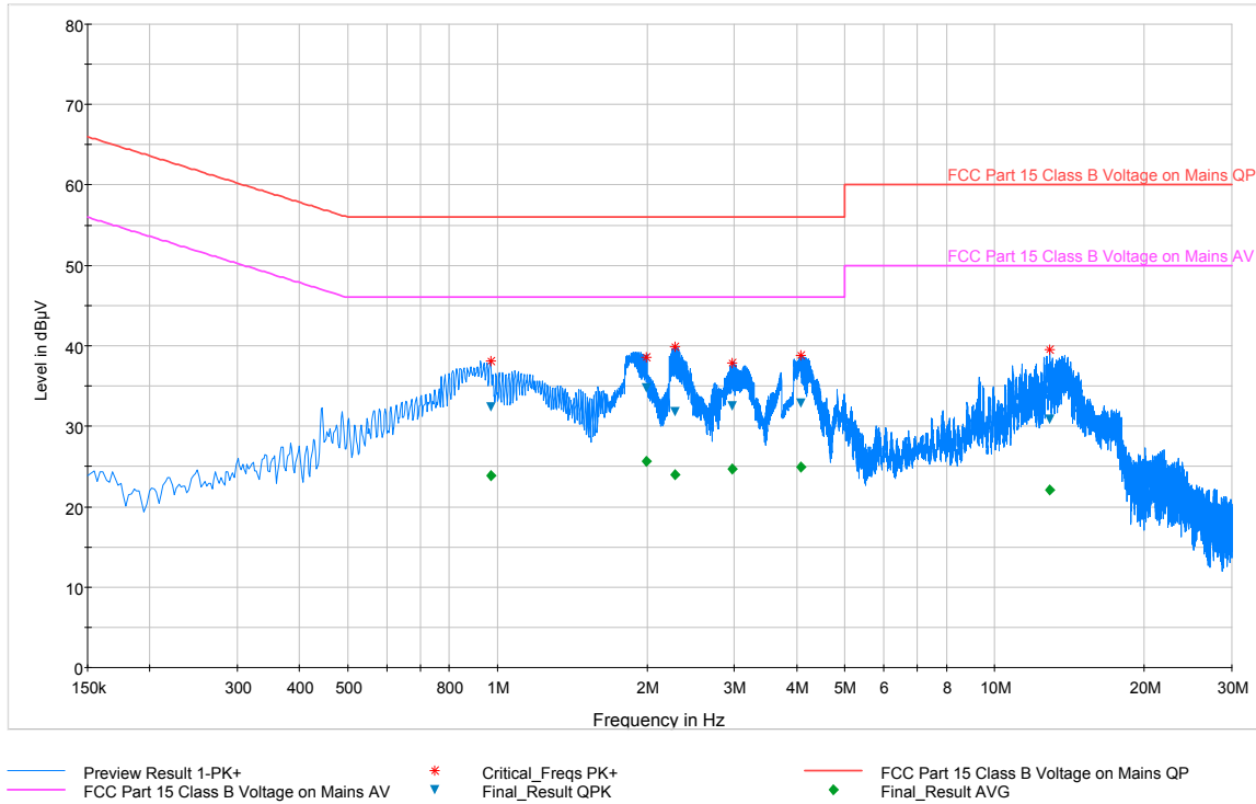
Plot 6-45. Line Conducted Plot with 802.11b (L1)
