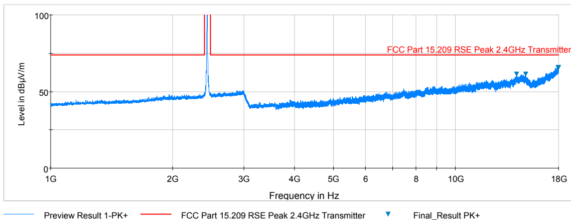
Plot 6-33. Radiated Spurious Plot above 1GHz (802.11b – Ch. 6, Ant. Pol. H)
