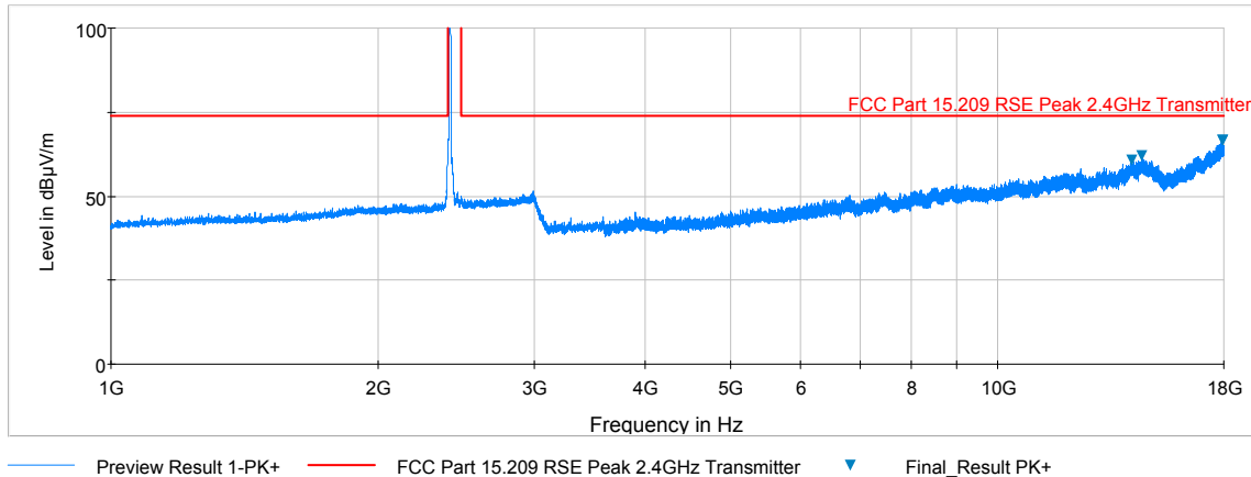
Plot 6-31. Radiated Spurious Plot above 1GHz (802.11b – Ch. 1, Ant. Pol. H)
