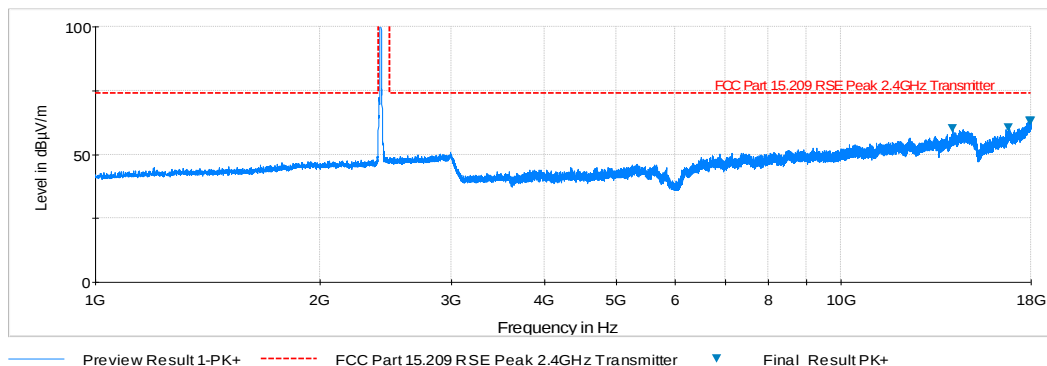
Plot 6-2. Radiated Spurious Plot above 1GHz (802.11b – Ch. 1, Ant. Pol. V)
