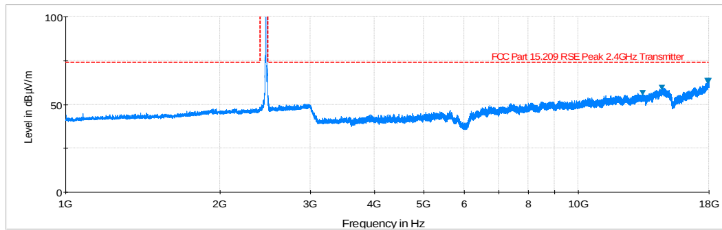
Plot 6-5. Radiated Spurious Plot above 1GHz (802.11b – Ch. 11, Ant. Pol. H)
