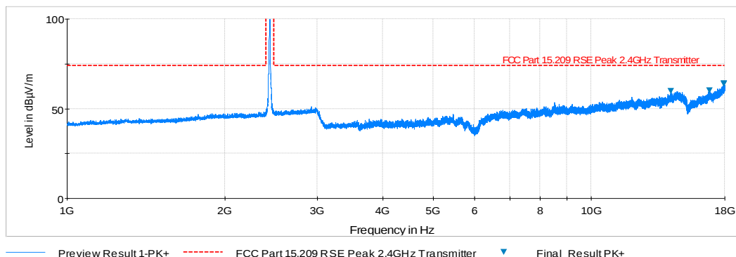
Plot 6-3. Radiated Spurious Plot above 1GHz (802.11b – Ch. 6, Ant. Pol. H)
