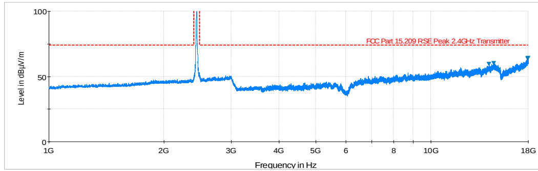
Plot 6-4. Radiated Spurious Plot above 1GHz (802.11b – Ch. 6, Ant. Pol. V)
