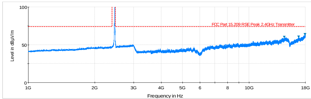
Plot 6-6. Radiated Spurious Plot above 1GHz (802.11b – Ch. 11, Ant. Pol. V)
