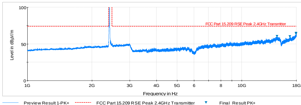
Plot 6-1. Radiated Spurious Plot above 1GHz (802.11b – Ch. 1, Ant. Pol. H)
