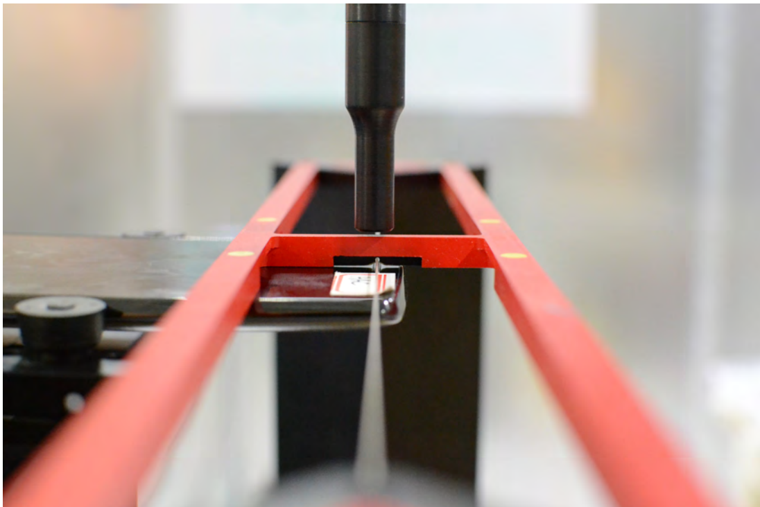
Figure 17-4 HAC Phantom Plane Alignment (Standard Battery Cover)
