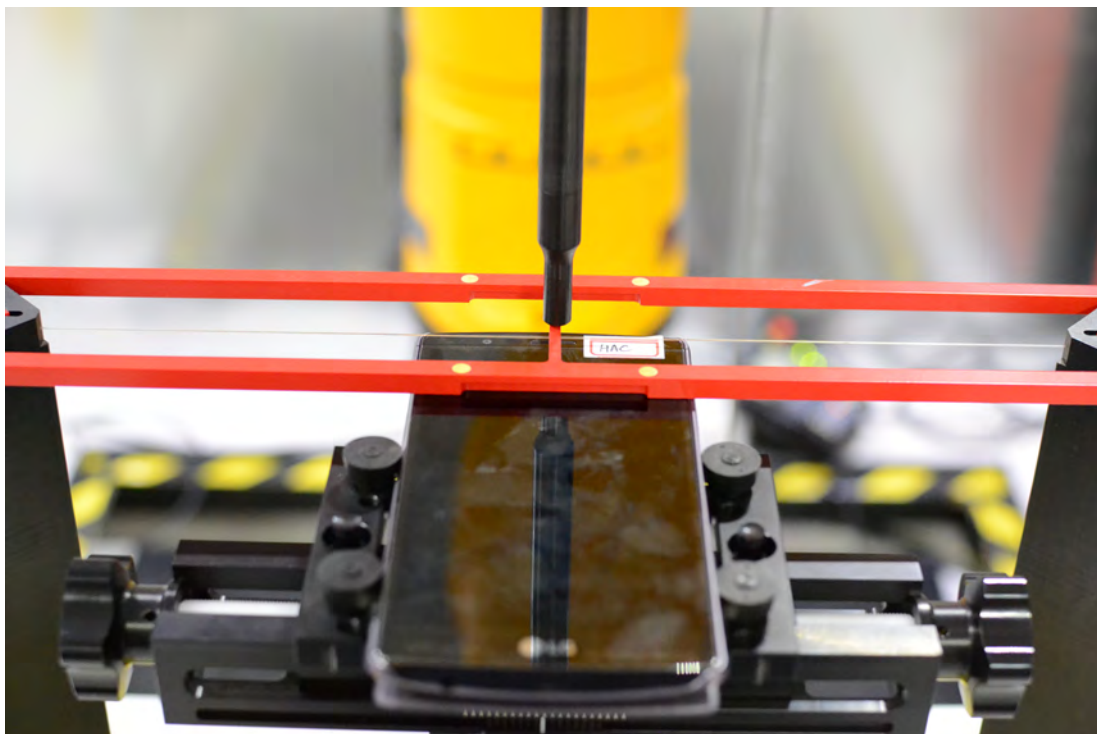
Figure 17-2 Ear Reference Point HAC Phantom Alignment (Wireless Charging Cover - Open)
