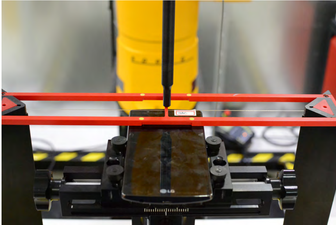
Figure 17-1 Ear Reference Point HAC Phantom Alignment (Standard Battery Cover)
