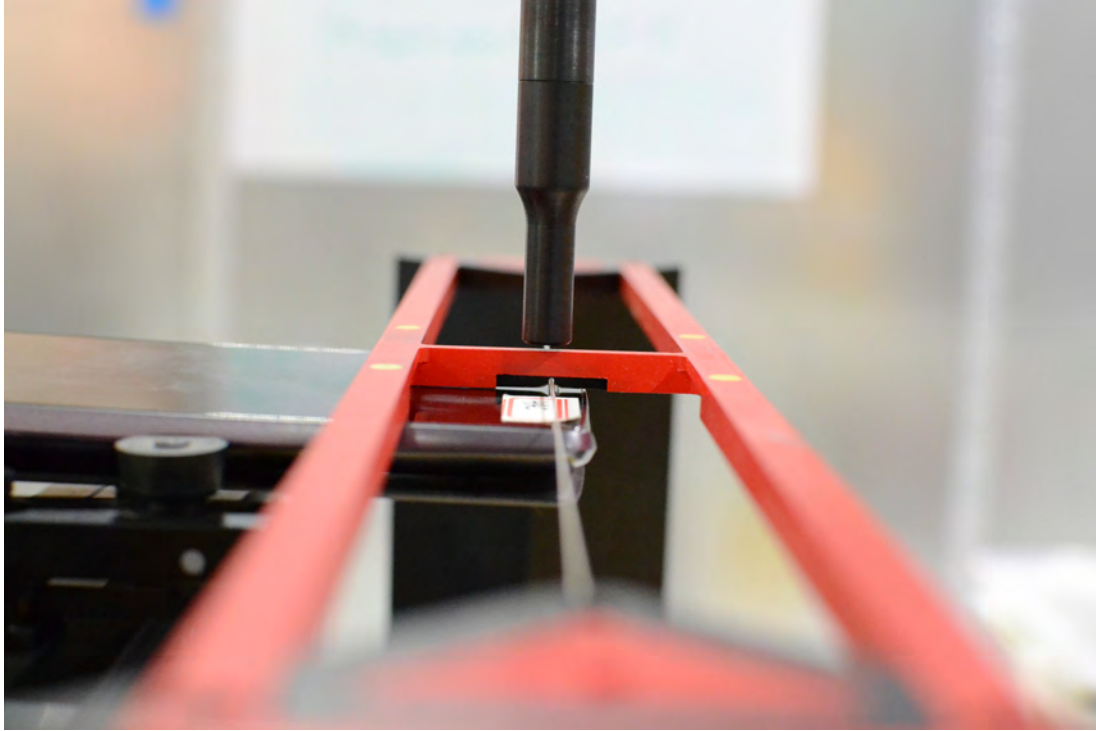
Figure 17-5 HAC Phantom Plane Alignment (Wireless Charging Cover - Open)
