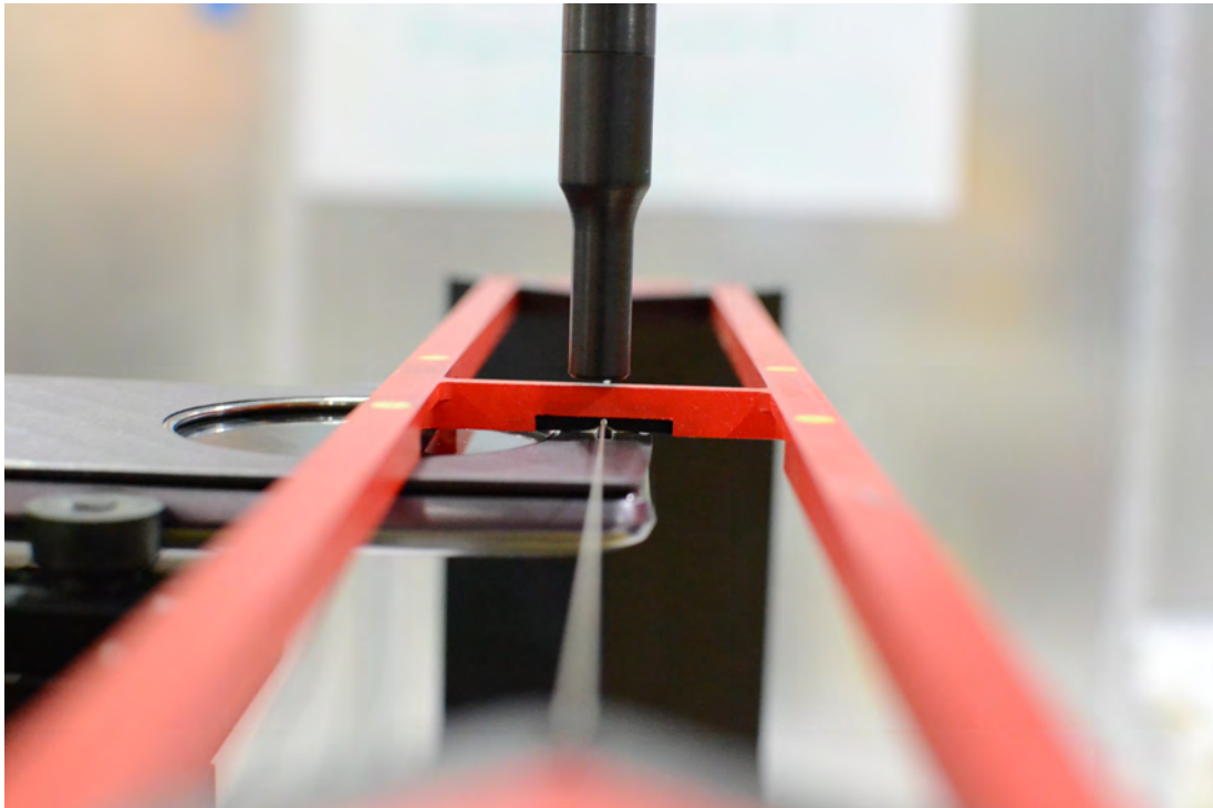
Figure 17-6 HAC Phantom Plane Alignment (Wireless Charging Cover - Closed)
