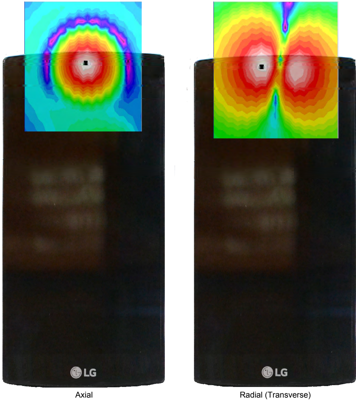
Figure 12-7 T-Coil Scan Overlay Magnetic Field Distributions
