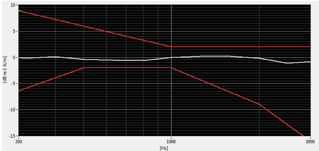
Figure 6-1 Axial Frequency Response
