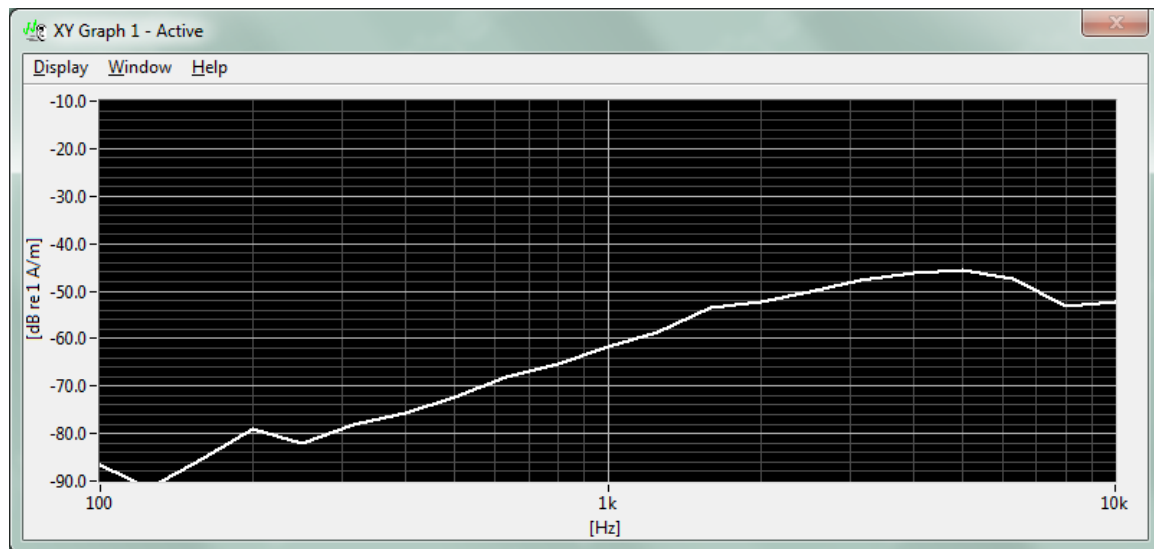
Figure 6-3 Worst-case ABM2 Plot for UMTS
