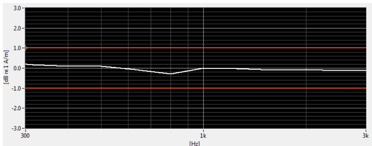
Figure 6-4 Helmholtz Coil Validation for Frequency Response
