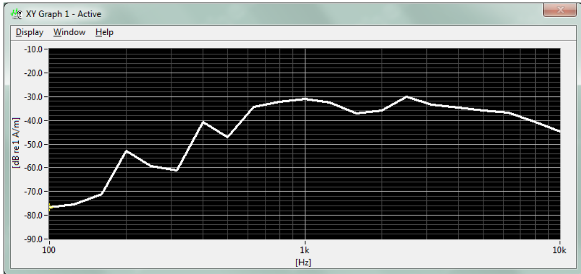
Figure 6-2 Worst-case ABM2 Plot for GSM
