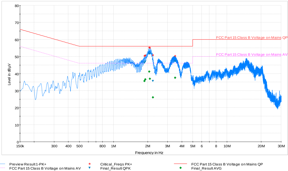
Plot 6-55. Line-Conducted Test Plot (N)
