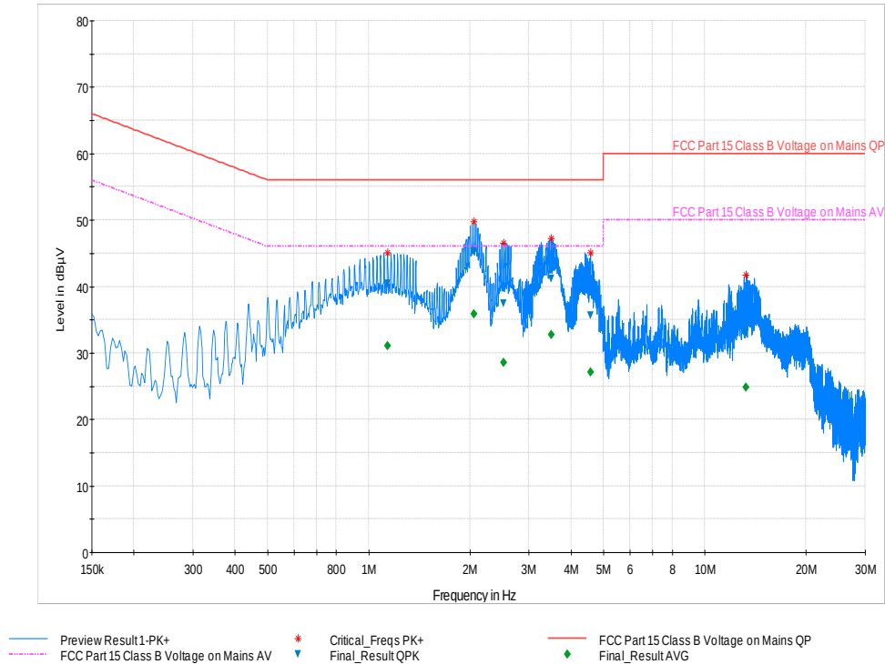
Plot 6-54. Line-Conducted Test Plot (L1)
