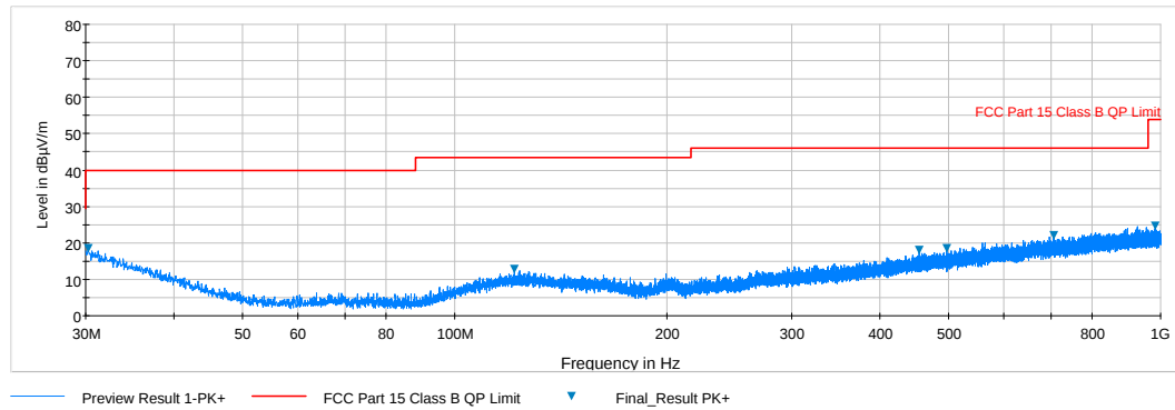
Plot 6-13. Radiated Spurious Plot below 1GHz (Pol. H)
