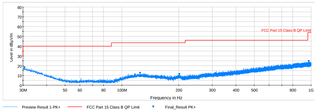
Plot 6-14. Radiated Spurious Plot below 1GHz (Pol. V)
