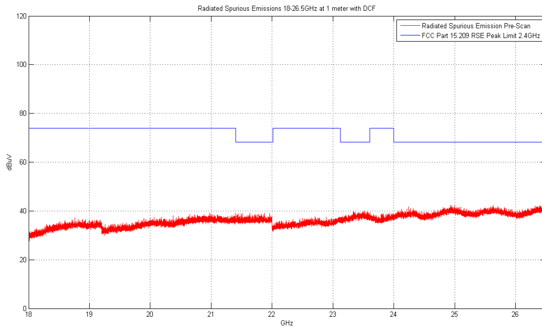
Plot 6-8. Radiated Spurious Plot above 18GHz (Pol. V)
