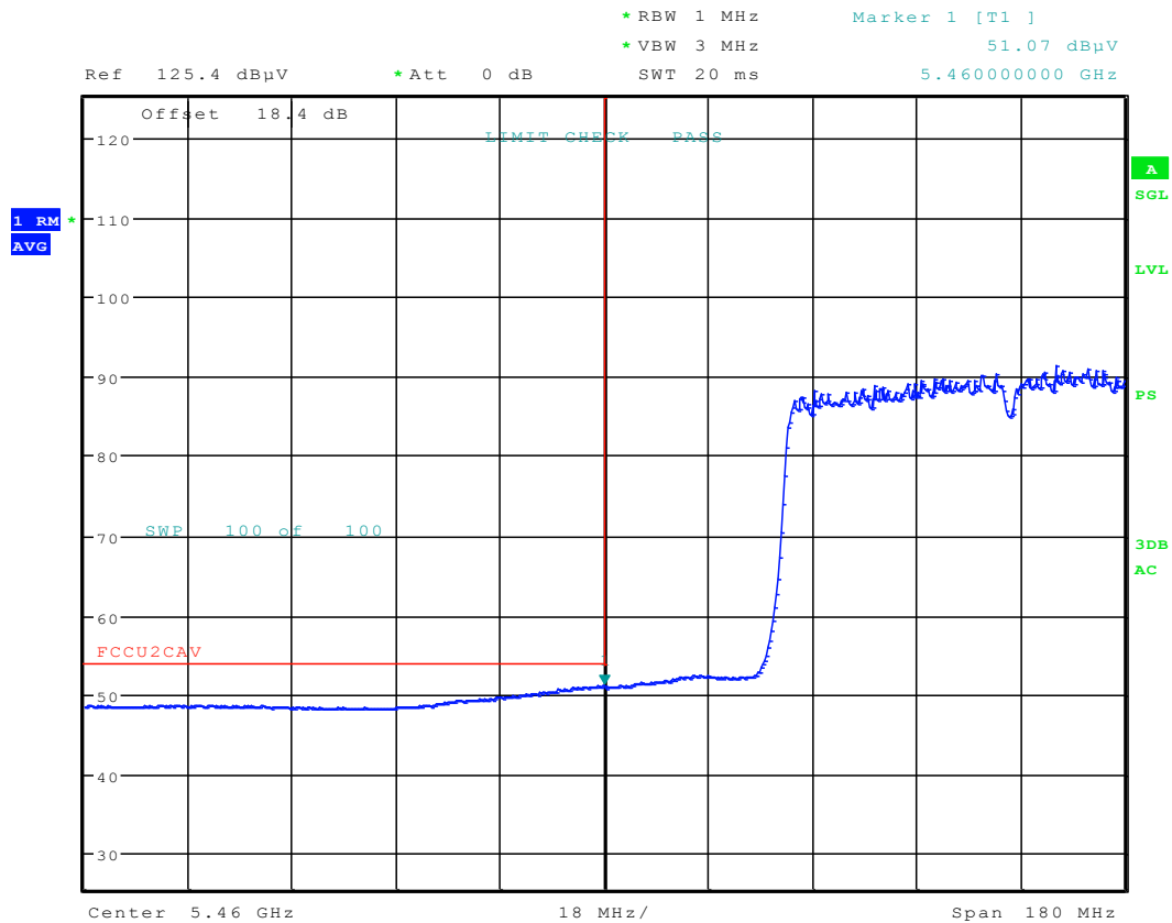
Plot 6-105. Radiated Restricted Lower Band Edge Plot (Average – UNII Band 2C)
