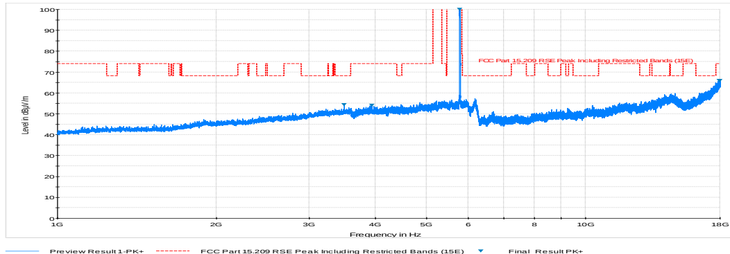
Plot 6-83. Radiated Spurious Plot above 1GHz (802.11a – U3 Ch. 157, Ant. Pol. H)
