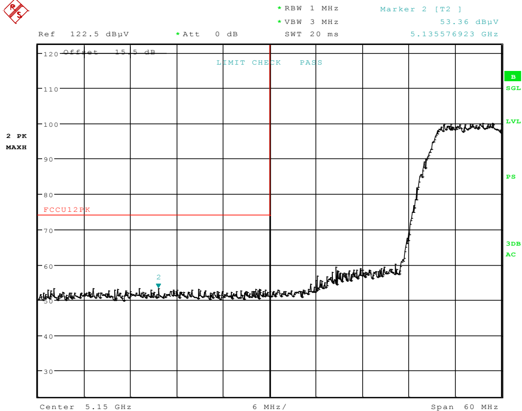
Plot 6-88. Radiated Restricted Lower Band Edge Plot (Peak – UNII Band 1)
