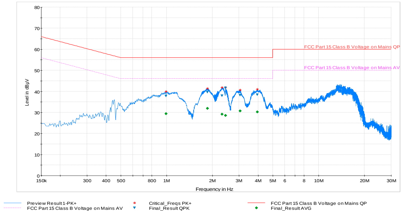
Plot 6-117. Line Conducted Plot with 802.11a UNII Band 3 (N)
