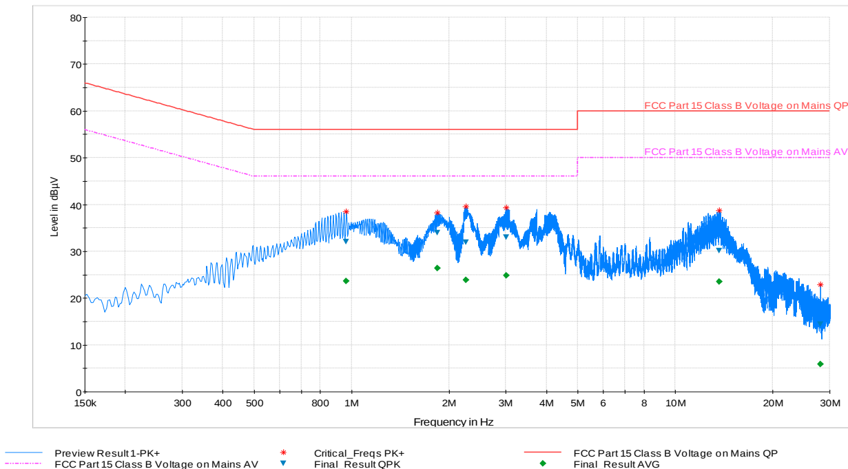
Plot 6-110. Line Conducted Plot with 802.11a UNII Band 1 (L1)
