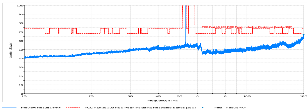
Plot 6-79. Radiated Spurious Plot above 1GHz (802.11a – U2A Ch. 56, Ant. Pol. H)
