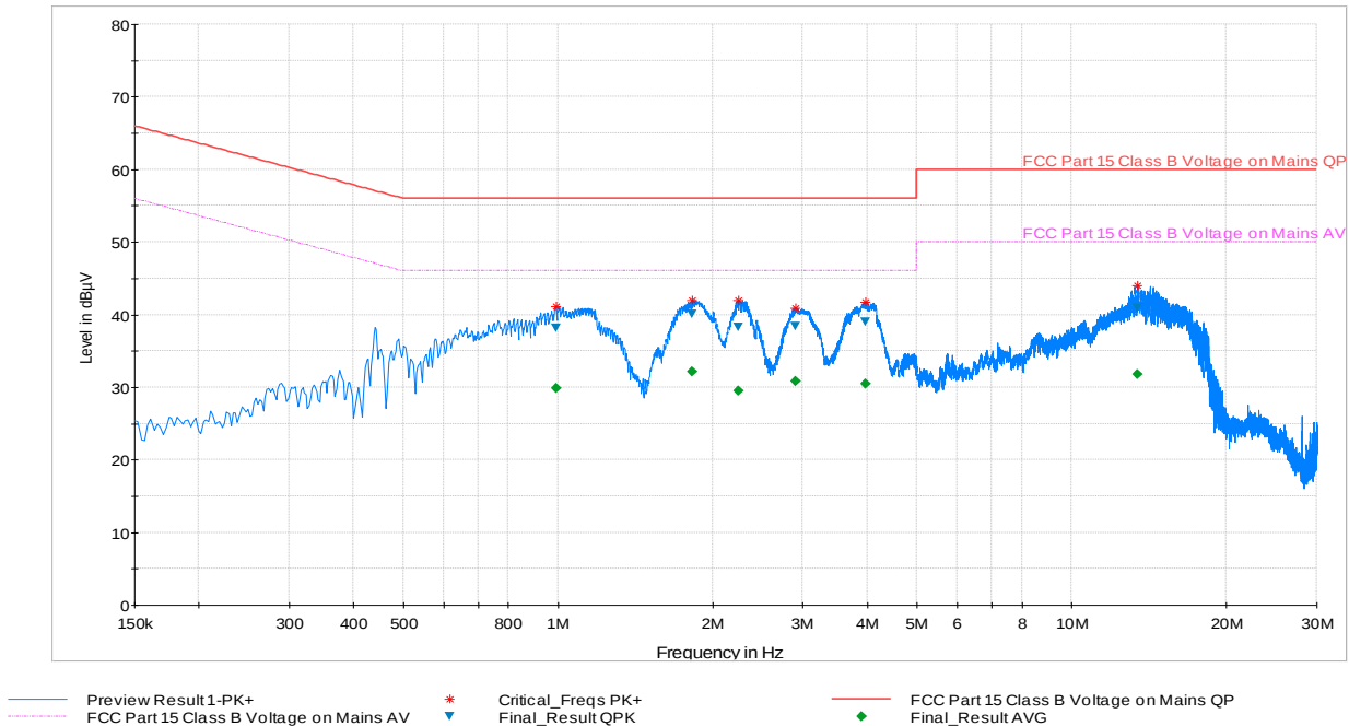
Plot 6-111. Line Conducted Plot with 802.11a UNII Band 1 (N)
