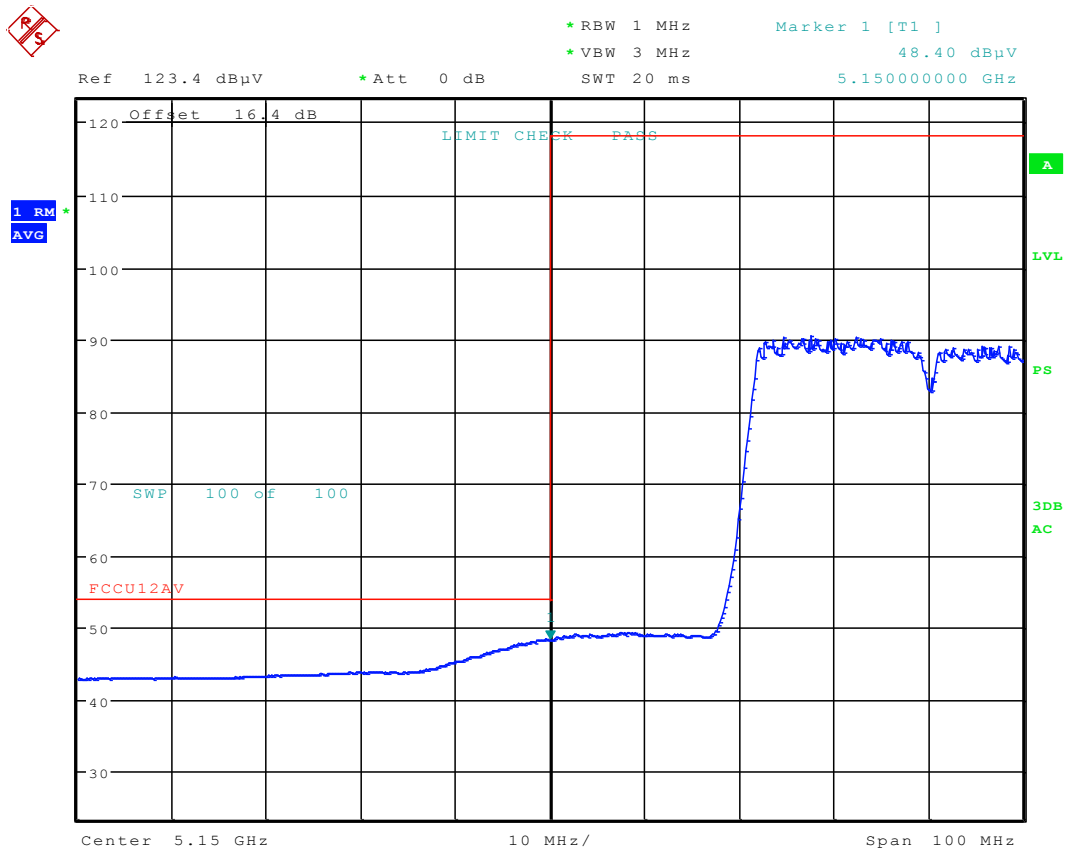
Plot 6-94. Radiated Restricted Lower Band Edge Plot (Average – UNII Band 1)
