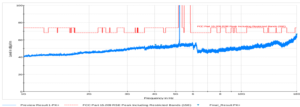
Plot 6-77. Radiated Spurious Plot above 1GHz (802.11a – U1 Ch. 40, Ant. Pol. H)
