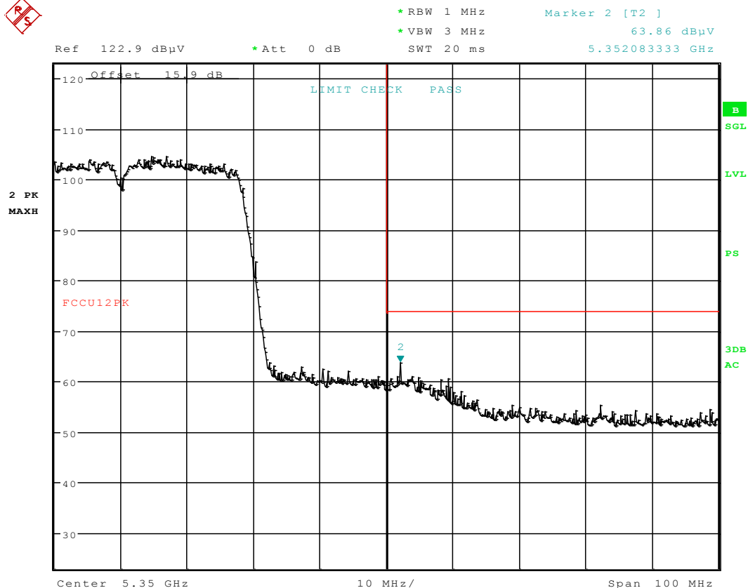
Plot 6-97. Radiated Restricted Upper Band Edge Plot (Peak – UNII Band 2A)
