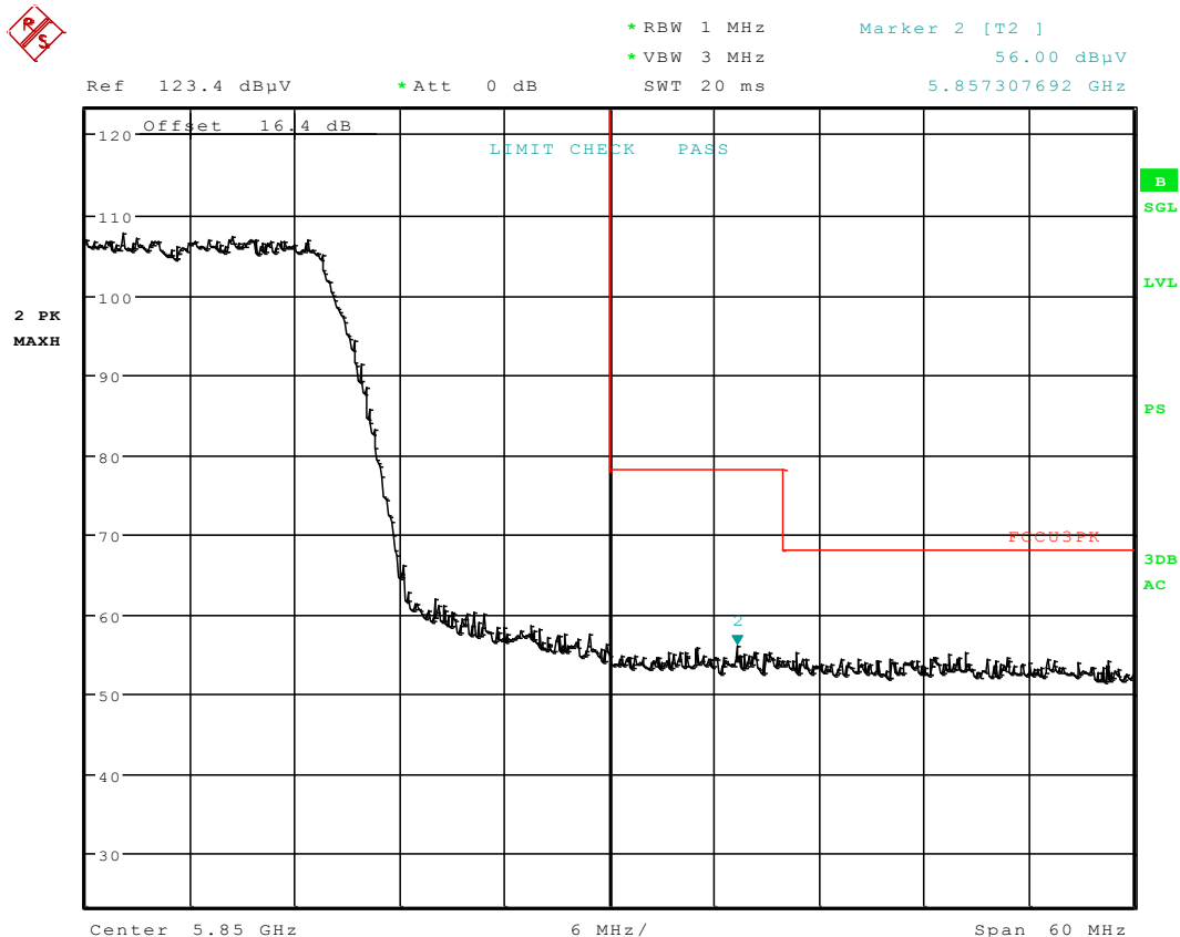
Plot 6-93. Radiated Upper Band Edge Plot (Peak – UNII Band 3)
