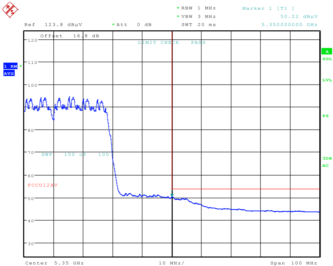
Plot 6-96. Radiated Restricted Upper Band Edge Plot (Average – UNII Band 2A)
