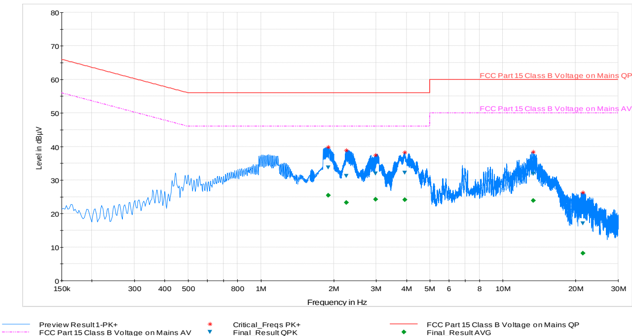
Plot 6-116. Line Conducted Plot with 802.11a UNII Band 3 (L1)
