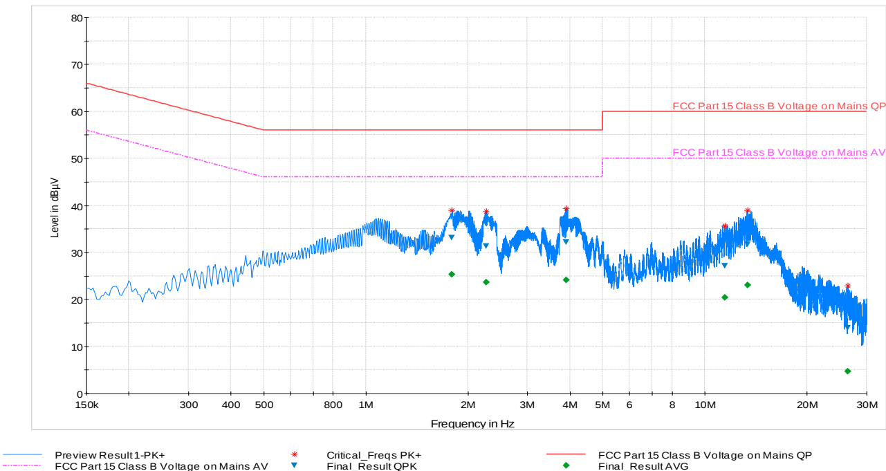
Plot 6-114. Line Conducted Plot with 802.11a UNII Band 2C (L1)
