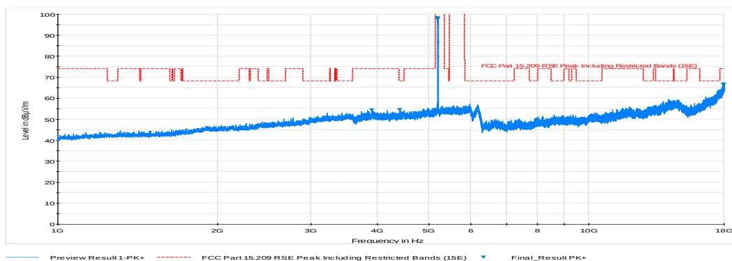
Plot 6-78. Radiated Spurious Plot above 1GHz (802.11a – U1 Ch. 40, Ant. Pol. V)
