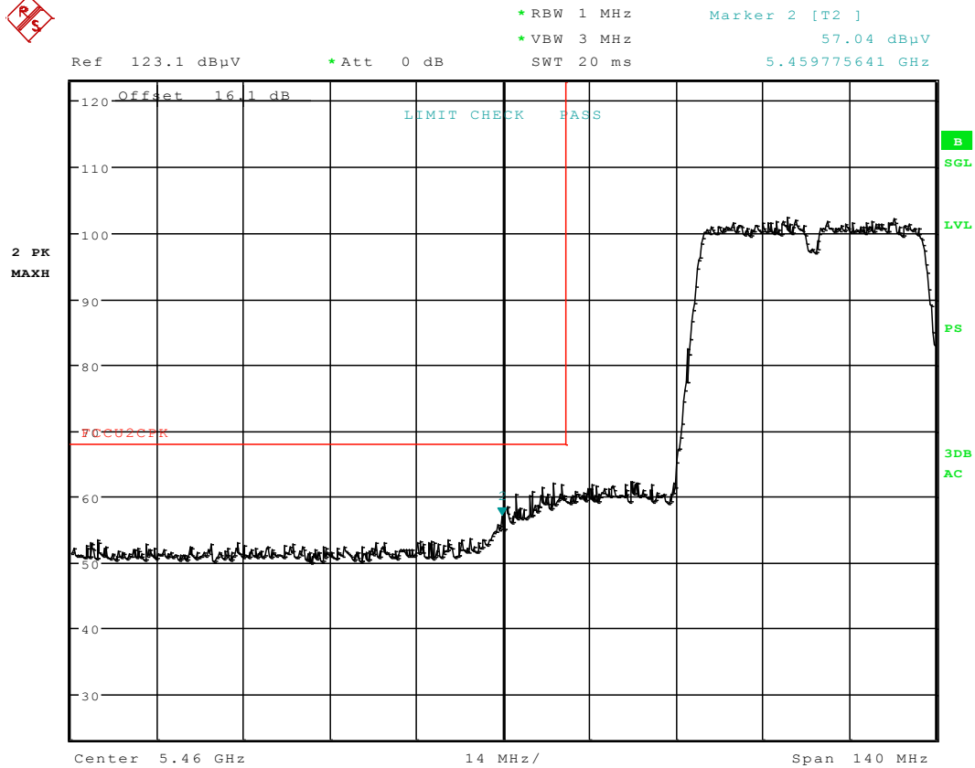
Plot 6-99. Radiated Restricted Lower Band Edge Plot (Peak – UNII Band 2C)
