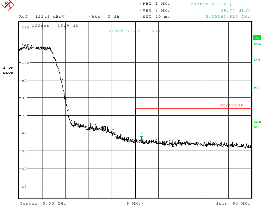
Plot 6-90. Radiated Restricted Upper Band Edge Plot (Peak – UNII Band 2A)
