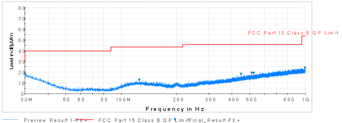
Plot 6-108. Radiated Spurious Plot below 1GHz (802.11a – U3 Ch. 157, Ant. Pol. H)
