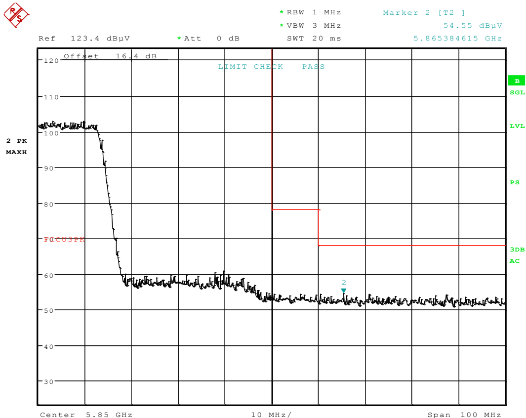
Plot 6-100. Radiated Upper Band Edge Plot (Peak – UNII Band 3)
