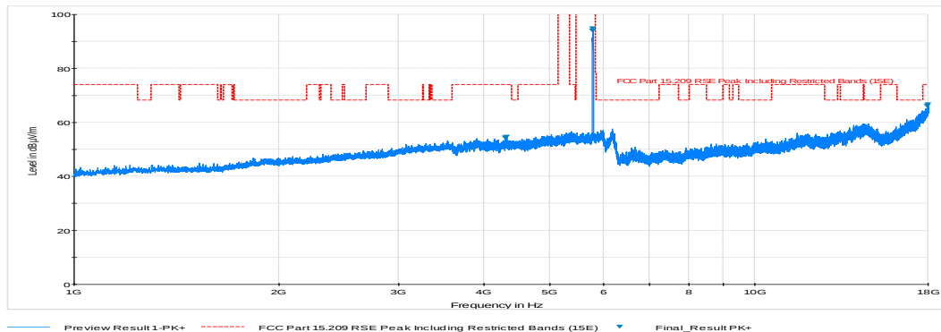
Plot 6-84. Radiated Spurious Plot above 1GHz (802.11a – U3 Ch. 157, Ant. Pol. V)
