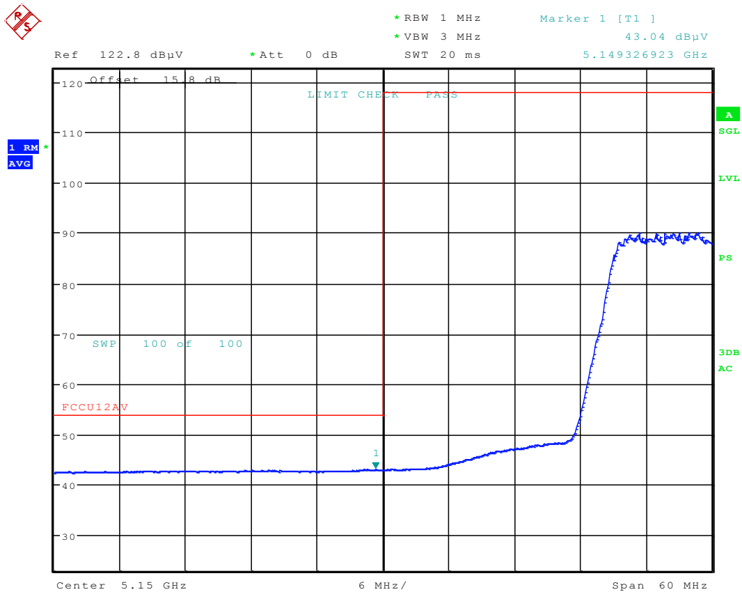
Plot 6-87. Radiated Restricted Lower Band Edge Plot (Average – UNII Band 1)
