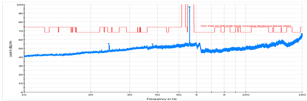
Plot 6-82. Radiated Spurious Plot above 1GHz (802.11a – U2C Ch. 116, Ant. Pol. V)
