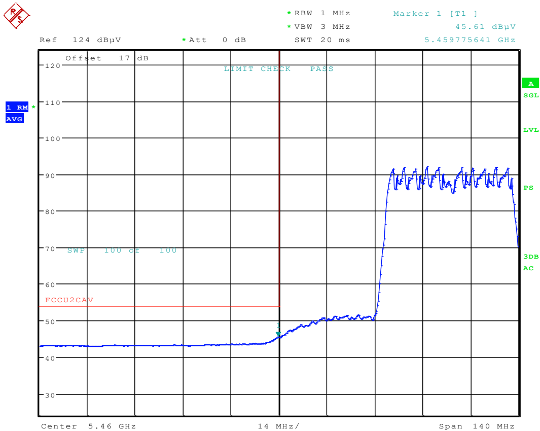
Plot 6-98. Radiated Restricted Lower Band Edge Plot (Average – UNII Band 2C)
