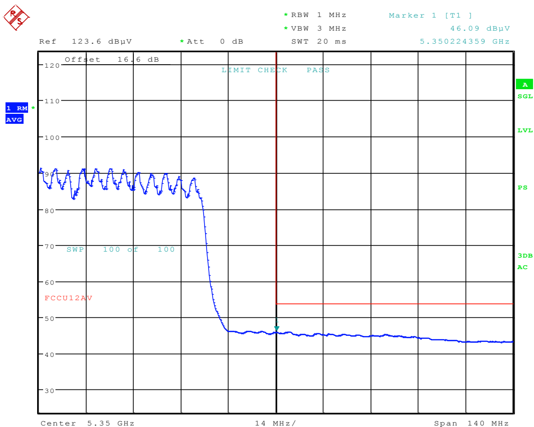
Plot 6-103. Radiated Restricted Upper Band Edge Plot (Average – UNII Band 2A)
