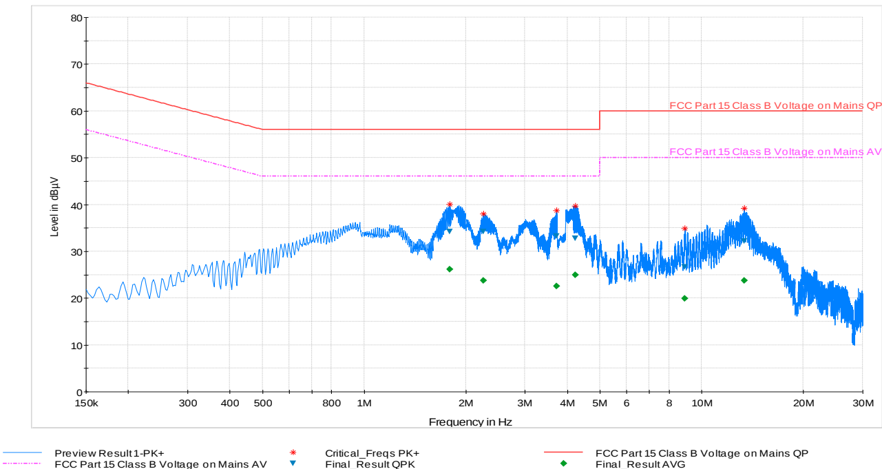
Plot 6-112. Line Conducted Plot with 802.11a UNII Band 2A (L1)
