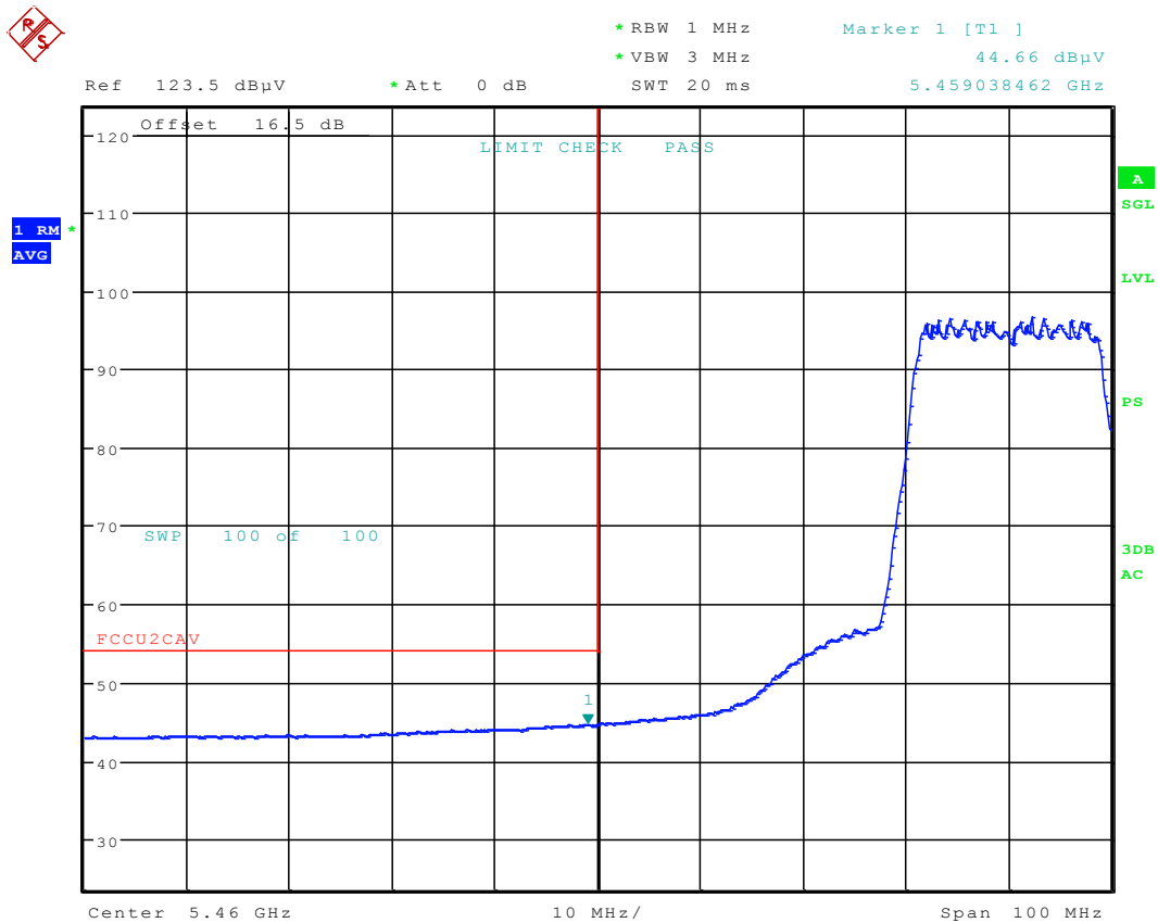
Plot 6-91. Radiated Restricted Lower Band Edge Plot (Average – UNII Band 2C)
