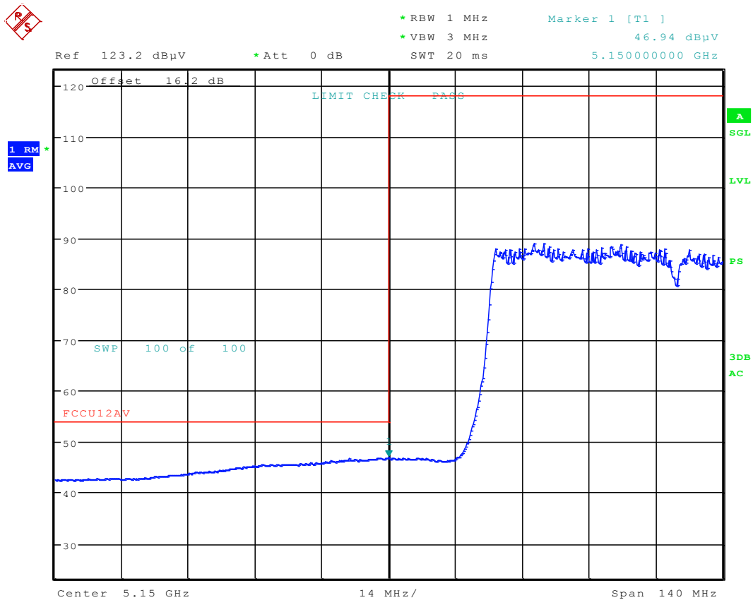
Plot 6-101. Radiated Restricted Lower Band Edge Plot (Average – UNII Band 1)
