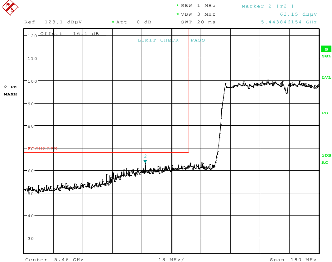
Plot 6-106. Radiated Restricted Lower Band Edge Plot (Peak – UNII Band 2C)
