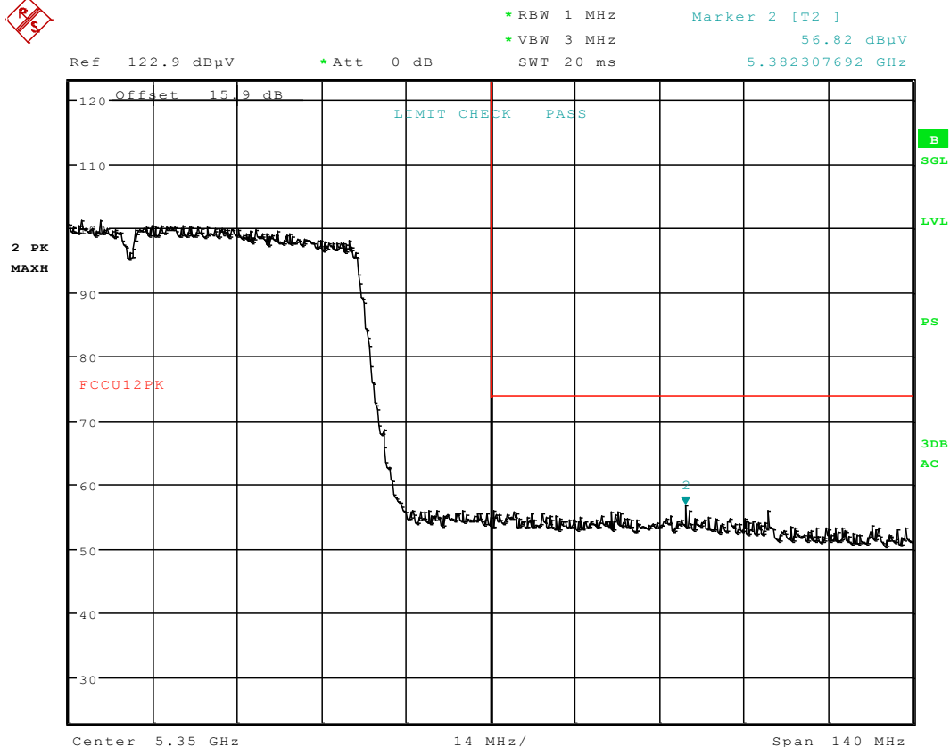
Plot 6-104. Radiated Restricted Upper Band Edge Plot (Peak – UNII Band 2A)
