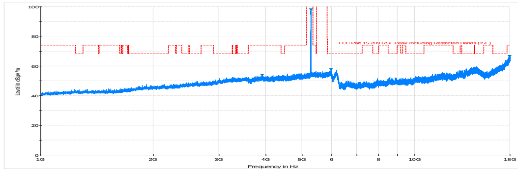
Plot 6-80. Radiated Spurious Plot above 1GHz (802.11a – U2A Ch. 56, Ant. Pol. V)
