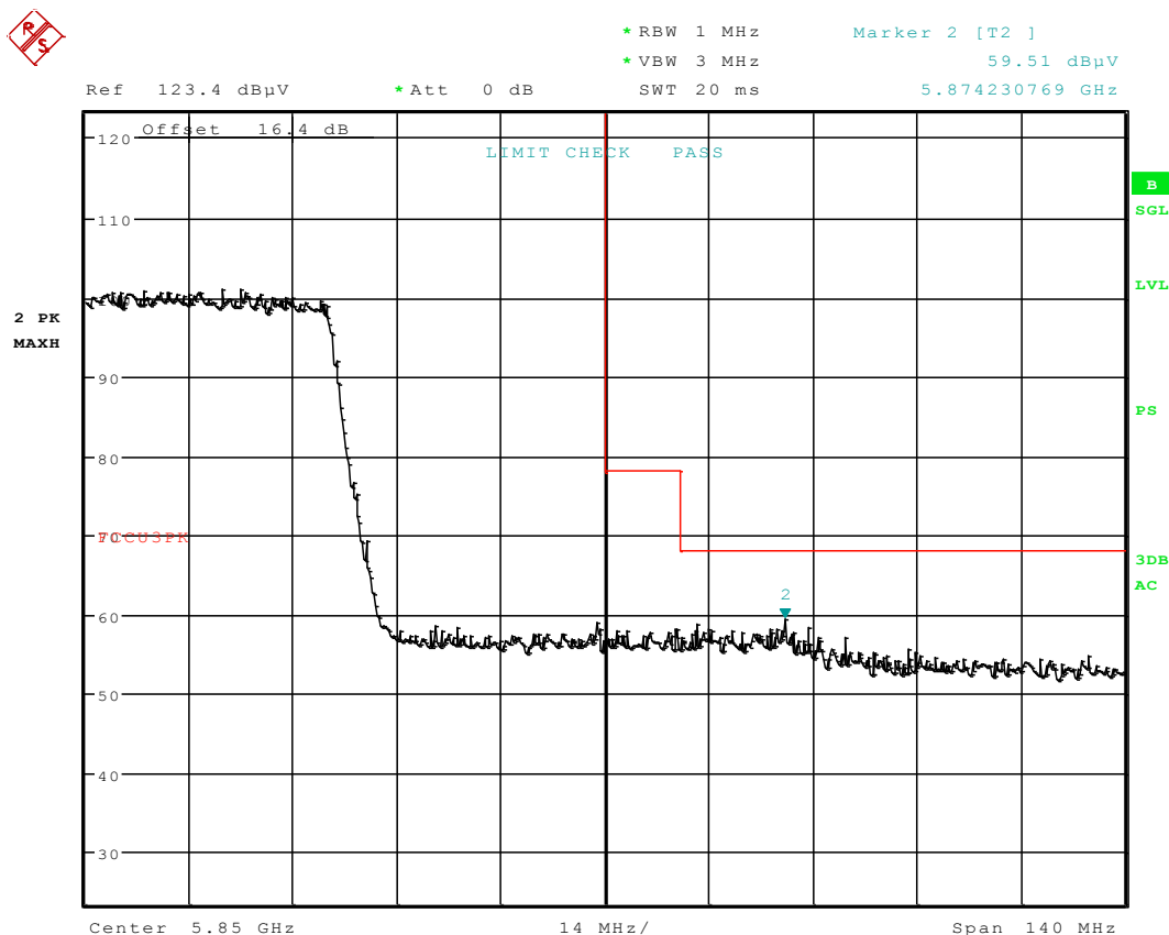
Plot 6-107. Radiated Upper Band Edge Plot (Peak – UNII Band 3)
