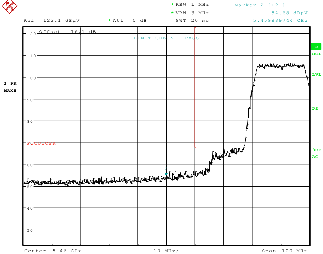
Plot 6-92. Radiated Restricted Lower Band Edge Plot (Peak – UNII Band 2C)
