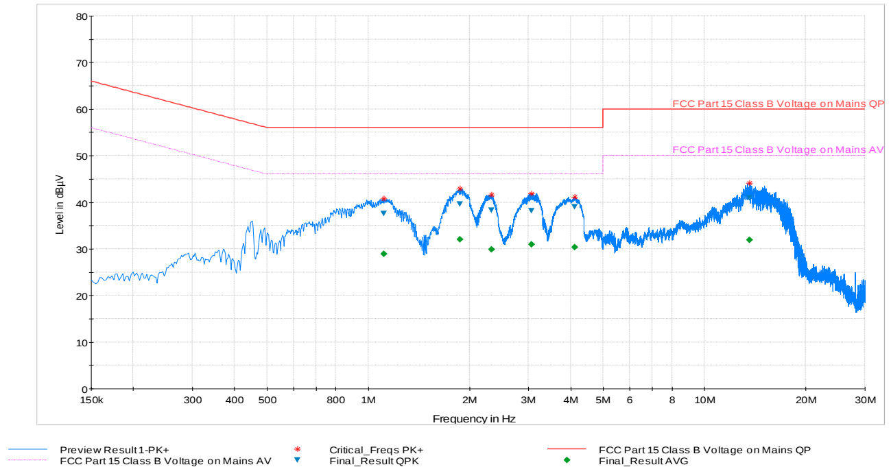
Plot 6-115. Line Conducted Plot with 802.11a UNII Band 2C (N)
