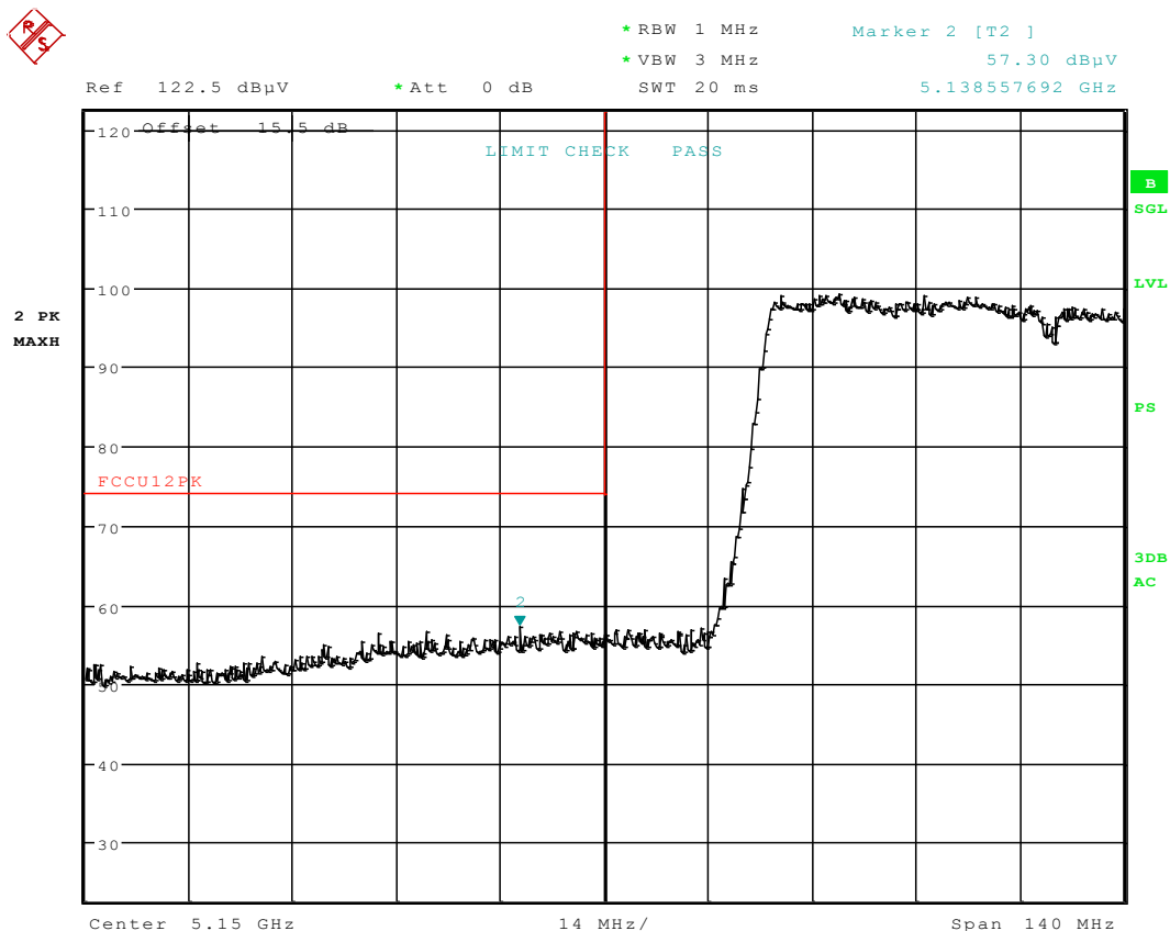
Plot 6-102. Radiated Restricted Lower Band Edge Plot (Peak – UNII Band 1)
