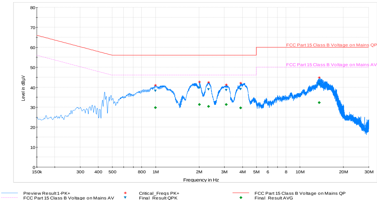
Plot 6-113. Line Conducted Plot with 802.11a UNII Band 2A (N)
