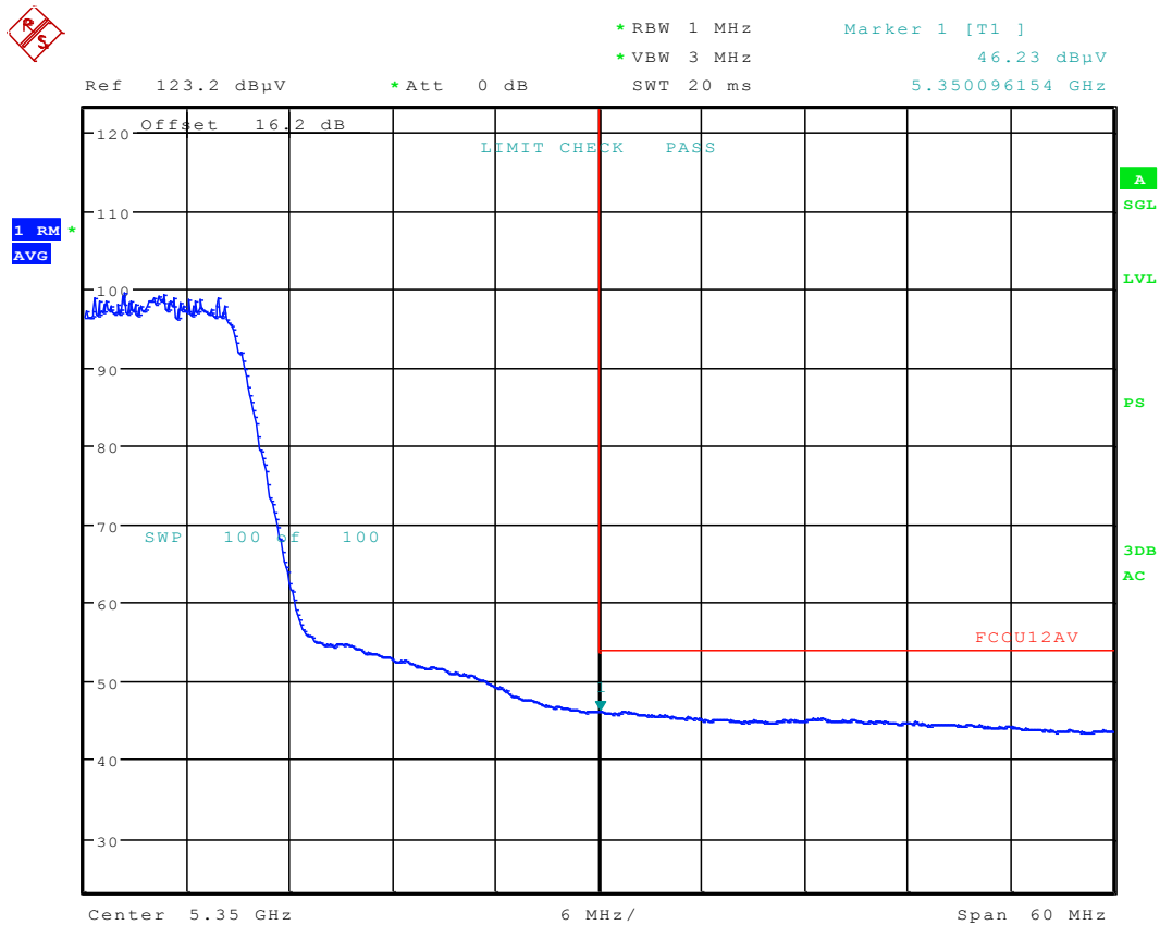
Plot 6-89. Radiated Restricted Upper Band Edge Plot (Average – UNII Band 2A)
