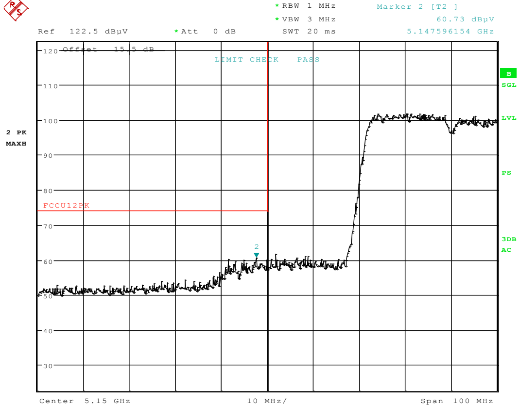
Plot 6-95. Radiated Restricted Lower Band Edge Plot (Peak – UNII Band 1)
