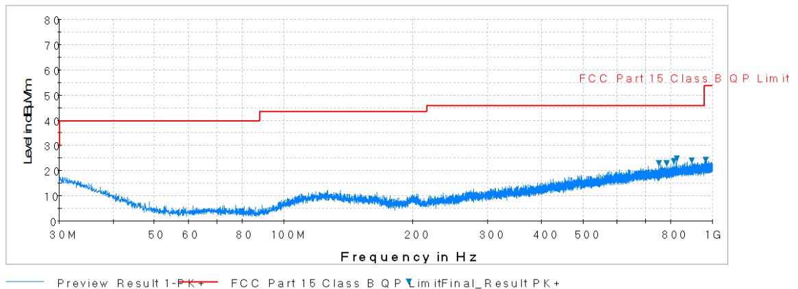
Plot 6-109. Radiated Spurious Plot below 1GHz (802.11a – U3 Ch. 157, Ant. Pol. V)
