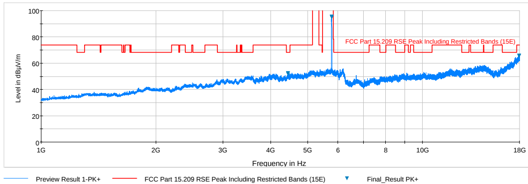
Plot 6-8. Radiated Spurious Plot above 1GHz (802.11a – U3 Ch. 157, Ant. Pol. V)
