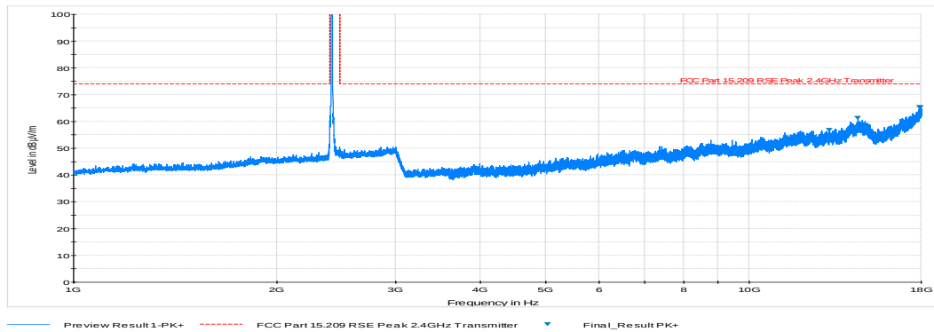
Plot 6-32. Radiated Spurious Plot above 1GHz (802.11b – Ch. 1, Ant. Pol. V)
