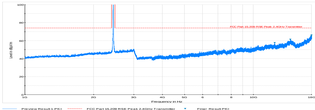
Plot 6-34. Radiated Spurious Plot above 1GHz (802.11b – Ch. 6, Ant. Pol. V)
