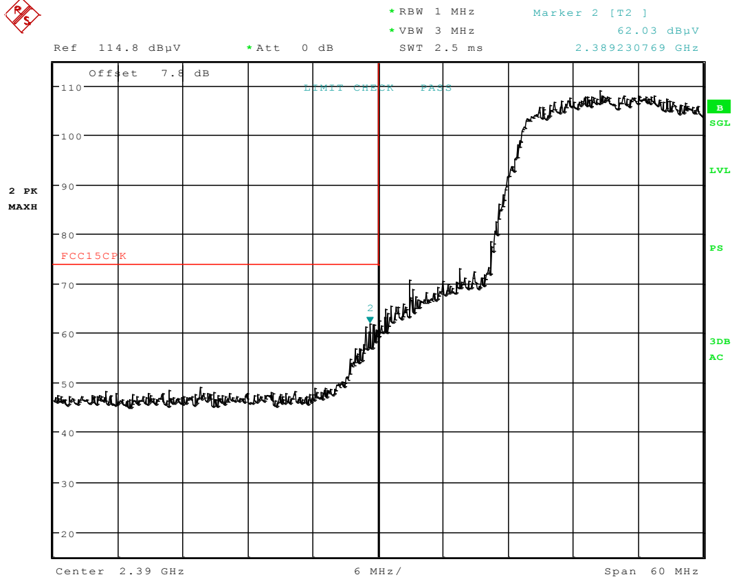
Plot 6-40. Radiated Restricted Lower Band Edge Measurement (Peak)
