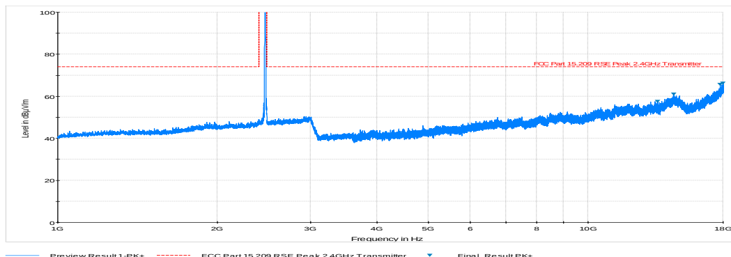
Plot 6-36. Radiated Spurious Plot above 1GHz (802.11b – Ch. 11, Ant. Pol. V)
