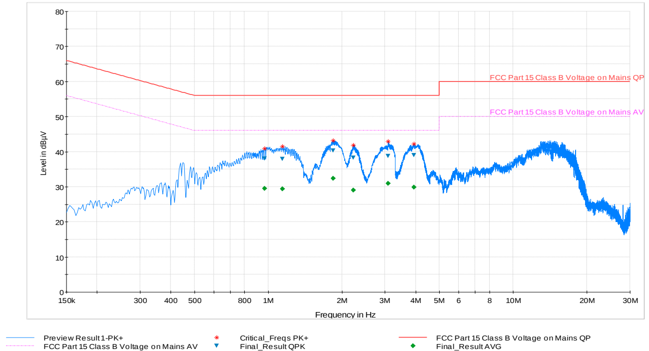
Plot 6-46. Line Conducted Plot with 802.11b (N)
