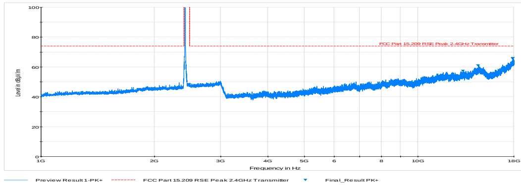
Plot 6-31. Radiated Spurious Plot above 1GHz (802.11b – Ch. 1, Ant. Pol. H)
