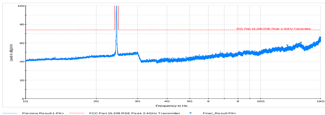
Plot 6-33. Radiated Spurious Plot above 1GHz (802.11b – Ch. 6, Ant. Pol. H)
