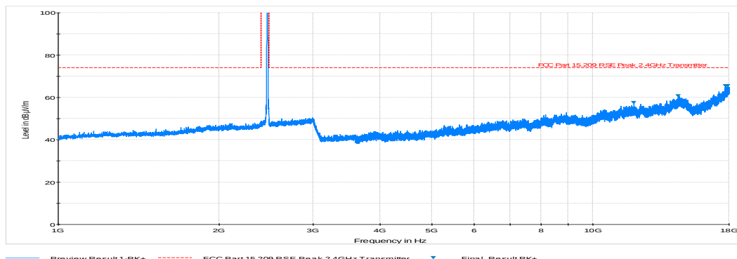
Plot 6-35. Radiated Spurious Plot above 1GHz (802.11b – Ch. 11, Ant. Pol. H)
