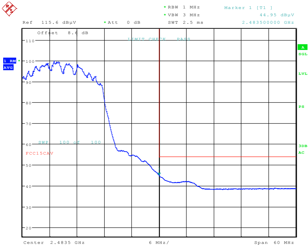
Plot 6-41. Radiated Restricted Upper Band Edge Measurement (Average)
