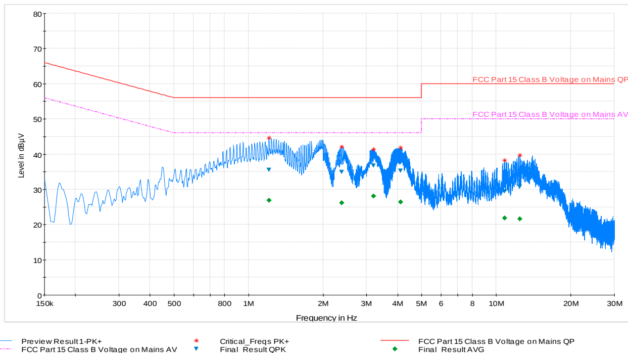
Plot 6-45. Line Conducted Plot with 802.11b (L1)
