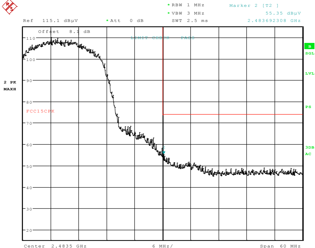
Plot 6-42. Radiated Restricted Upper Band Edge Measurement (Peak)
