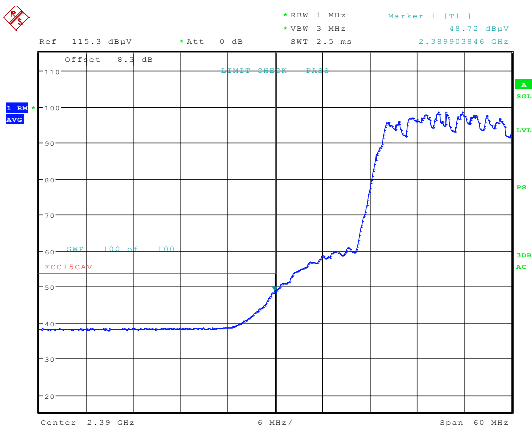
Plot 6-39. Radiated Restricted Lower Band Edge Measurement (Average)
