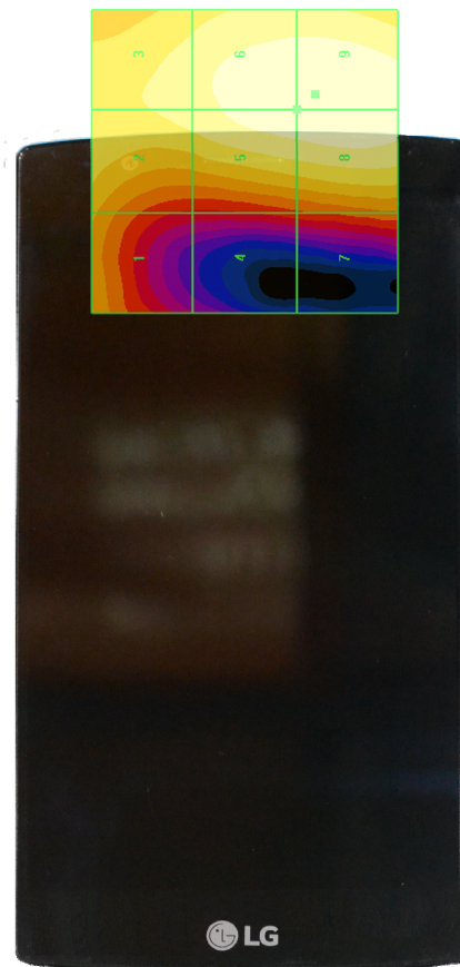
Figure 17-8 E-Field WD Scan overlay
