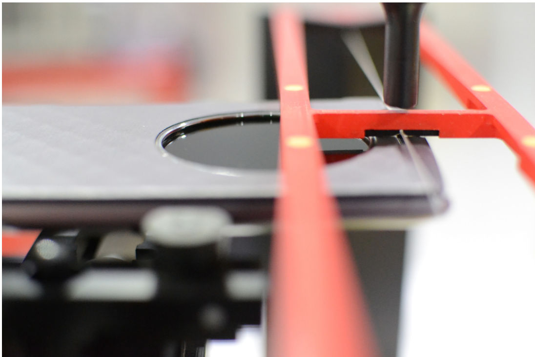
Figure 17-6 HAC Phantom Plane Alignment, Wireless Charging Cover (Cover Closed)
