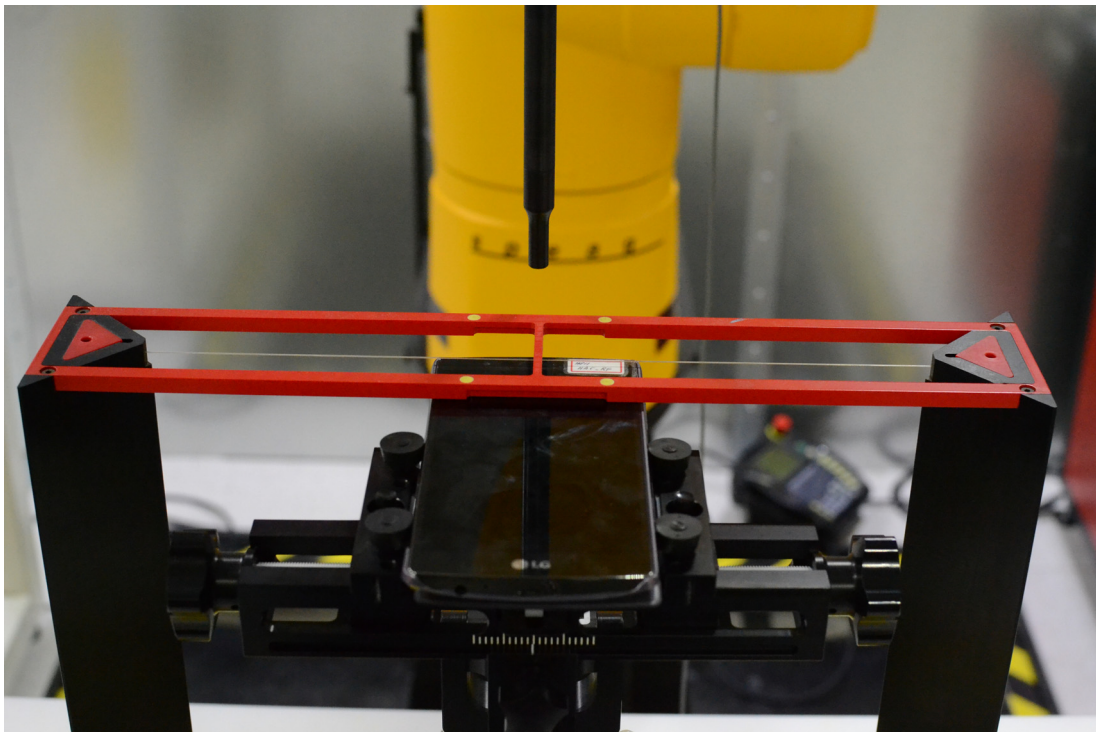
Figure 17-2 Ear Reference Point HAC Phantom Alignment, Wireless Charging Cover (Cover Open)
