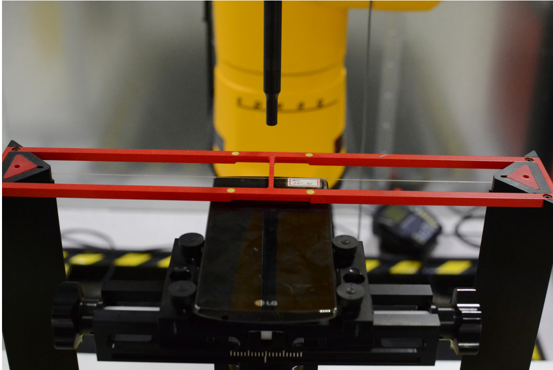
Figure 17-1 Ear Reference Point HAC Phantom Alignment, Standard Cover
