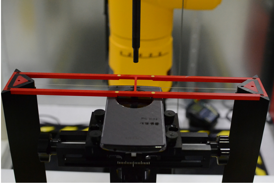
Figure 17-3 Ear Reference Point HAC Phantom Alignment, Wireless Charging Cover (Cover Closed)
