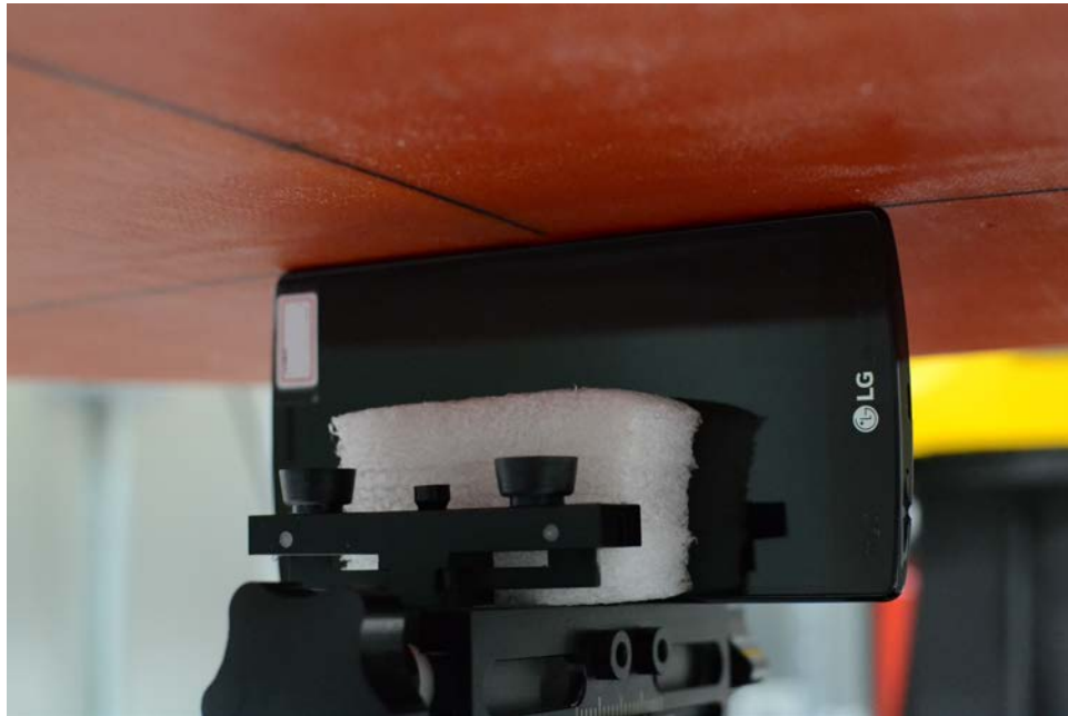
SAR Test Setup Photo 26: Right Edge, Standard Cover at 0 mm
