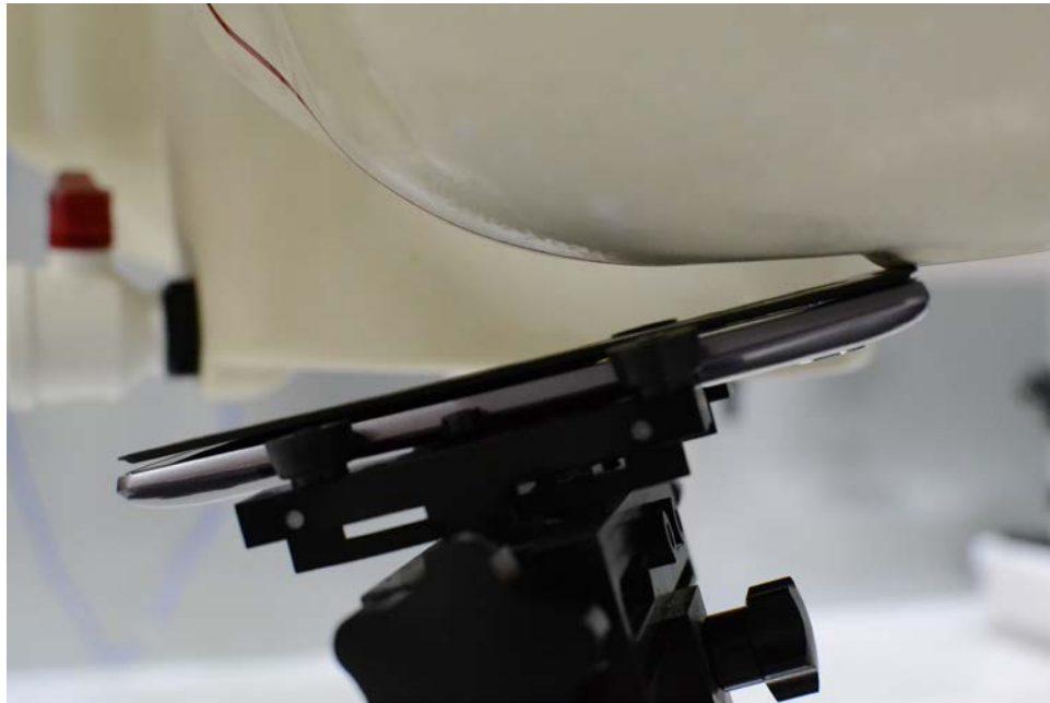
SAR Test Setup Photo 12: Left Tilt, Quick Cover (Closed)
