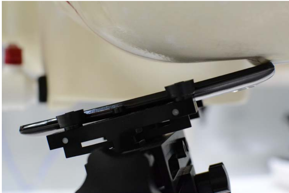
SAR Test Setup Photo 10: Left Tilt, Standard Cover
