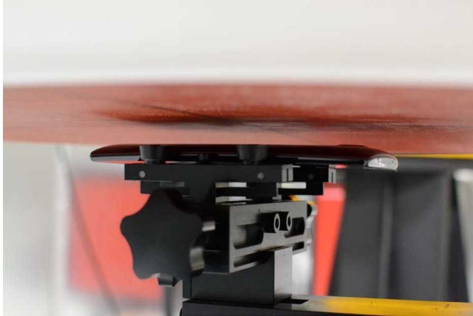
SAR Test Setup Photo 13: Back Side, Standard Cover at 10 mm
