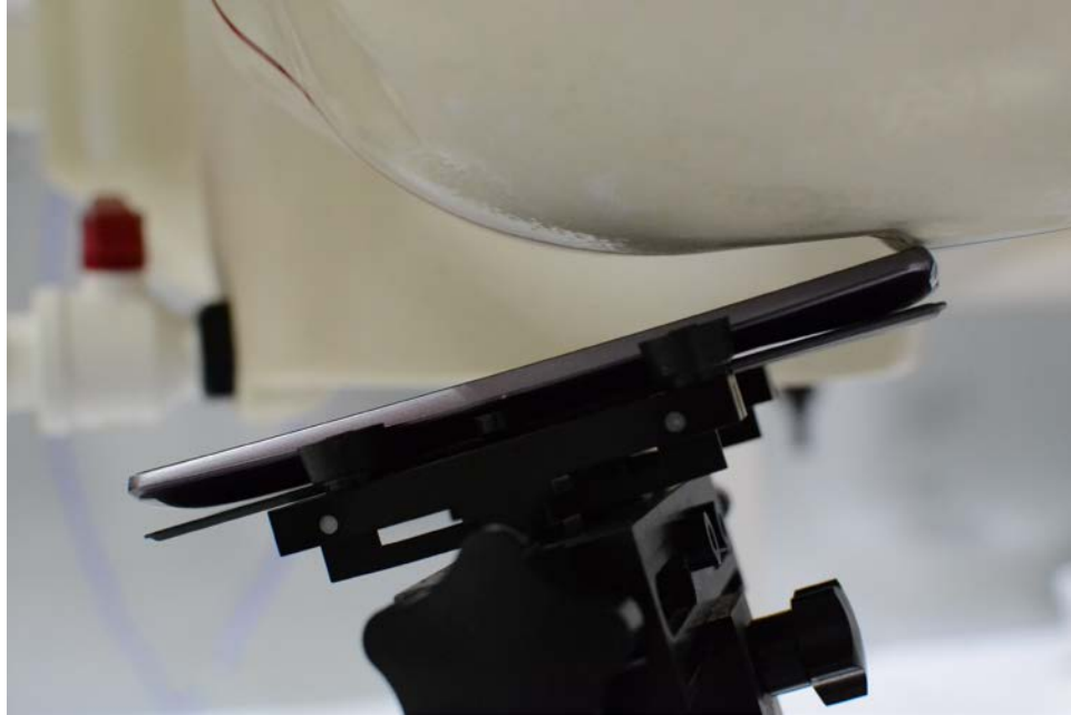
SAR Test Setup Photo 11: Left Tilt, Quick Cover (Open)
