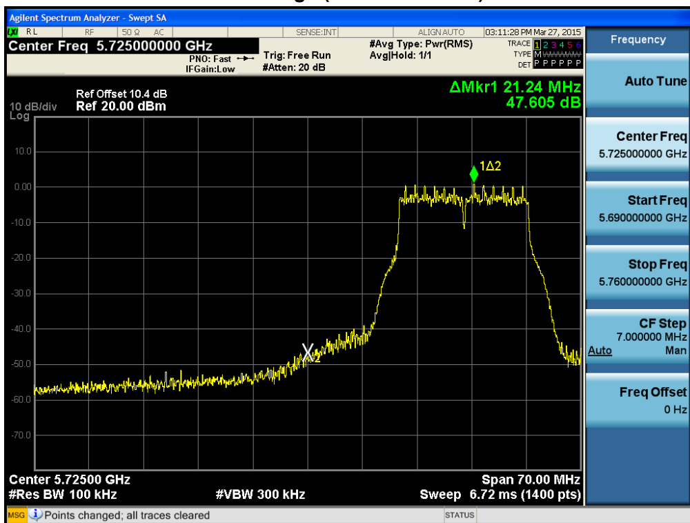
BandEdge (802.11a-CH 149)
