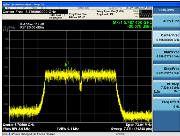
802.11n_40MHz BW UNII 3 BAND PSD
