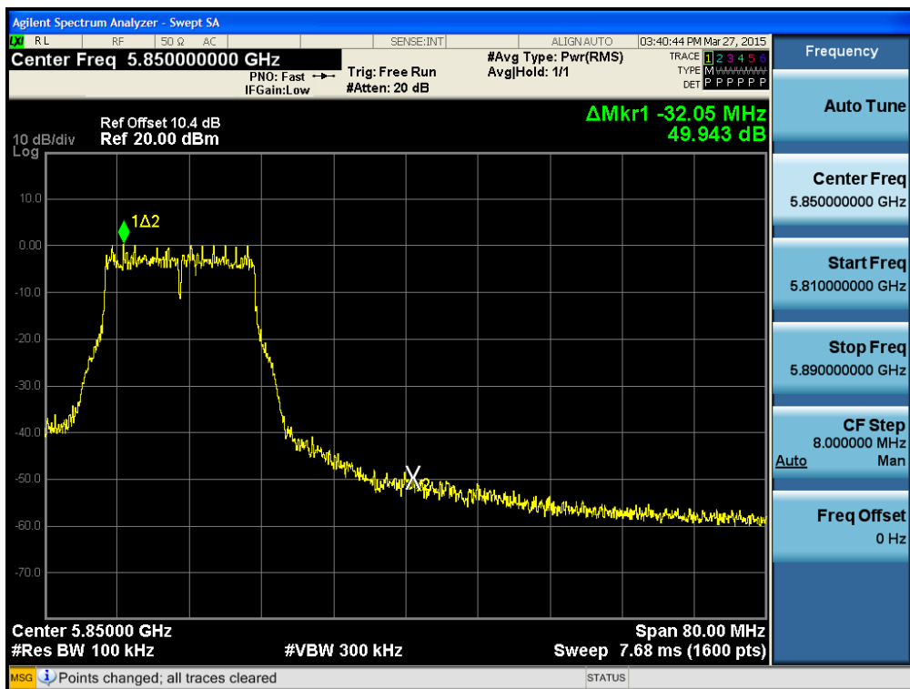
BandEdge (802.11a-CH 165)
