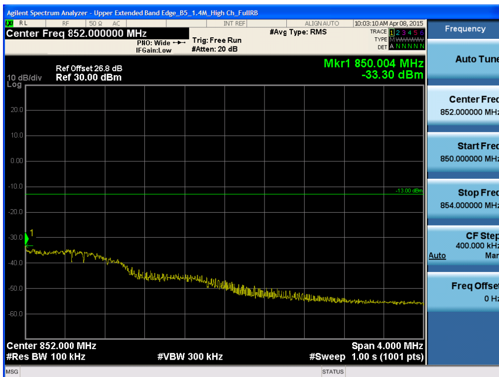
BAND 5. Upper Extended Band Edge Plot (1.4M BW Ch.20643 QPSK_RB6_0)
