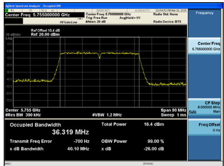
802.11ac_40 MHz BW UNII 3 BAND 26dB Bandwidth
