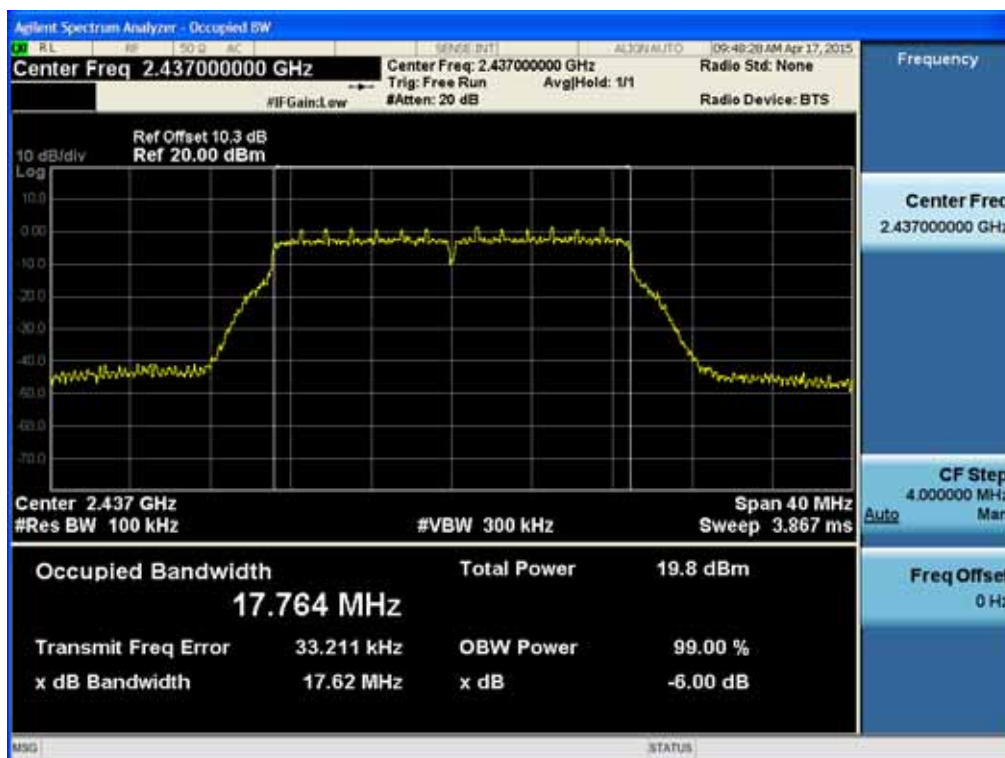
6dB Bandwidth plot (802.11ac_20MHz BW-CH 6)
