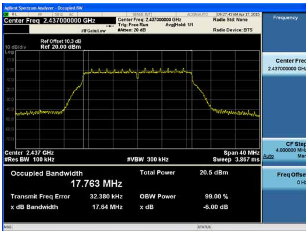
6dB Bandwidth plot (802.11n_20 MHz BW-CH 6)
