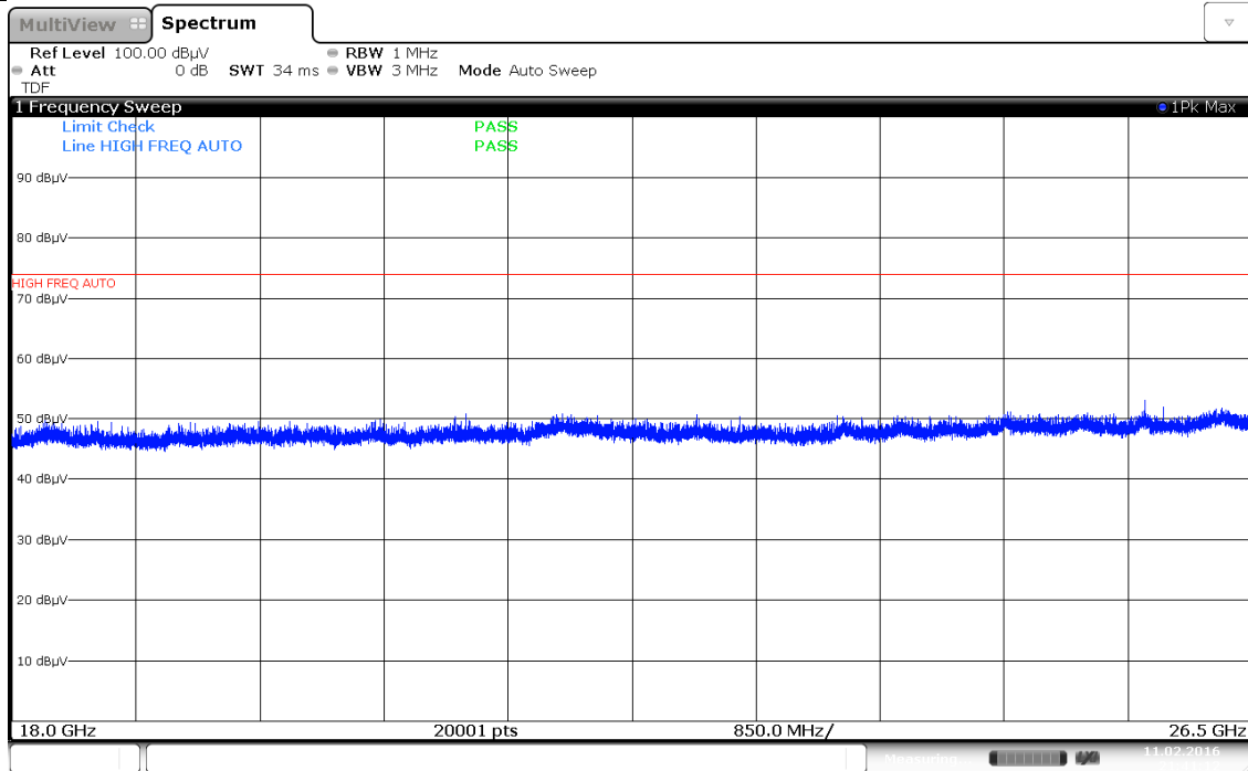
Plot 7-85. Radiated Spurious Plot above 18GHz (802.11a – Ant. Pol. H)
