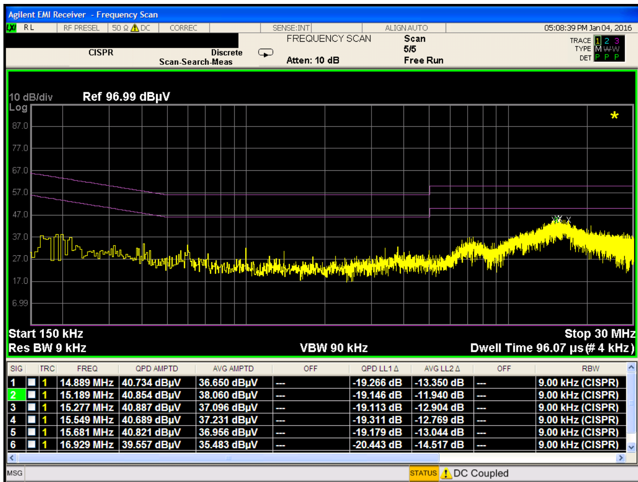
Plot 7-116. Line Conducted Plot with 802.11a UNII Band 1 (L1)
