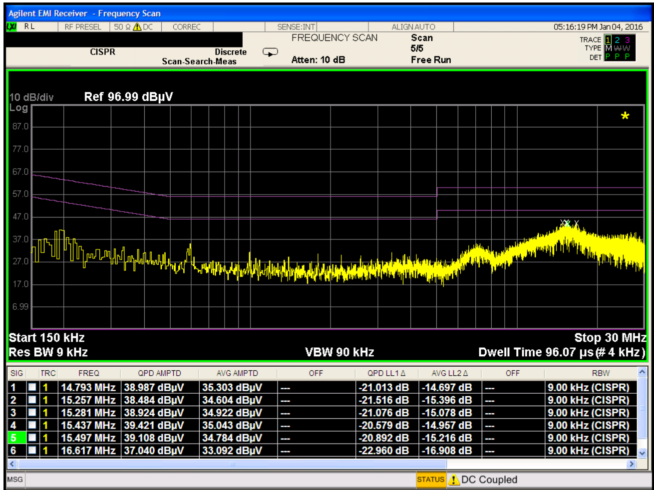
Plot 7-118. Line Conducted Plot with 802.11a UNII Band 2A (L1)
