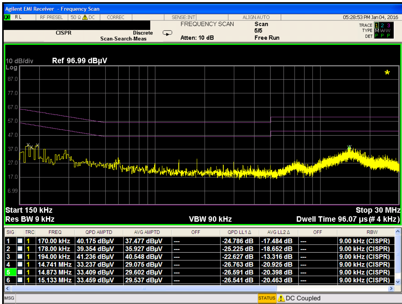
Plot 7-121. Line Conducted Plot with 802.11a UNII Band 2C (N)
