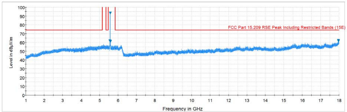
Plot 7-82. Radiated Spurious Plot above 1GHz (802.11a – U2C Ch. 116, Ant. Pol. V)
