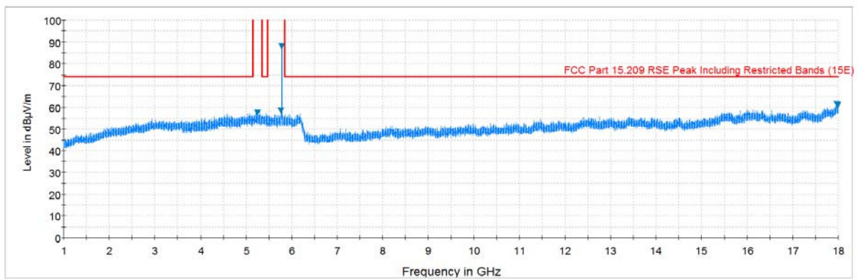
Plot 7-84. Radiated Spurious Plot above 1GHz (802.11a – U3 Ch. 157, Ant. Pol. V)
