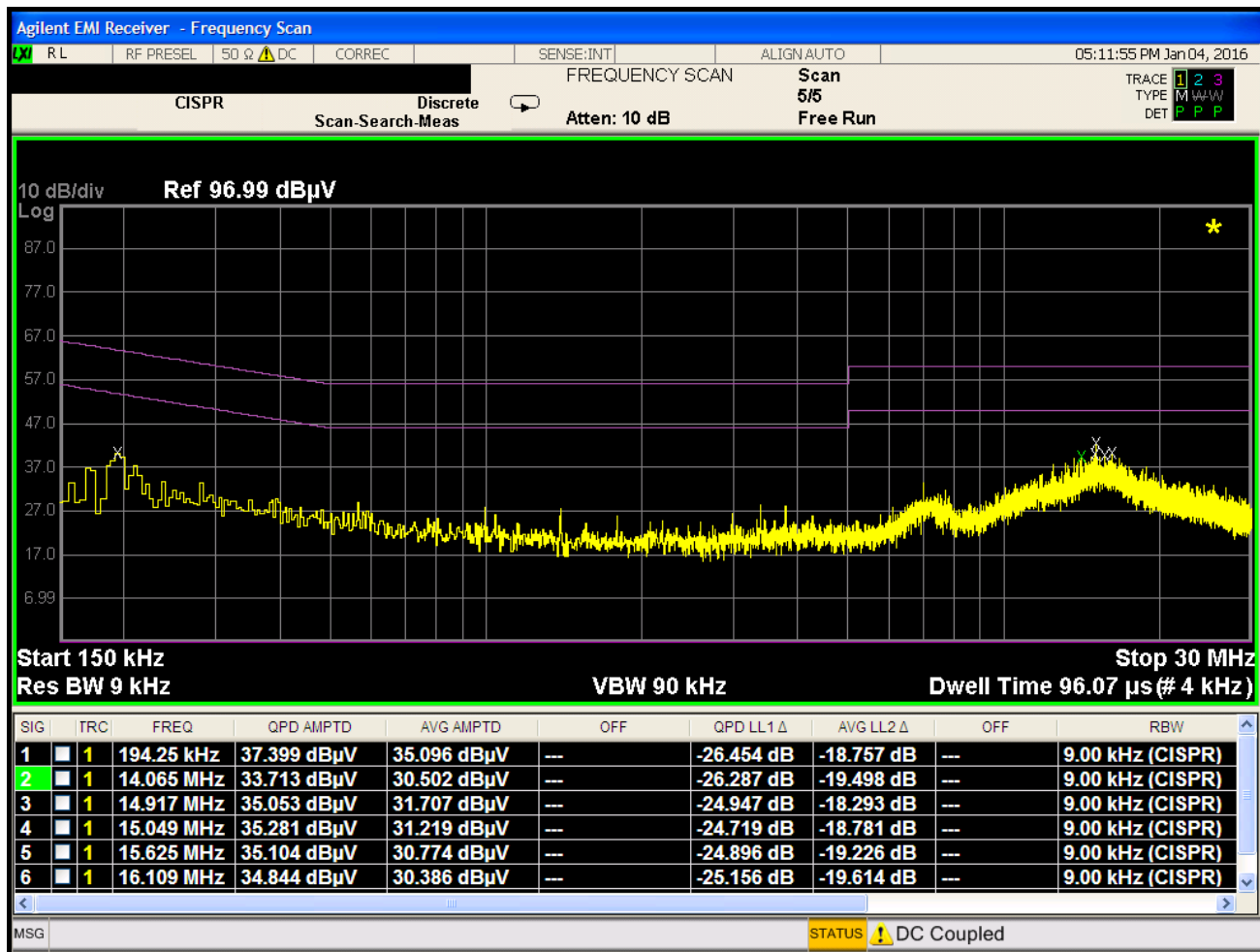
Plot 7-117. Line Conducted Plot with 802.11a UNII Band 1 (N)
