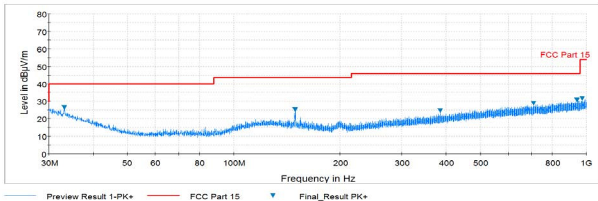
Plot 7-115. Radiated Spurious Plot below 1GHz (802.11a – U3 Ch. 157, Ant. Pol. V)
