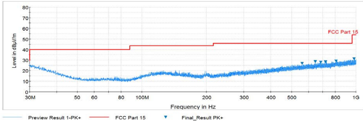
Plot 7-114. Radiated Spurious Plot below 1GHz (802.11a – U3 Ch. 157, Ant. Pol. H)
