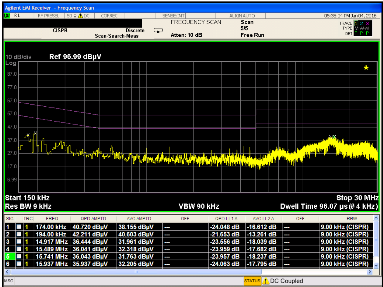
Plot 7-122. Line Conducted Plot with 802.11a UNII Band 3 (L1)
