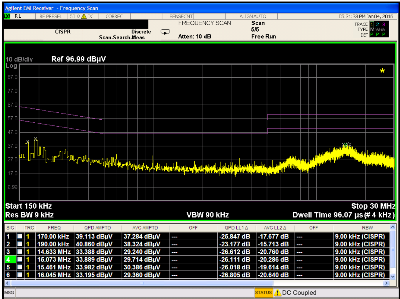
Plot 7-119. Line Conducted Plot with 802.11a UNII Band 2A (N)
