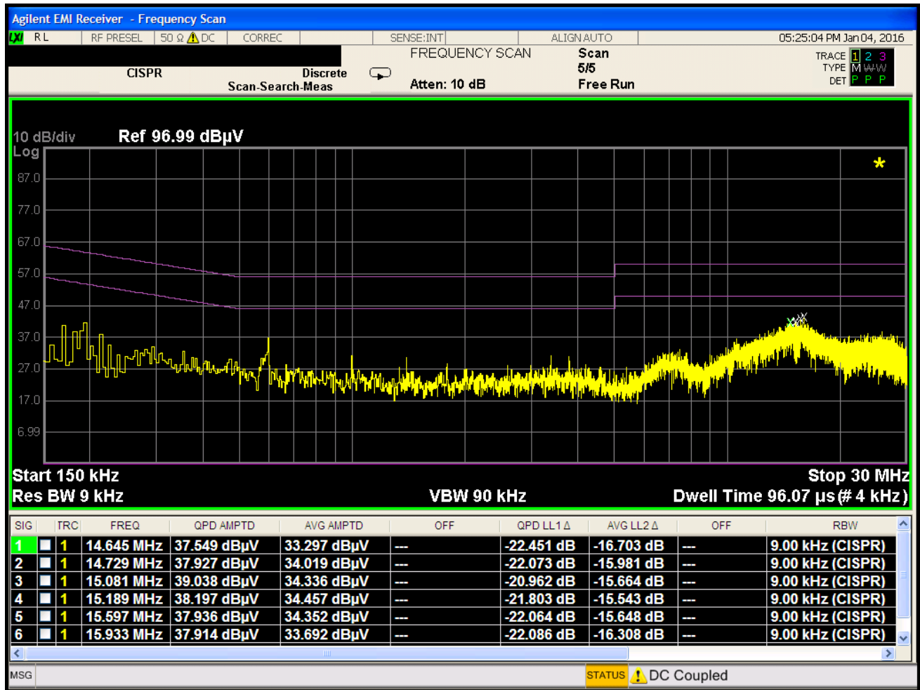
Plot 7-120. Line Conducted Plot with 802.11a UNII Band 2C (L1)
