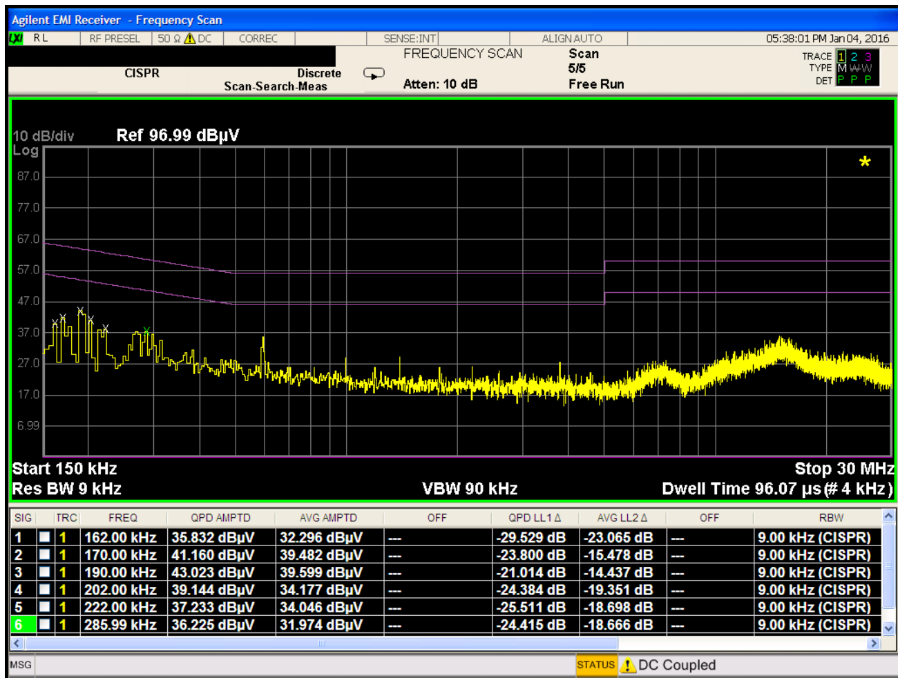
Plot 7-123. Line Conducted Plot with 802.11a UNII Band 3 (N)
