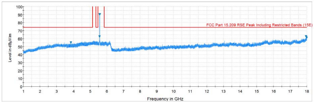
Plot 7-81. Radiated Spurious Plot above 1GHz (802.11a – U2C Ch. 116, Ant. Pol. H)
