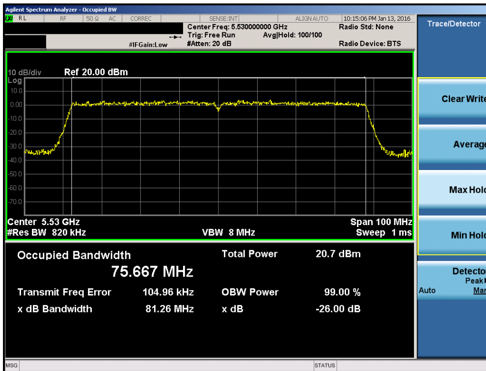
Plot 7-57. 26dB Bandwidth Plot (80MHz BW 802.11ac (UNII Band 2C) – Ch. 106)
