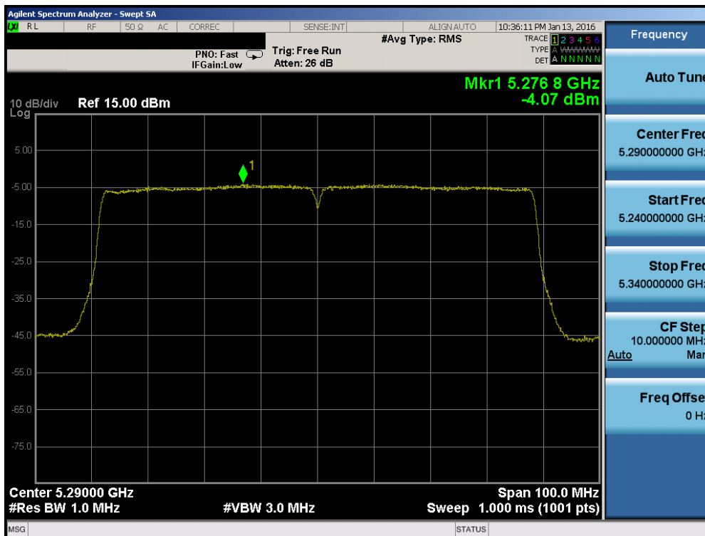
Plot 7-94. Power Spectral Density Plot (80MHz BW 802.11ac (UNII Band 2A) – Ch. 58)
