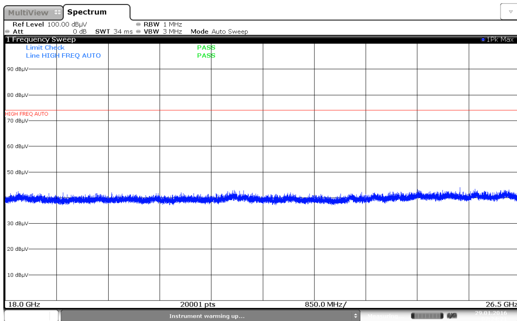
Plot 7-73. Radiated Spurious Plot above 18GHz (Pol. H)
