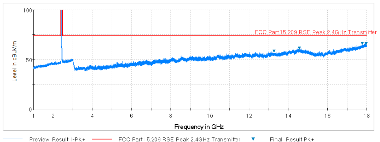
Plot 7-68. Radiated Spurious Plot above 1GHz (802.11b – Ch. 1, Ant. Pol. V)
