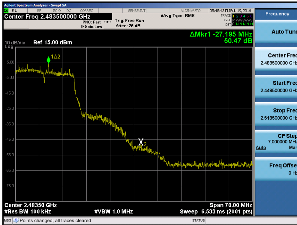
Plot 7-47. Band Edge Plot (802.11n (2.4GHz) – Ch. 10)
