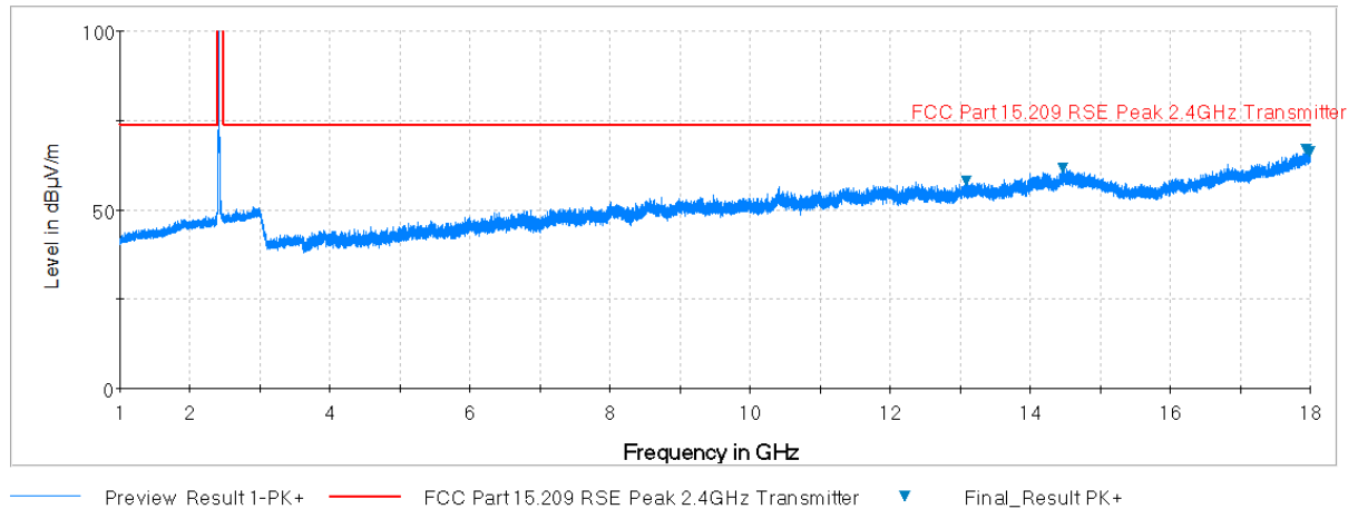
Plot 7-67. Radiated Spurious Plot above 1GHz (802.11b – Ch. 1, Ant. Pol. H)
