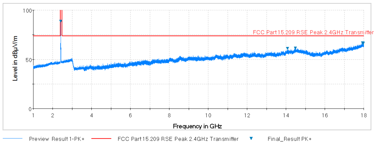
Plot 7-76. Radiated Spurious Plot above 1GHz (802.11b – Ch. 1, Ant. Pol. V)
