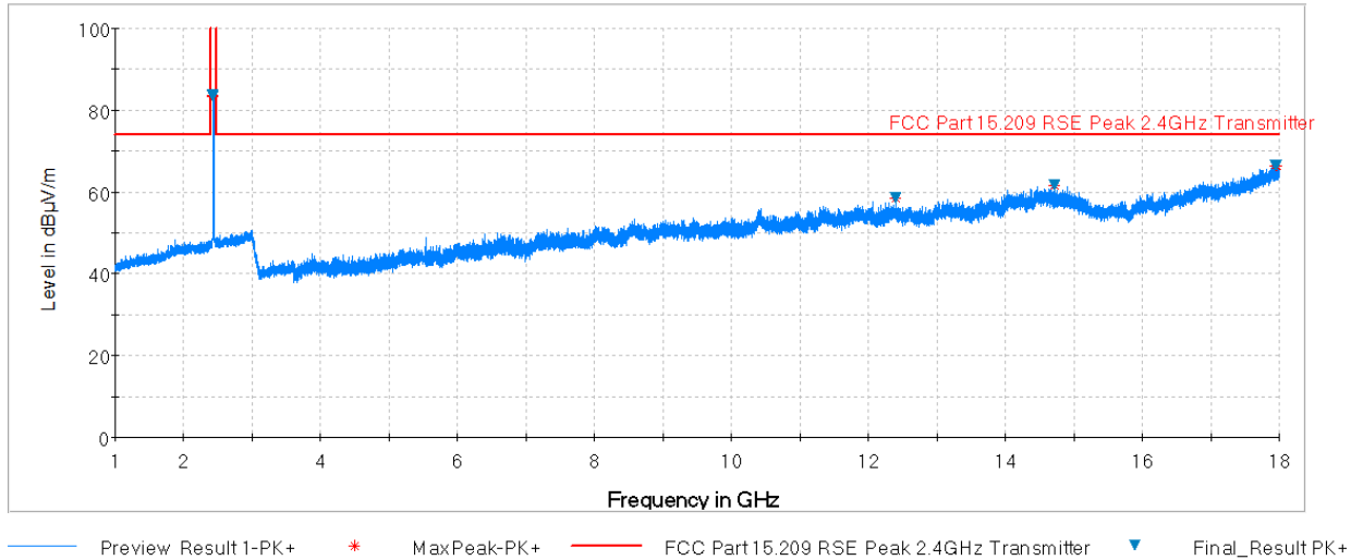
Plot 7-77. Radiated Spurious Plot above 1GHz (802.11b – Ch. 6, Ant. Pol. H)
