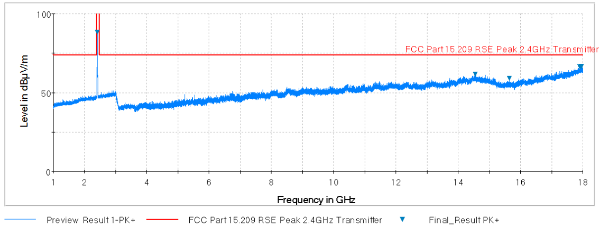
Plot 7-75. Radiated Spurious Plot above 1GHz (802.11b – Ch. 1, Ant. Pol. H)
