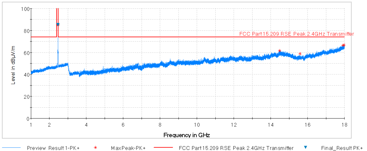
Plot 7-80. Radiated Spurious Plot above 1GHz (802.11b – Ch. 11, Ant. Pol. V)
