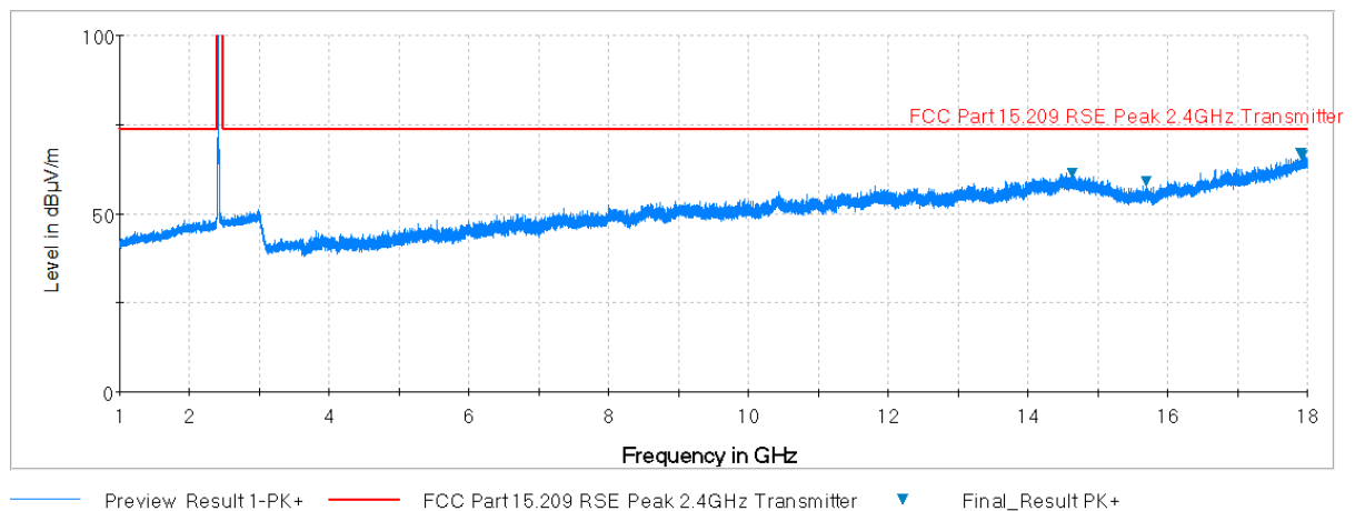
Plot 7-68. Radiated Spurious Plot above 1GHz (802.11b – Ch. 1, Ant. Pol. V)
