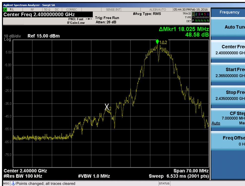
Plot 7-38. Band Edge Plot (802.11b – Ch. 2)
