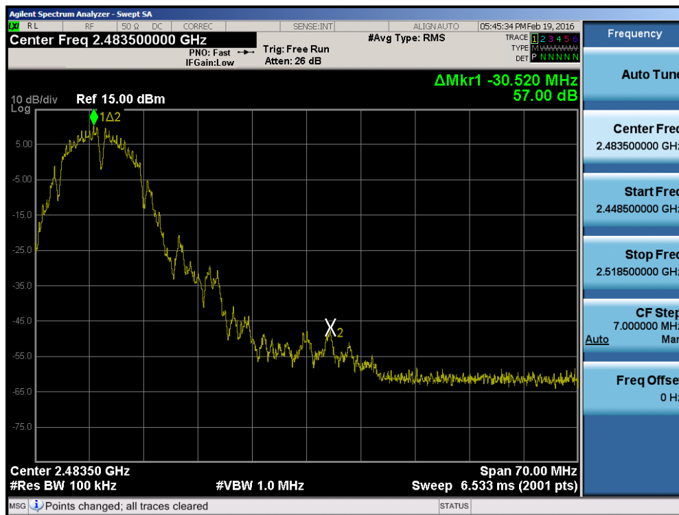
Plot 7-39. Band Edge Plot (802.11b – Ch. 10)
