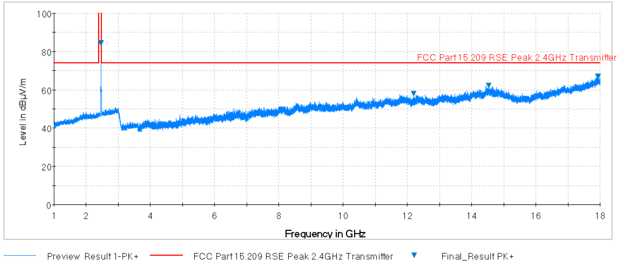
Plot 7-79. Radiated Spurious Plot above 1GHz (802.11b – Ch. 11, Ant. Pol. H)
