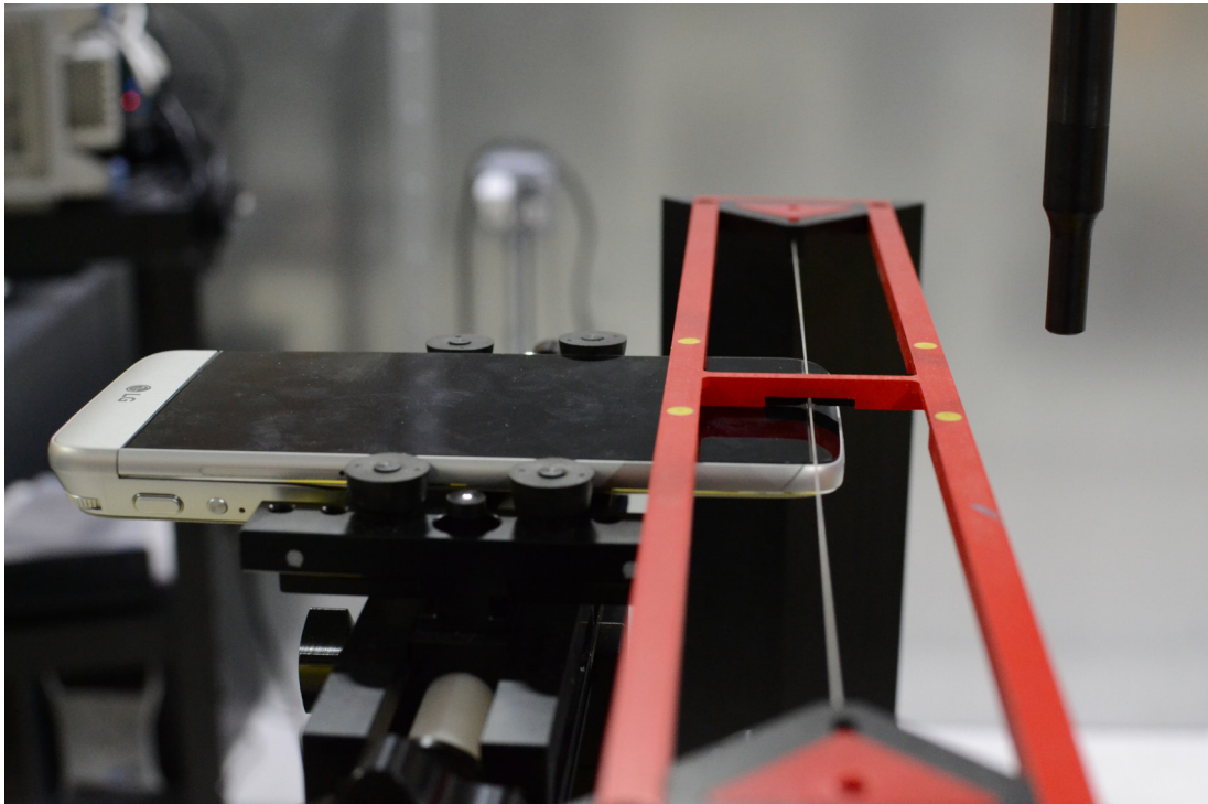
Figure 18-4 HAC Phantom Plane Alignment – Camera Module accessory
