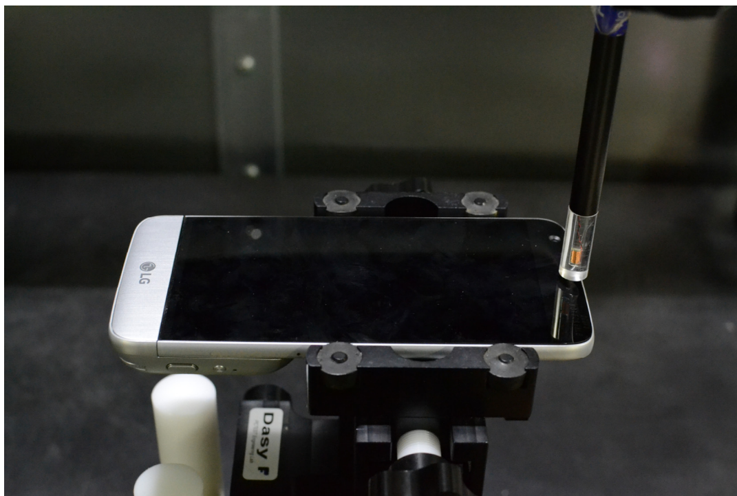
Figure 14-3 Test Setup for Wireless Device – Camera Module Accessory
