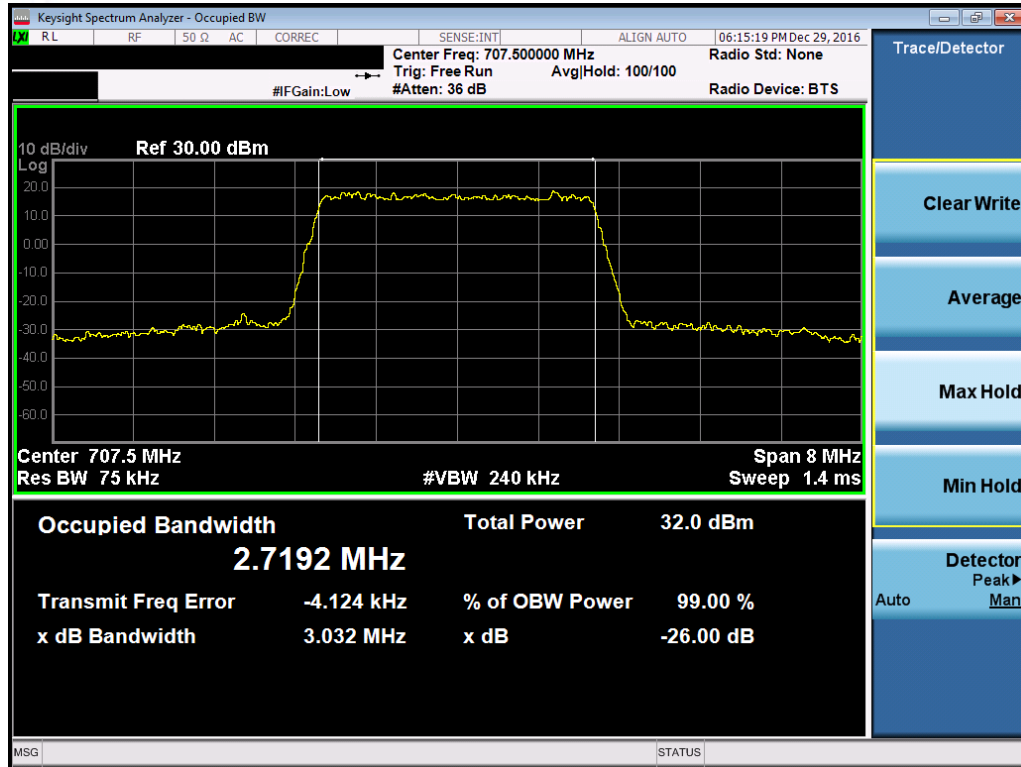
Plot 7-5. Occupied Bandwidth Plot (Band 12/17 - 3.0MHz 16-QAM - RB Size 15)
