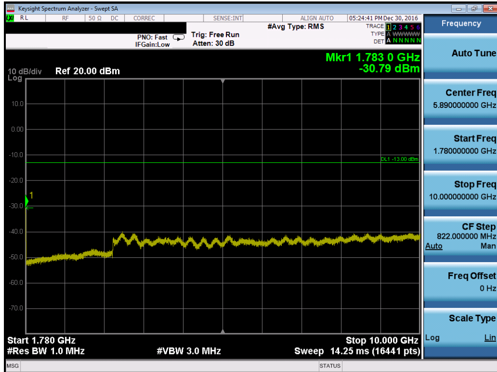
Plot 7-110. Conducted Spurious Plot (Band 4/66 – 20.0MHz QPSK – RB Size 1, RB Offset 0 – Mid Channel)
