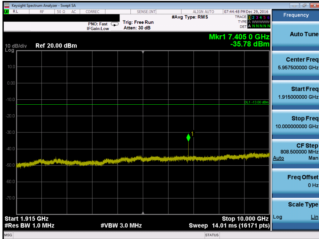
Plot 7-116. Conducted Spurious Plot (Band 2/25 – 20.0MHz QPSK – RB Size 1, RB Offset 0 – Low Channel)
