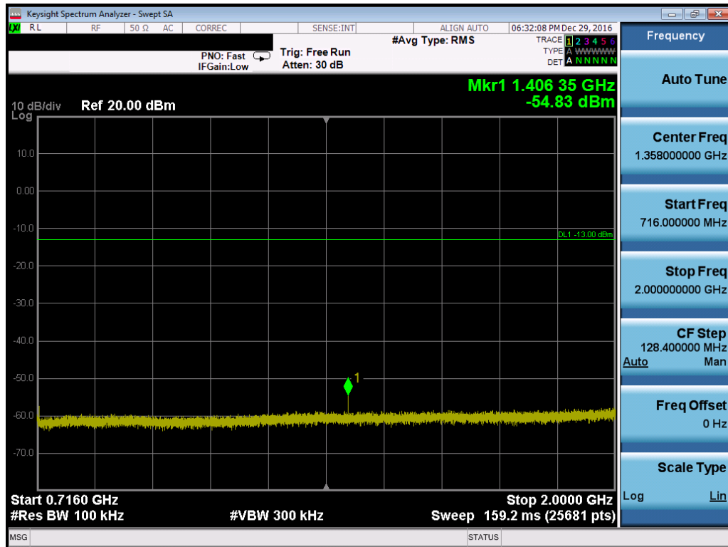
Plot 7-89. Conducted Spurious Plot (Band 12/17 – 10.0MHz QPSK – RB Size 1, RB Offset 0 – Mid Channel)
