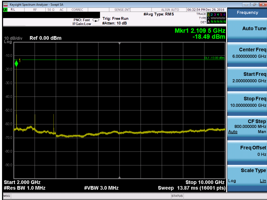
Plot 7-90. Conducted Spurious Plot (Band 12/17 – 10.0MHz QPSK – RB Size 1, RB Offset 0 – Mid Channel)
