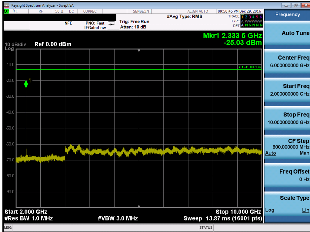
Plot 7-96. Conducted Spurious Plot (Band 13 – 10.0MHz QPSK – RB Size 1, RB Offset 0)
