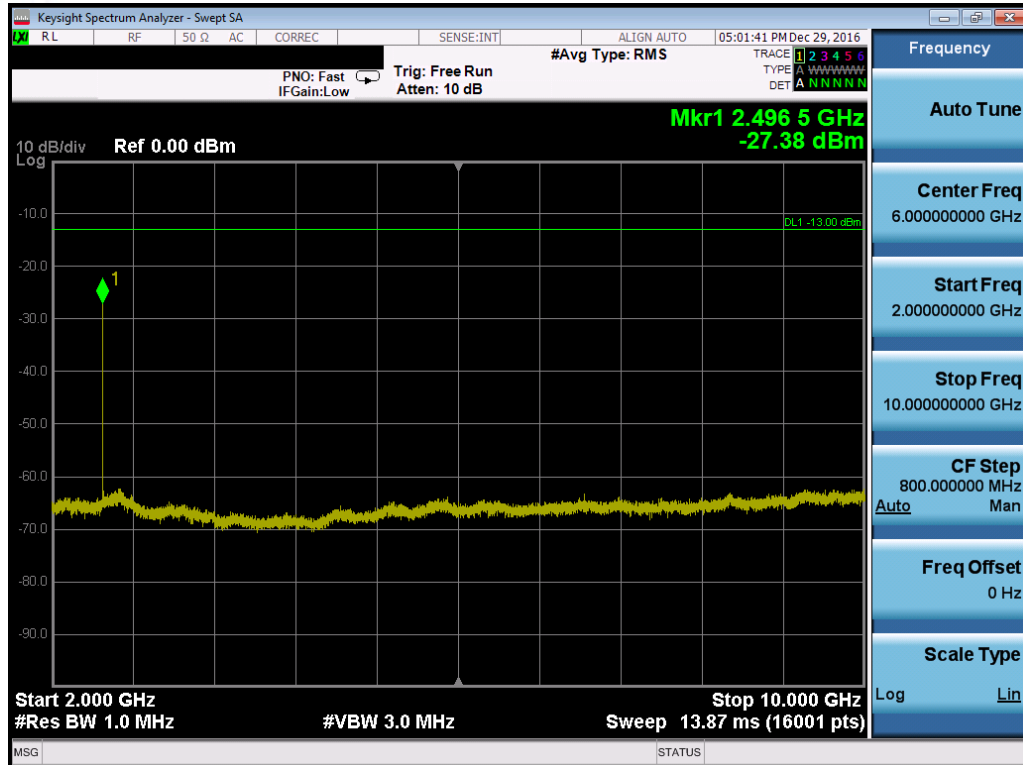
Plot 7-102. Conducted Spurious Plot (Band 5 – 10.0MHz QPSK – RB Size 1, RB Offset 0 – Mid Channel)
