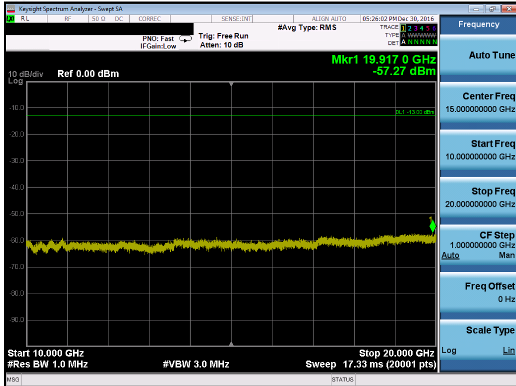
Plot 7-108. Conducted Spurious Plot (Band 4/66 – 20.0MHz QPSK – RB Size 1, RB Offset 0 – Low Channel)
