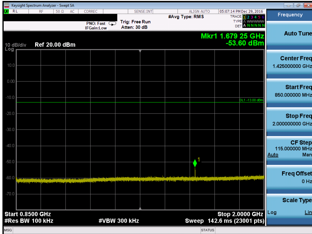
Plot 7-104. Conducted Spurious Plot (Band 5 – 10.0MHz QPSK – RB Size 1, RB Offset 0 – High Channel)
