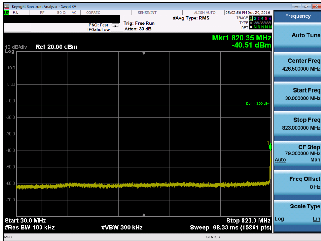
Plot 7-97. Conducted Spurious Plot (Band 5 – 10.0MHz QPSK – RB Size 1, RB Offset 0– Low Channel)
