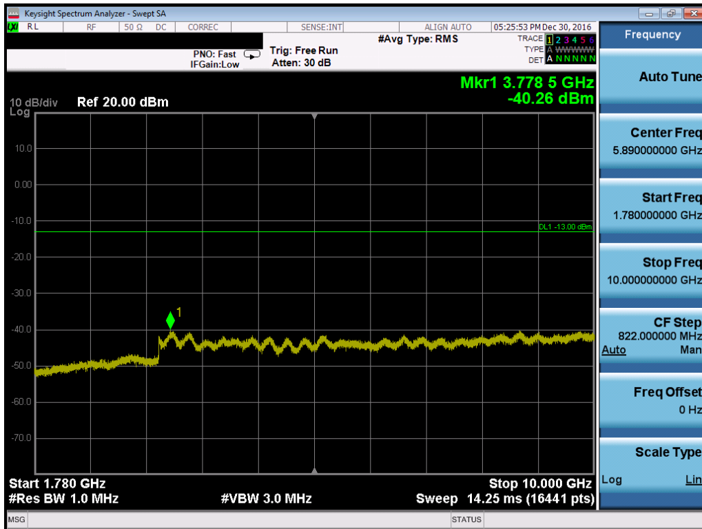
Plot 7-107. Conducted Spurious Plot (Band 4/66 – 20.0MHz QPSK – RB Size 1, RB Offset 0 – Low Channel)
