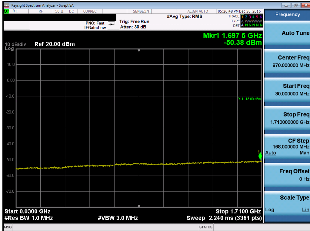
Plot 7-112. Conducted Spurious Plot (Band 4/66 – 20.0MHz QPSK – RB Size 1, RB Offset 0 – High Channel)
