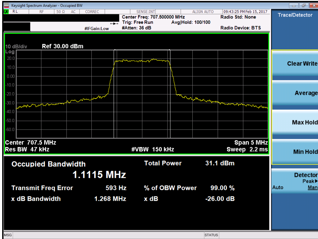
Plot 7-3. Occupied Bandwidth Plot (Band 12/17 – 1.4MHz 64-QAM – RB Size 6)
