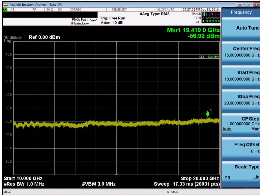
Plot 7-114. Conducted Spurious Plot (Band 4/66 – 20.0MHz QPSK – RB Size 1, RB Offset 0 – High Channel)
