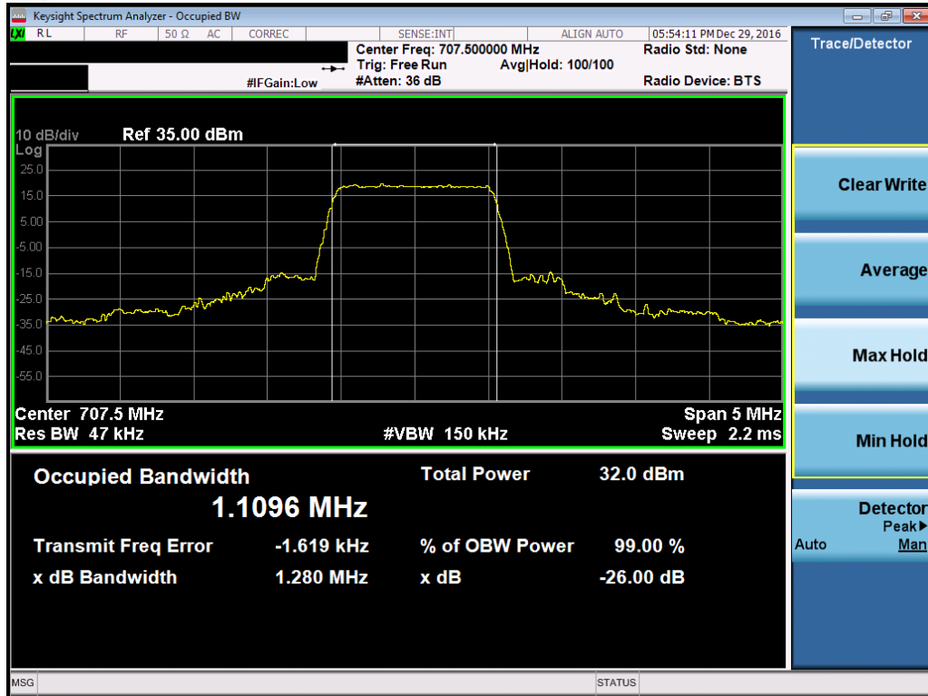
Plot 7-1. Occupied Bandwidth Plot (Band 12/17 – 1.4MHz QPSK – RB Size 6)
