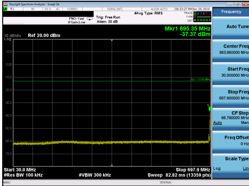
Plot 7-85. Conducted Spurious Plot (Band 12/17 – 10.0MHz QPSK – RB Size 1, RB Offset 0– Low Channel)
