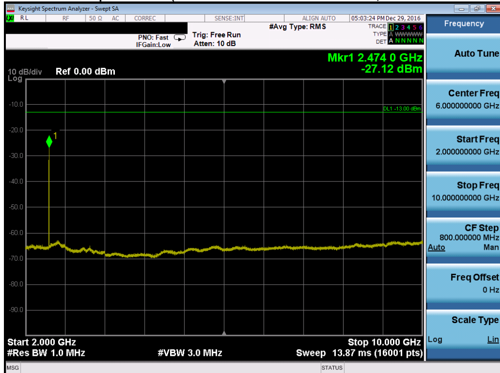
Plot 7-99. Conducted Spurious Plot (Band 5 – 10.0MHz QPSK – RB Size 1, RB Offset 0 – Low Channel)
