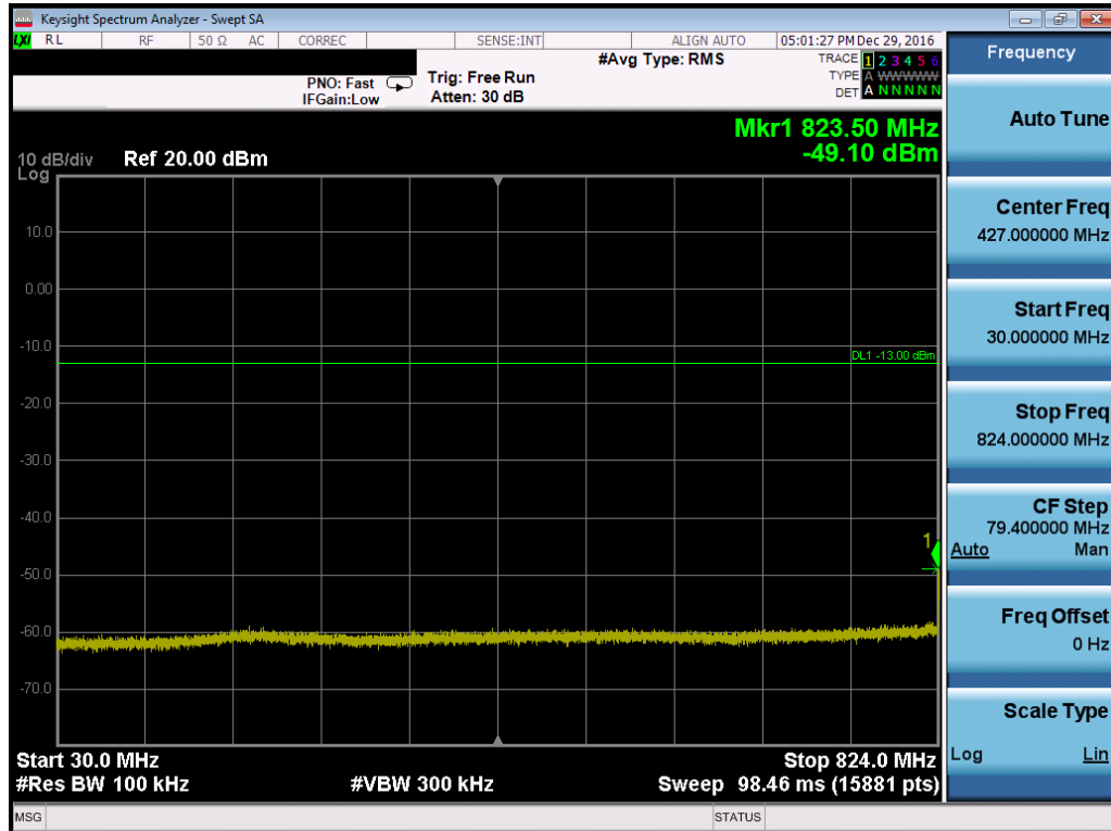
Plot 7-100. Conducted Spurious Plot (Band 5 – 10.0MHz QPSK – RB Size 1, RB Offset 0 – Mid Channel)
