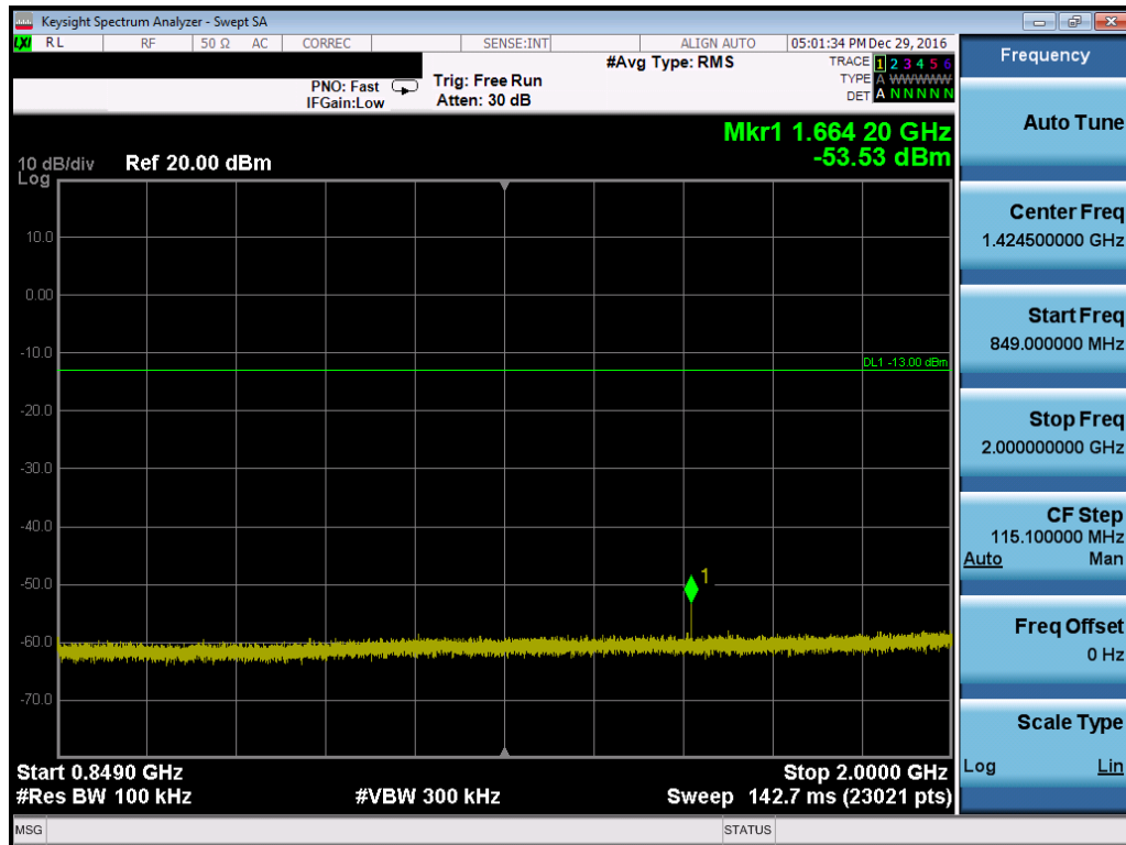
Plot 7-101. Conducted Spurious Plot (Band 5 – 10.0MHz QPSK – RB Size 1, RB Offset 0 – Mid Channel)
