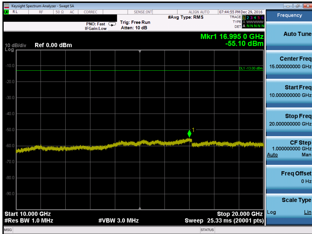
Plot 7-117. Conducted Spurious Plot (Band 2/25 – 20.0MHz QPSK – RB Size 1, RB Offset 0 – Low Channel)
