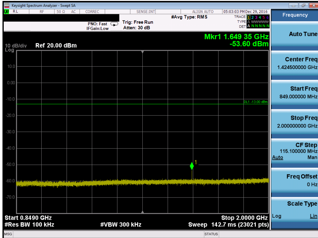
Plot 7-98. Conducted Spurious Plot (Band 5 – 10.0MHz QPSK – RB Size 1, RB Offset 0 – Low Channel)
