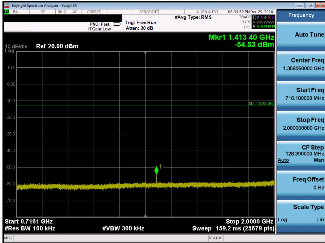
Plot 7-92. Conducted Spurious Plot (Band 12/17 – 10.0MHz QPSK – RB Size 1, RB Offset 0 – High Channel)
