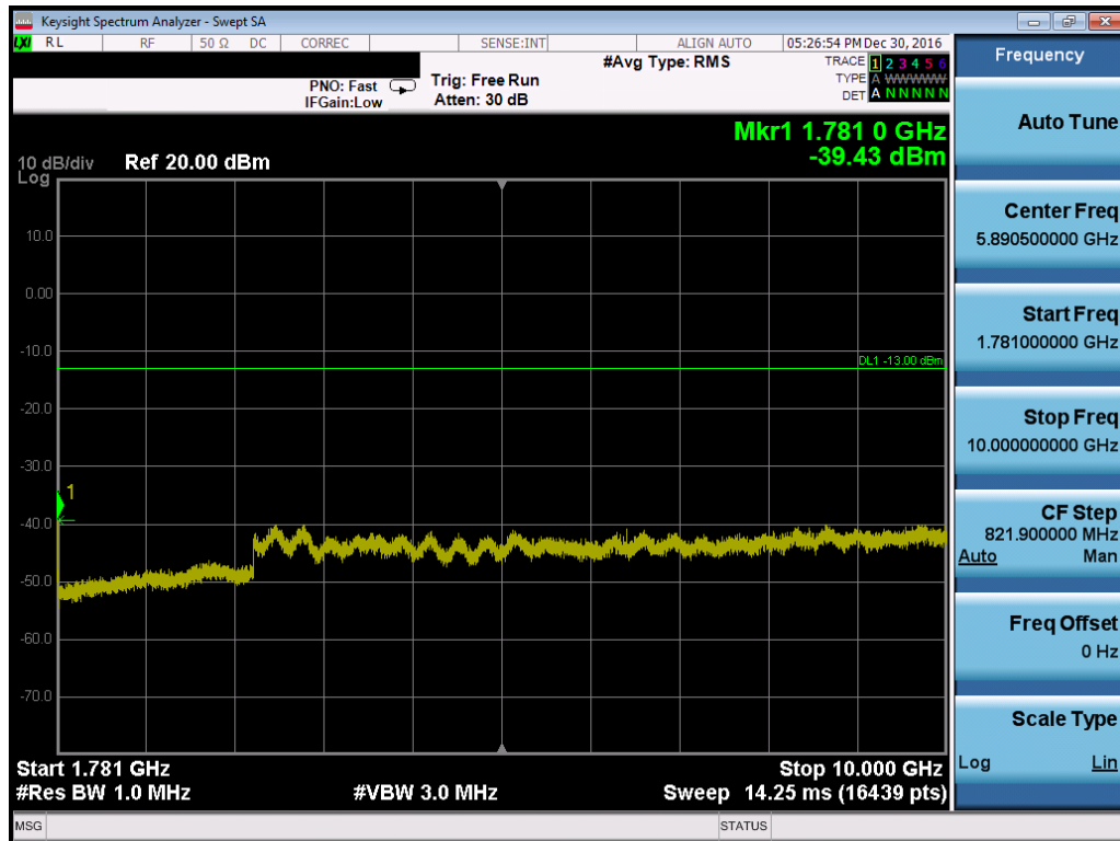
Plot 7-113. Conducted Spurious Plot (Band 4/66 – 20.0MHz QPSK – RB Size 1, RB Offset 0 – High Channel)
