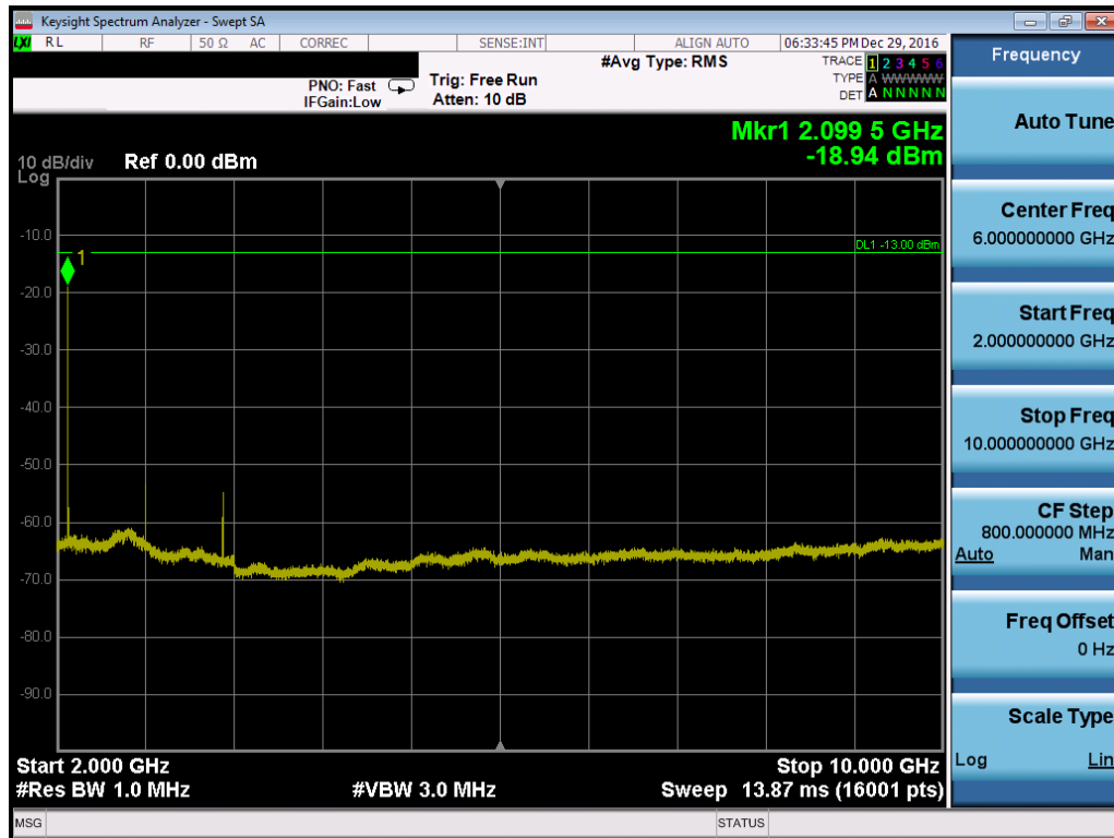
Plot 7-87. Conducted Spurious Plot (Band 12/17 – 10.0MHz QPSK – RB Size 1, RB Offset 0 – Low Channel)
