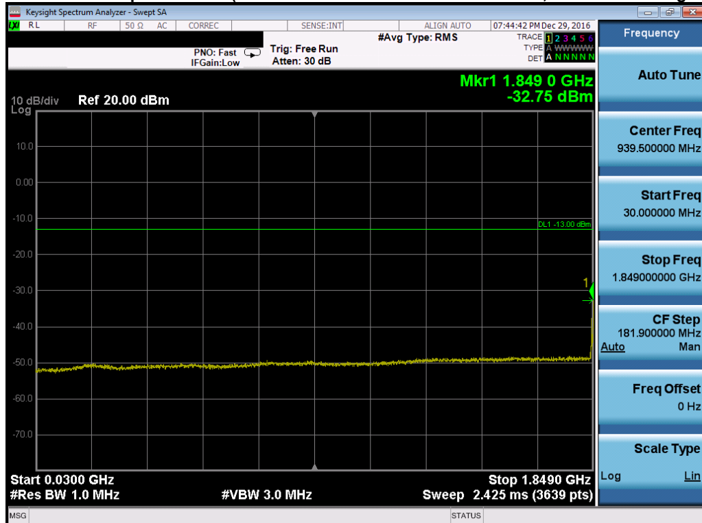
Plot 7-115. Conducted Spurious Plot (Band 2/25 – 20.0MHz QPSK – RB Size 1, RB Offset 0– Low Channel)
