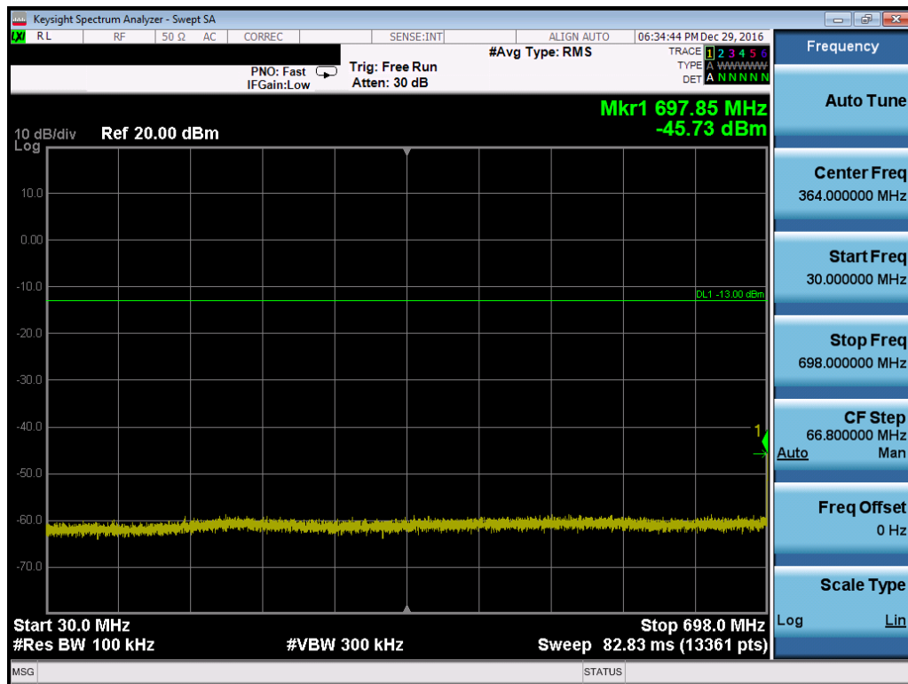
Plot 7-91. Conducted Spurious Plot (Band 12/17 – 10.0MHz QPSK – RB Size 1, RB Offset 0 – High Channel)
