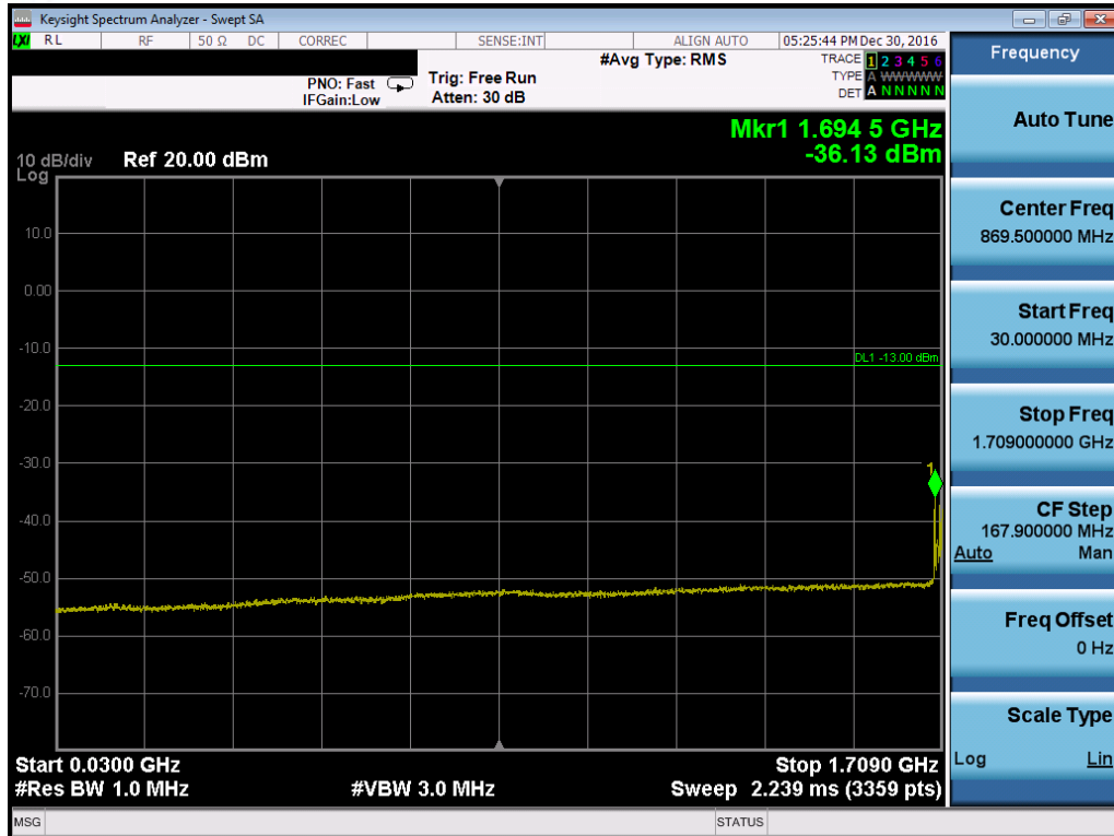
Plot 7-106. Conducted Spurious Plot (Band 4/66 – 20.0MHz QPSK – RB Size 1, RB Offset 0– Low Channel)
