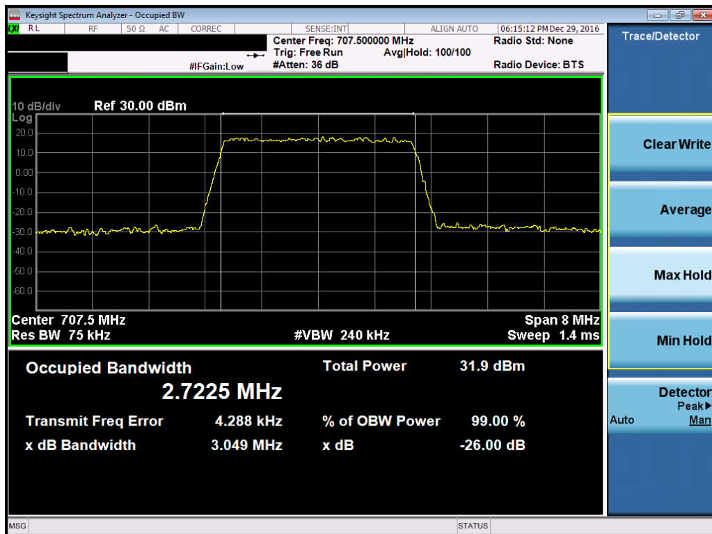
Plot 7-4. Occupied Bandwidth Plot (Band 12/17 – 3.0MHz QPSK – RB Size 15)
