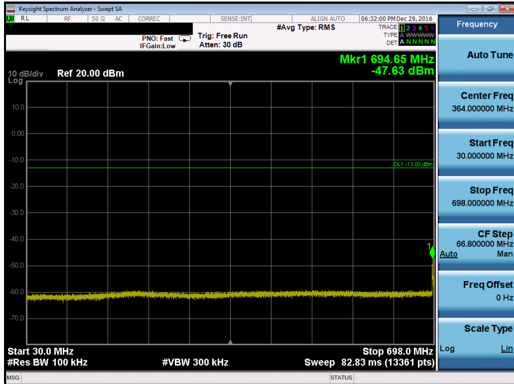
Plot 7-88. Conducted Spurious Plot (Band 12/17 – 10.0MHz QPSK – RB Size 1, RB Offset 0 – Mid Channel)
