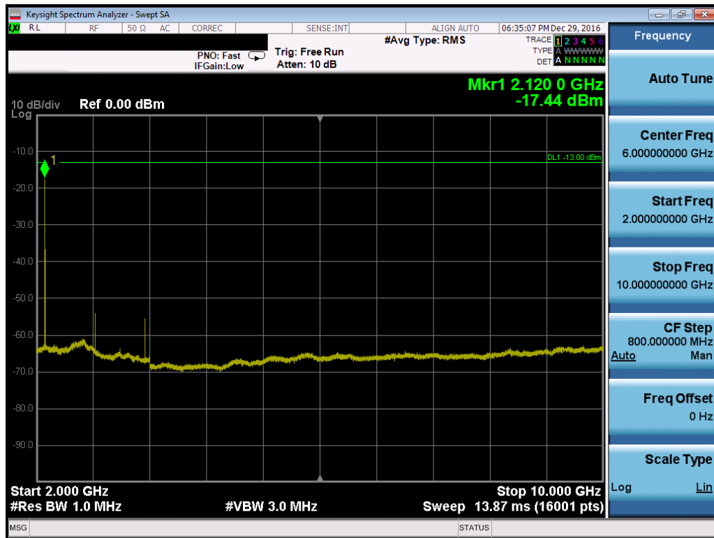
Plot 7-93. Conducted Spurious Plot (Band 12/17 – 10.0MHz QPSK – RB Size 1, RB Offset 0 – High Channel)
