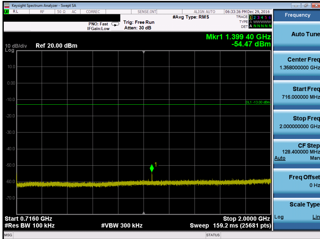
Plot 7-86. Conducted Spurious Plot (Band 12/17 – 10.0MHz QPSK – RB Size 1, RB Offset 0 – Low Channel)
