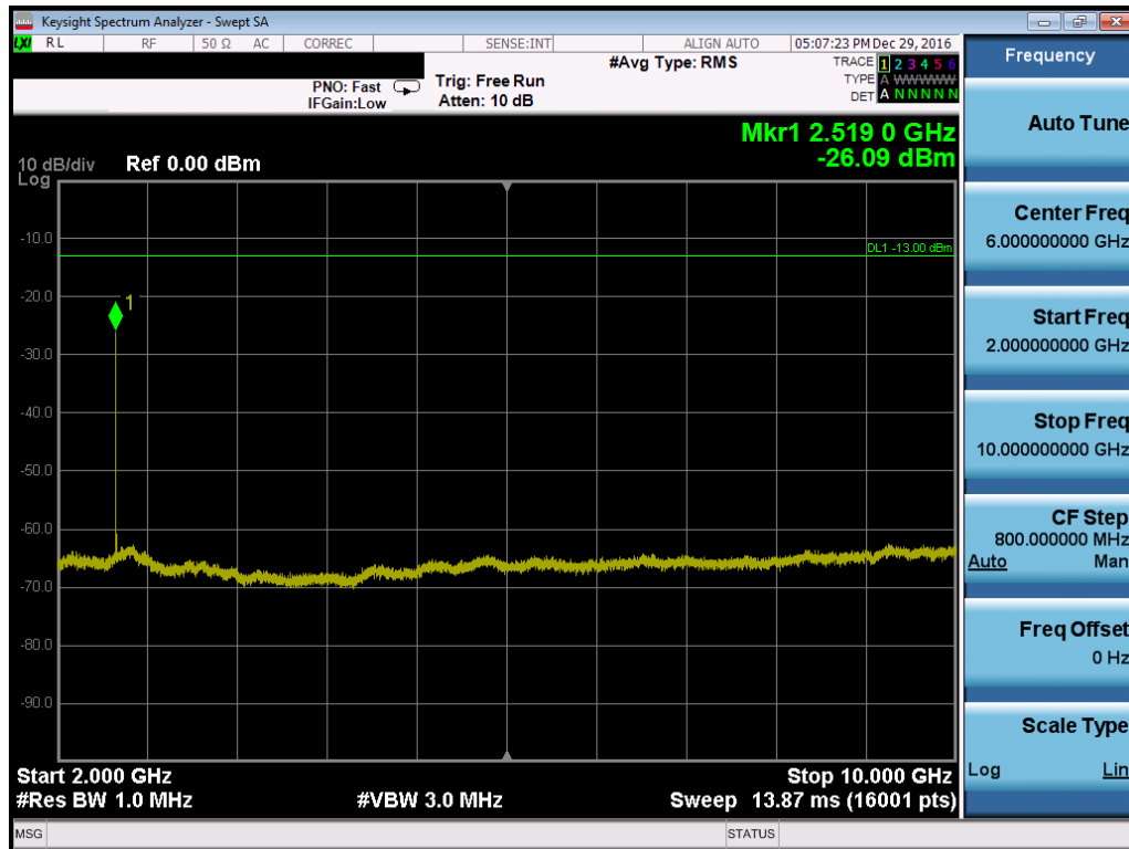
Plot 7-105. Conducted Spurious Plot (Band 5 – 10.0MHz QPSK – RB Size 1, RB Offset 0 – High Channel)
