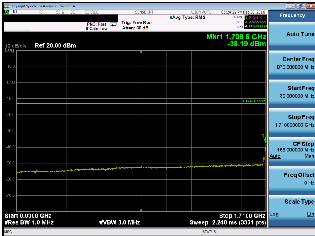
Plot 7-109. Conducted Spurious Plot (Band 4/66 – 20.0MHz QPSK – RB Size 1, RB Offset 0 – Mid Channel)
