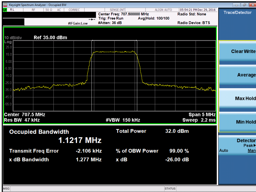
Plot 7-2. Occupied Bandwidth Plot (Band 12/17 – 1.4MHz 16-QAM – RB Size 6)
