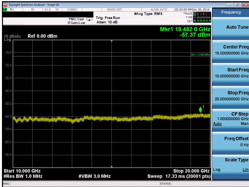
Plot 7-111. Conducted Spurious Plot (Band 4/66 – 20.0MHz QPSK – RB Size 1, RB Offset 0 – Mid Channel)
