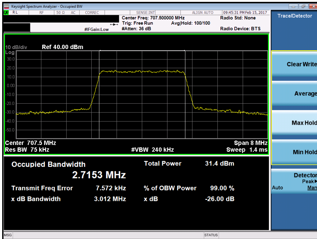
Plot 7-6. Occupied Bandwidth Plot (Band 12/17 - 3.0MHz 64-QAM - RB Size 15)
