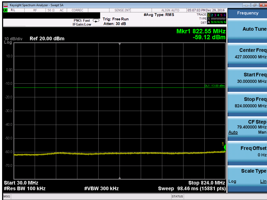
Plot 7-103. Conducted Spurious Plot (Band 5 – 10.0MHz QPSK – RB Size 1, RB Offset 0 – High Channel)
