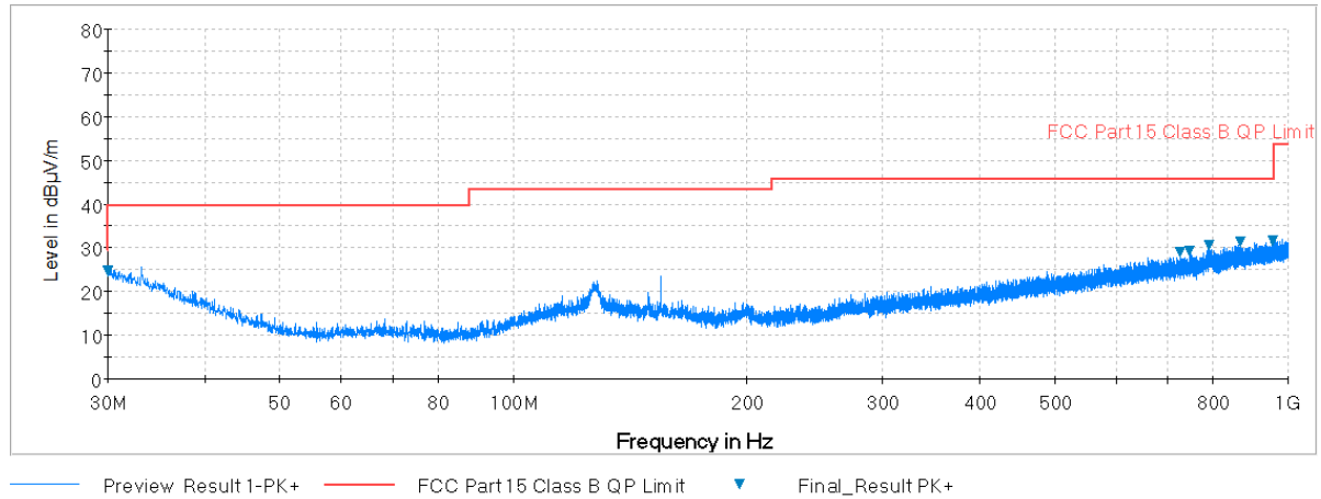
Plot 7-261. Radiated Spurious Plot below 1GHz (802.11a – U3 Ch. 157, Ant. Pol. H)
