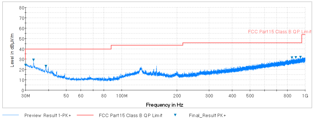
Plot 7-262. Radiated Spurious Plot below 1GHz (802.11a – U3 Ch. 157, Ant. Pol. V)
