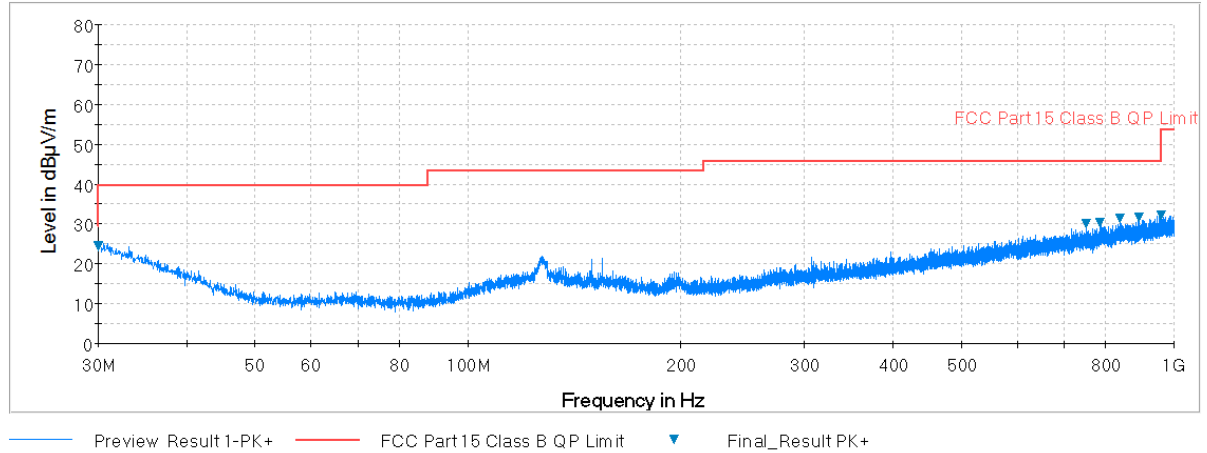
Plot 7-263. Radiated Spurious Plot below 1GHz (802.11a – U3 Ch. 157, Ant. Pol. H)
