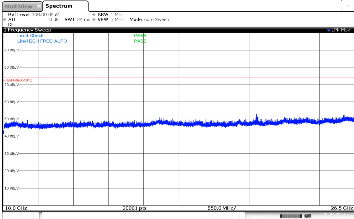
Plot 7-179. Radiated Spurious Plot above 18GHz (2.4GHz – 5GHz, Ant. Pol. H)
