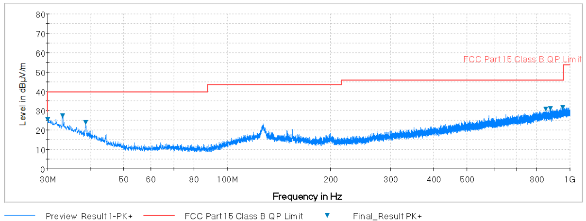
Plot 7-264. Radiated Spurious Plot below 1GHz (802.11a – U3 Ch. 157, Ant. Pol. V)
