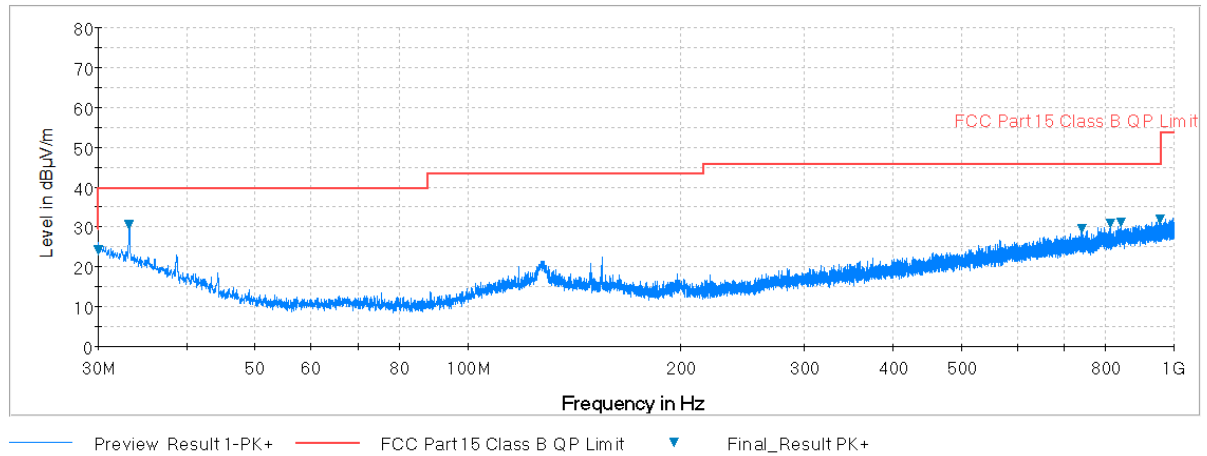
Plot 7-95. Radiated Spurious Plot below 1GHz (Pol. V)
