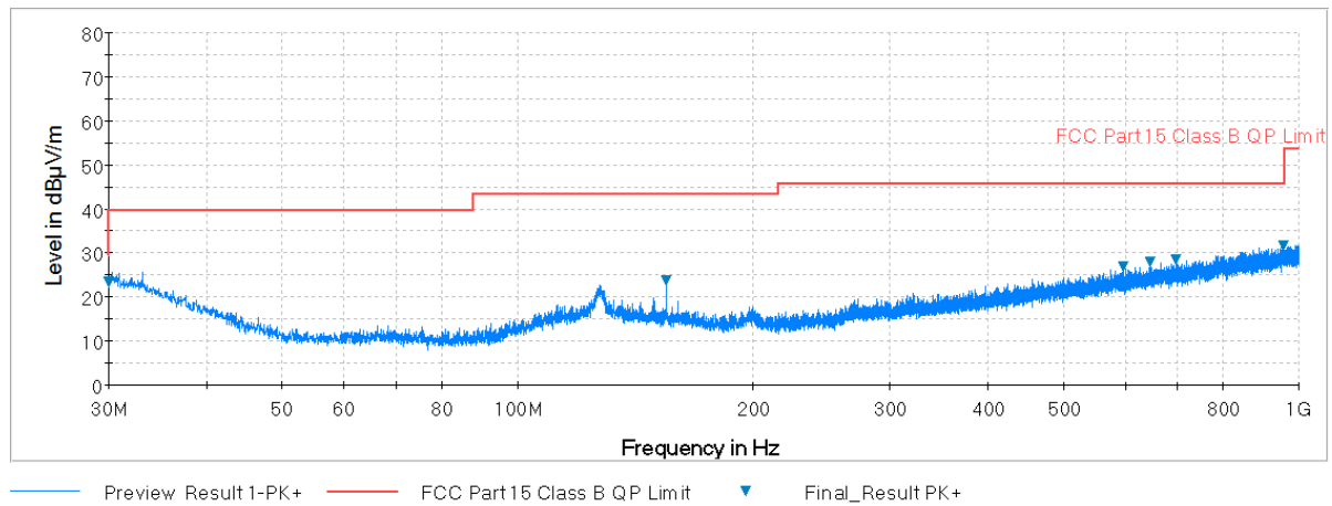
Plot 7-92. Radiated Spurious Plot below 1GHz (Pol. H)
