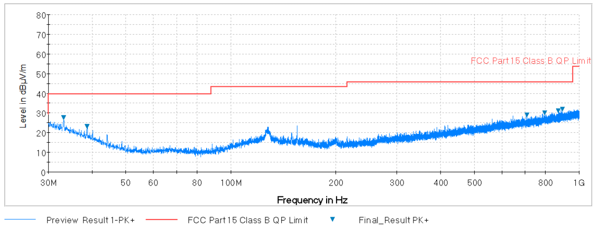
Plot 7-93. Radiated Spurious Plot below 1GHz (Pol. V)
