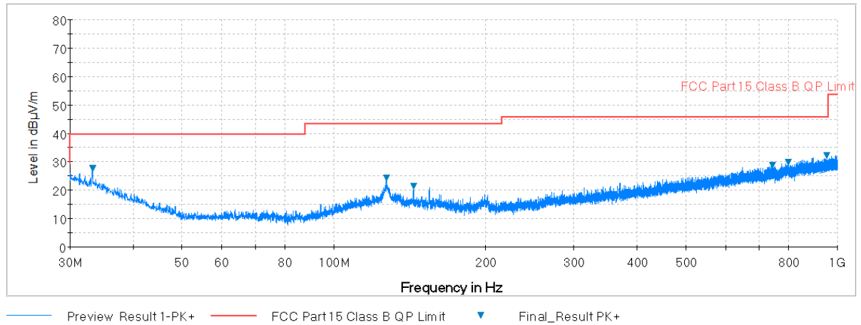
Plot 7-94. Radiated Spurious Plot below 1GHz (Pol. H)
