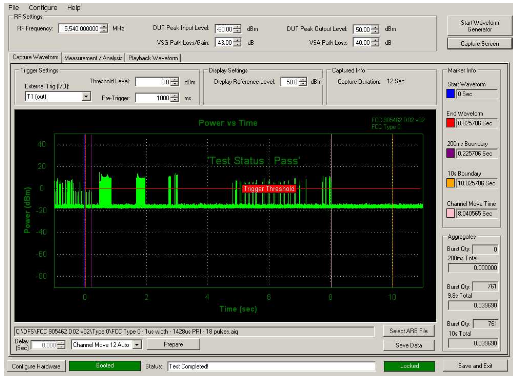
Figure 5-5. Band 2C Move Time and Aggregate Time
