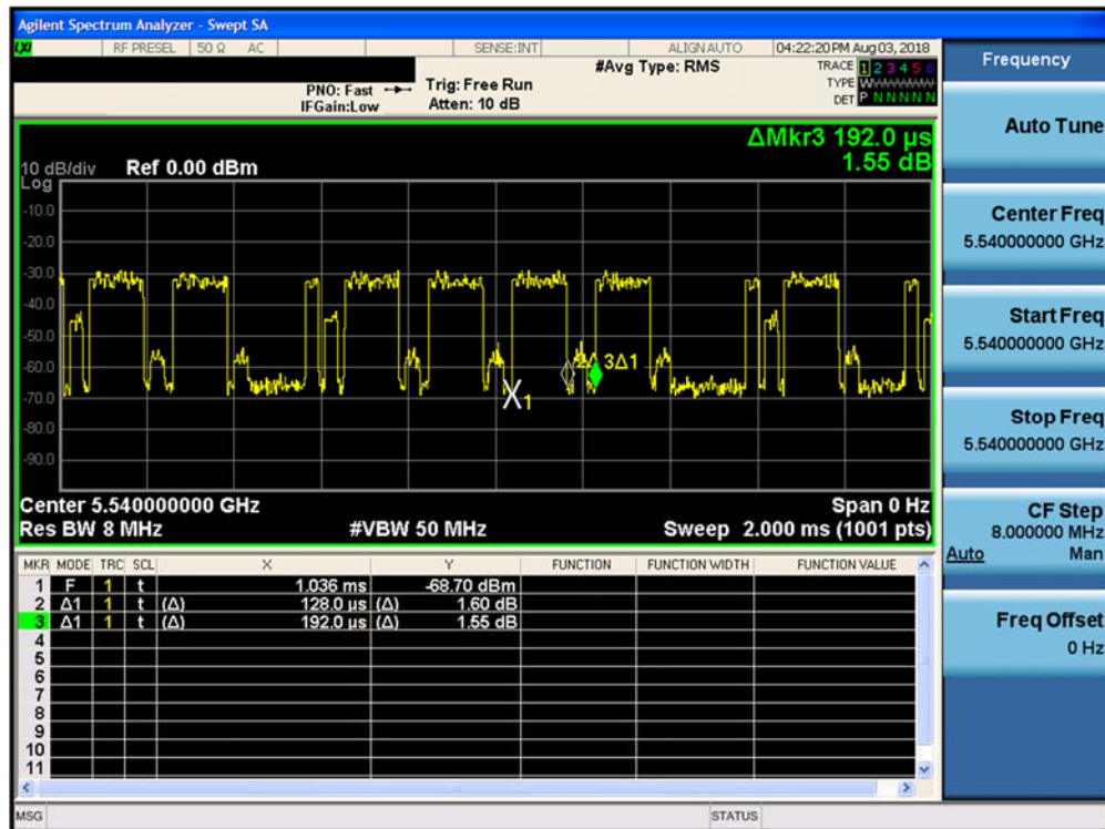
Figure 5-3. Channel Loading Plot
