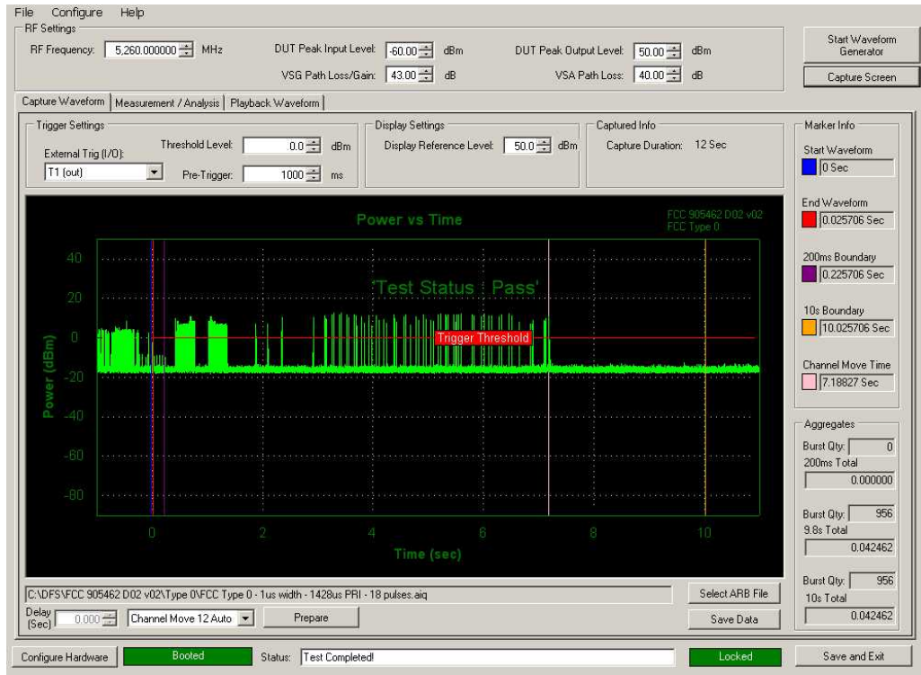
Figure 5-4. Band 2A Move Time and Aggregate Time
