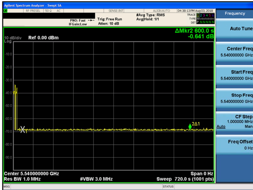
Figure 5-7. Band 2C Client Beacon Test – Monitoring live spectrum – Elapse time 10 minutes
