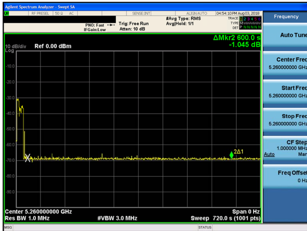
Figure 5-6. Band 2A Client Beacon Test – Monitoring live spectrum – Elapse time 10 minutes
