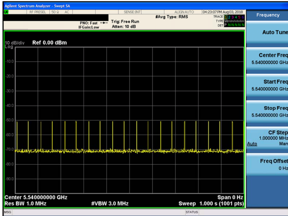
Figure 5-1. No Traffic Plot
