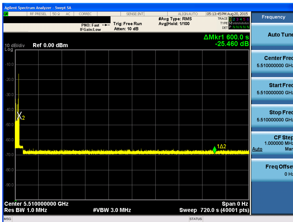
Figure 5-8. Band 2C Non-occupancy Period - Monitoring live spectrum - Elapse time 10 minutes
