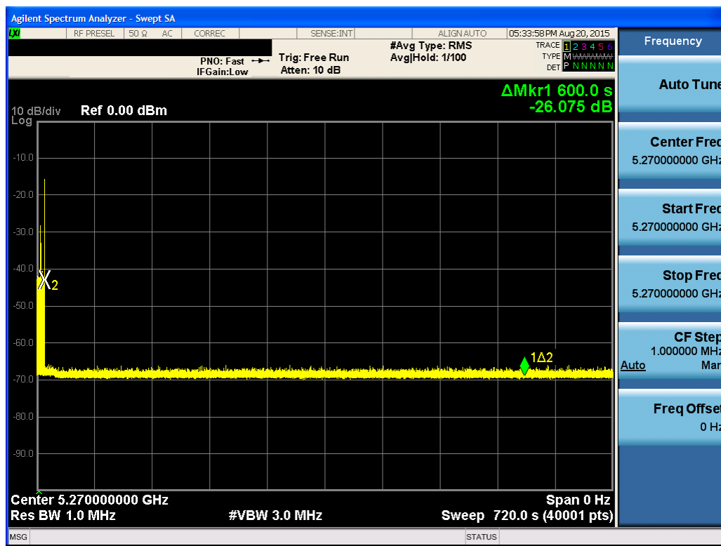
Figure 5-7. Band 2A Non-occupancy Period - Monitoring live spectrum - Elapse time 10 minutes
