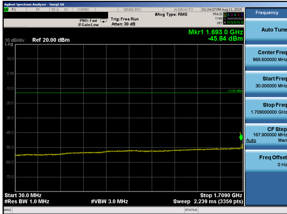
Plot 6-63. Conducted Spurious Plot (Band 4 – 20.0MHz QPSK – RB Size 1, RB Offset 0– Low Channel)
