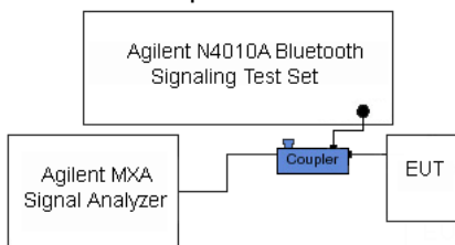
Figure 6-2. Test Instrument & Measurement Setup
