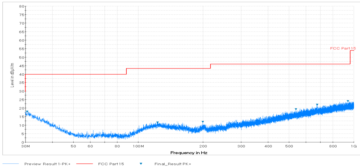
Plot 6-56. Radiated Spurious Plot below 1GHz (Pol. V)
