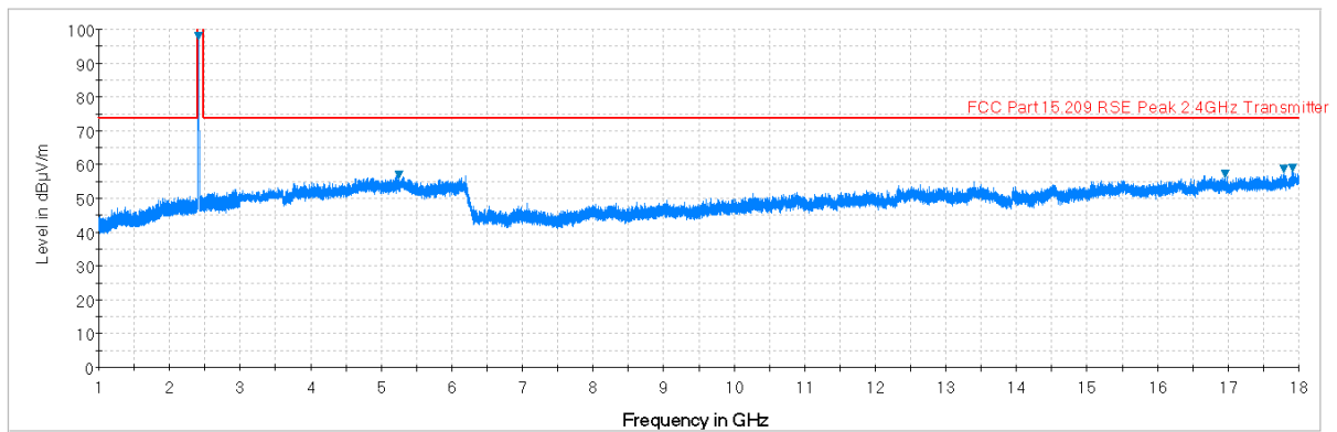
Plot 6-38. Radiated Spurious Plot above 1GHz (802.11b – Ch. 1, Ant. Pol. V)
