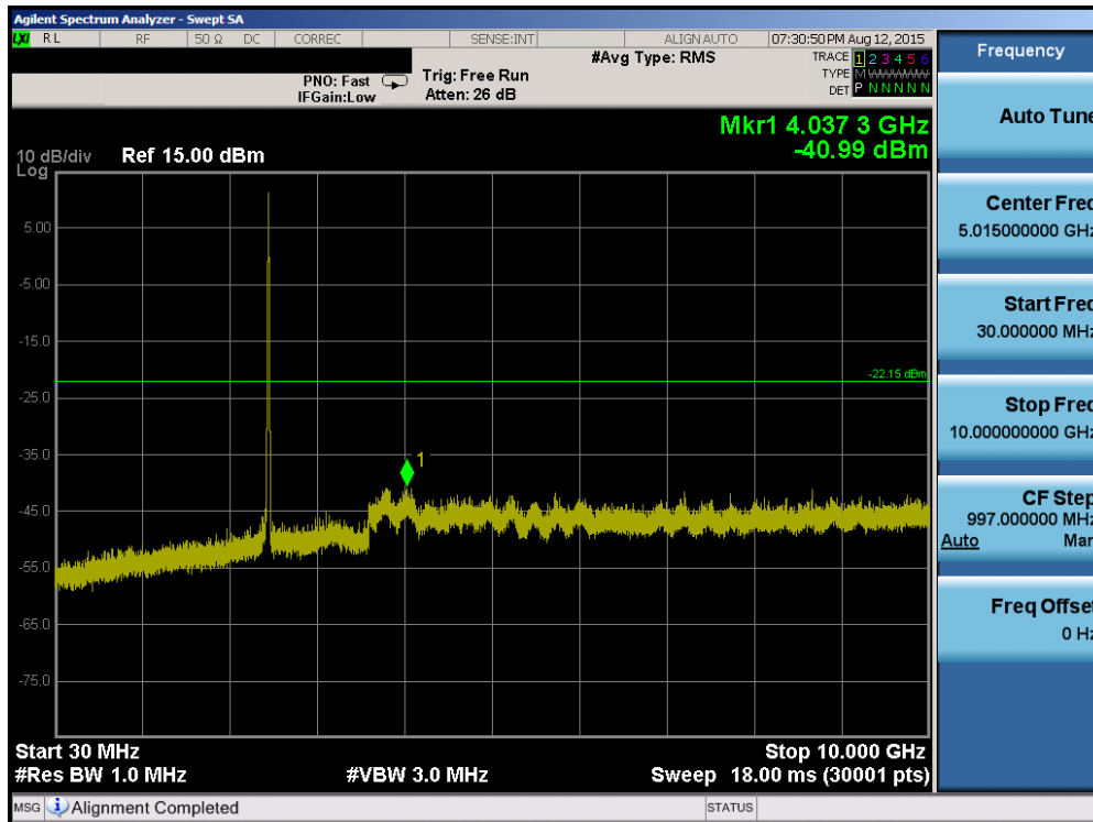
Plot 6-35. Conducted Spurious Plot (802.11b – Ch. 11)
