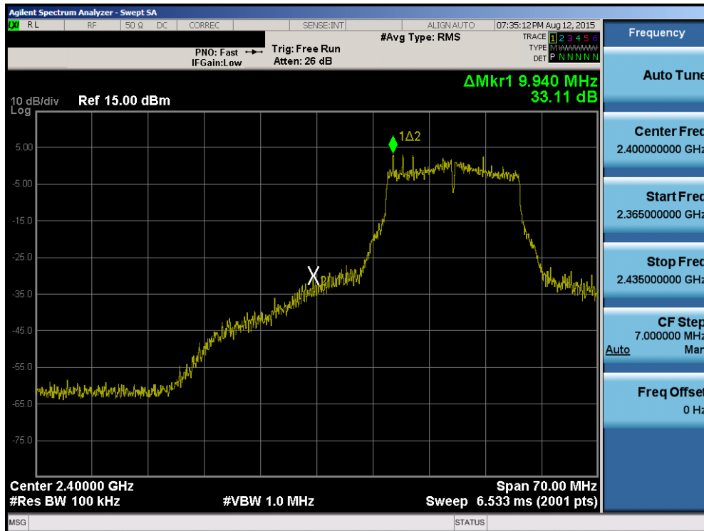
6-24. Band Edge Plot (802.11g - Ch. 2)
