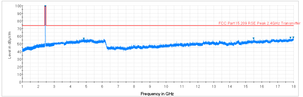
Plot 6-40. Radiated Spurious Plot above 1GHz (802.11b – Ch. 6, Ant. Pol. V)
