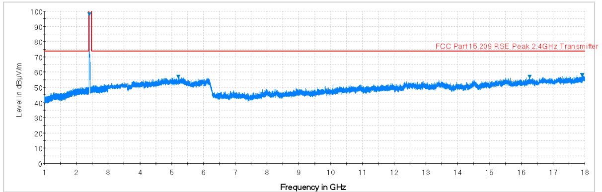
Plot 6-37. Radiated Spurious Plot above 1GHz (802.11b – Ch. 1, Ant. Pol. H)
