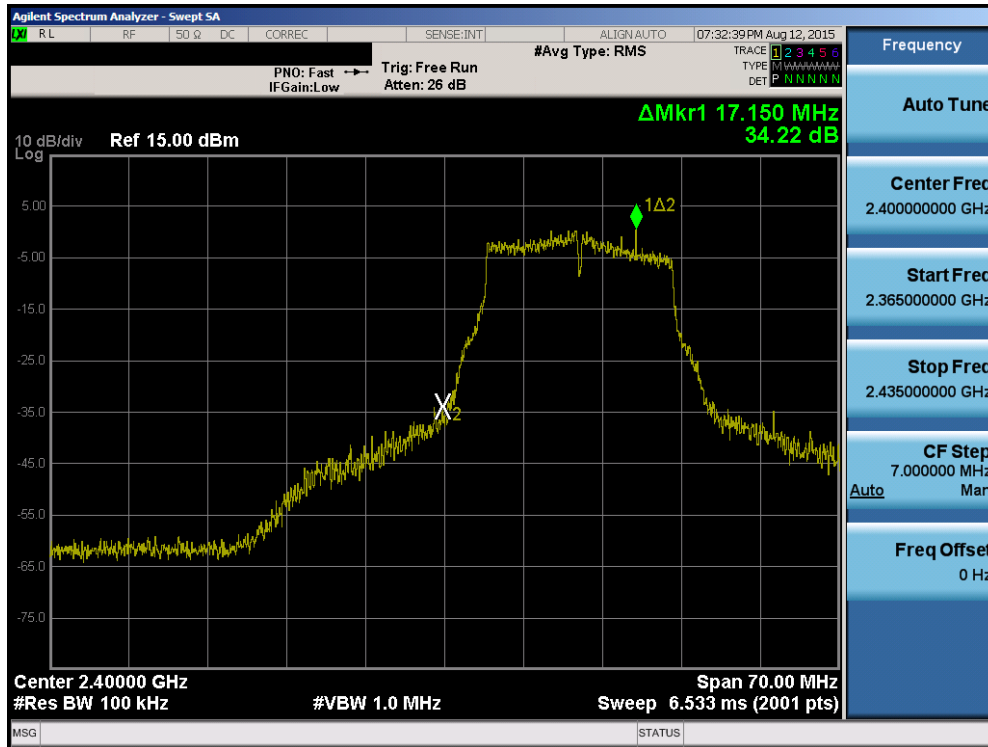
Plot 6-23. Band Edge Plot (802.11g– Ch. 1)
