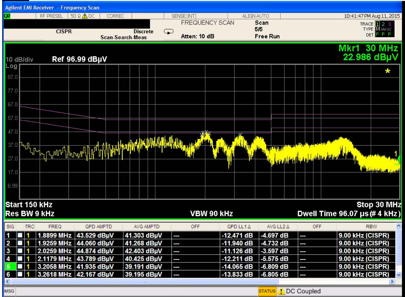
Plot 6-57. Line Conducted Plot with 802.11b (L1)
