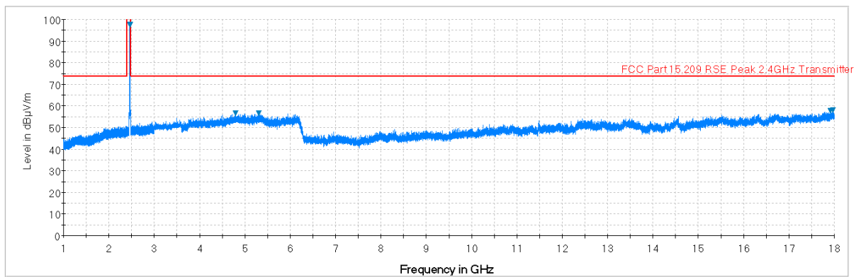
Plot 6-41. Radiated Spurious Plot above 1GHz (802.11b – Ch. 11, Ant. Pol. H)
