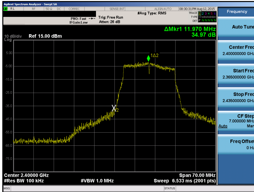
Plot 6-27. Band Edge Plot (802.11n (2.4GHz) – Ch. 1)
