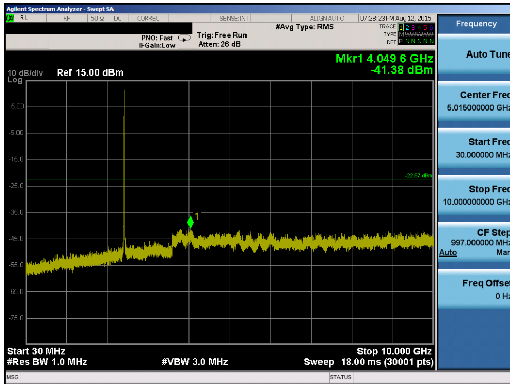
Plot 6-33. Conducted Spurious Plot (802.11b – Ch. 6)
