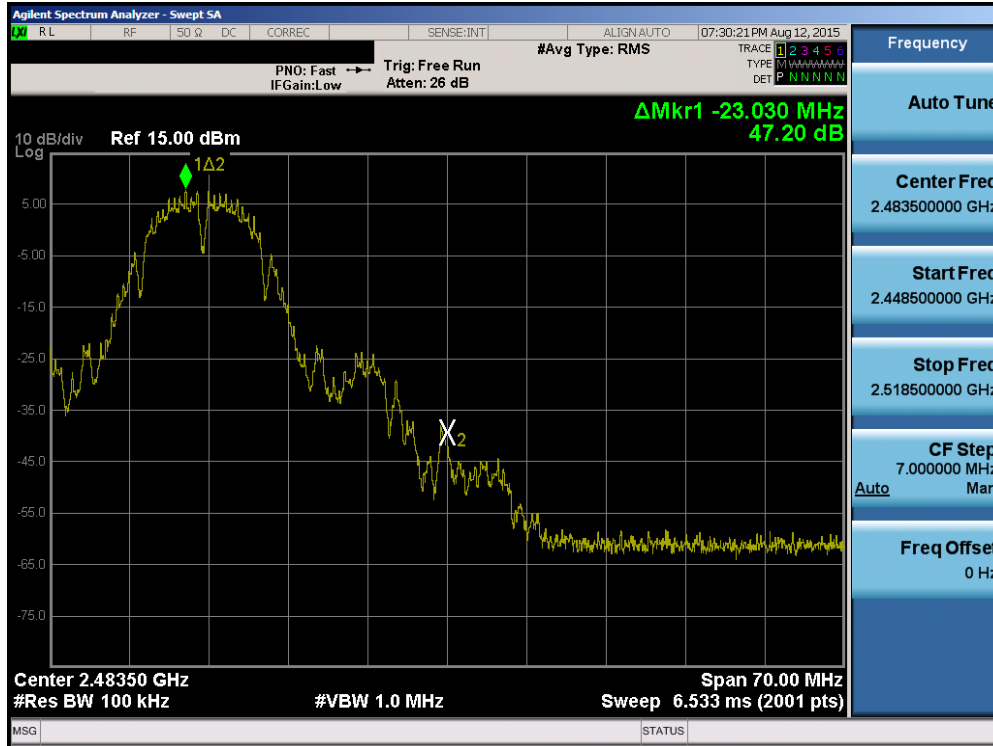
Plot 6-21. Band Edge Plot (802.11b – Ch. 11)
