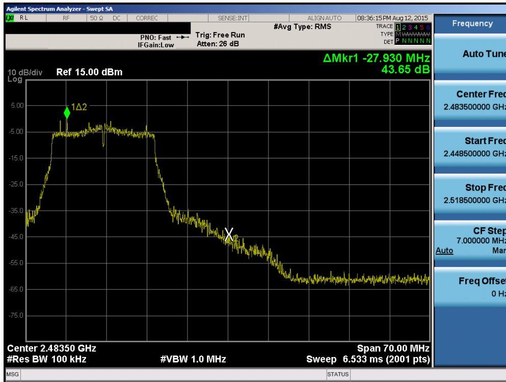
Plot 6-29. Band Edge Plot (802.11n (2.4GHz) – Ch. 11)
