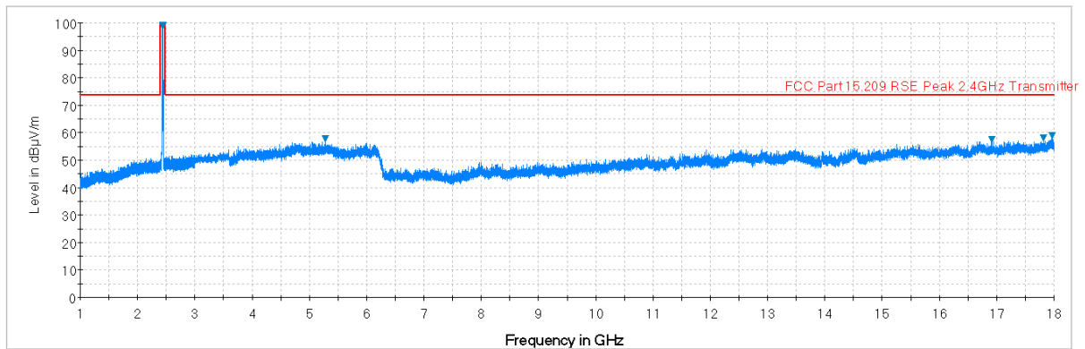
Plot 6-39. Radiated Spurious Plot above 1GHz (802.11b – Ch. 6, Ant. Pol. H)
