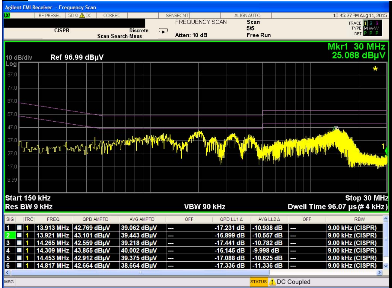
Plot 6-58. Line Conducted Plot with 802.11b (N)
