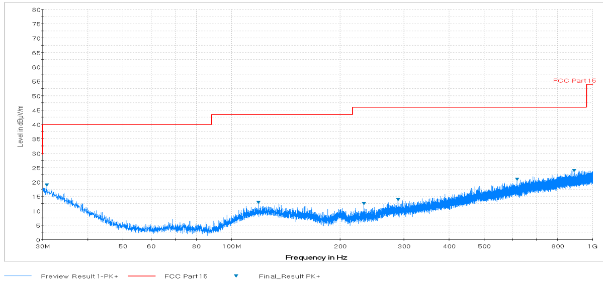
Plot 6-55. Radiated Spurious Plot below 1GHz (Pol. H)
