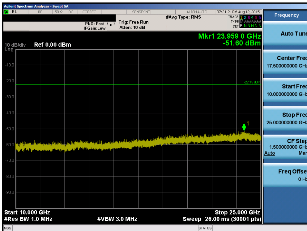
Plot 6-36. Conducted Spurious Plot (802.11b – Ch. 11)
