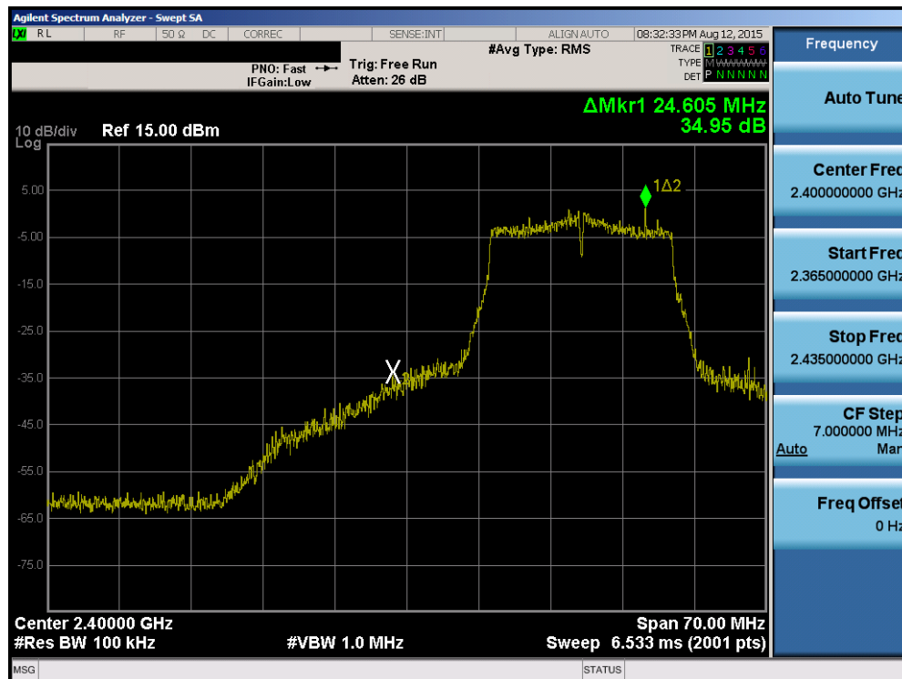
Plot 6-28. Band Edge Plot (802.11n (2.4GHz) - Ch. 2)
