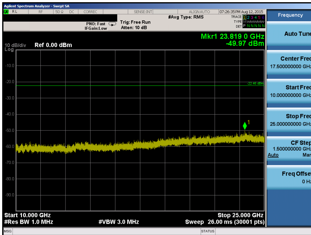
Plot 6-32. Conducted Spurious Plot (802.11b – Ch. 1)
