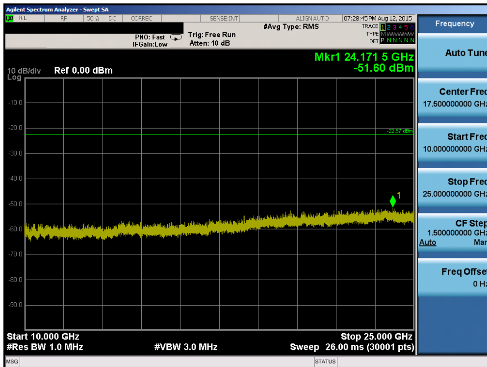
Plot 6-34. Conducted Spurious Plot (802.11b – Ch. 6)
