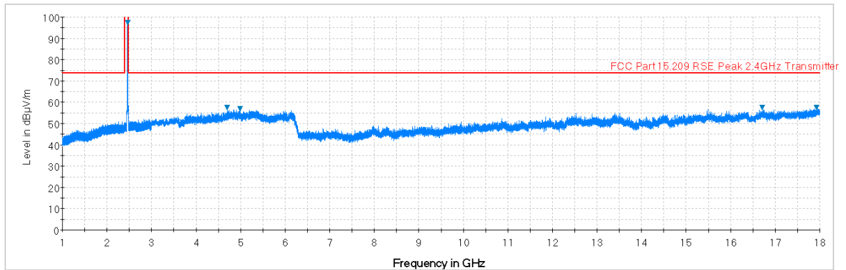
Plot 6-42. Radiated Spurious Plot above 1GHz (802.11b – Ch. 11, Ant. Pol. V)
