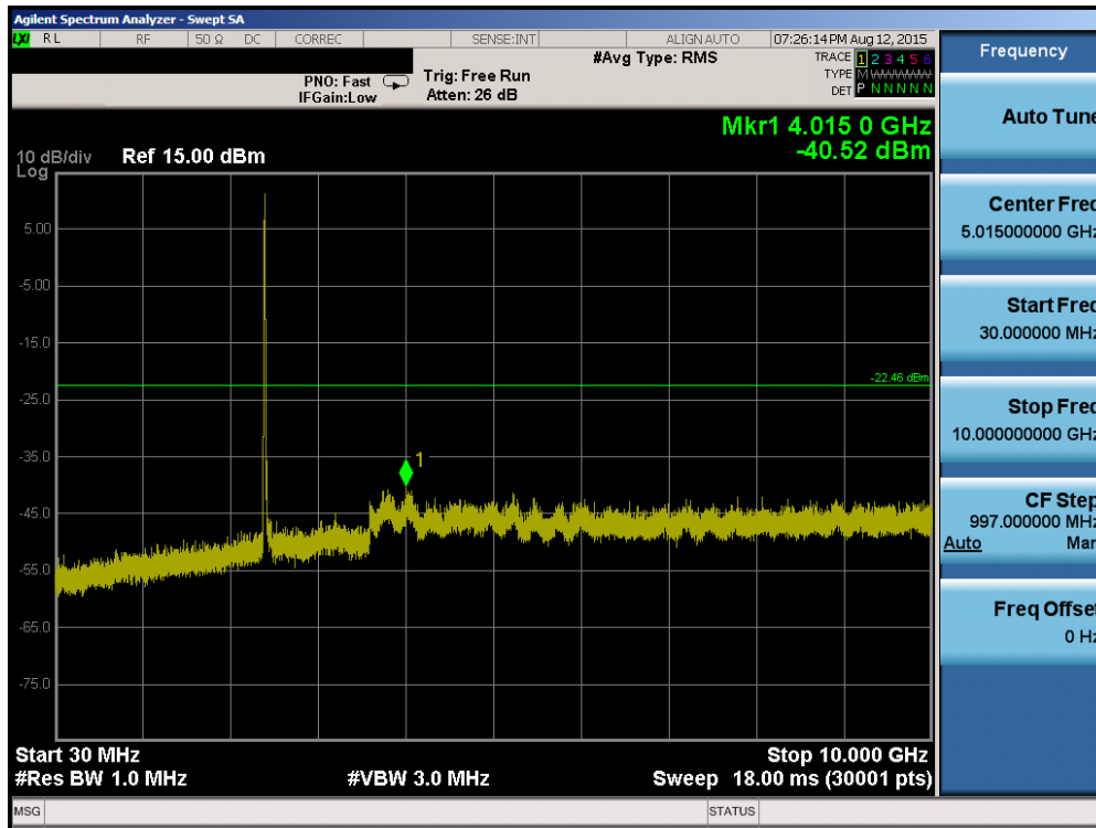
Plot 6-31. Conducted Spurious Plot (802.11b – Ch. 1)
