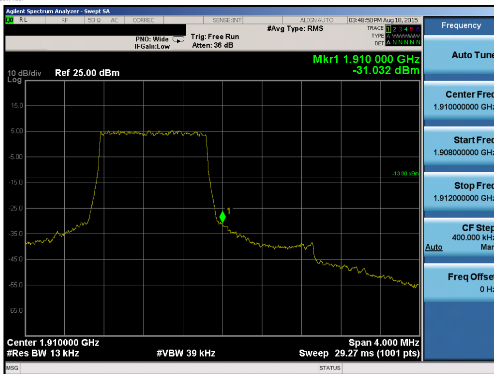
Plot 6-131. Upper Band Edge Plot (Band 2 – 1.4MHz QPSK – RB Size 6)
