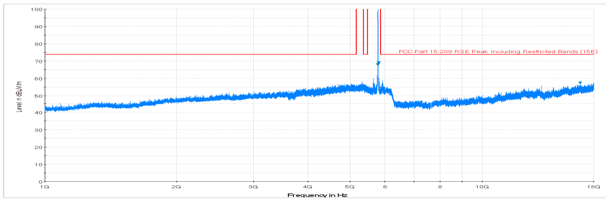
Plot 6-84. Radiated Spurious Plot above 1GHz (802.11a – U3 Ch. 157, Ant. Pol. V)
