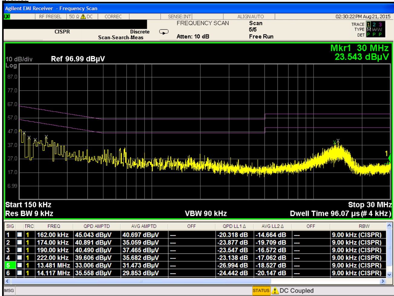
Plot 6-127. Line Conducted Plot with 802.11a UNII Band 2A (N)
