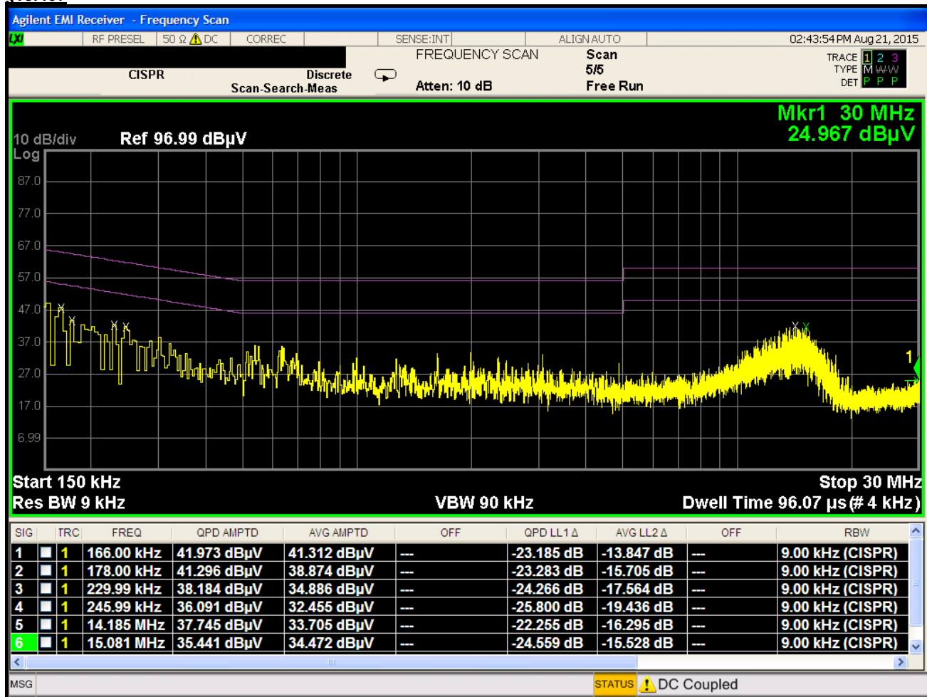
Plot 6-130. Line Conducted Plot with 802.11a UNII Band 3 (L1)
