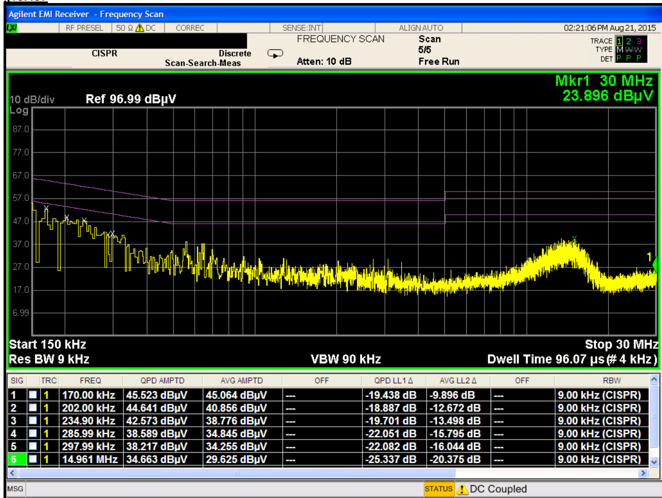
Plot 6-125. Line Conducted Plot with 802.11a UNII Band 1 (N)
