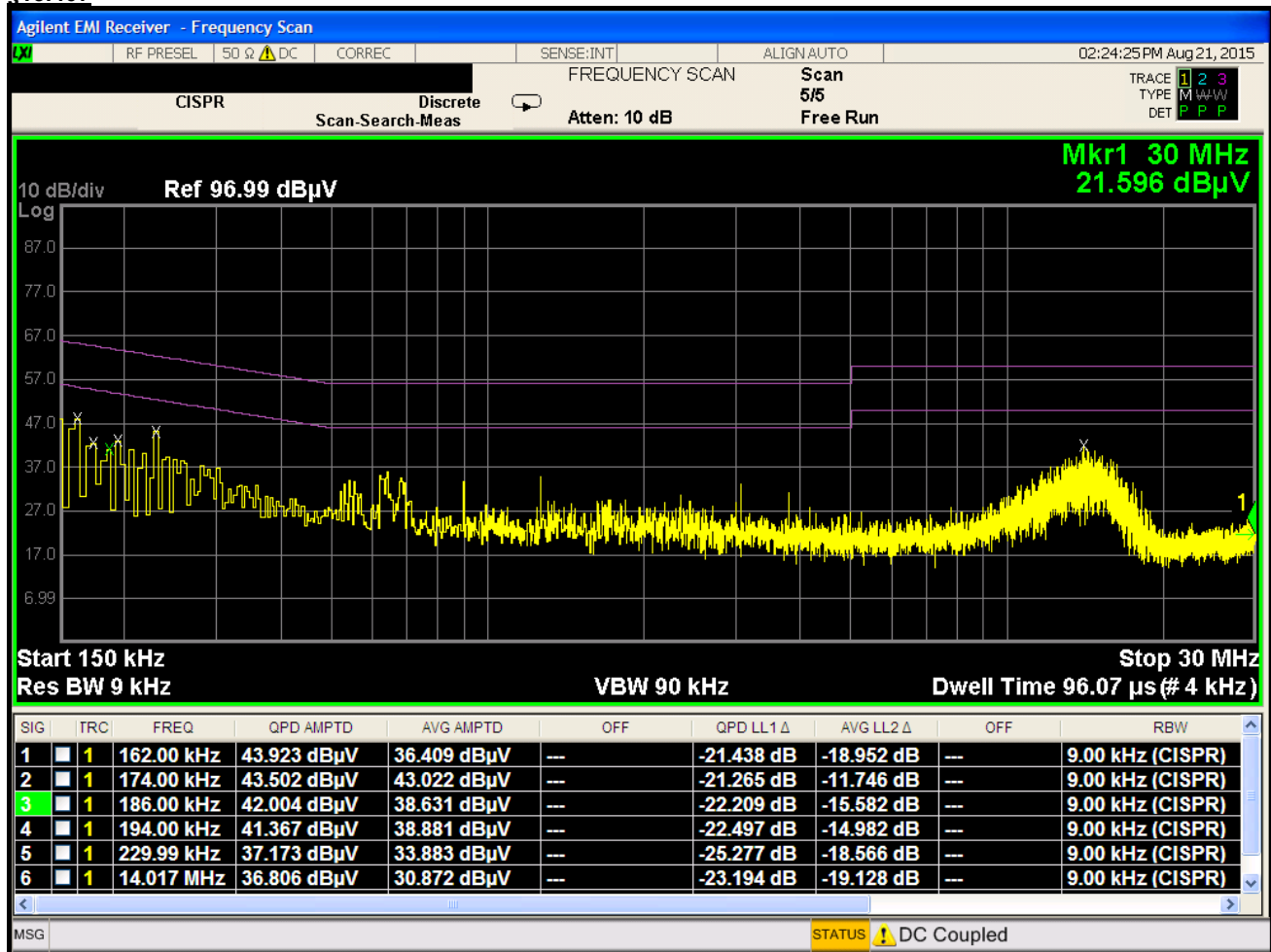
Plot 6-124. Line Conducted Plot with 802.11a UNII Band 1 (L1)
