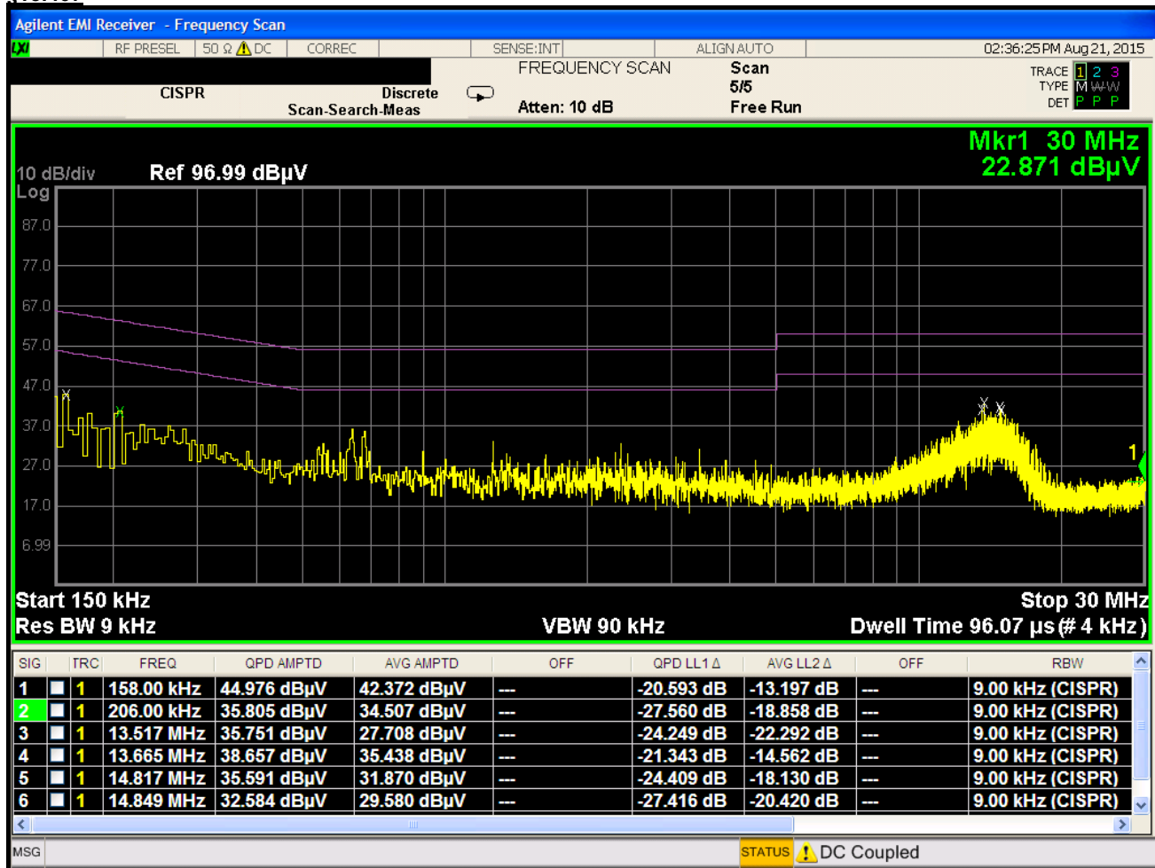
Plot 6-128. Line Conducted Plot with 802.11a UNII Band 2C (L1)
