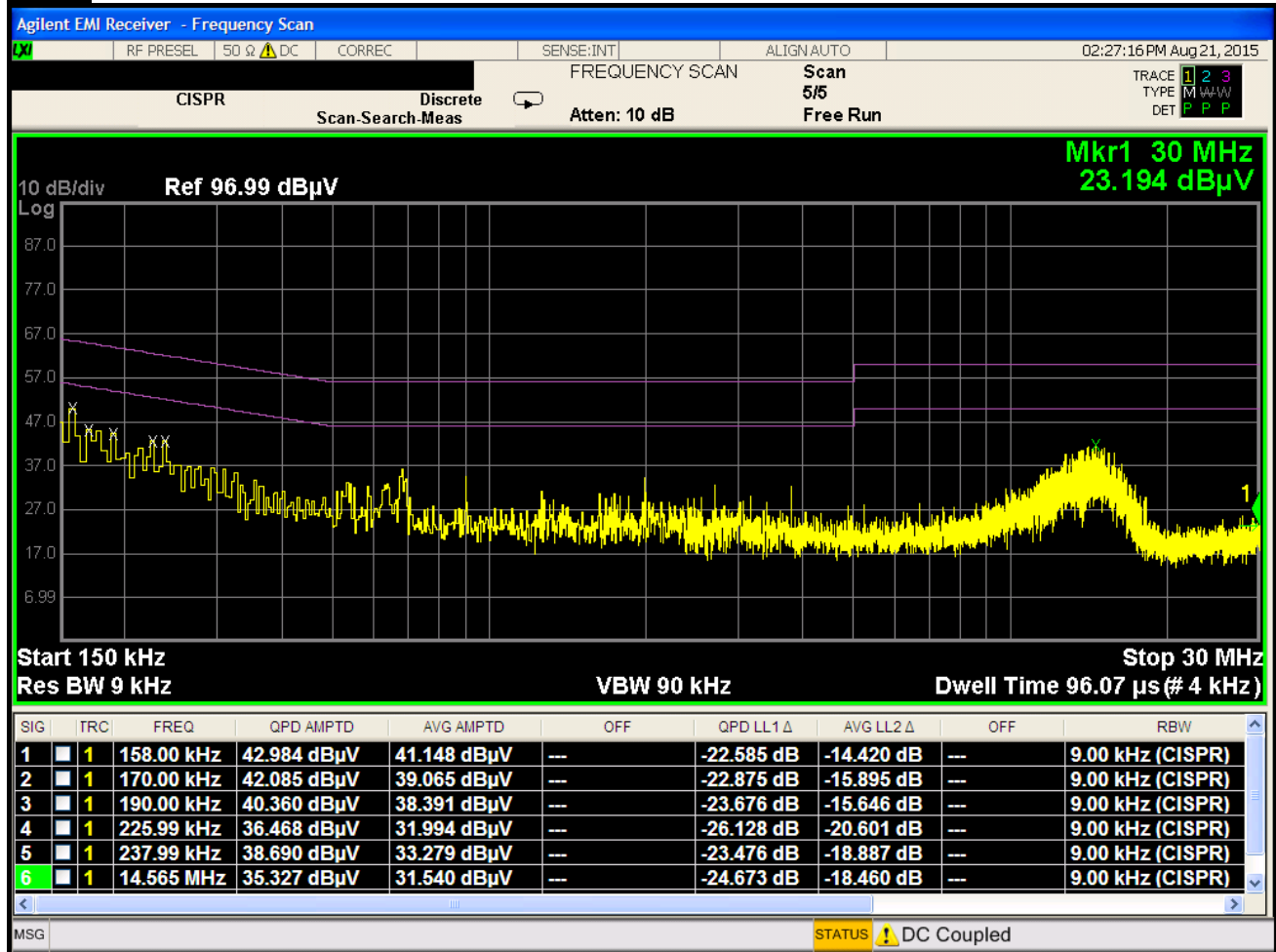
Plot 6-126. Line Conducted Plot with 802.11a UNII Band 2A (L1)
