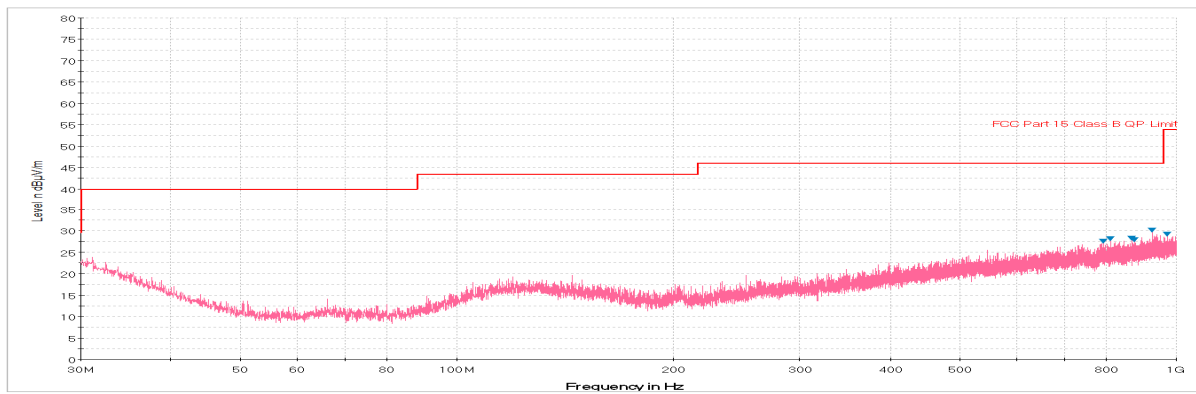
Plot 6-123. Radiated Spurious Plot below 1GHz (802.11a – U3 Ch. 157, Ant. Pol. V)
