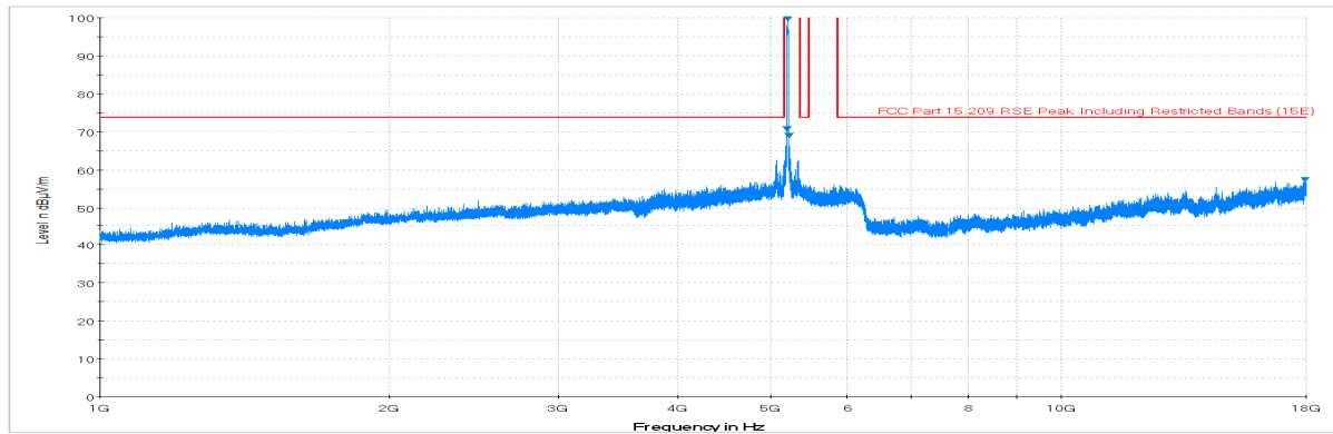
Plot 6-77. Radiated Spurious Plot above 1GHz (802.11a – U1 Ch. 40, Ant. Pol. H)
