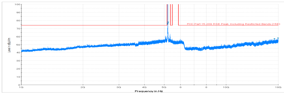
Plot 6-78. Radiated Spurious Plot above 1GHz (802.11a – U1 Ch. 40, Ant. Pol. V)
