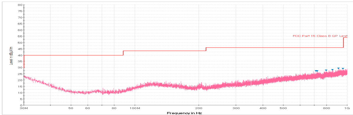
Plot 6-122. Radiated Spurious Plot below 1GHz (802.11a – U3 Ch. 157, Ant. Pol. H)
