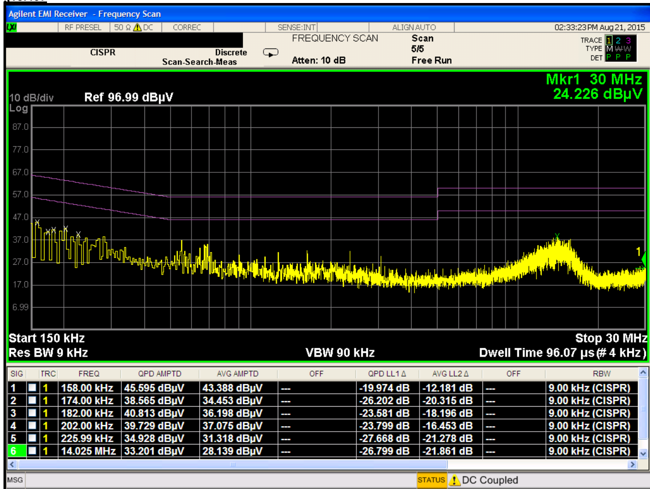
Plot 6-129. Line Conducted Plot with 802.11a UNII Band 2C (N)
