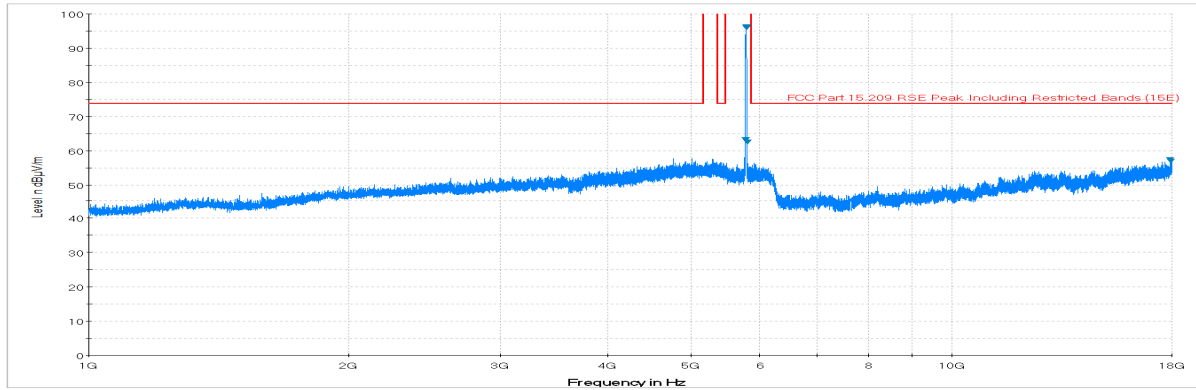
Plot 6-83. Radiated Spurious Plot above 1GHz (802.11a – U3 Ch. 157, Ant. Pol. H)
