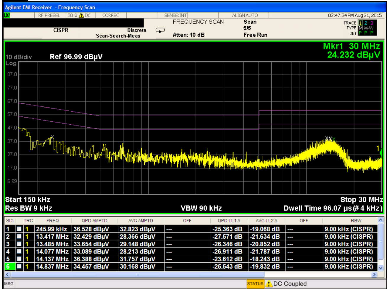
Plot 6-131. Line Conducted Plot with 802.11a UNII Band 3 (N)
