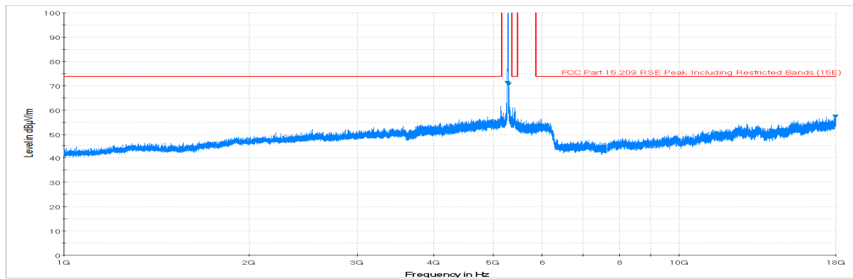
Plot 6-79. Radiated Spurious Plot above 1GHz (802.11a – U2A Ch. 56, Ant. Pol. H)
