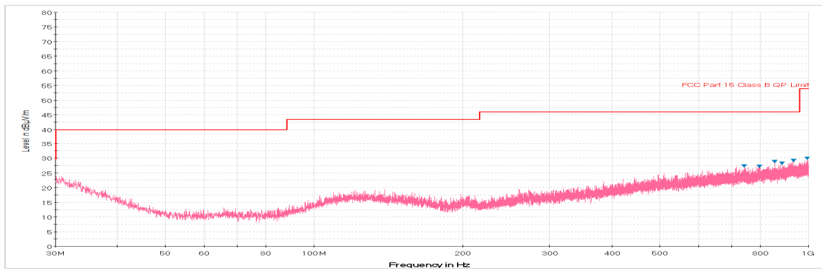
Plot 6-56. Radiated Spurious Plot below 1GHz (Pol. V)
