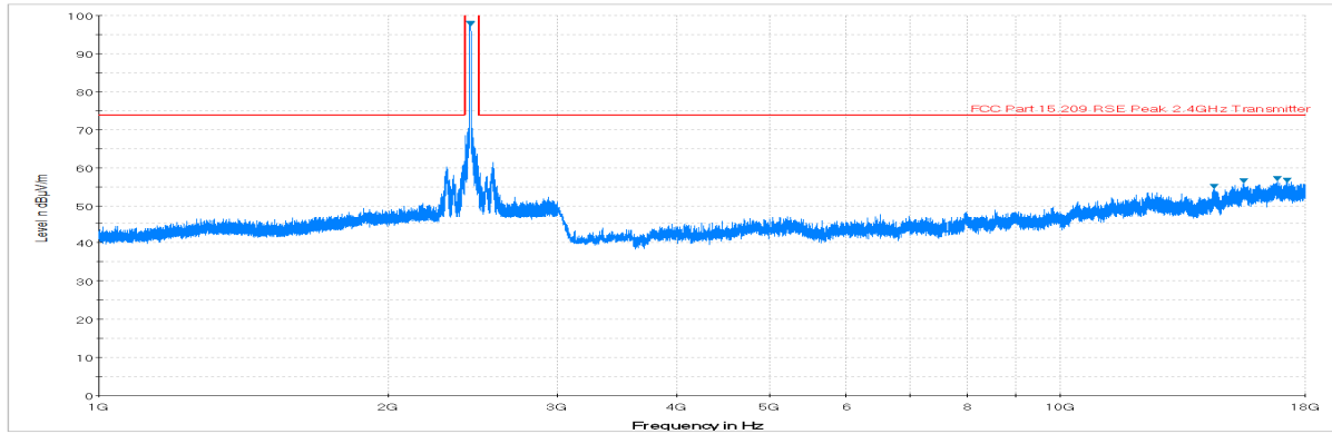
Plot 6-40. Radiated Spurious Plot above 1GHz (802.11b – Ch. 6, Ant. Pol. V)
