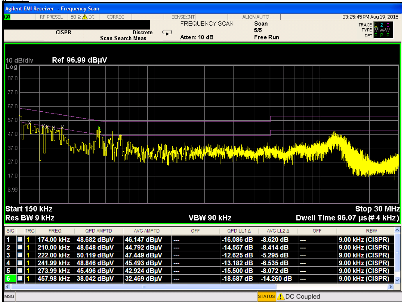
Plot 6-57. Line Conducted Plot with 802.11b (L1)
