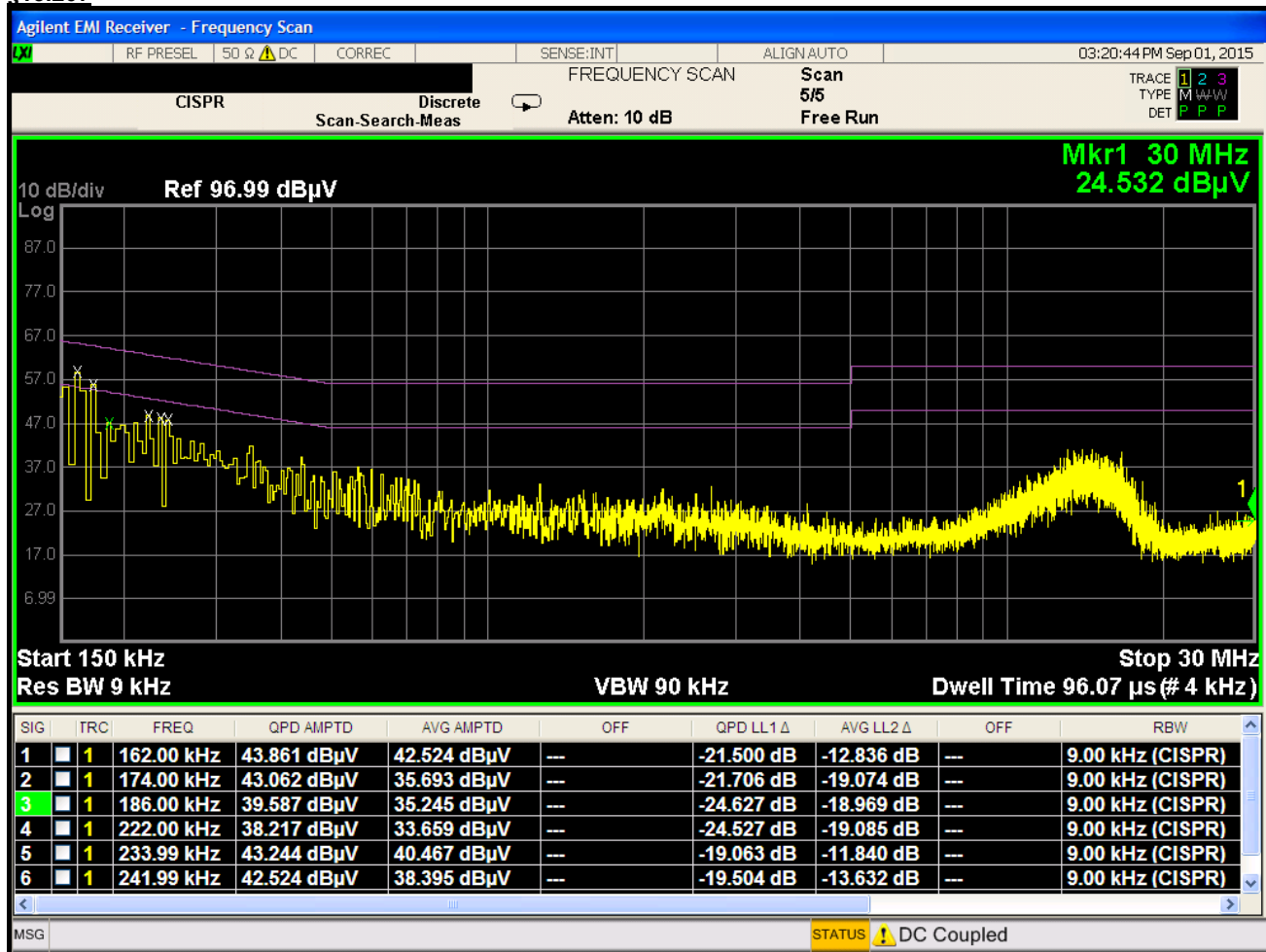
Plot 6-58. Line Conducted Plot with 802.11b (N)
