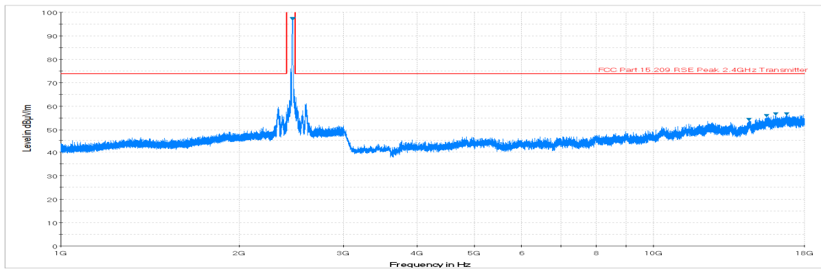
Plot 6-41. Radiated Spurious Plot above 1GHz (802.11b – Ch. 11, Ant. Pol. H)
