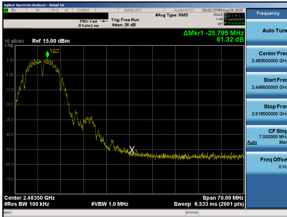
Plot 6-21. Band Edge Plot (802.11b – Ch. 10)
