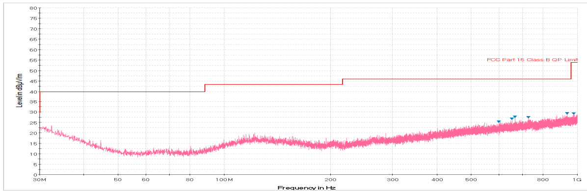
Plot 6-55. Radiated Spurious Plot below 1GHz (Pol. H)
