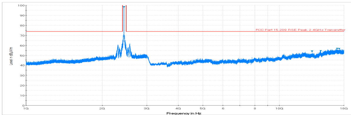
Plot 6-39. Radiated Spurious Plot above 1GHz (802.11b – Ch. 6, Ant. Pol. H)
