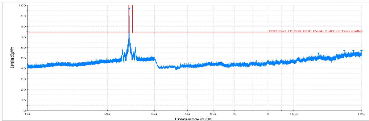
Plot 6-38. Radiated Spurious Plot above 1GHz (802.11b – Ch. 1, Ant. Pol. V)
