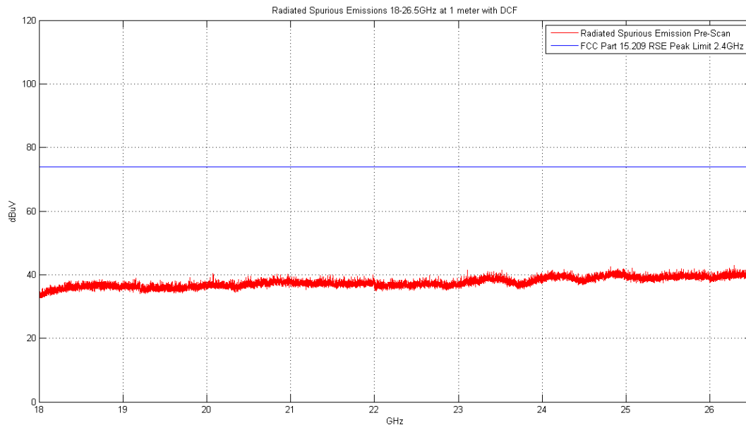
Plot 6-44. Radiated Spurious Plot above 18GHz (Pol. V)
