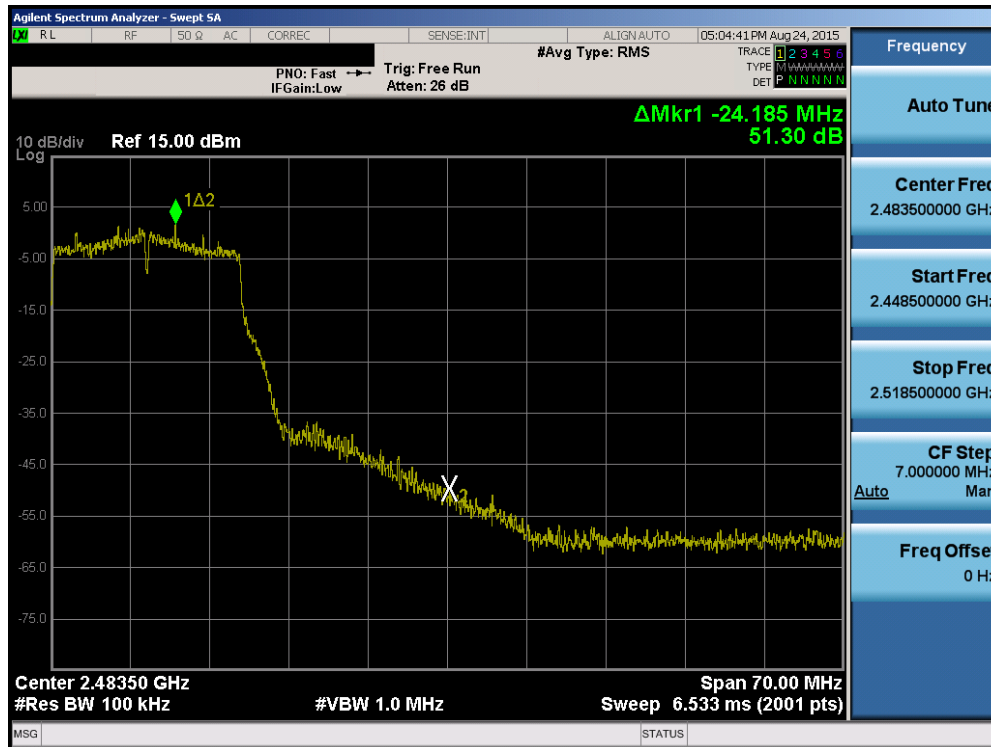
Plot 6-25. Band Edge Plot (802.11g– Ch. 10)
