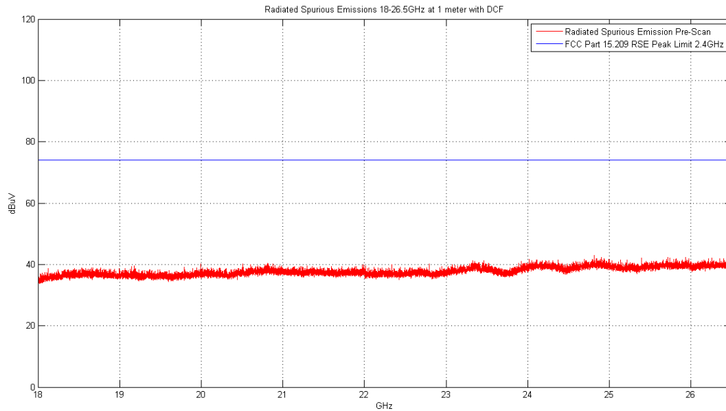
Plot 6-43. Radiated Spurious Plot above 18GHz (Pol. H)
