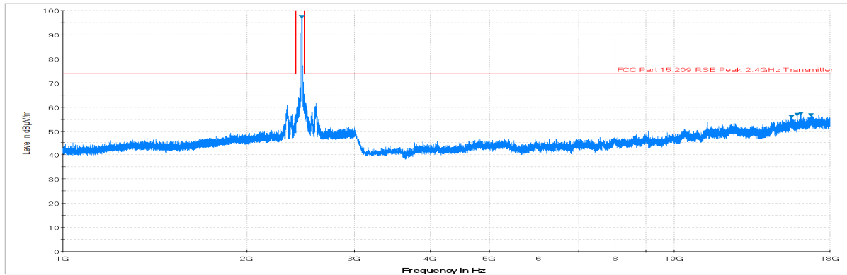
Plot 6-42. Radiated Spurious Plot above 1GHz (802.11b – Ch. 11, Ant. Pol. V)
