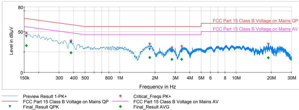
Plot 8-1. Line-Conducted Test Plot (L1)
