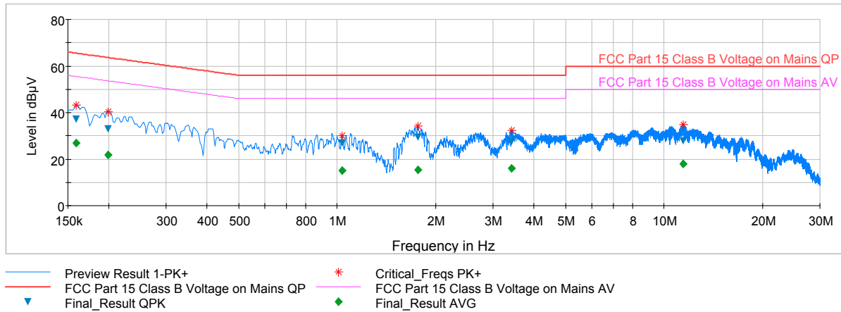
Plot 8-2. Line-Conducted Test Plot (N)
