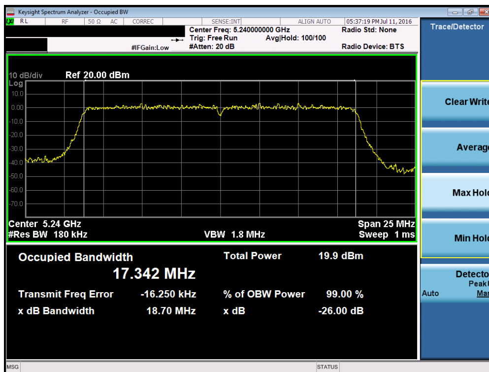
Plot 7-6. 26dB Bandwidth Plot (20MHz BW 802.11n (UNII Band 1) – Ch. 48)
