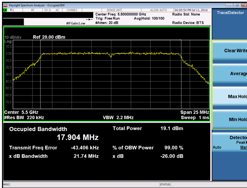
Plot 7-51. 26dB Bandwidth Plot (20MHz BW 802.11n (UNII Band 2C) – Ch. 100)
