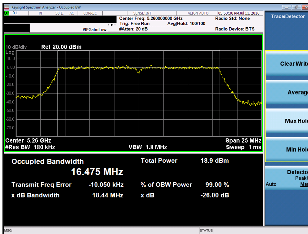
Plot 7-39. 26dB Bandwidth Plot (802.11a (UNII Band 2A) – Ch. 52)
