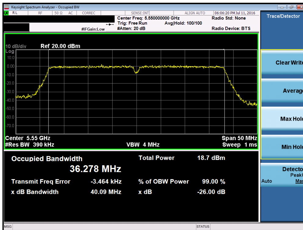
Plot 7-55. 26dB Bandwidth Plot (40MHz BW 802.11n (UNII Band 2C) – Ch. 110)
