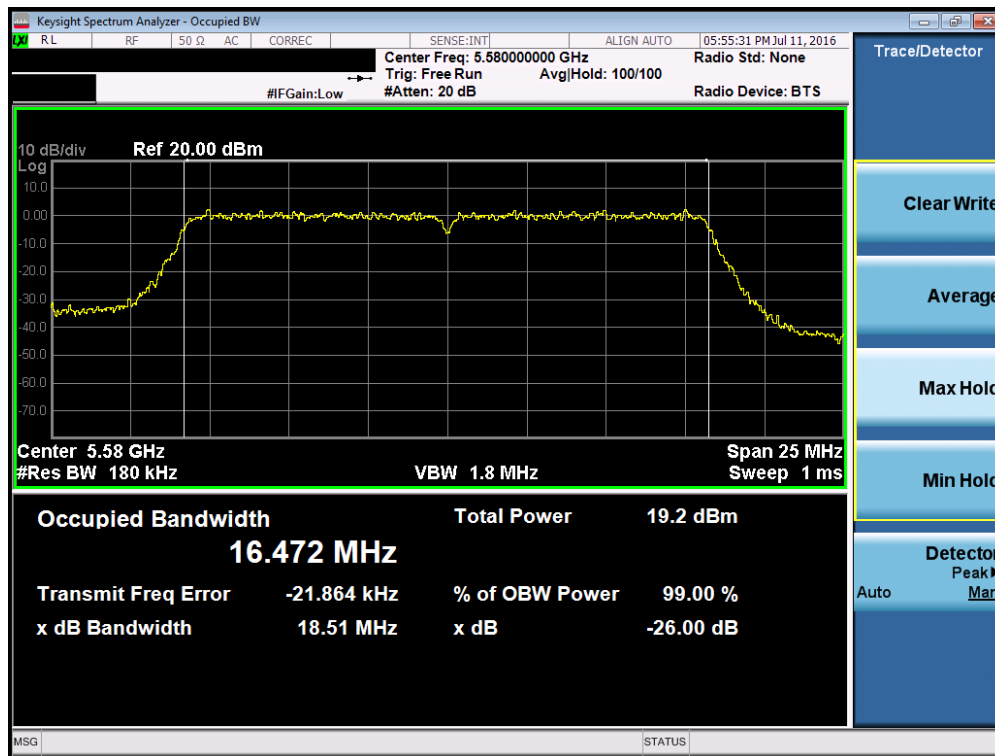
Plot 7-49. 26dB Bandwidth Plot (802.11a (UNII Band 2C) – Ch. 116)
