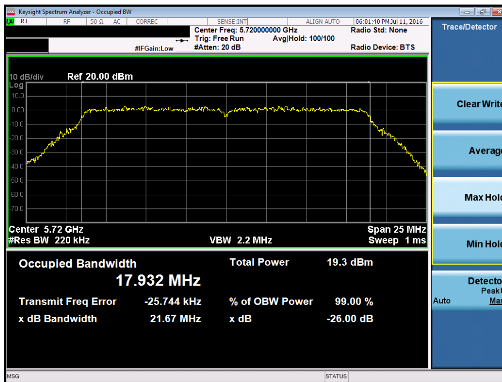
Plot 7-53. 26dB Bandwidth Plot (20MHz BW 802.11n (UNII Band 2C) – Ch. 144)
