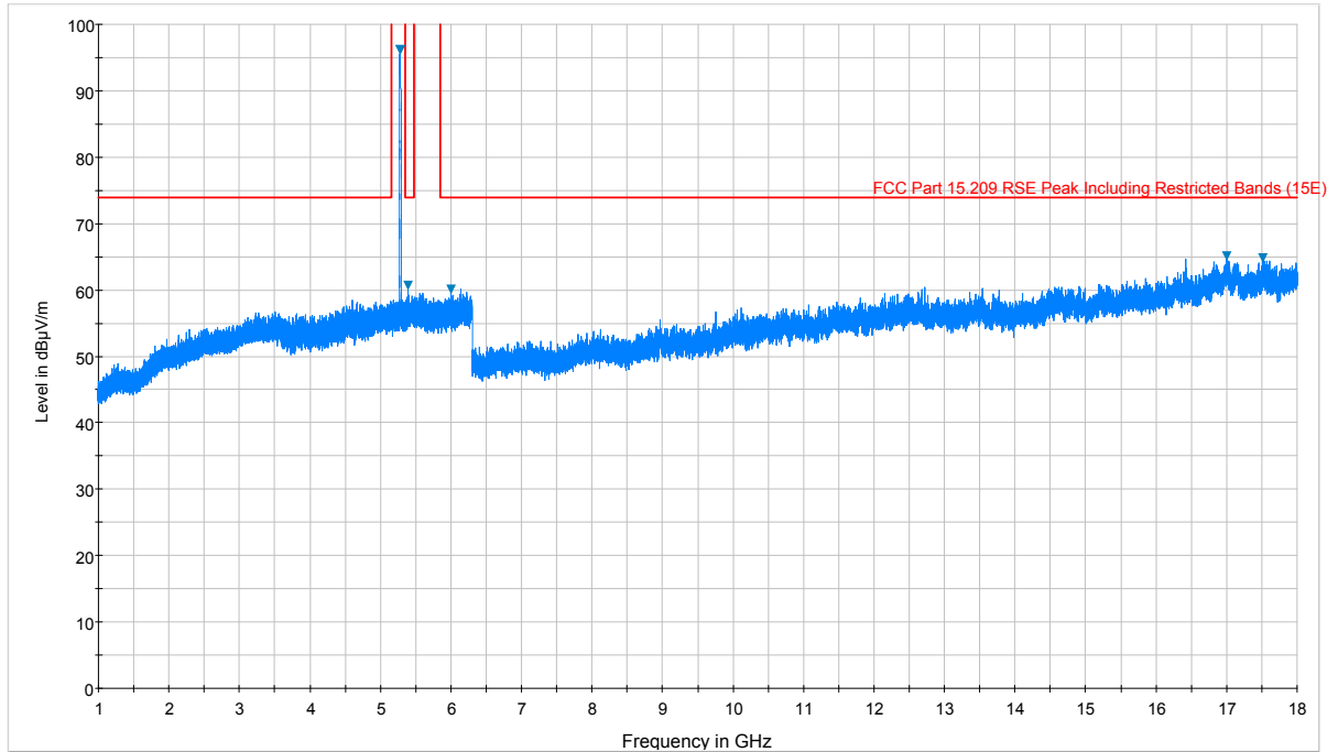
Plot 7-155. Radiated Spurious Plot above 1GHz (802.11a – U2A Ch. 56, Ant. Pol. H)
