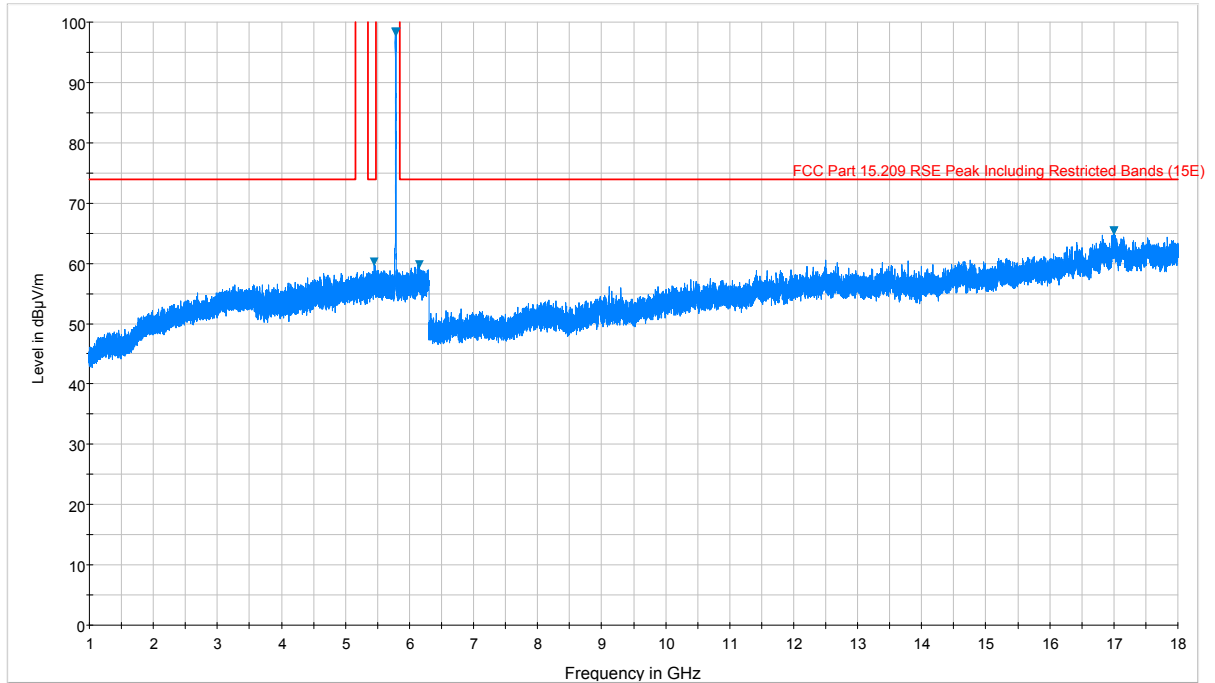
Plot 7-171. Radiated Spurious Plot above 1GHz (802.11a – U3 Ch. 157, Ant. Pol. H)
