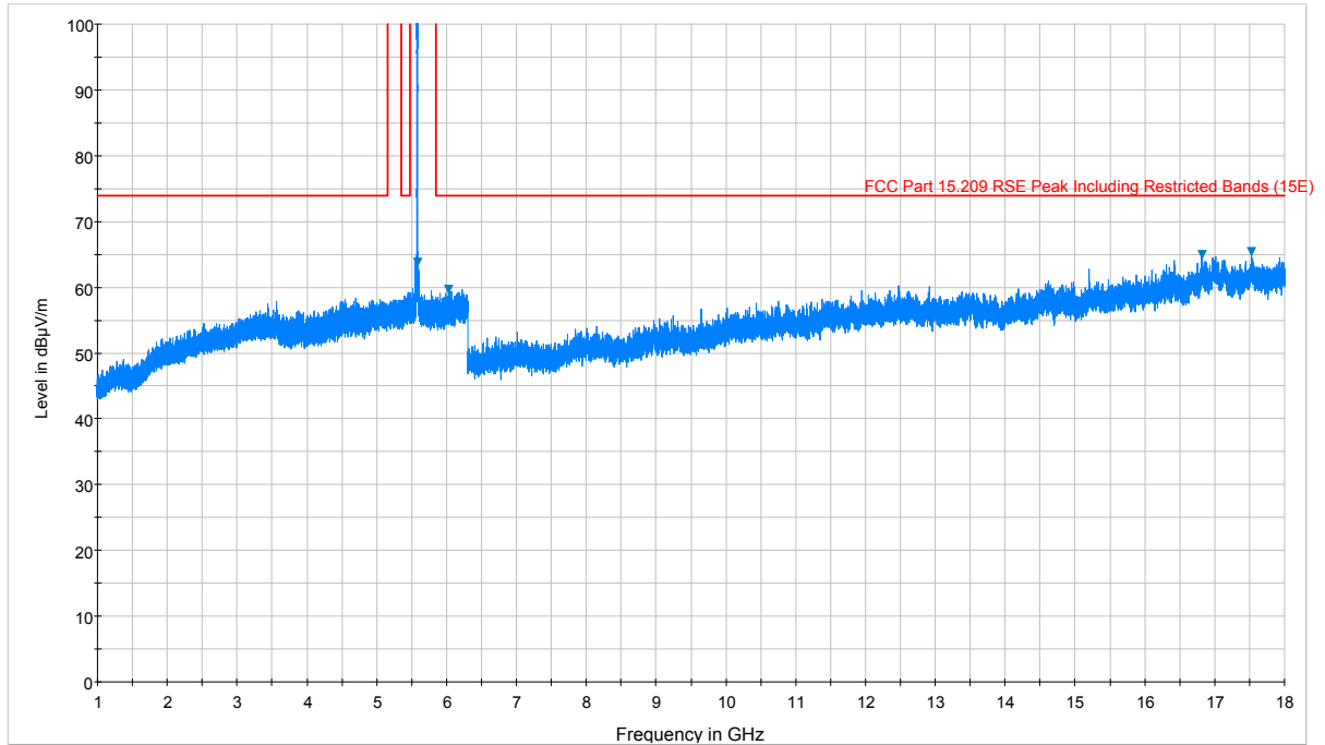
Plot 7-169. Radiated Spurious Plot above 1GHz (802.11a – U2C Ch. 116, Ant. Pol. H)
