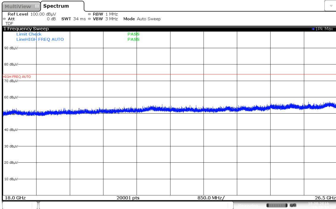
Plot 7-20. Radiated Spurious Plot above 18GHz (802.11a – Ant. Pol. V)
