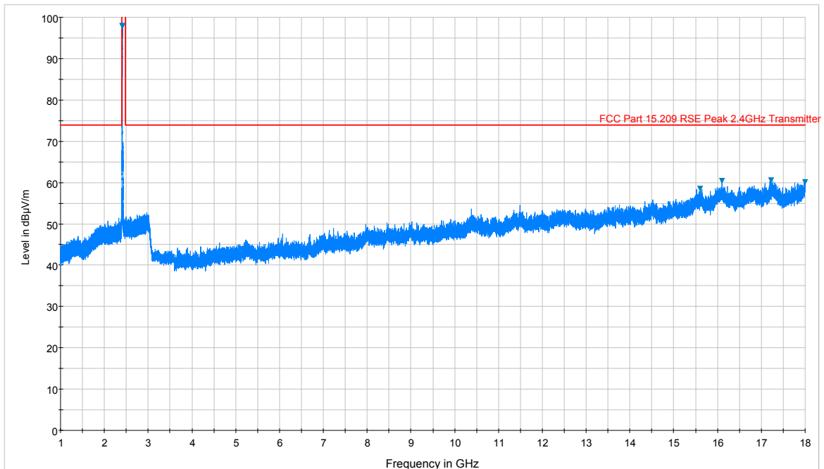
Plot 7-69. Radiated Spurious Plot above 1GHz (802.11b – Ch. 1, Ant. Pol. H)
