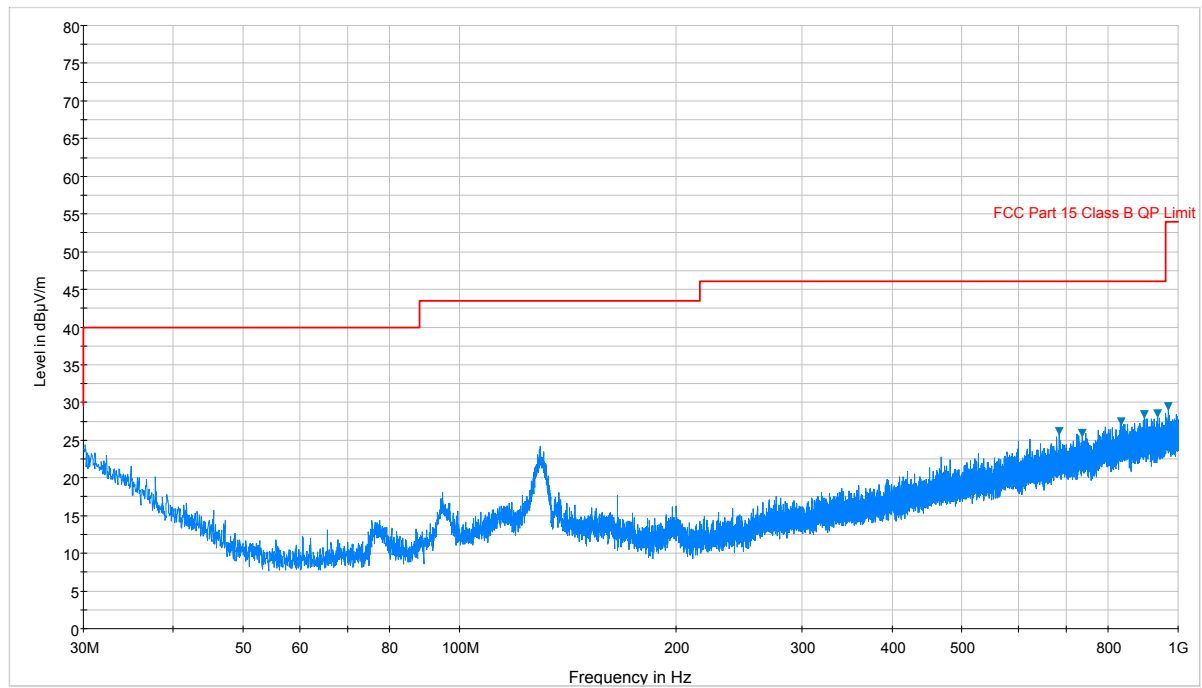
Plot 7-92. Radiated Spurious Plot below 1GHz (Pol. V)
