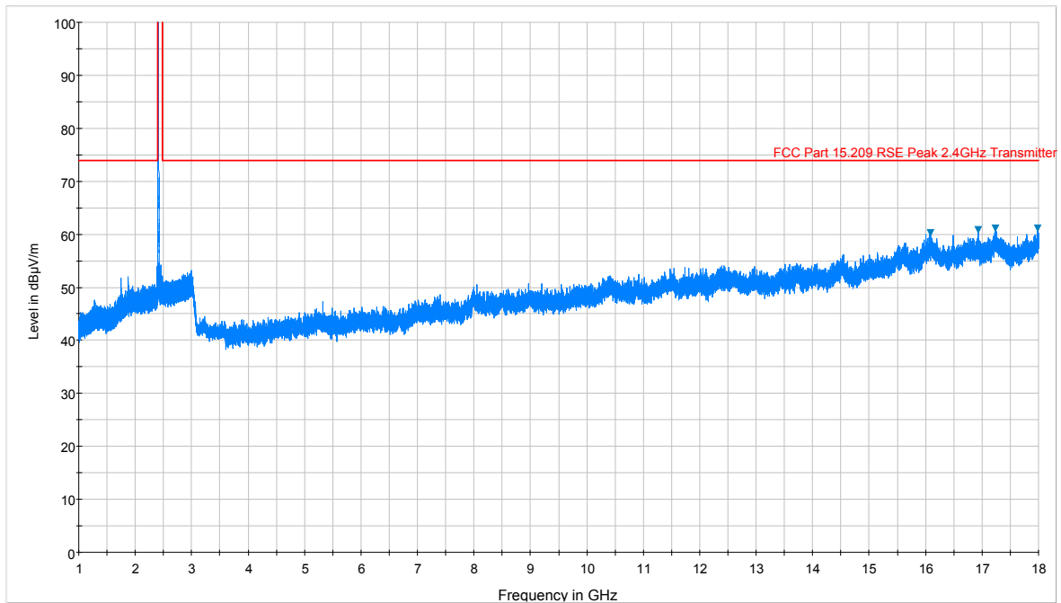
Plot 7-61. Radiated Spurious Plot above 1GHz (802.11b – Ch. 1, Ant. Pol. H)
