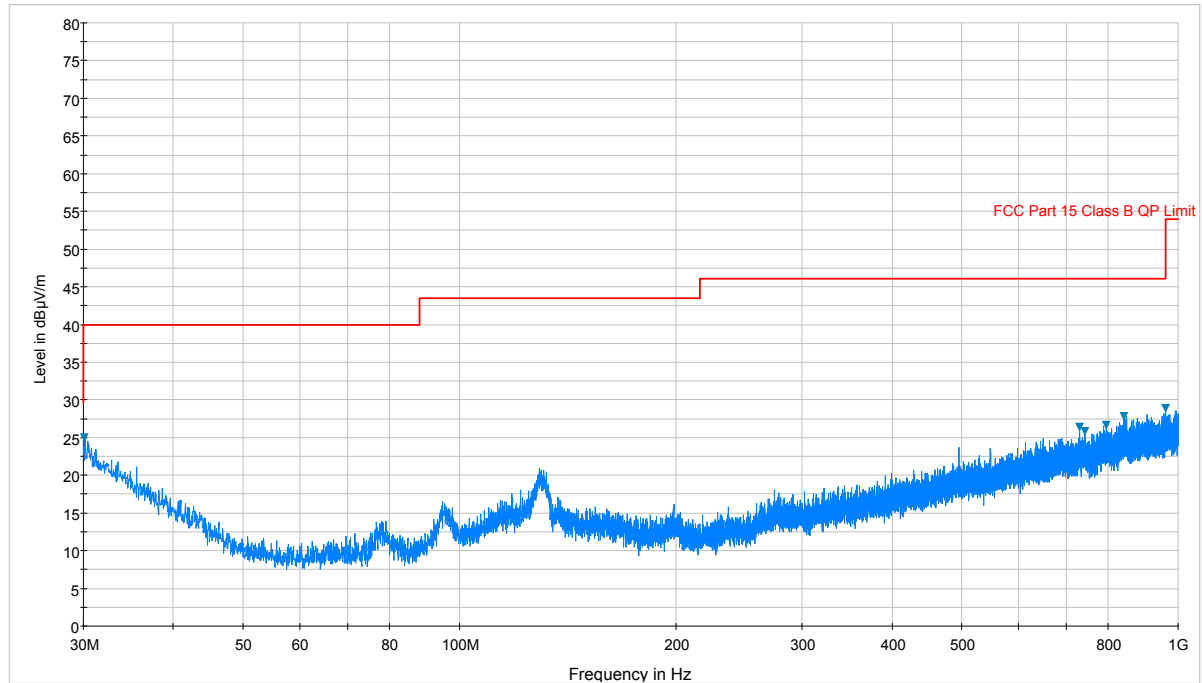
Plot 7-91. Radiated Spurious Plot below 1GHz (Pol. H)
