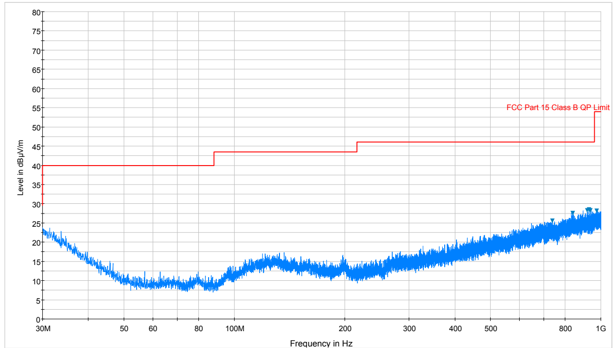
Plot 7-89. Radiated Spurious Plot below 1GHz (Pol. H)
