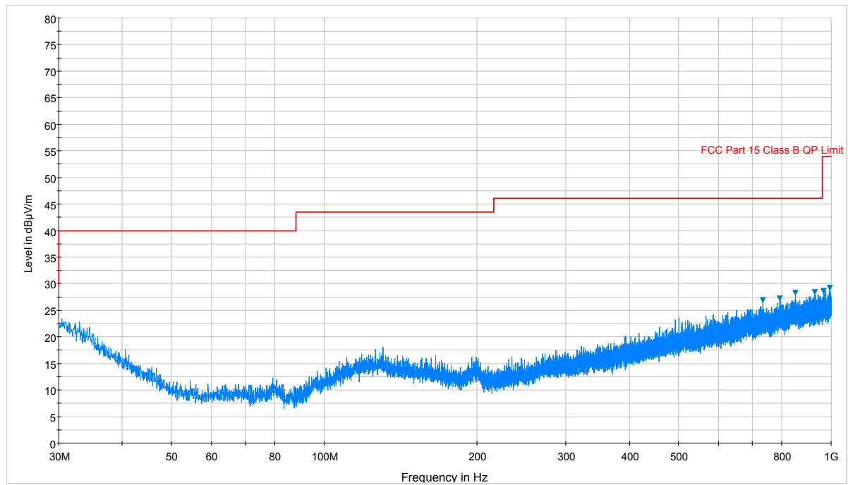
Plot 7-90. Radiated Spurious Plot below 1GHz (Pol. V)
