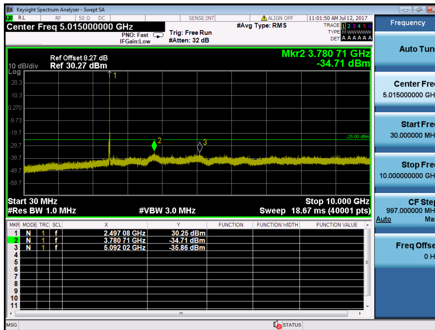
LTE Band 41 / 20MHz / 16QAM - RB Size/Offset (1/0) – Low Channel
