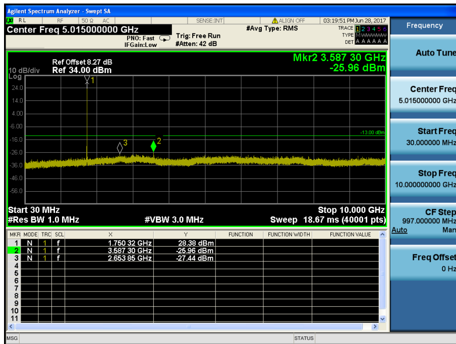
LTE Band 4 / 10MHz / 64QAM - RB Size/Offset (1/24) – High Channel
