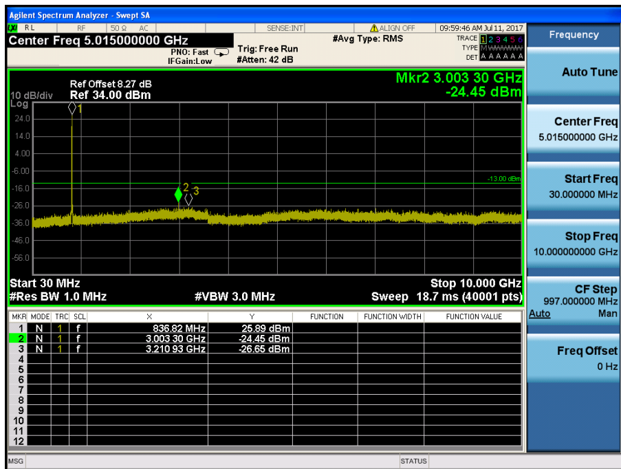
LTE Band 5 / 5MHz / 64QAM - RB Size/Offset (25/0) – Mid Channel
