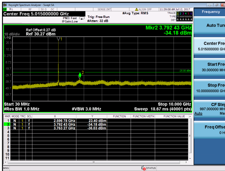
LTE Band 41 / 10MHz / 64QAM - RB Size/Offset (25/25) – Mid Channel
