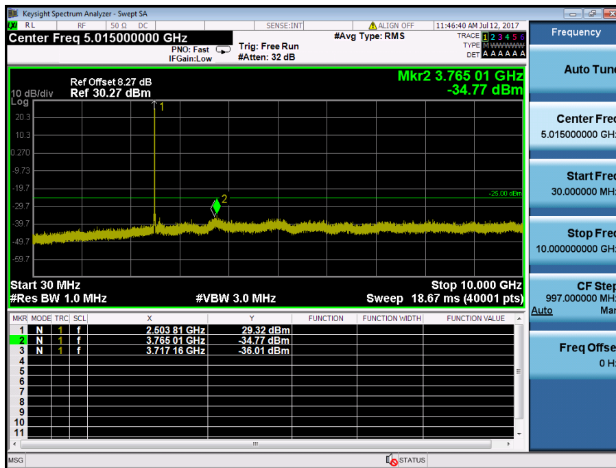
LTE Band 41 / 15MHz / 64QAM - RB Size/Offset (1/37) – Low Channel
