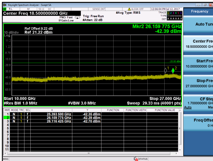
LTE Band 41 / 20MHz / 64QAM - RB Size/Offset (1/0) – Mid Channel
