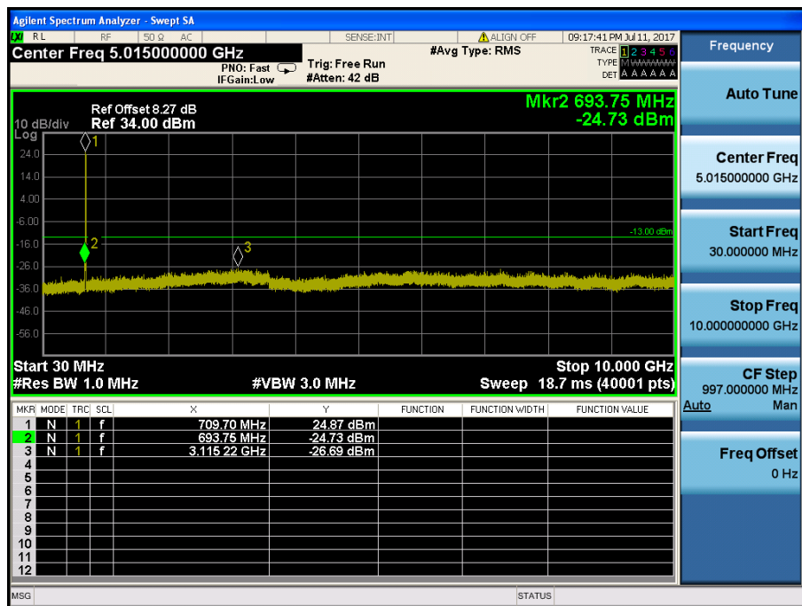
LTE Band 17 / 5MHz / 64QAM - RB Size/Offset (25/0)–Mid Channel
