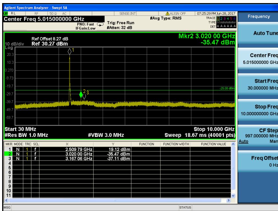
LTE Band 7 / 20MHz / 16QAM - RB Size/Offset (100/0) – Low Channel
