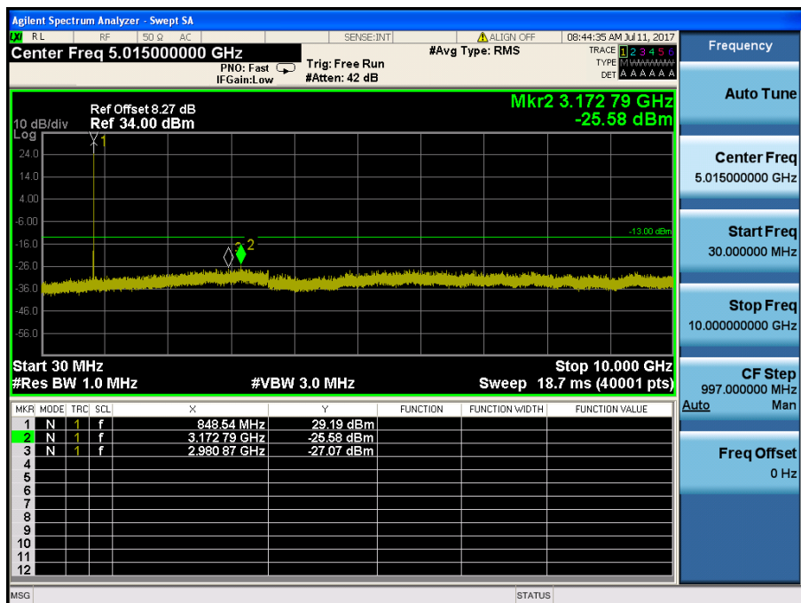
LTE Band 5 / 1.4MHz / 64QAM - RB Size/Offset (1/3) – High Channel
