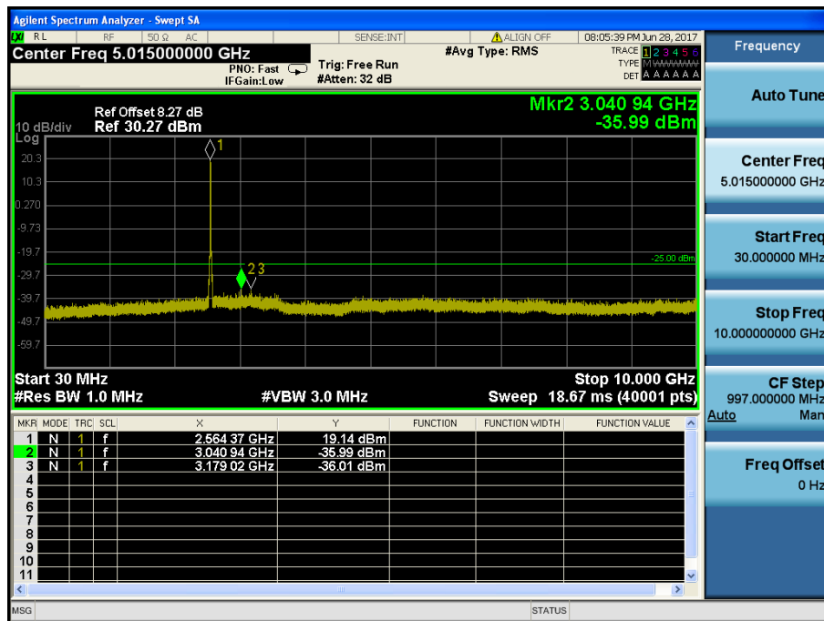
LTE Band 7 / 10MHz / 64QAM - RB Size/Offset (50/0) – High Channel
