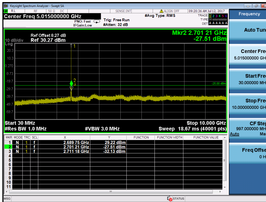
LTE Band 41 / 5MHz / QPSK - RB Size/Offset (1/24) – High Channel
