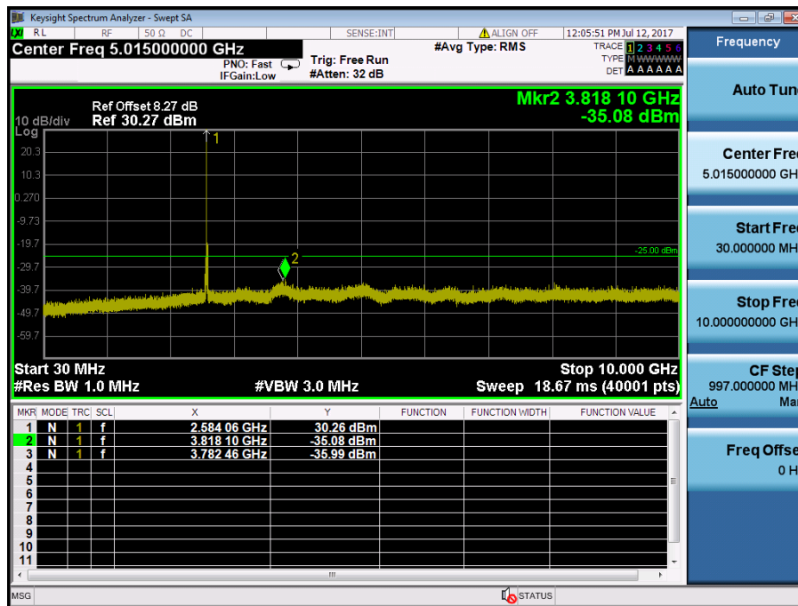
LTE Band 41 / 20MHz / 64QAM - RB Size/Offset (1/0) – Mid Channel
