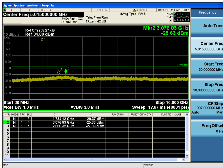
LTE Band 4 / 3MHz / 64QAM - RB Size/Offset (1/14) – Mid Channel
