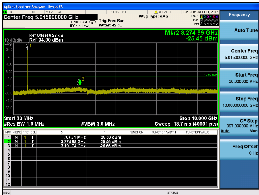
LTE Band 12 / 1.4MHz / 64QAM - RB Size/Offset (6/0) – Mid Channel
