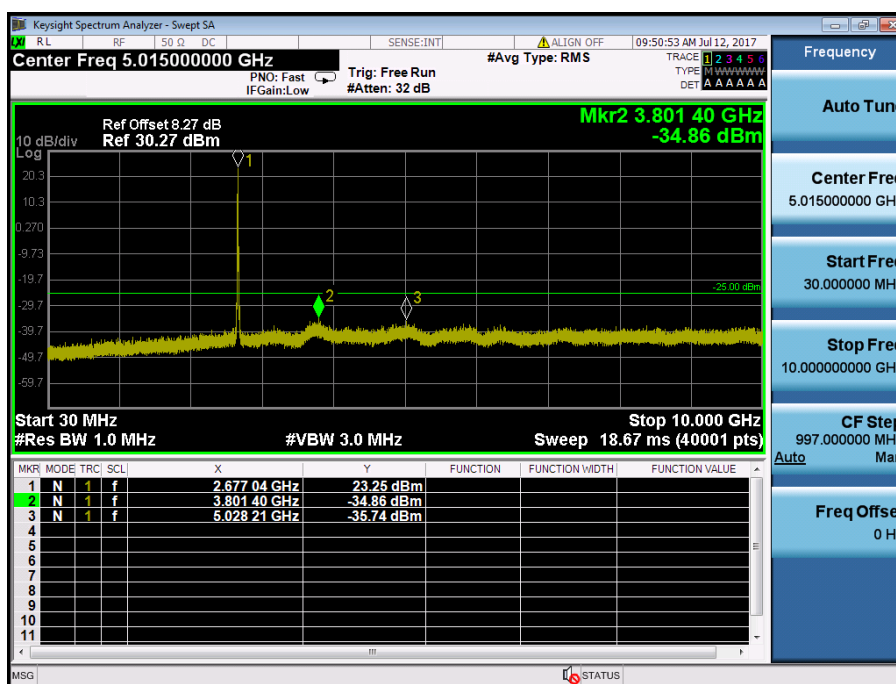
LTE Band 41 / 15MHz / QPSK - RB Size/Offset (36/0) – High Channel
