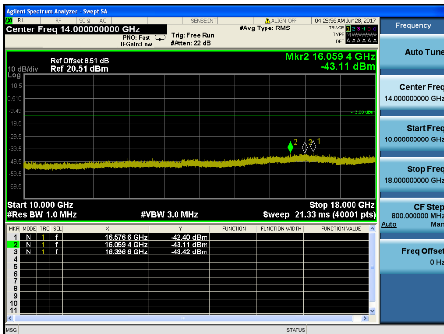
LTE Band 4 / 3MHz / QPSK - RB Size/Offset (8/3) – High Channel
