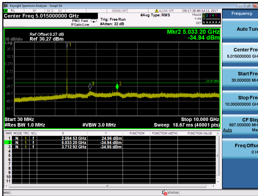
LTE Band 41 / 5MHz / QPSK - RB Size/Offset (12/13) – Mid Channel
