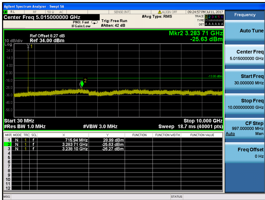
LTE Band 17 / 5MHz / 64QAM - RB Size/Offset (1/24) – High Channel
