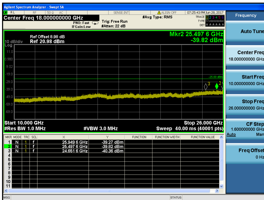
LTE Band 7 / 20MHz / 16QAM - RB Size/Offset (100/0) – Low Channel
