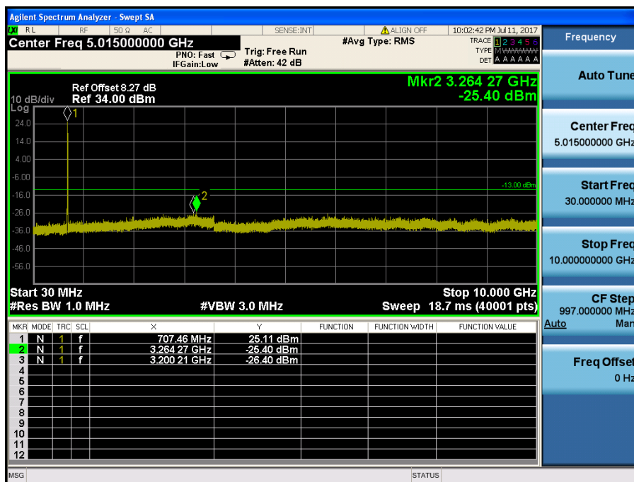
LTE Band 17 / 10MHz / 64QAM - RB Size/Offset (25/0) – High Channel
