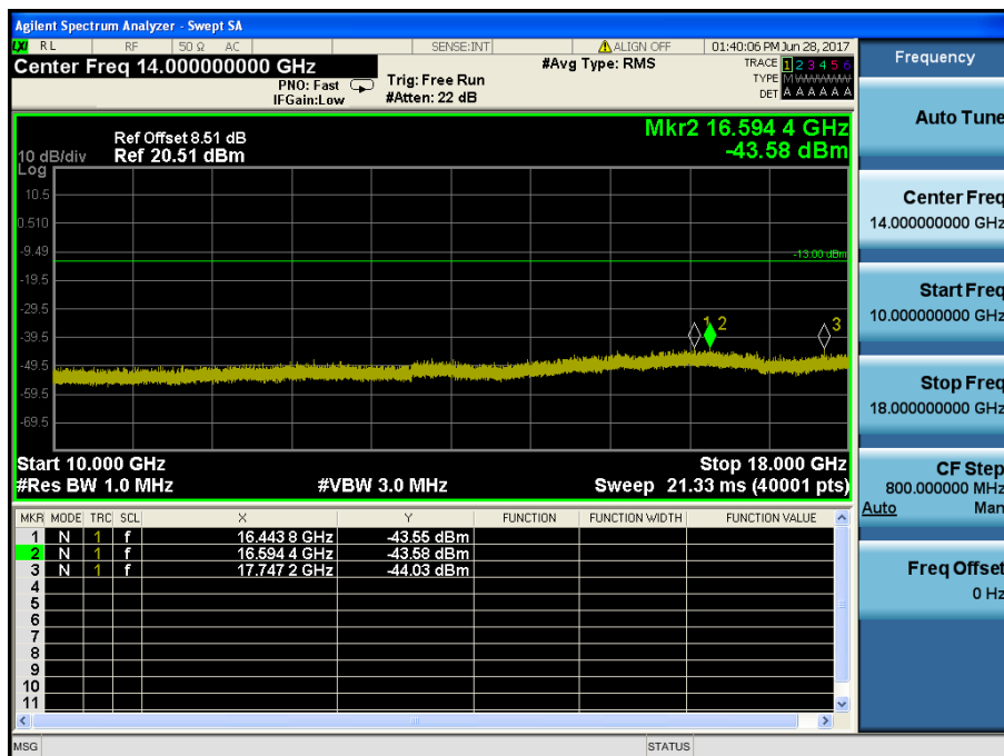
LTE Band 4 / 3MHz / 64QAMK - RB Size/Offset (1/14) – Mid Channel
