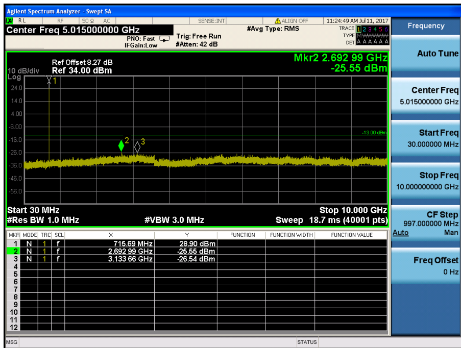
LTE Band 12 / 1.4MHz / QPSK - RB Size/Offset (1/3) – High Channel
