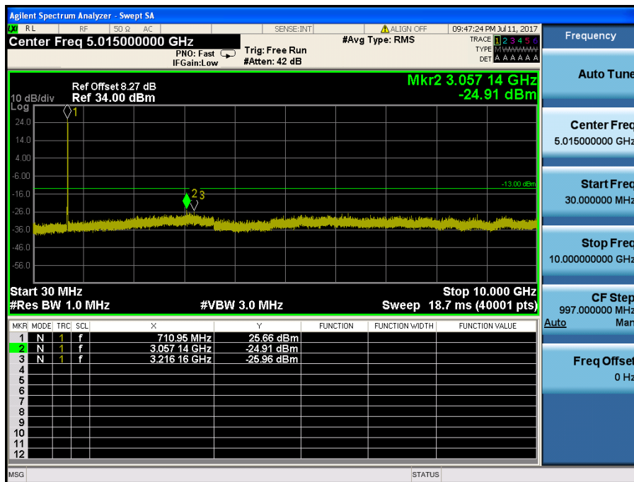
LTE Band 17 / 10MHz / 64QAM - RB Size/Offset (25/12) – Low Channel
