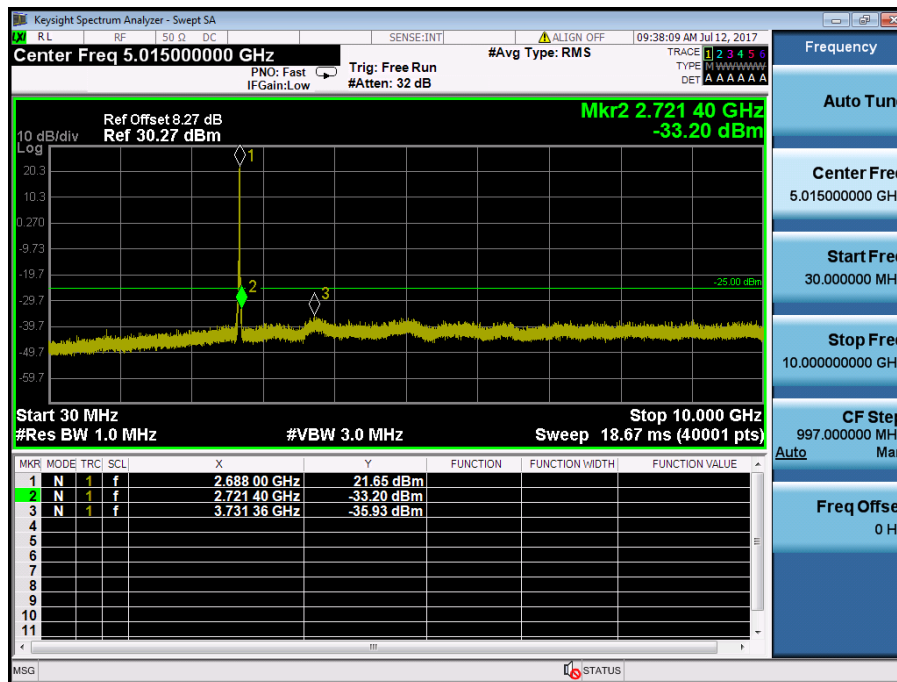
LTE Band 41 / 10MHz / QPSK - RB Size/Offset (25/0) – High Channel
