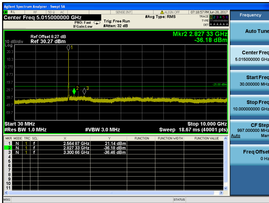
LTE Band 7 / 15MHz / 16QAM - RB Size/Offset (36/39) – High Channel
