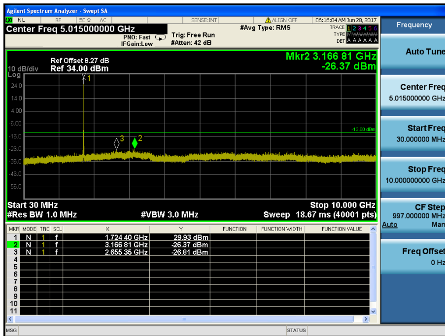
LTE Band 4 / 15MHz / QPSK - RB Size/Offset (1/74)-Low Channel
