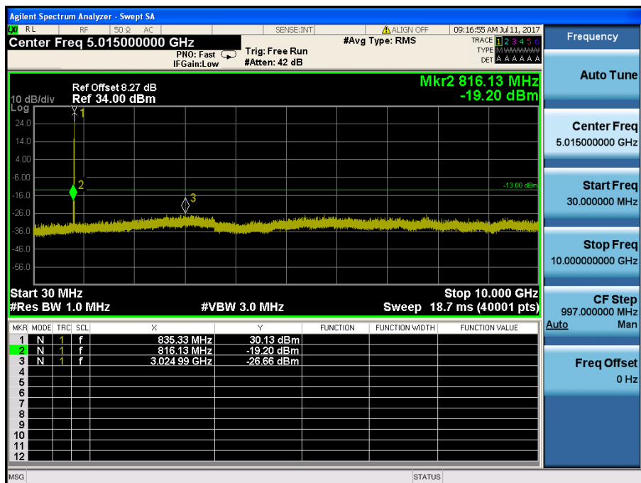
LTE Band 5 / 3MHz / 64QAM - RB Size/Offset (1/0) – Mid Channel
