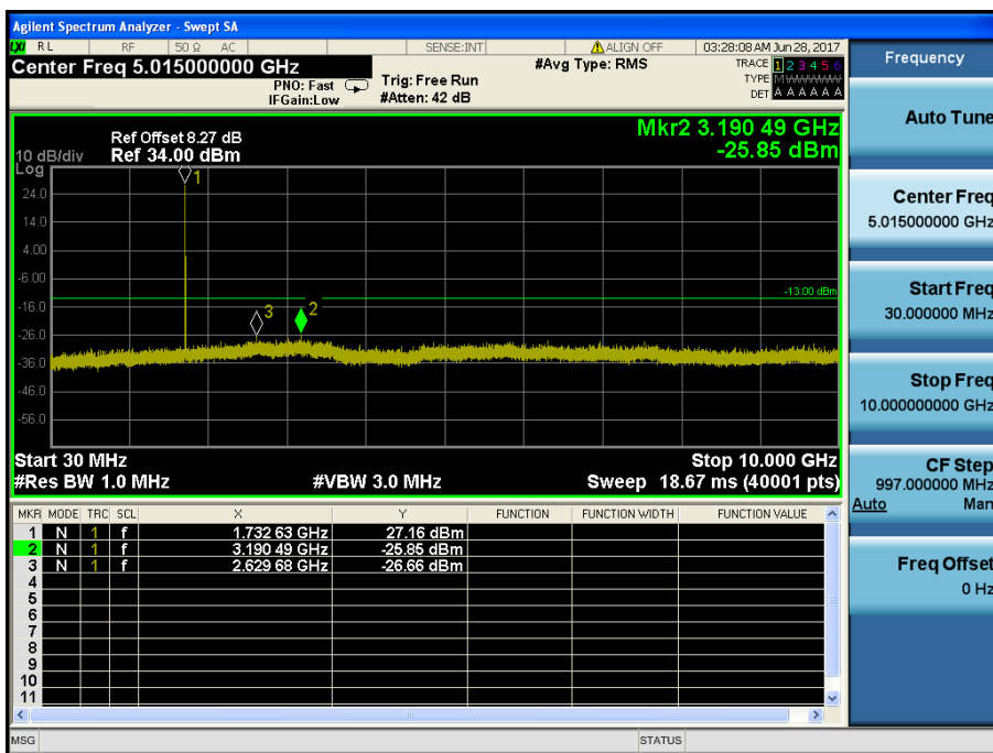
LTE Band 4 / 1.4MHz / QPSK - RB Size/Offset (6/0) – Mid Channel
