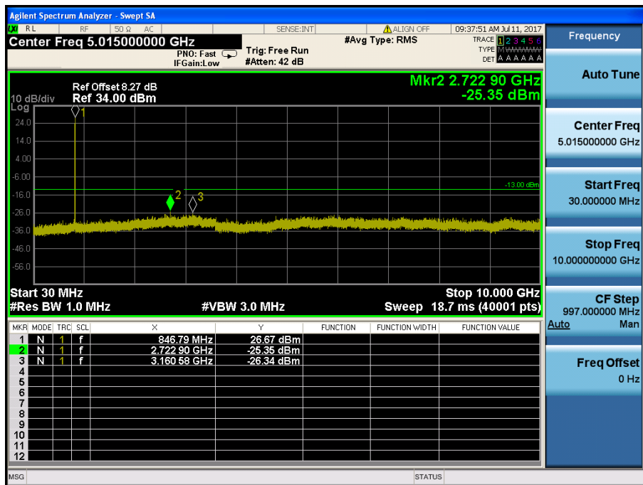
LTE Band 5 / 3MHz / 64QAM - RB Size/Offset (15/0) – High Channel
