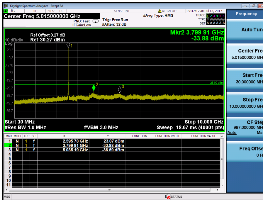
LTE Band 41 / 15MHz / QPSK - RB Size/Offset (36/39) – Mid Channel
