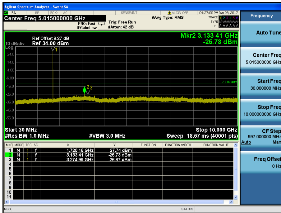
LTE Band 4 / 20MHz / 64QAM - RB Size/Offset (1/50) –Low Channel
