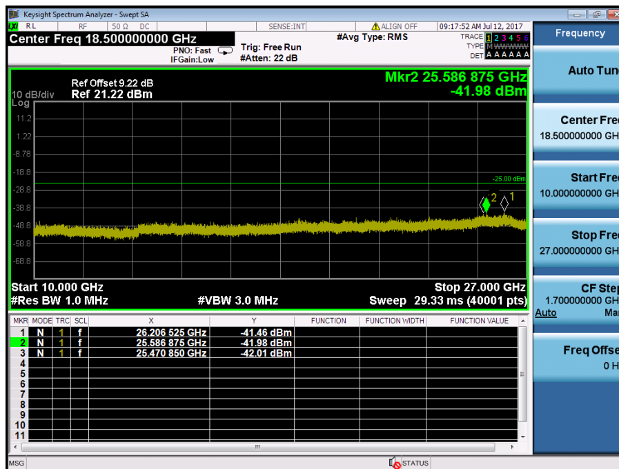
LTE Band 41 / 5MHz / QPSK - RB Size/Offset (12/13) – Mid Channel
