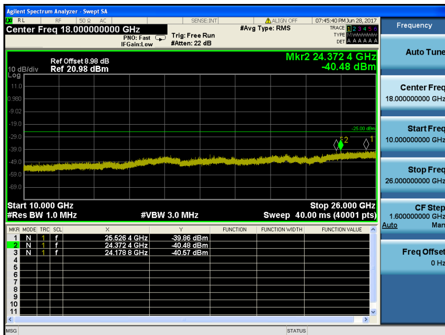
LTE Band 7 / 5MHz / 64QAM - RB Size/Offset (12/13) – Mid Channel
