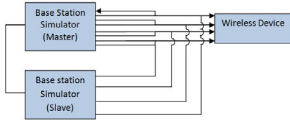
Figure I 1 Power Measurement Setup
