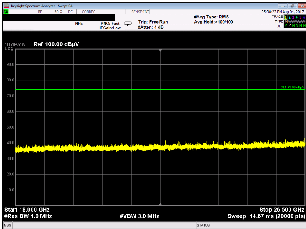
Plot 7-49. Radiated Spurious Plot above 18GHz (Pol. V)
