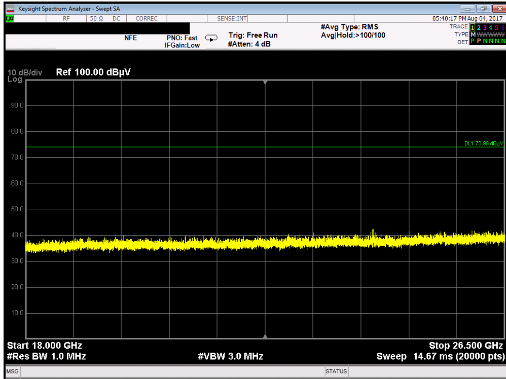
Plot 7-48. Radiated Spurious Plot above 18GHz (Pol. H)
