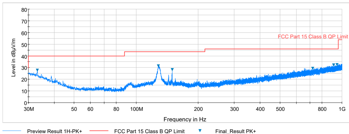
Plot 7-2. Radiated Spurious Plot 30MHz – 1GHz (Pol. V)
