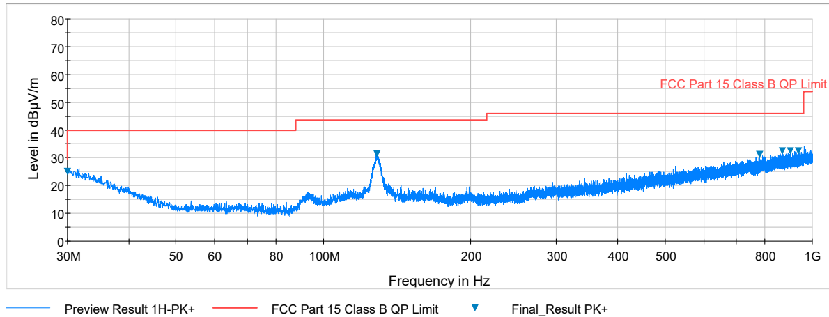
Plot 7-1. Radiated Spurious Plot 30MHz – 1GHz (Pol. H)
