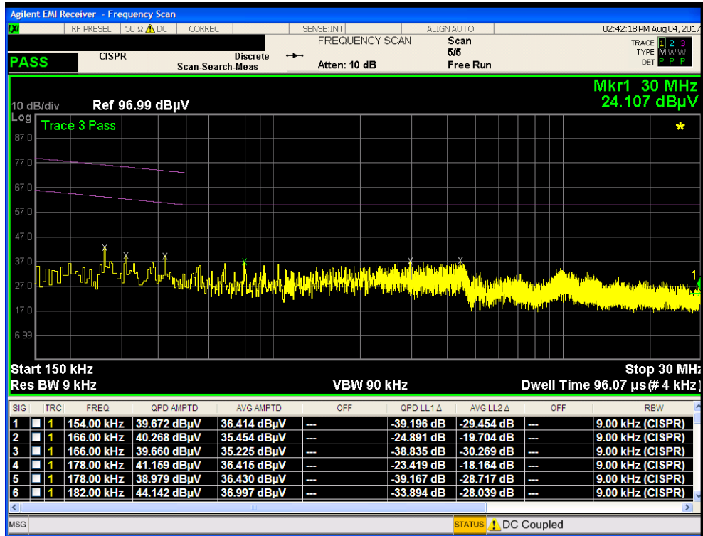
Plot 7-5. Line-Conducted Test Plot (L1) - With Antenna Terminated in 50 Ω
