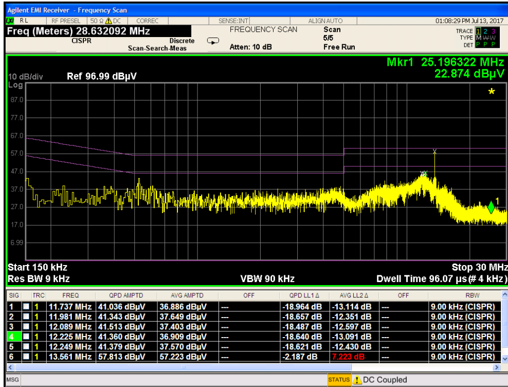
Plot 7-3. Line-Conducted Test Plot (L1) - With Antenna Connected
