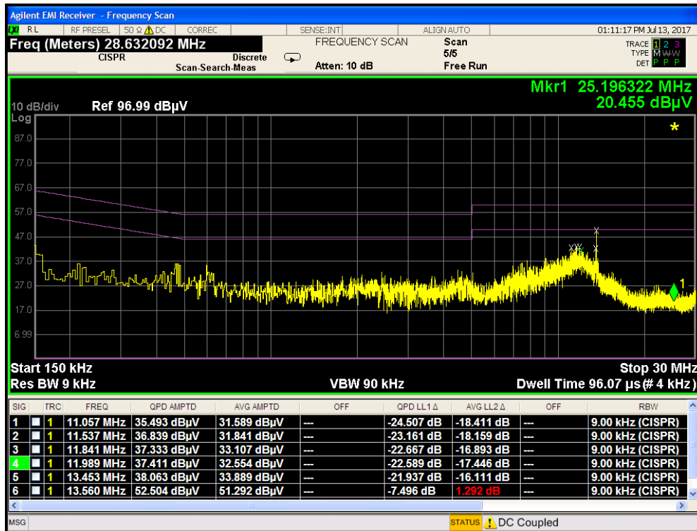
Plot 7-4. Line-Conducted Test Plot (N) – With Antenna Connected
