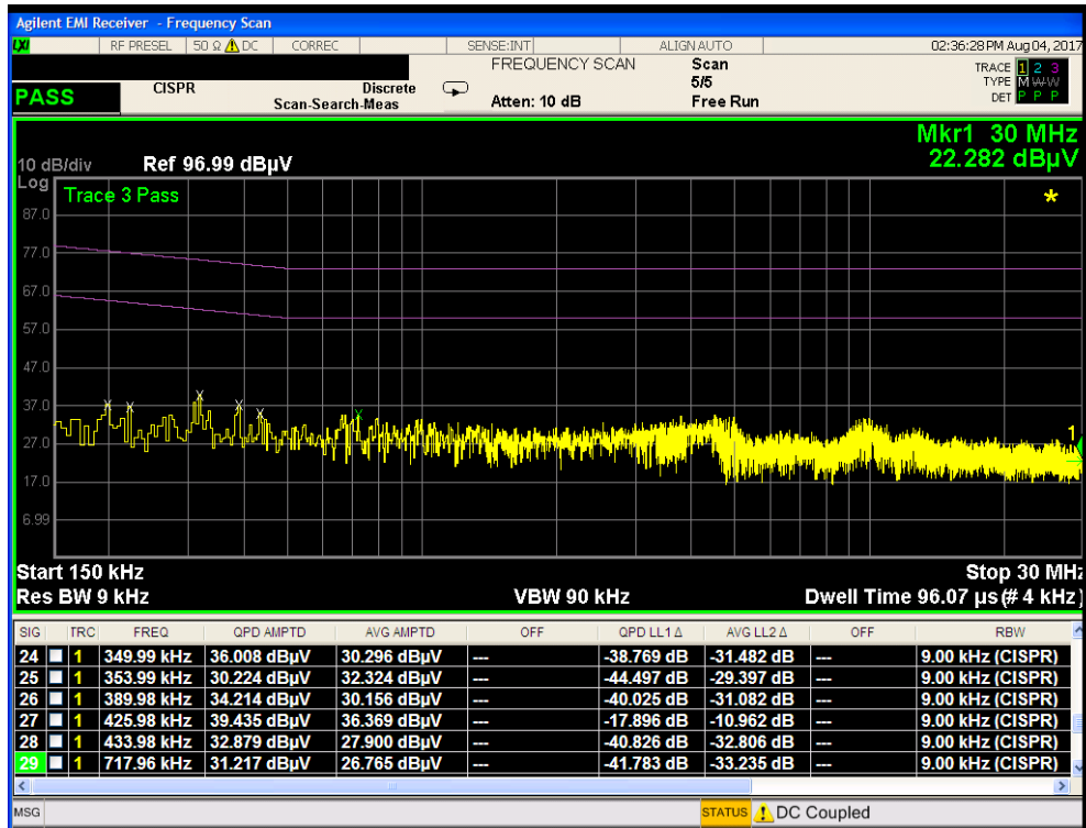
Plot 7-6. Line-Conducted Test Plot (N) - With Antenna Terminated in 50 Ω
