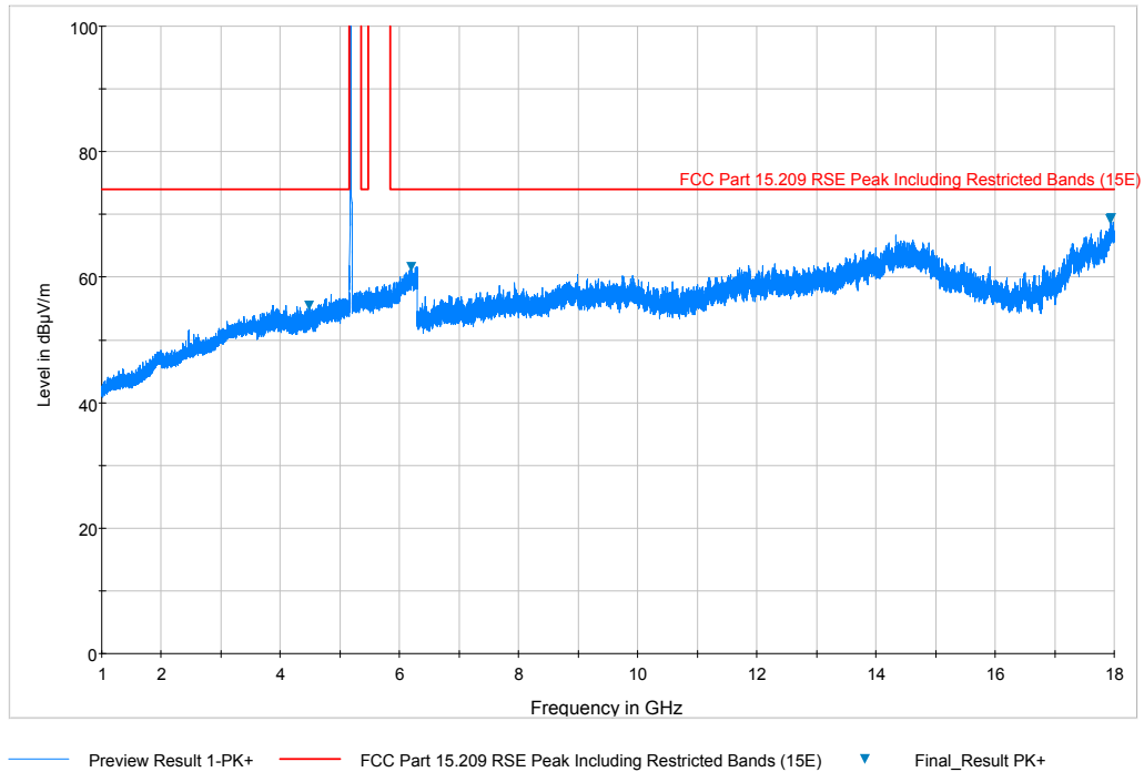
Plot 7-153. Radiated Spurious Plot above 1GHz (802.11a – U1 Ch. 40, Ant. Pol. H)
