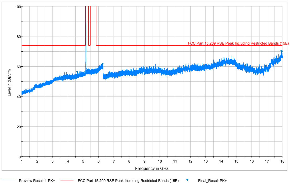
Plot 7-166. Radiated Spurious Plot above 1GHz (802.11a – U1 Ch. 40, Ant. Pol. V)
