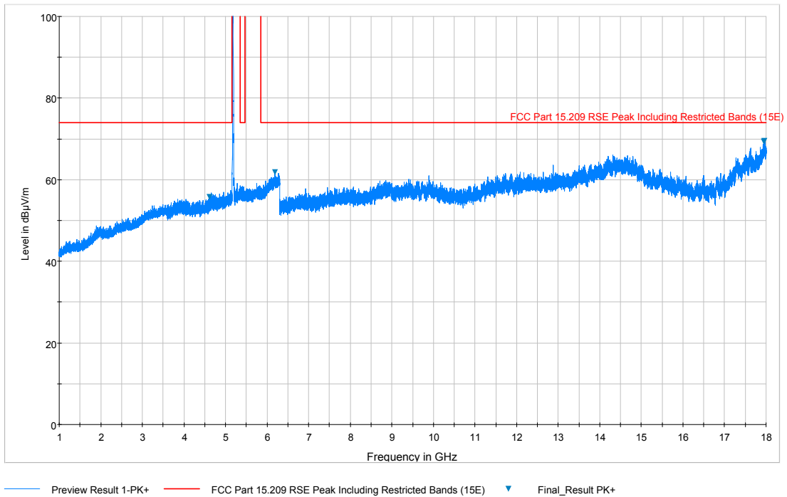
Plot 7-165. Radiated Spurious Plot above 1GHz (802.11a – U1 Ch. 40, Ant. Pol. H)
