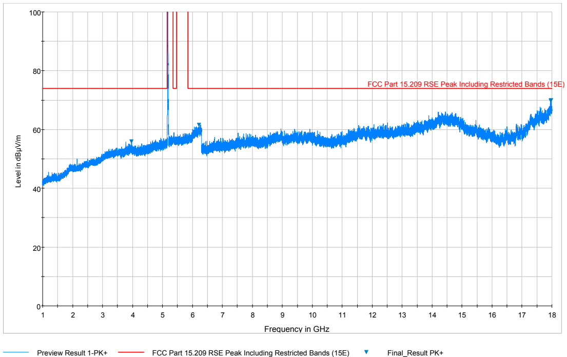
Plot 7-154. Radiated Spurious Plot above 1GHz (802.11a – U1 Ch. 40, Ant. Pol. V)
